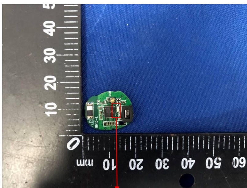
RF Antenna
