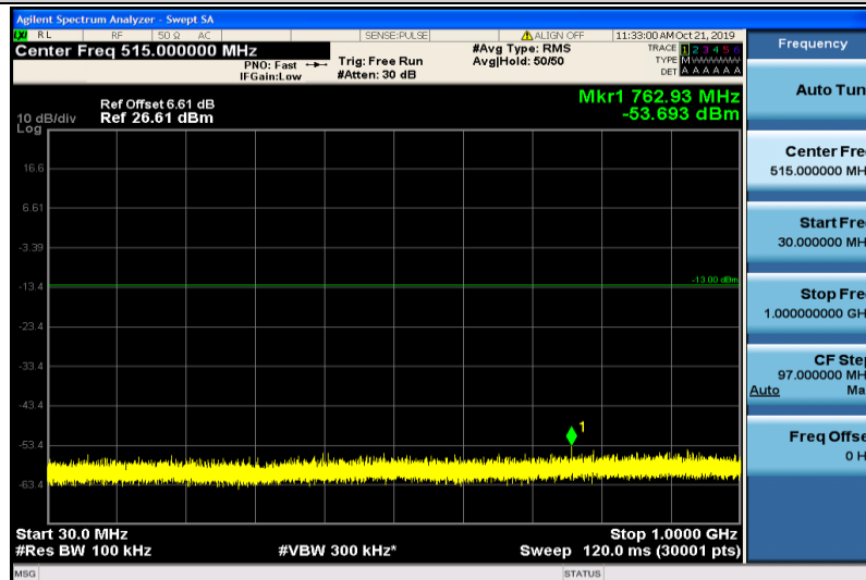
Band4-3MHz-16QAM-20175-1RB#0-30~1000MHz
