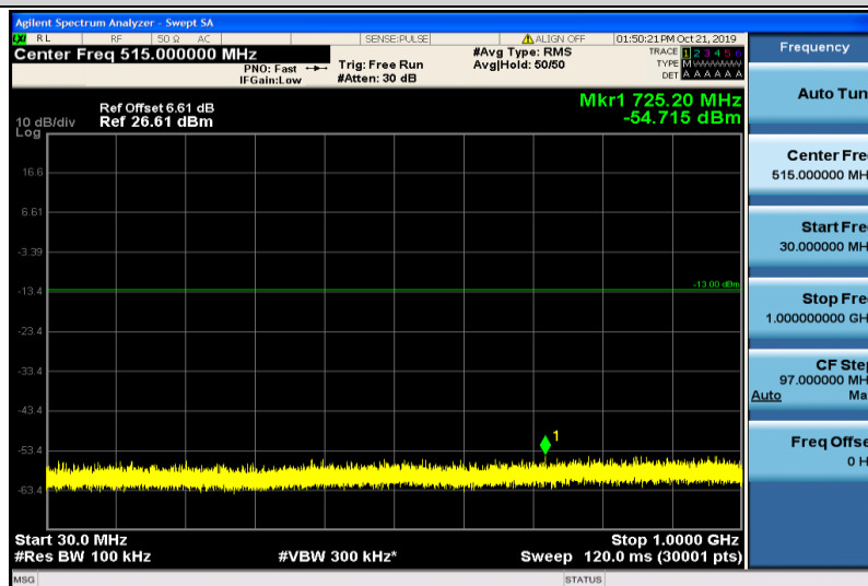
Band4-5MHz-16QAM-20175-1RB#0-30~1000MHz
