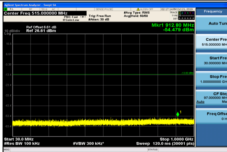
Band4-10MHz-16QAM-20000-1RB#0-30~1000MHz
