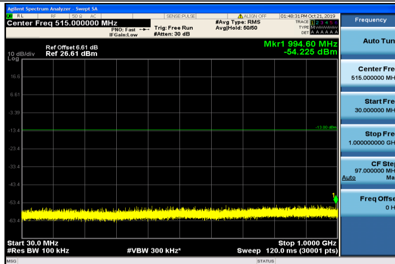
Band4-5MHz-QPSK-19975-1RB#0-30~1000MHz
