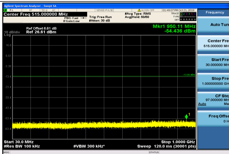
Band4-5MHz-16QAM-19975-1RB#0-30~1000MHz
