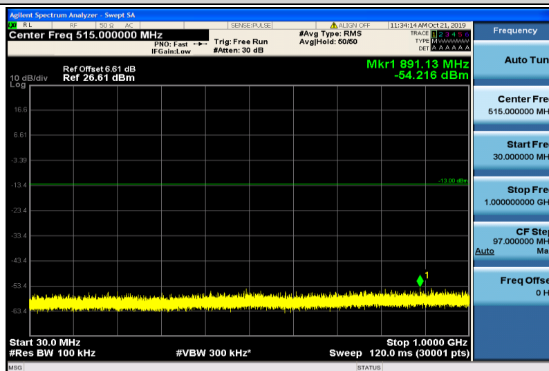
Band4-3MHz-16QAM-20385-1RB#0-30~1000MHz
