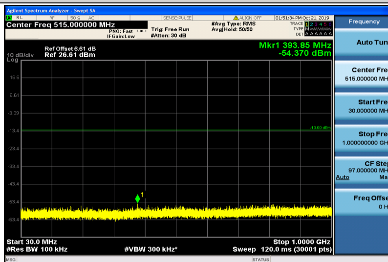
Band4-5MHz-16QAM-20375-1RB#0-30~1000MHz
