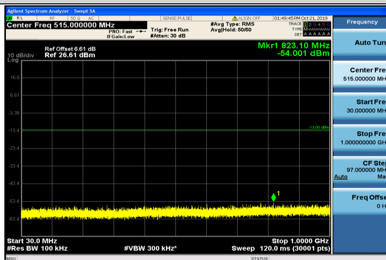
Band4-5MHz-QPSK-20175-1RB#0-30~1000MHz
