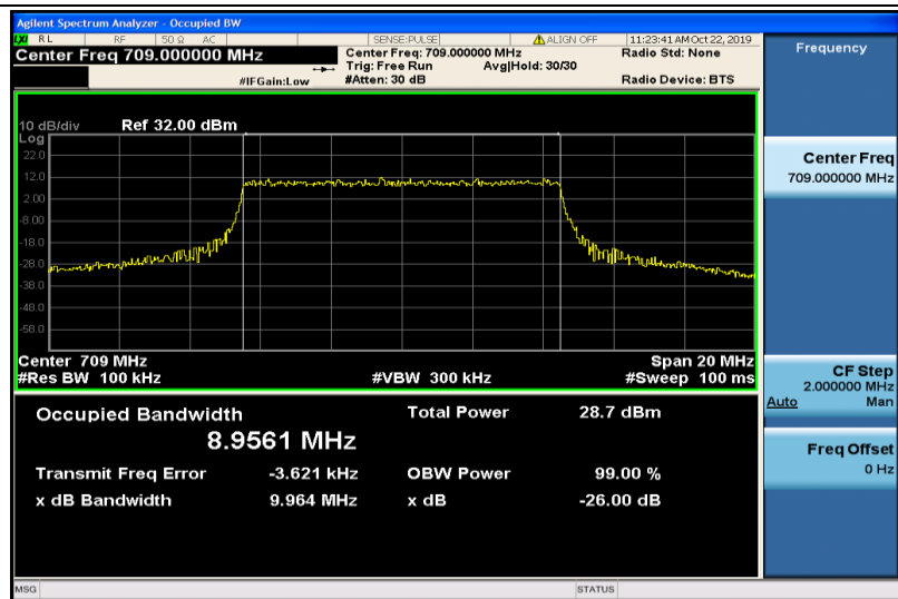
Band17-10MHz-16QAM-23780-50RB#0-8.9561
