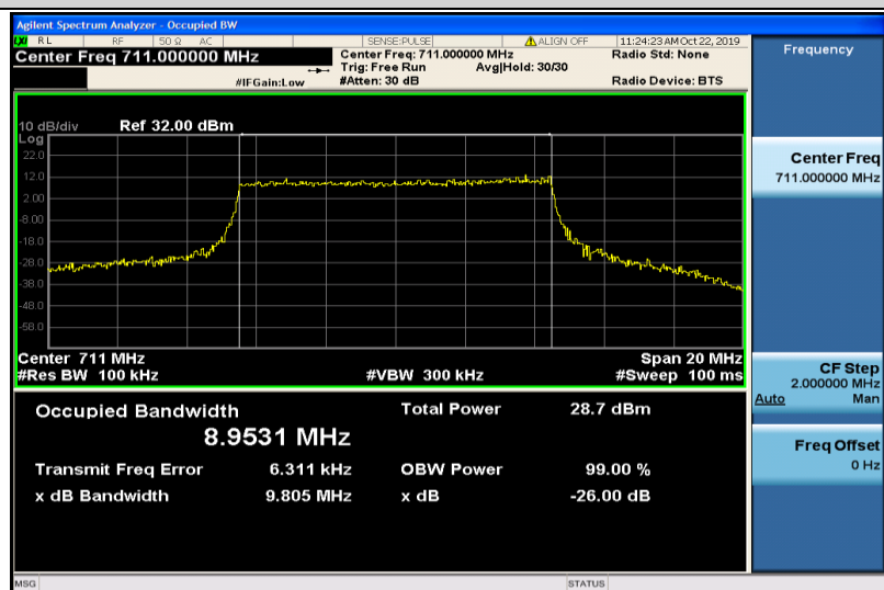
Band17-10MHz-16QAM-23800-50RB#0-8.9531
