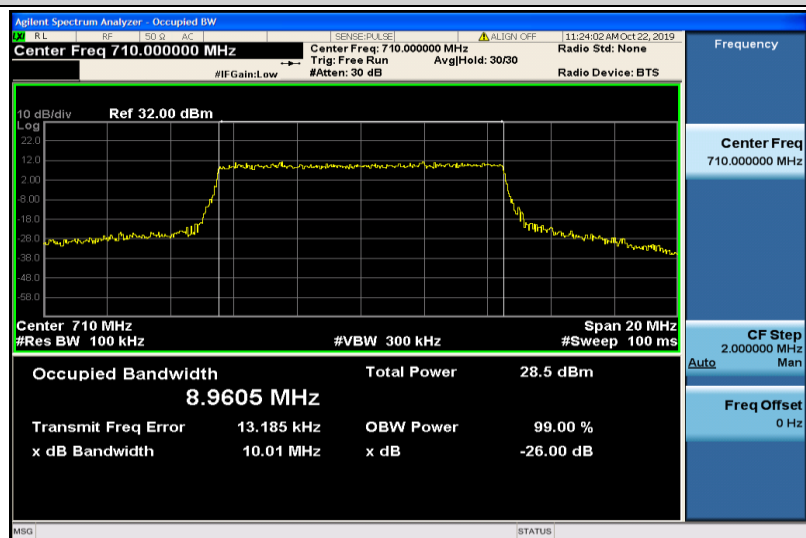
Band17-10MHz-16QAM-23790-50RB#0-8.9605
