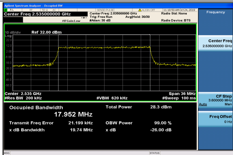
Band7-20MHz-16QAM-21100-100RB#0-17.952
