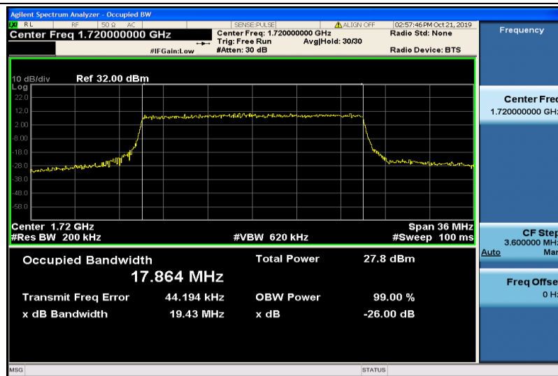
Band4-20MHz-16QAM-20050-100RB#0-17.864
