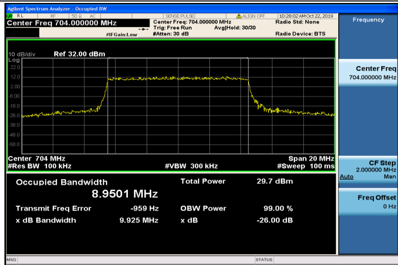
Band12-10MHz-QPSK-23060-50RB#0-8.9501
