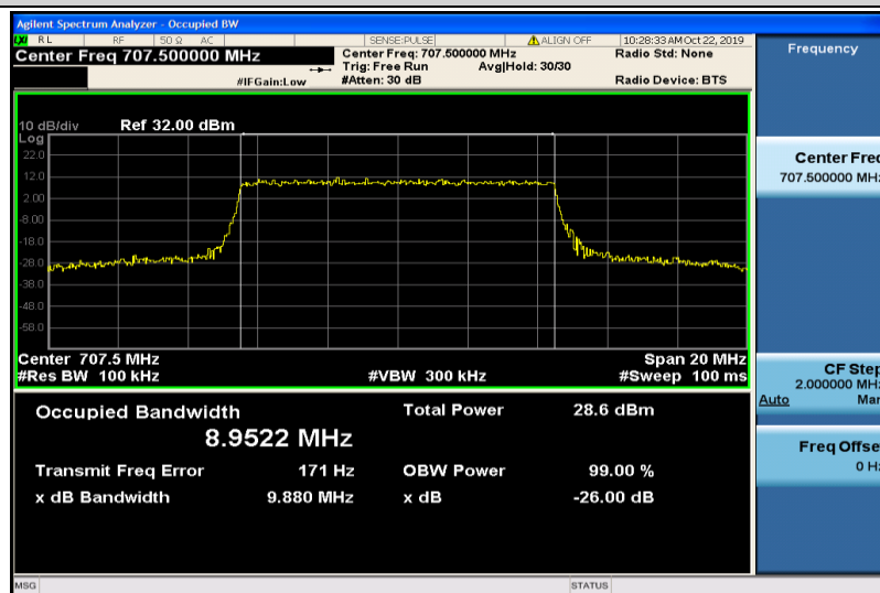
Band12-10MHz-16QAM-23095-50RB#0-8.9522
