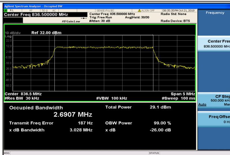
Band5-3MHz-QPSK-20525-15RB#0-2.6907
