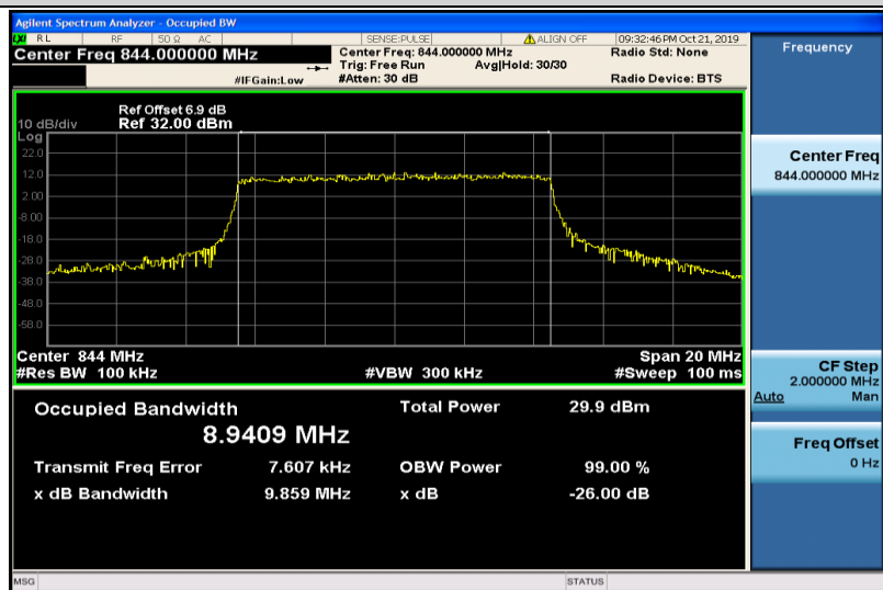
Band5-10MHz-QPSK-20600-50RB#0-8.9409
