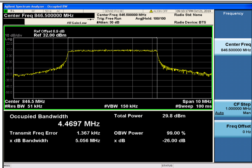
Band5-5MHz-QPSK-20625-25RB#0-4.4697
