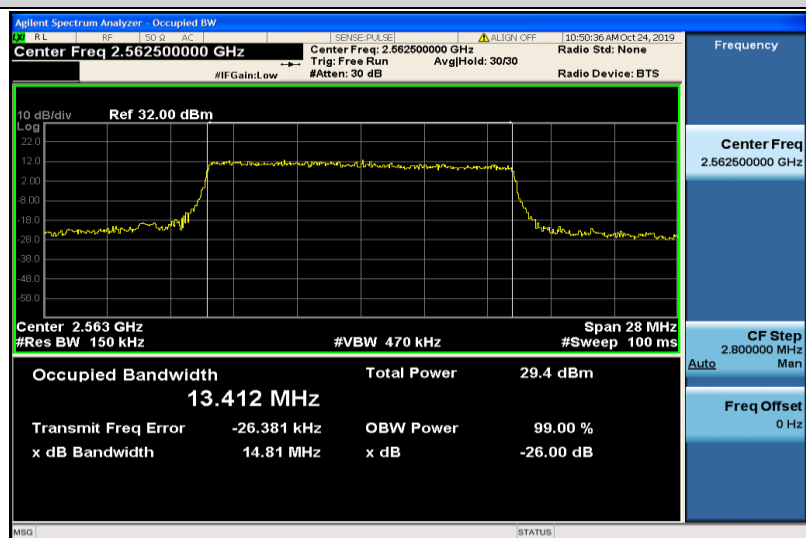
Band7-15MHz-QPSK-21375-75RB#0-13.412
