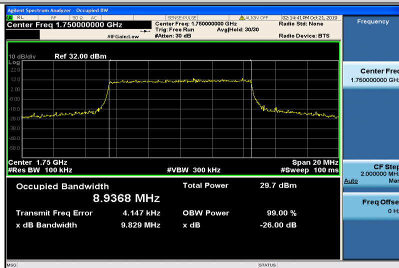
Band4-10MHz-QPSK-20350-50RB#0-8.9368
