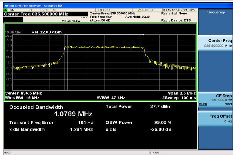
Band5-1.4MHz-16QAM-20525-6RB#0-1.0789
