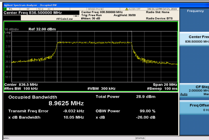
Band5-10MHz-16QAM-20525-50RB#0-8.9625
