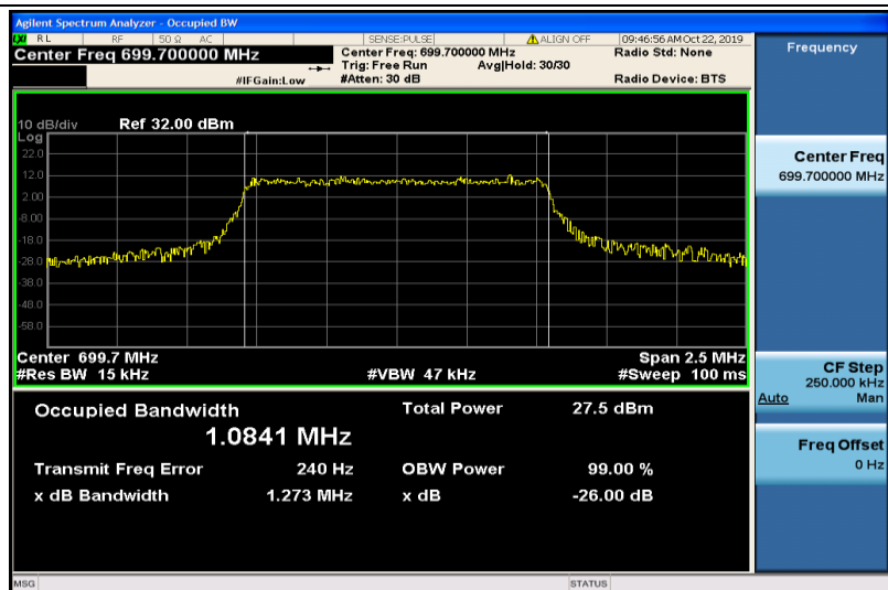
Band12-1.4MHz-16QAM-23017-6RB#0-1.0841
