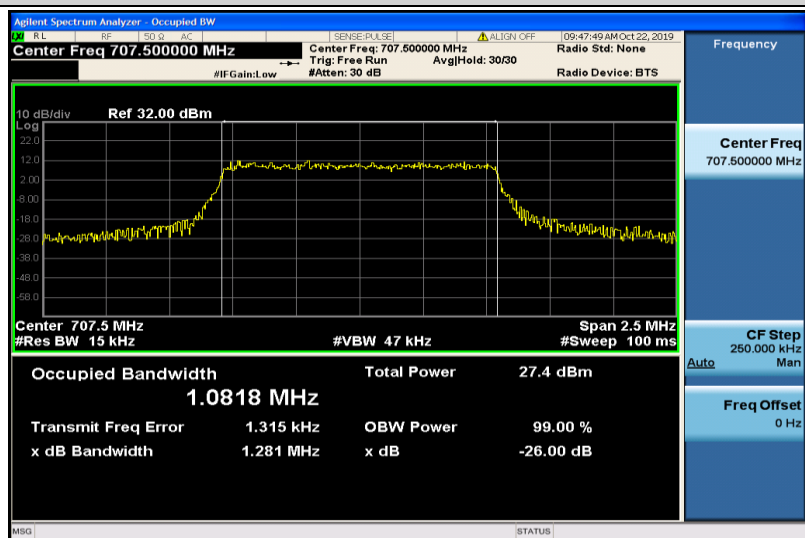
Band12-1.4MHz-16QAM-23095-6RB#0-1.0818
