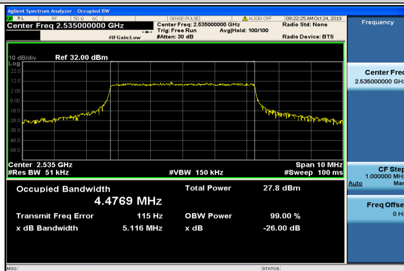
Band7-5MHz-QPSK-21100-25RB#0-4.4769
