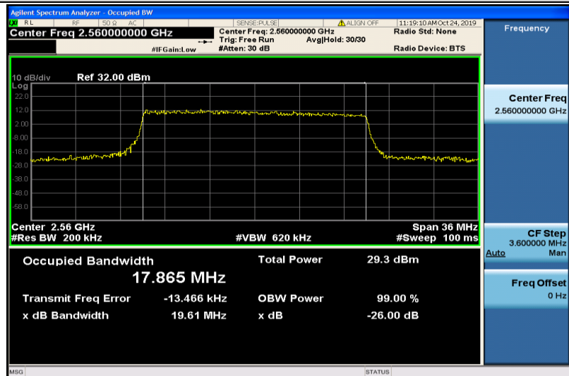
Band7-20MHz-16QAM-21350-100RB#0-17.865
