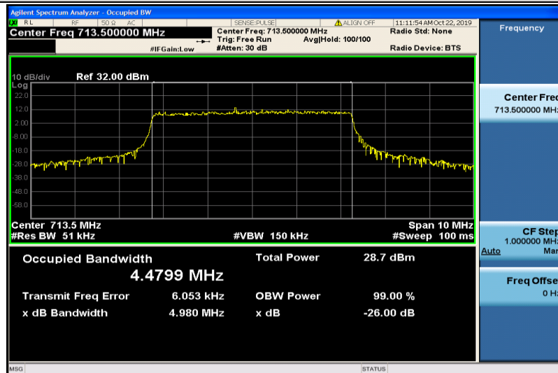
Band17-5MHz-16QAM-23825-25RB#0-4.4799
