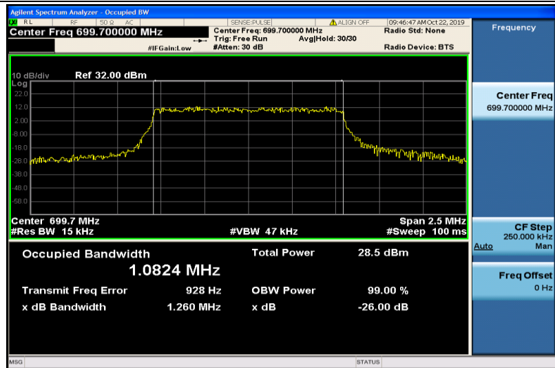
Band12-1.4MHz-QPSK-23017-6RB#0-1.0824
