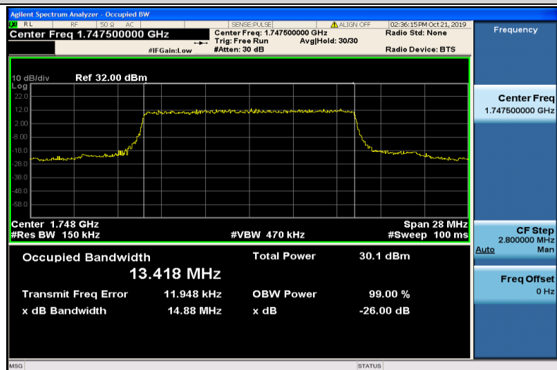
Band4-15MHz-QPSK-20325-75RB#0-13.418
