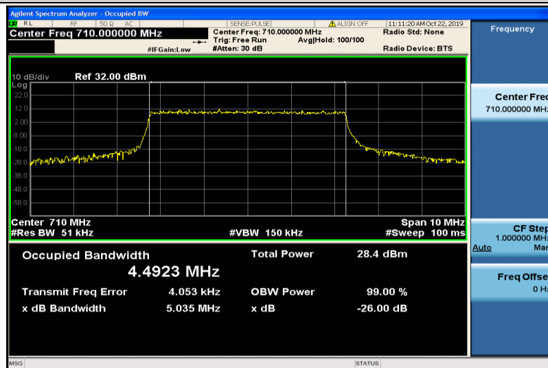
Band17-5MHz-16QAM-23790-25RB#0-4.4923
