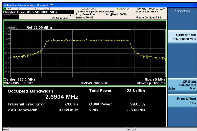
Band5-3MHz-16QAM-20415-15RB#0-2.6904
