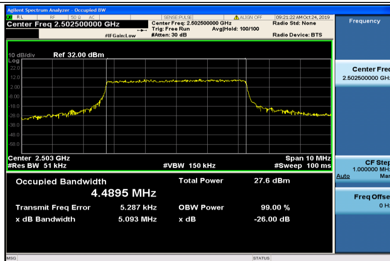
Band7-5MHz-QPSK-20775-25RB#0-4.4895
