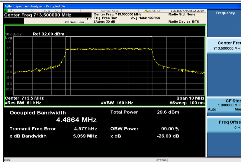
Band17-5MHz-QPSK-23825-25RB#0-4.4864
