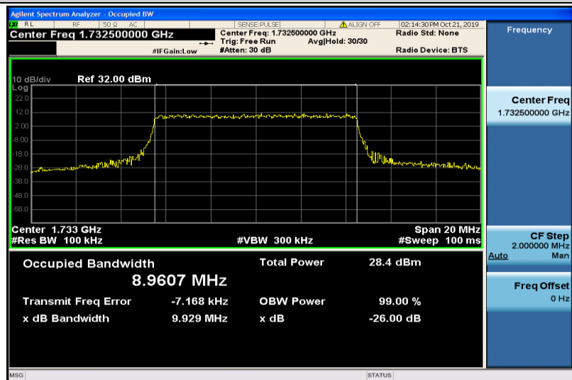
Band4-10MHz-16QAM-20175-50RB#0-8.9607
