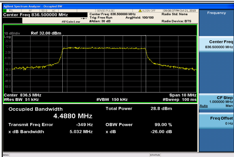
Band5-5MHz-16QAM-20525-25RB#0-4.4880
