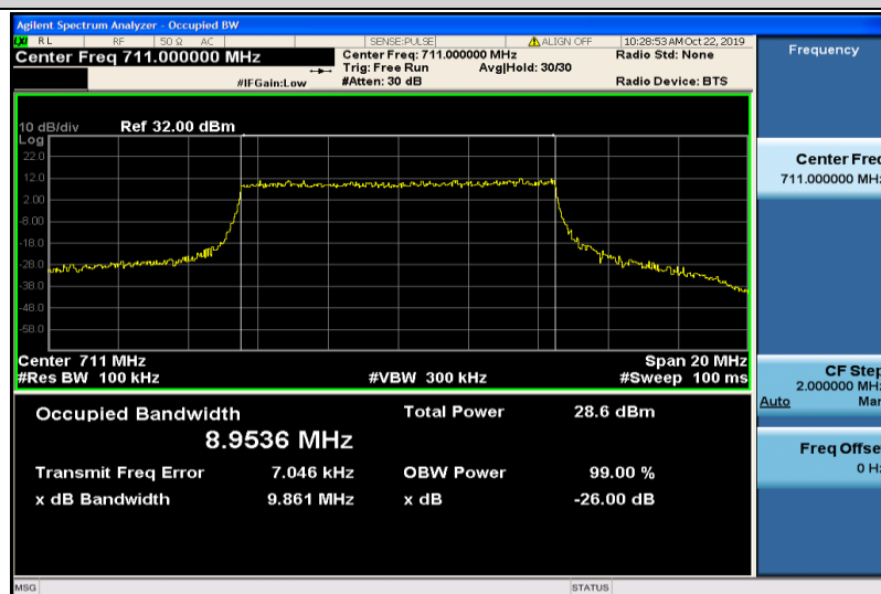
Band12-10MHz-16QAM-23130-50RB#0-8.9536
