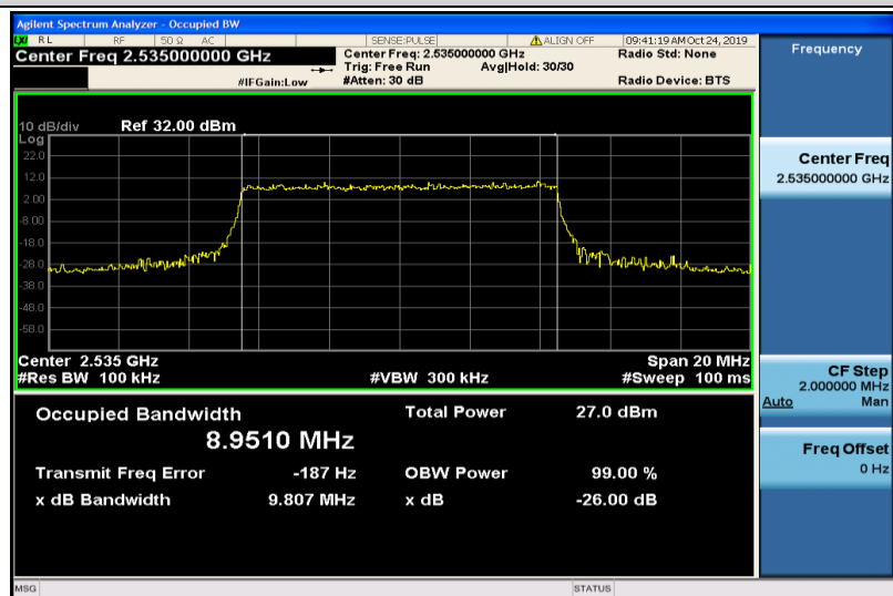
Band7-10MHz-QPSK-21100-50RB#0-8.9510
