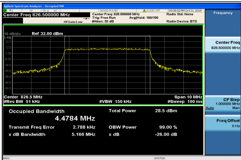
Band5-5MHz-16QAM-20425-25RB#0-4.4784
