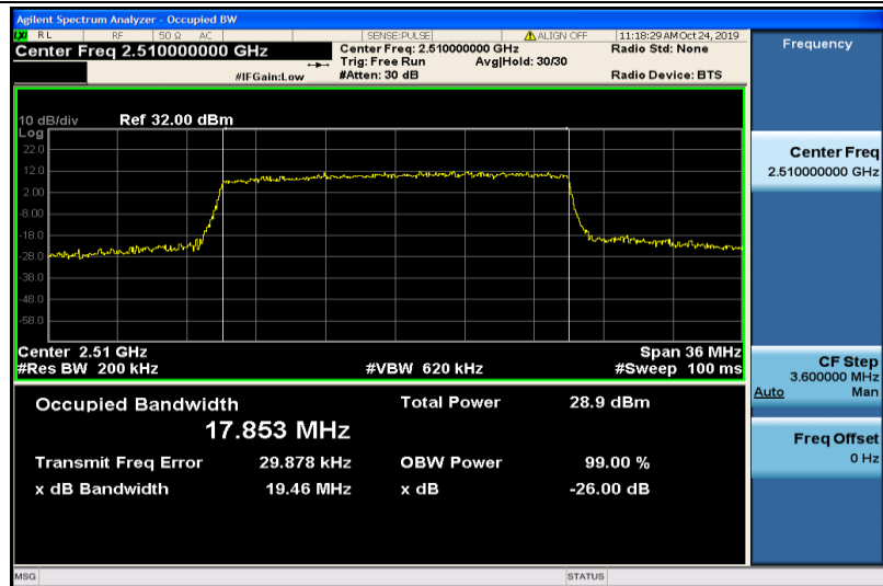
Band7-20MHz-16QAM-20850-100RB#0-17.853
