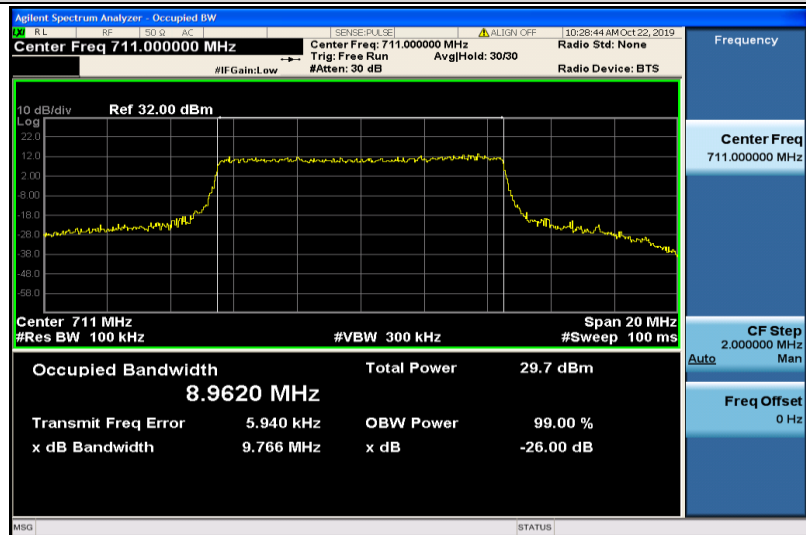
Band12-10MHz-QPSK-23130-50RB#0-8.9620
