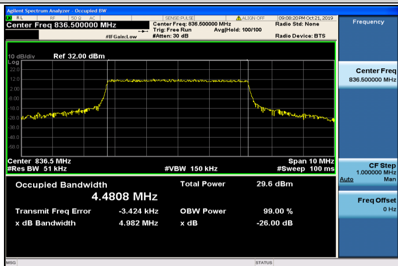
Band5-5MHz-QPSK-20525-25RB#0-4.4808
