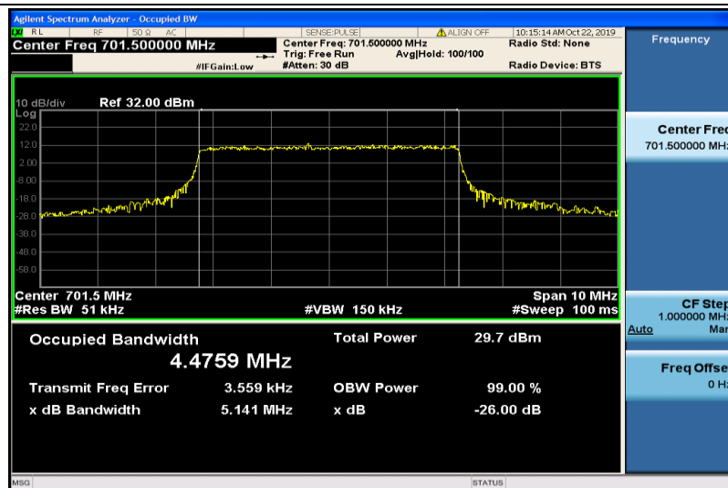
Band12-5MHz-QPSK-23035-25RB#0-4.4759
