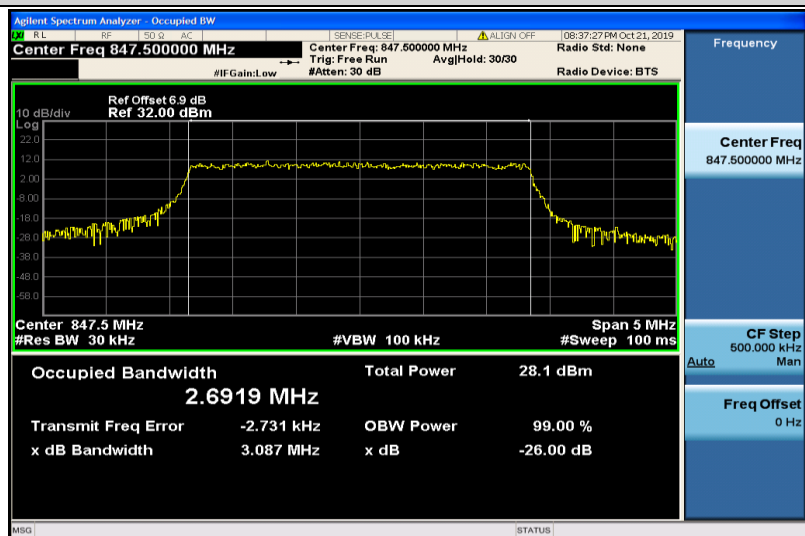
Band5-3MHz-16QAM-20635-15RB#0-2.6919
