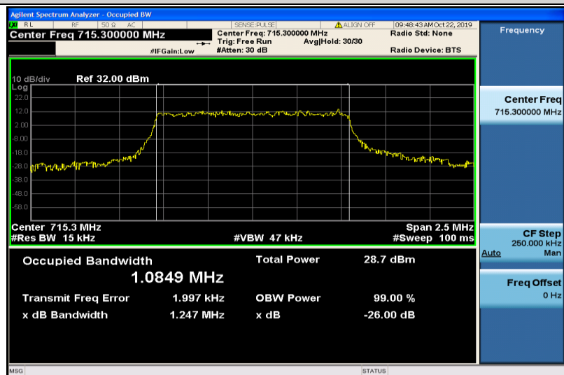
Band12-1.4MHz-QPSK-23173-6RB#0-1.0849
