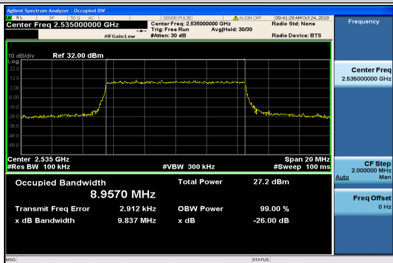
Band7-10MHz-16QAM-21100-50RB#0-8.9570
