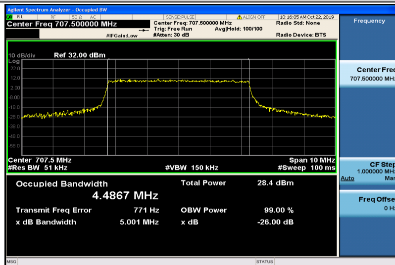
Band12-5MHz-16QAM-23095-25RB#0-4.4867
