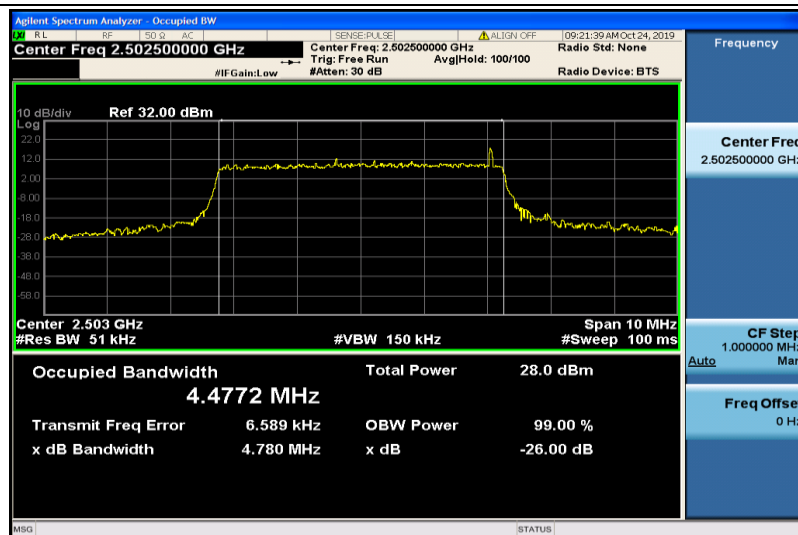
Band7-5MHz-16QAM-20775-25RB#0-4.4772
