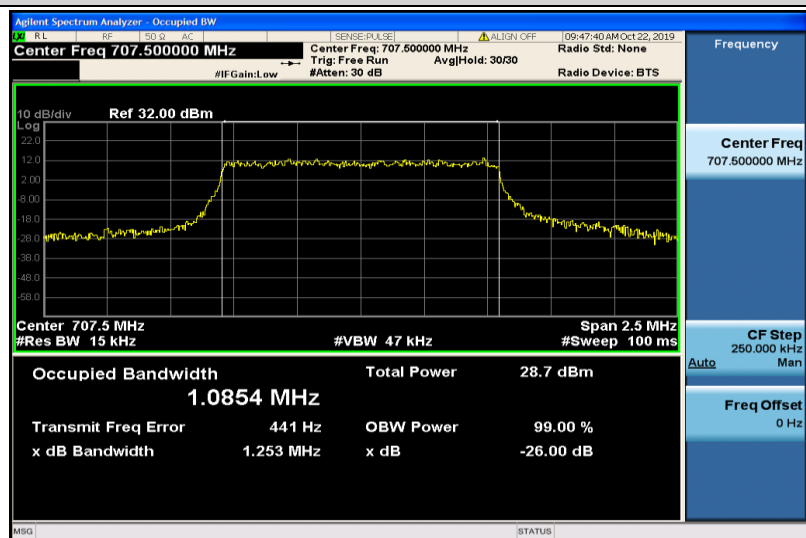
Band12-1.4MHz-QPSK-23095-6RB#0-1.0854
