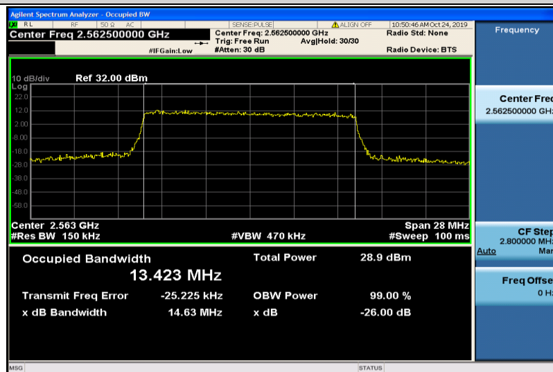
Band7-15MHz-16QAM-21375-75RB#0-13.423
