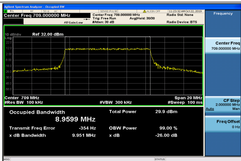
Band17-10MHz-QPSK-23780-50RB#0-8.9599
