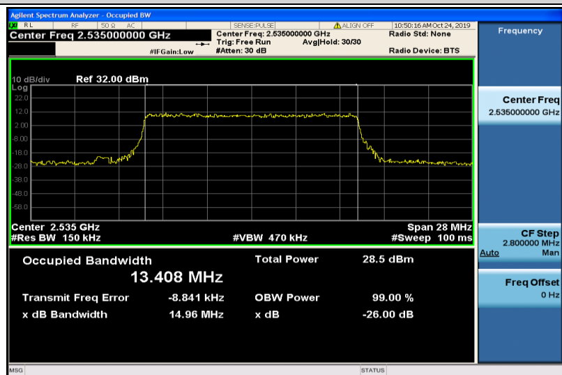
Band7-15MHz-QPSK-21100-75RB#0-13.408
