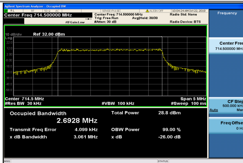
Band12-3MHz-QPSK-23165-15RB#0-2.6928
