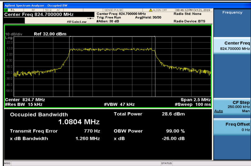
Band5-1.4MHz-QPSK-20407-6RB#0-1.0804
