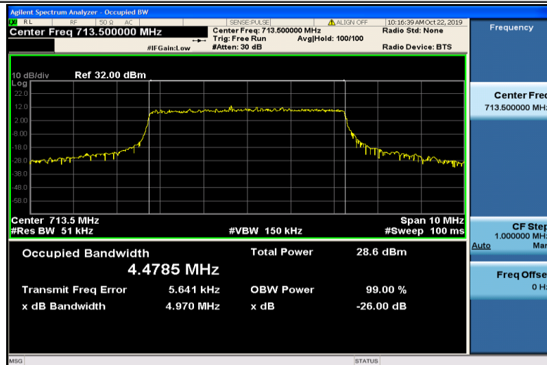
Band12-5MHz-16QAM-23155-25RB#0-4.4785
