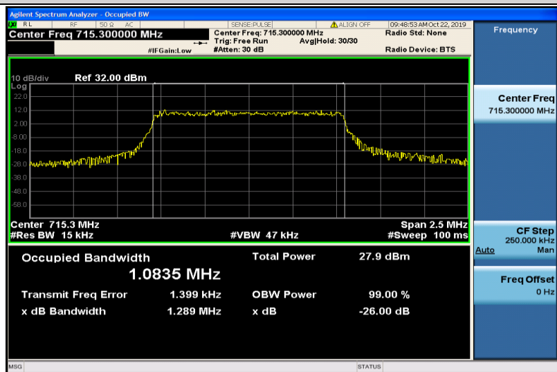
Band12-1.4MHz-16QAM-23173-6RB#0-1.0835
