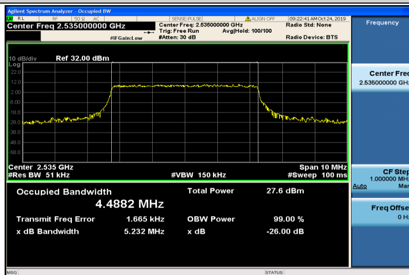
Band7-5MHz-16QAM-21100-25RB#0-4.4882
