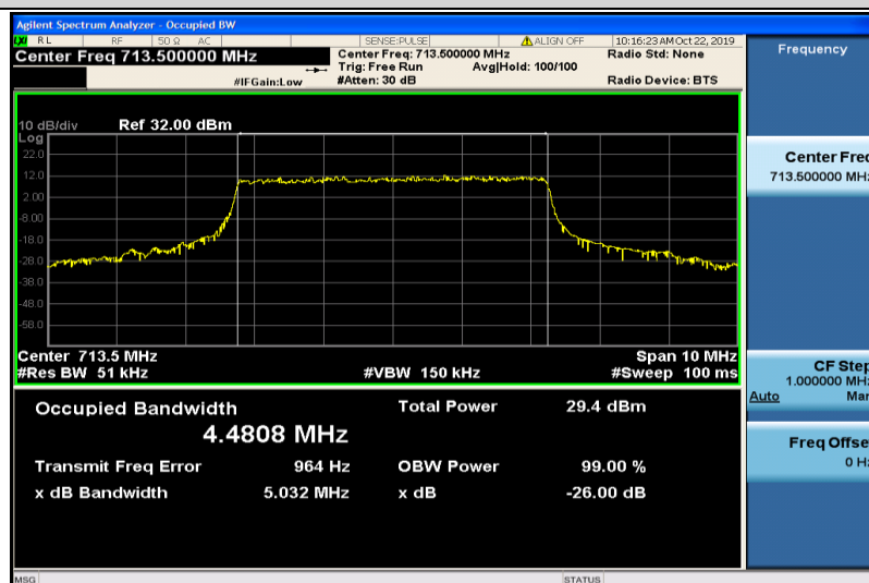
Band12-5MHz-QPSK-23155-25RB#0-4.4808
