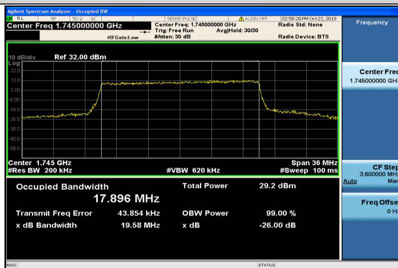
Band4-20MHz-16QAM-20300-100RB#0-17.896
