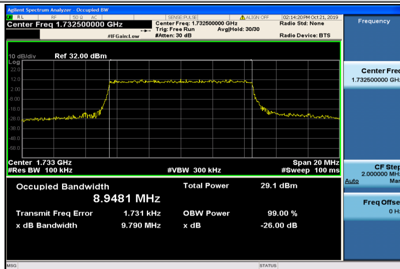
Band4-10MHz-QPSK-20175-50RB#0-8.9481
