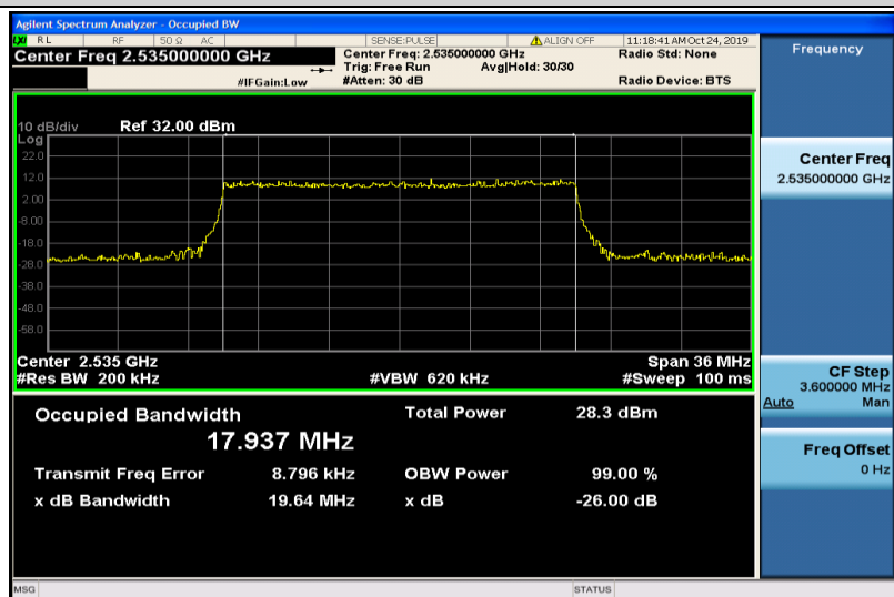
Band7-20MHz-QPSK-21100-100RB#0-17.937
