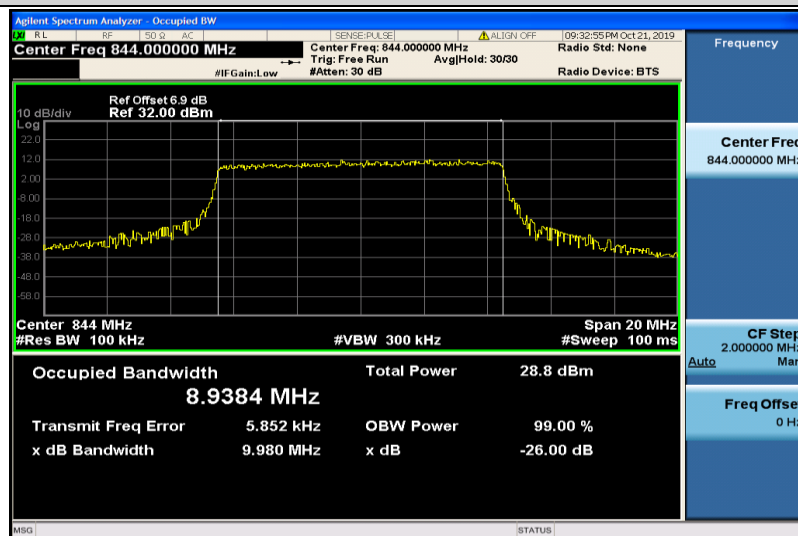
Band5-10MHz-16QAM-20600-50RB#0-8.9384
