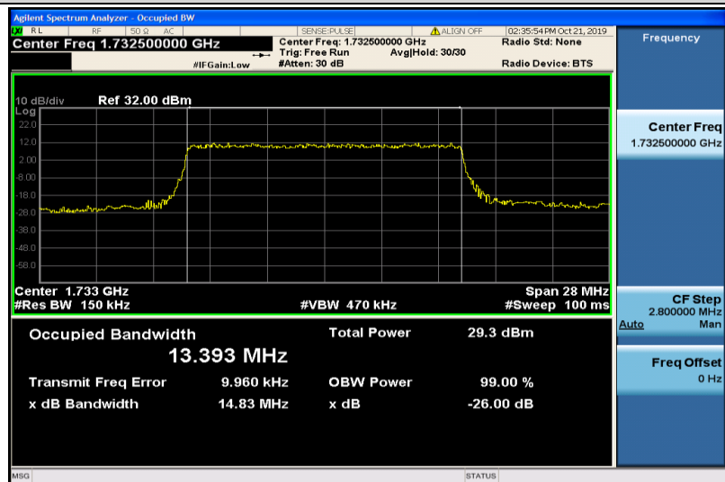
Band4-15MHz-QPSK-20175-75RB#0-13.393
