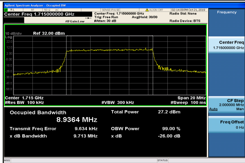
Band4-10MHz-16QAM-20000-50RB#0-8.9364
