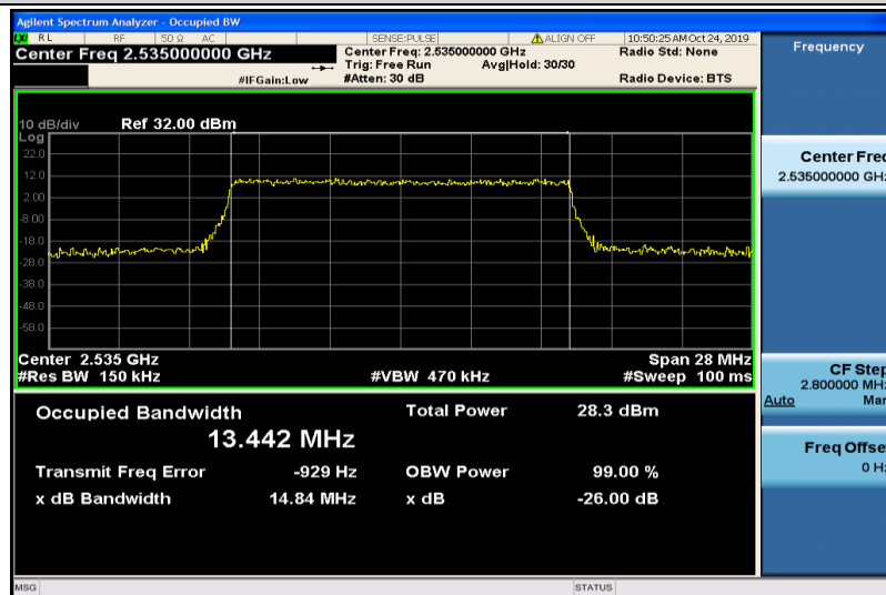
Band7-15MHz-16QAM-21100-75RB#0-13.442
