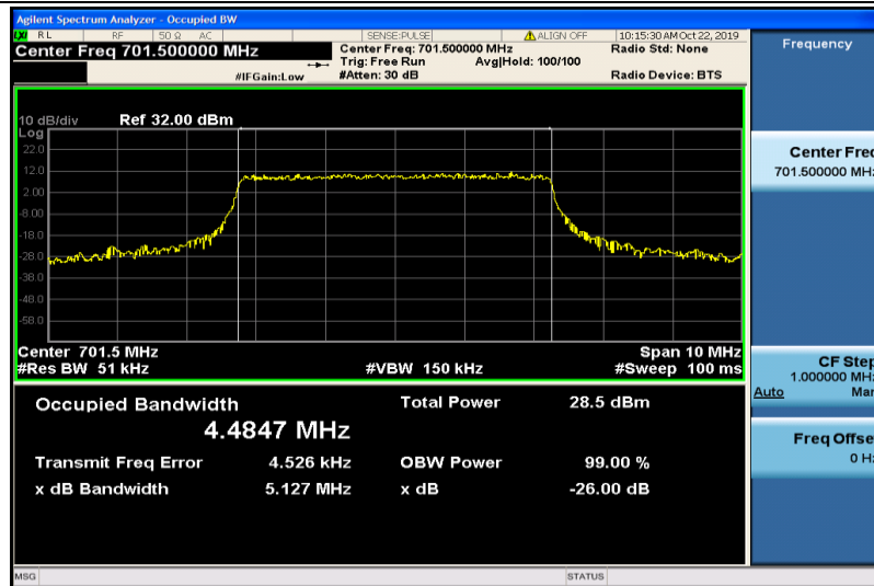
Band12-5MHz-16QAM-23035-25RB#0-4.4847
