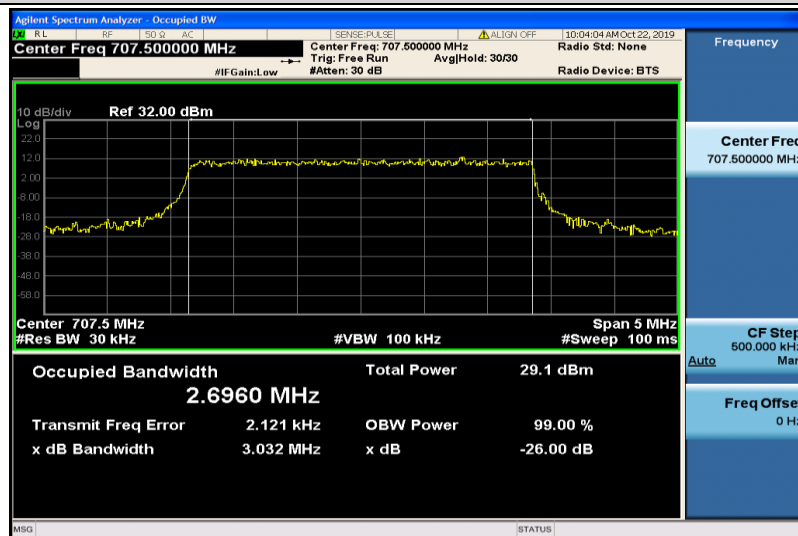
Band12-3MHz-QPSK-23095-15RB#0-2.6960
