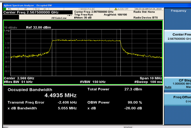
Band7-5MHz-16QAM-21425-25RB#0-4.4935
