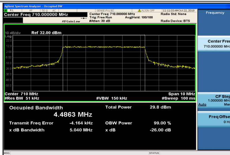
Band17-5MHz-QPSK-23790-25RB#0-4.4863
