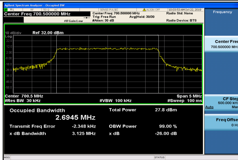
Band12-3MHz-16QAM-23025-15RB#0-2.6945
