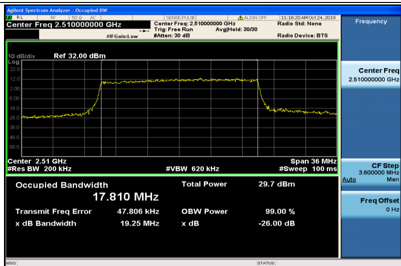
Band7-20MHz-QPSK-20850-100RB#0-17.810
