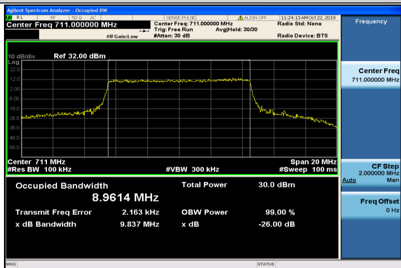
Band17-10MHz-QPSK-23800-50RB#0-8.9614
