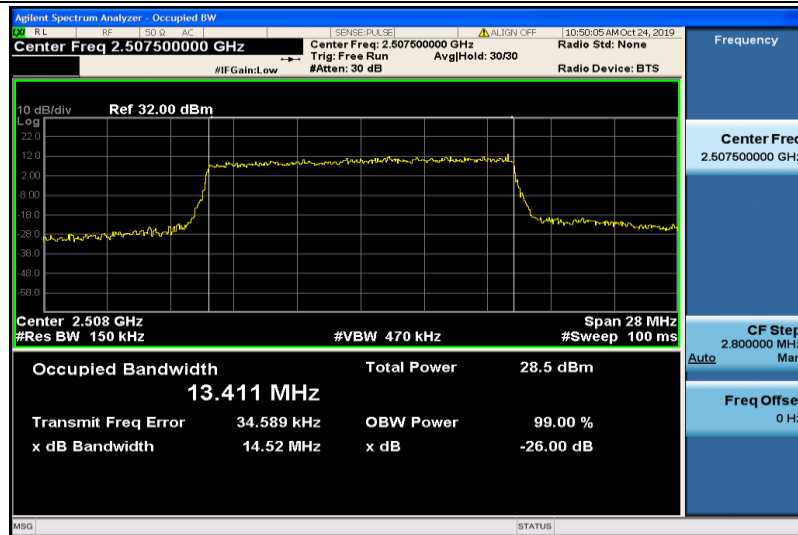
Band7-15MHz-16QAM-20825-75RB#0-13.411
