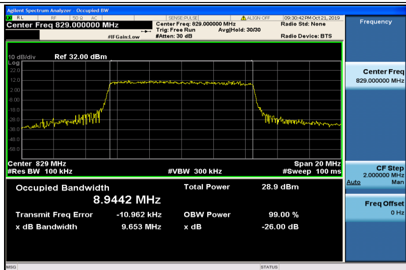
Band5-10MHz-QPSK-20450-50RB#0-8.9442
