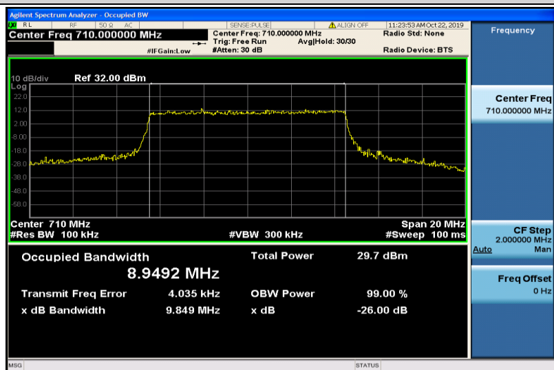
Band17-10MHz-QPSK-23790-50RB#0-8.9492
