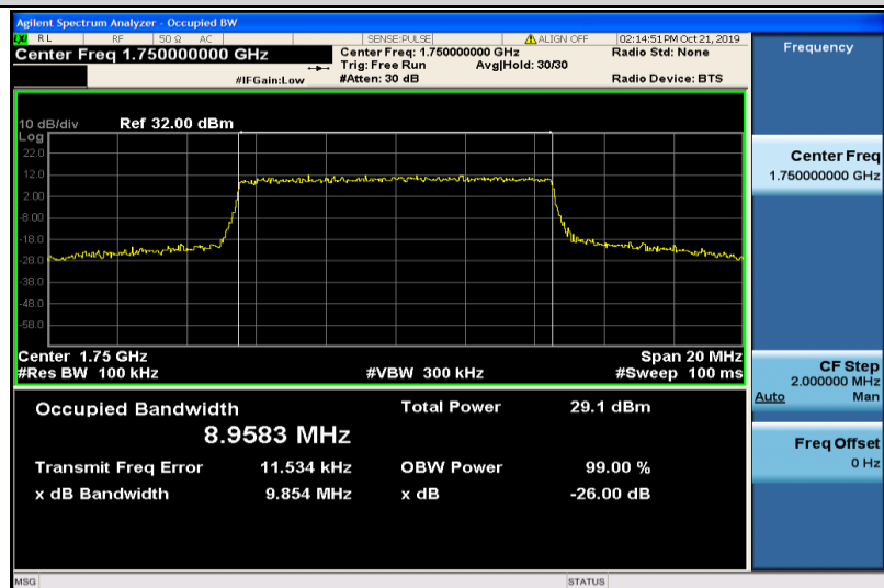
Band4-10MHz-16QAM-20350-50RB#0-8.9583
