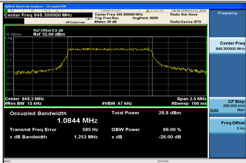
Band5-1.4MHz-QPSK-20643-6RB#0-1.0844
