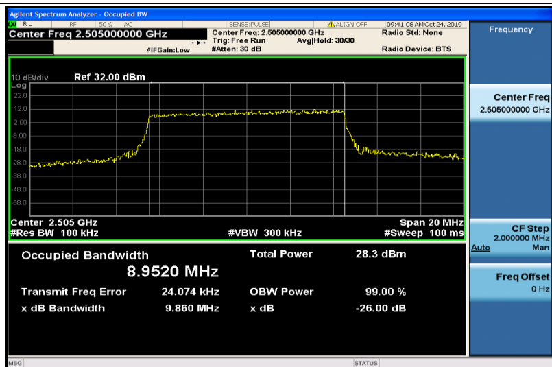
Band7-10MHz-16QAM-20800-50RB#0-8.9520
