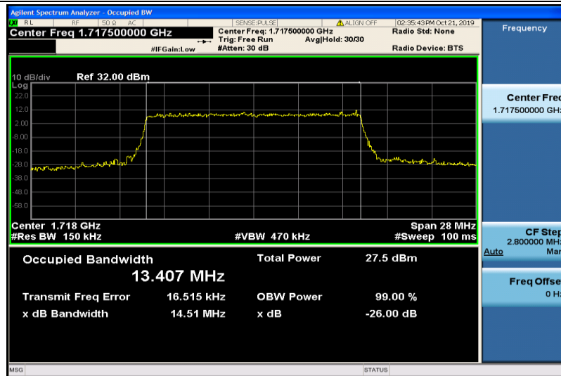
Band4-15MHz-16QAM-20025-75RB#0-13.407
