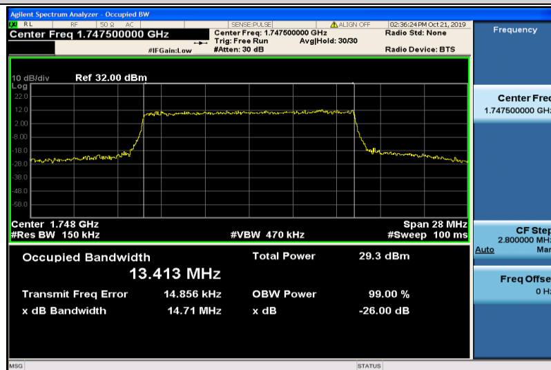
Band4-15MHz-16QAM-20325-75RB#0-13.413
