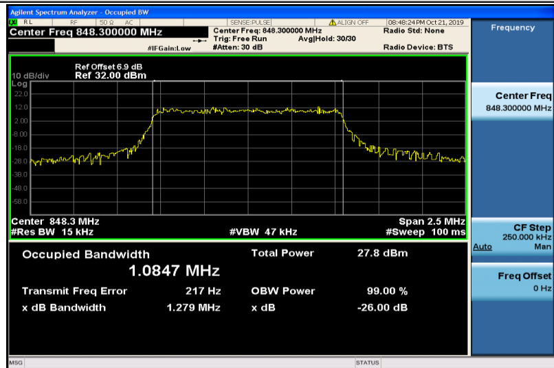
Band5-1.4MHz-16QAM-20643-6RB#0-1.0847
