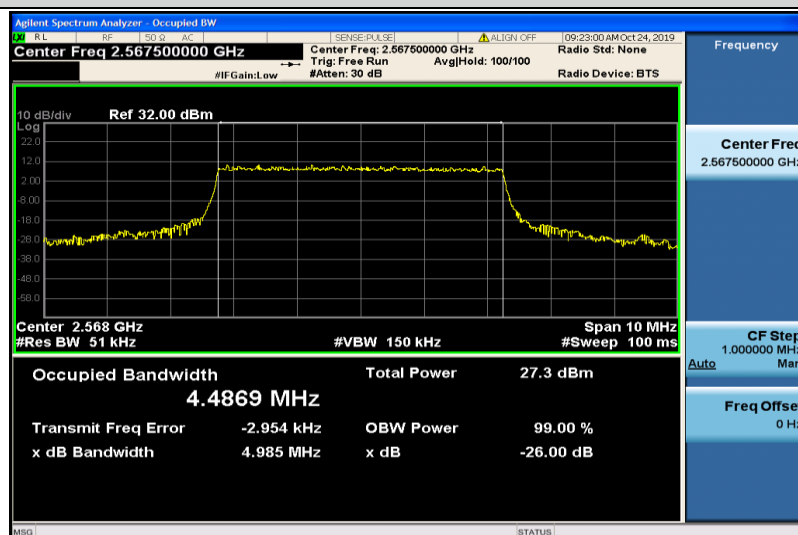
Band7-5MHz-QPSK-21425-25RB#0-4.4869
