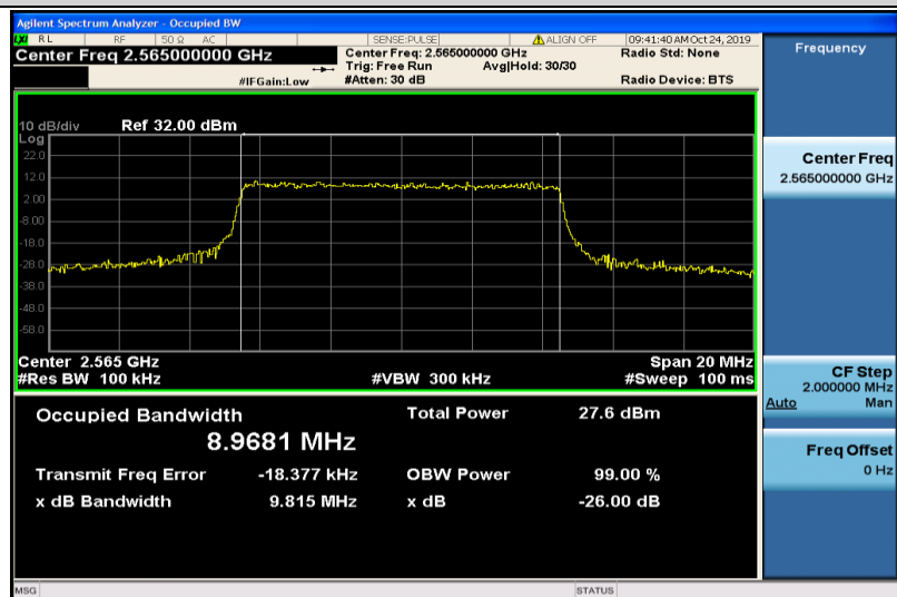
Band7-10MHz-QPSK-21400-50RB#0-8.9681
