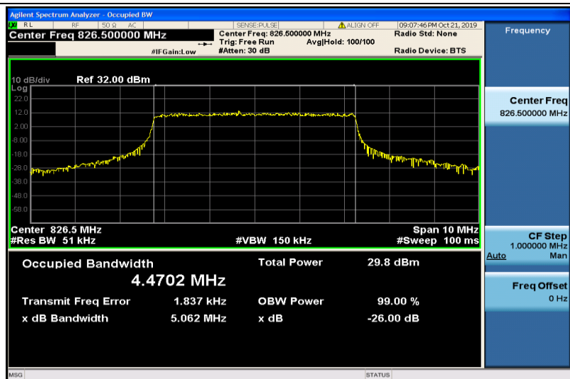
Band5-5MHz-QPSK-20425-25RB#0-4.4702
