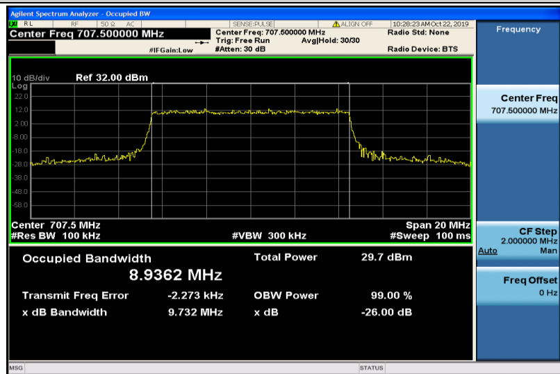
Band12-10MHz-QPSK-23095-50RB#0-8.9362
