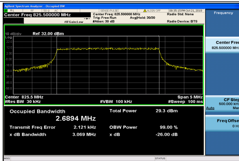
Band5-3MHz-QPSK-20415-15RB#0-2.6894
