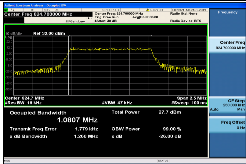
Band5-1.4MHz-16QAM-20407-6RB#0-1.0807
