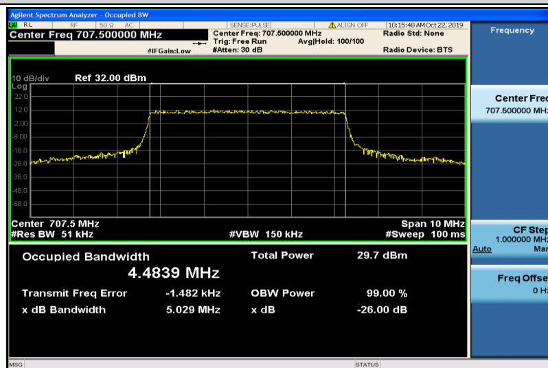
Band12-5MHz-QPSK-23095-25RB#0-4.4839
