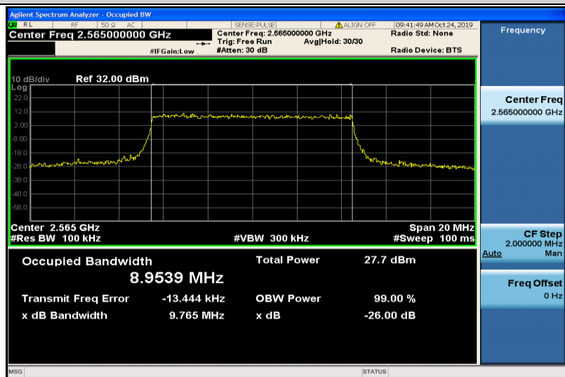
Band7-10MHz-16QAM-21400-50RB#0-8.9539
