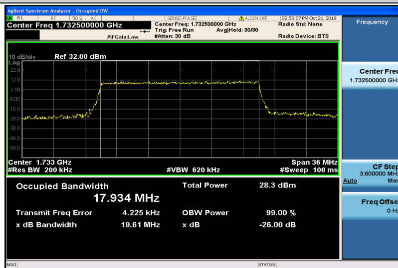
Band4-20MHz-16QAM-20175-100RB#0-17.934
