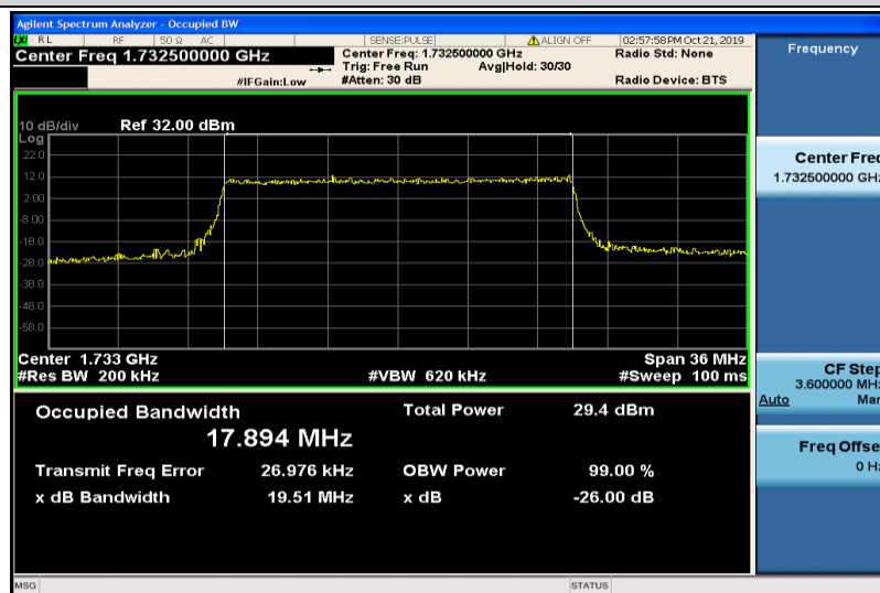
Band4-20MHz-QPSK-20175-100RB#0-17.894
