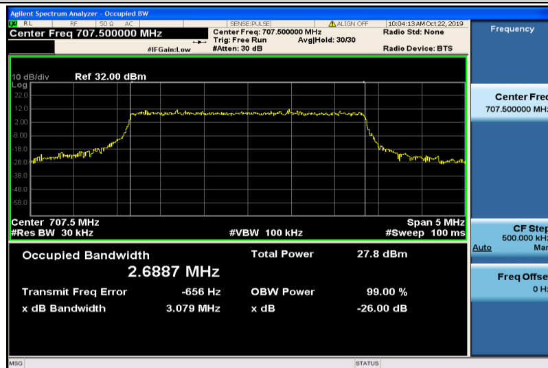
Band12-3MHz-16QAM-23095-15RB#0-2.6887
