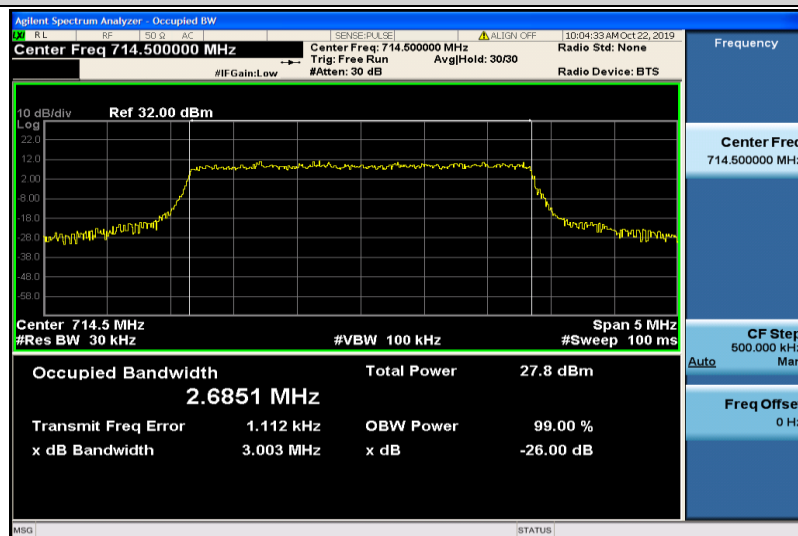
Band12-3MHz-16QAM-23165-15RB#0-2.6851
