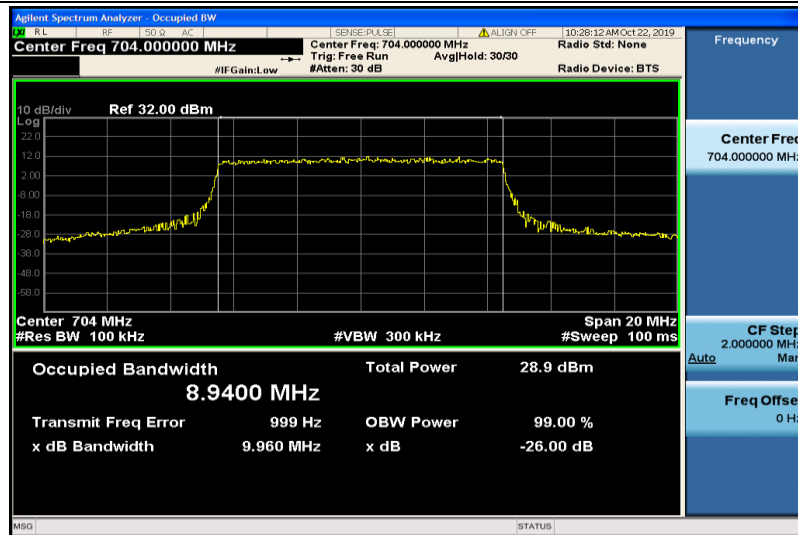
Band12-10MHz-16QAM-23060-50RB#0-8.9400
