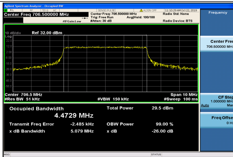
Band17-5MHz-QPSK-23755-25RB#0-4.4729
