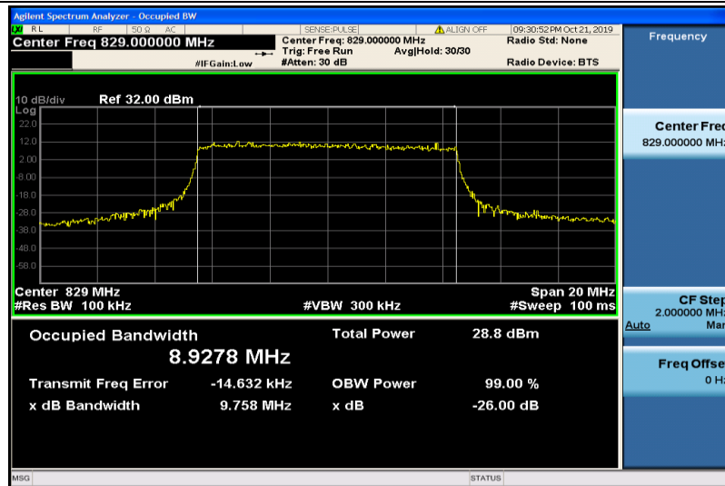
Band5-10MHz-16QAM-20450-50RB#0-8.9278
