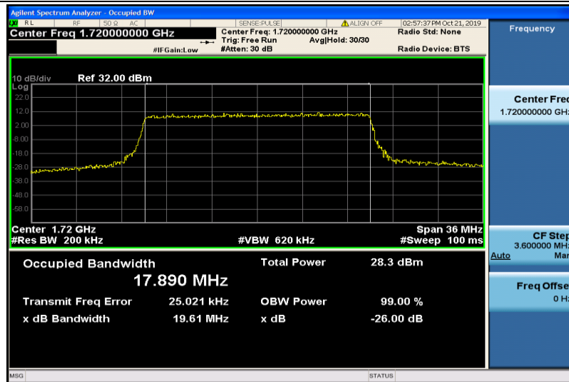
Band4-20MHz-QPSK-20050-100RB#0-17.890
