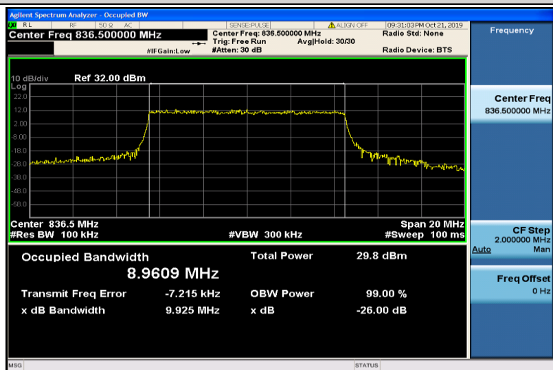
Band5-10MHz-QPSK-20525-50RB#0-8.9609
