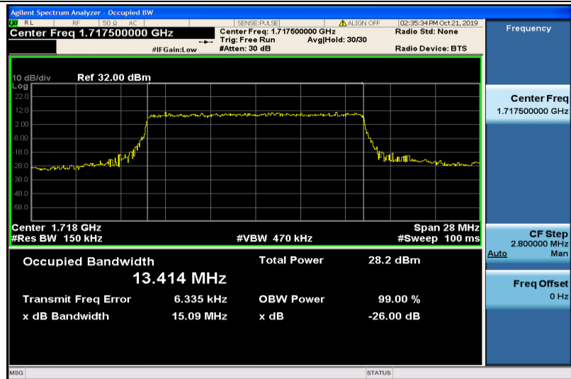
Band4-15MHz-QPSK-20025-75RB#0-13.414
