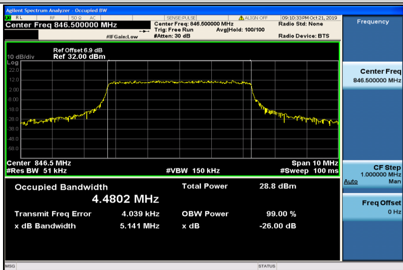
Band5-5MHz-16QAM-20625-25RB#0-4.4802
