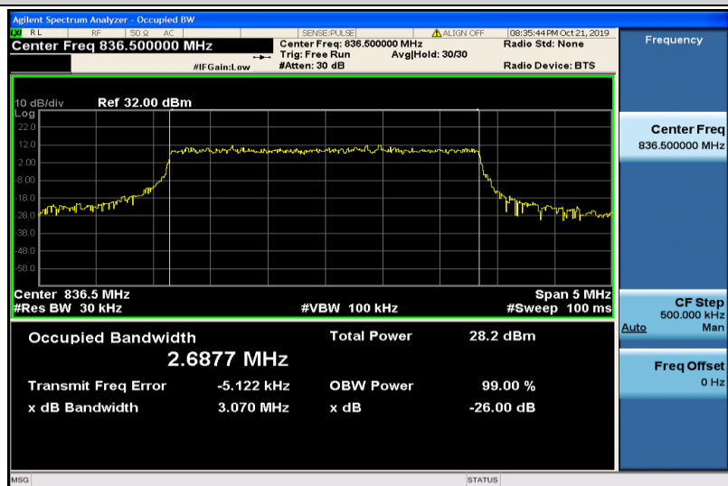
Band5-3MHz-16QAM-20525-15RB#0-2.6877
