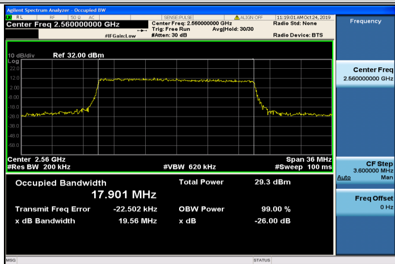
Band7-20MHz-QPSK-21350-100RB#0-17.901
