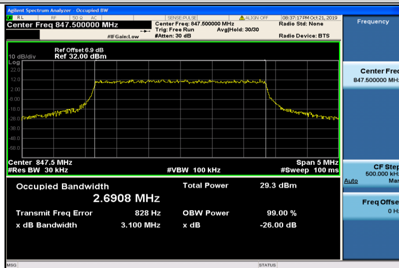
Band5-3MHz-QPSK-20635-15RB#0-2.6908
