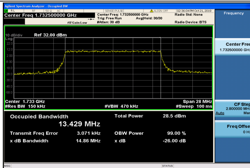
Band4-15MHz-16QAM-20175-75RB#0-13.429
