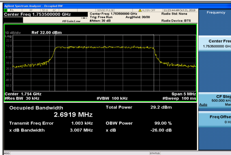
Band4-3MHz-QPSK-20385-15RB#0-2.6919
