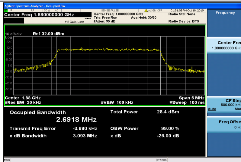
Band2-3MHz-16QAM-18900-15RB#0-2.6918
