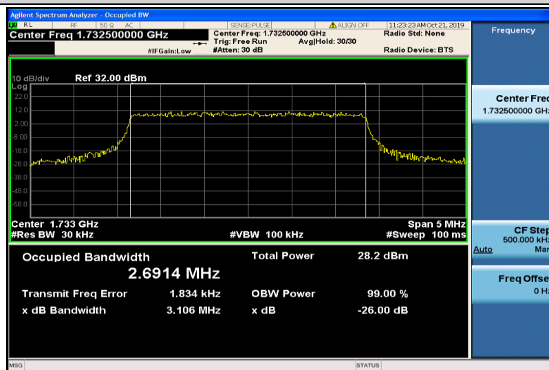
Band4-3MHz-QPSK-20175-15RB#0-2.6914
