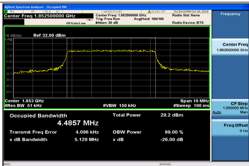
Band2-5MHz-16QAM-18625-25RB#0-4.4857
