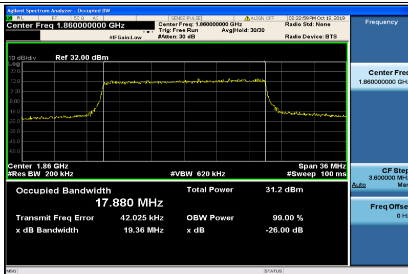
Band2-20MHz-QPSK-18700-100RB#0-17.880
