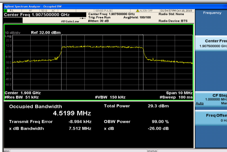
Band2-5MHz-QPSK-19175-25RB#0-4.5199
