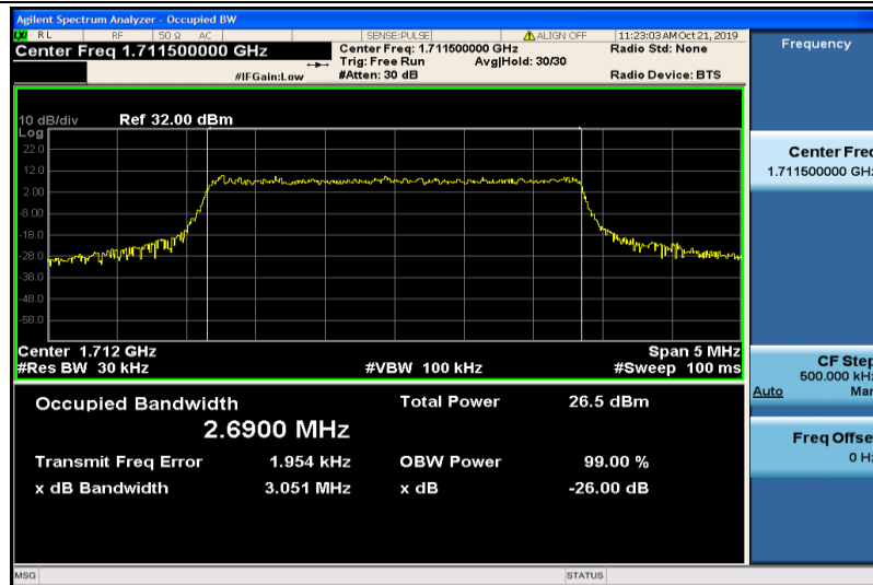
Band4-3MHz-QPSK-19965-15RB#0-2.6900
