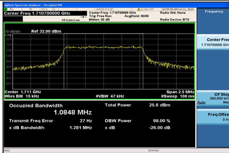
Band4-1.4MHz-16QAM-19957-6RB#0-1.0848
