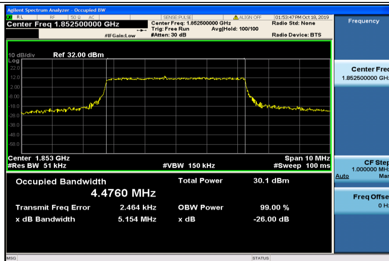
Band2-5MHz-QPSK-18625-25RB#0-4.4760
