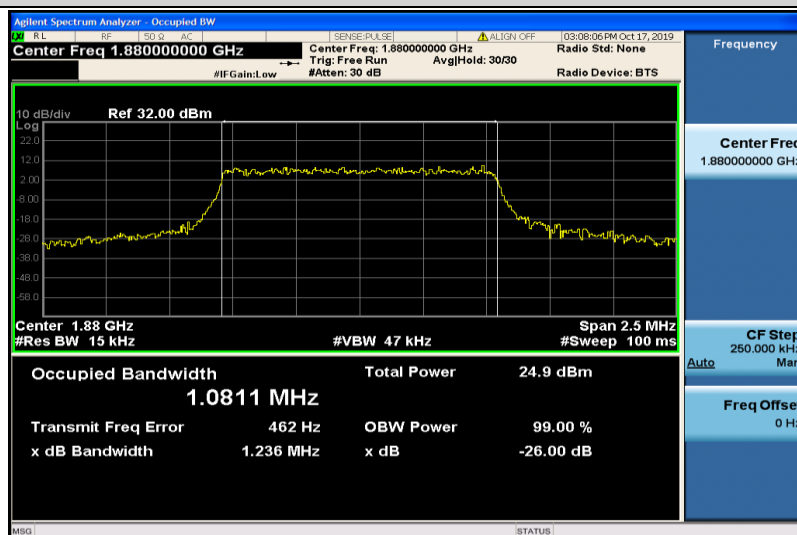
Band2-1.4MHz-QPSK-18900-6RB#0-1.0811
