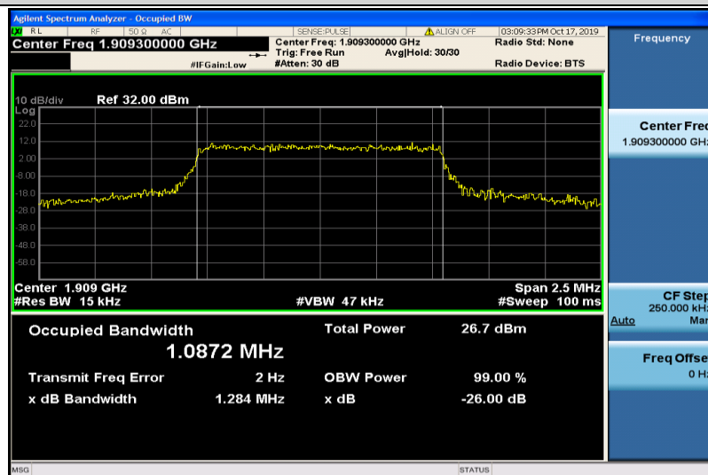
Band2-1.4MHz-16QAM-19193-6RB#0-1.0872
