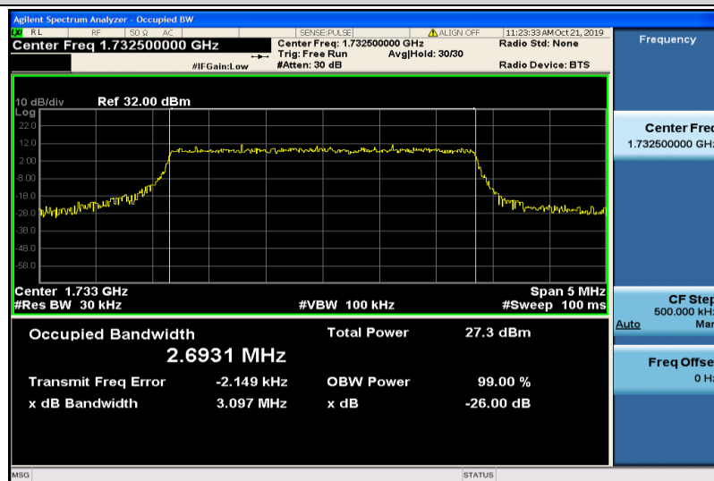
Band4-3MHz-16QAM-20175-15RB#0-2.6931
