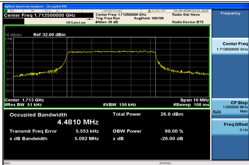
Band4-5MHz-16QAM-19975-25RB#0-4.4810
