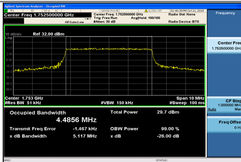
Band4-5MHz-QPSK-20375-25RB#0-4.4856
