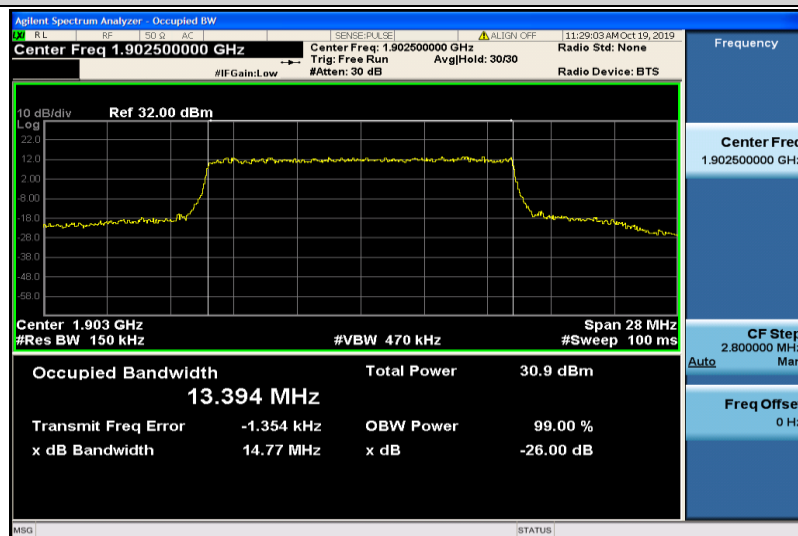
Band2-15MHz-16QAM-19125-75RB#0-13.394
