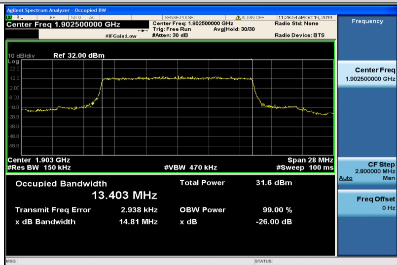
Band2-15MHz-QPSK-19125-75RB#0-13.403
