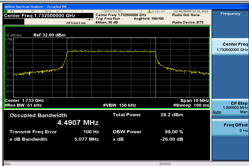
Band4-5MHz-16QAM-20175-25RB#0-4.4907
