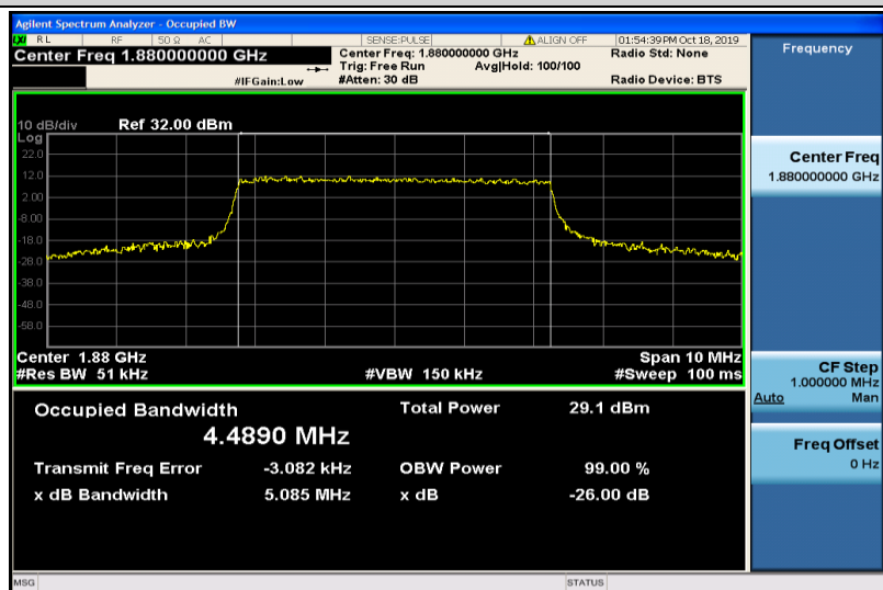
Band2-5MHz-16QAM-18900-25RB#0-4.4890
