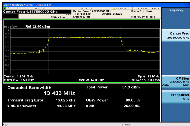
Band2-15MHz-QPSK-18675-75RB#0-13.433
