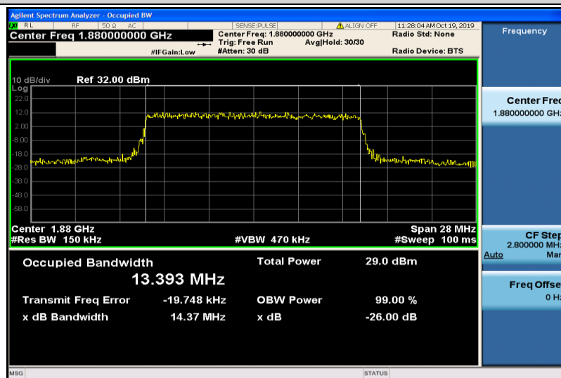
Band2-15MHz-16QAM-18900-75RB#0-13.393
