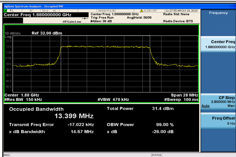
Band2-15MHz-QPSK-18900-75RB#0-13.399
