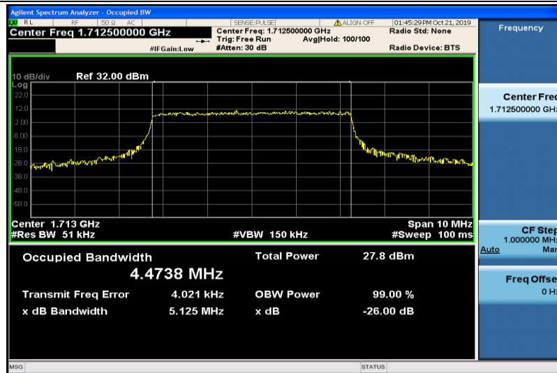
Band4-5MHz-QPSK-19975-25RB#0-4.4738
