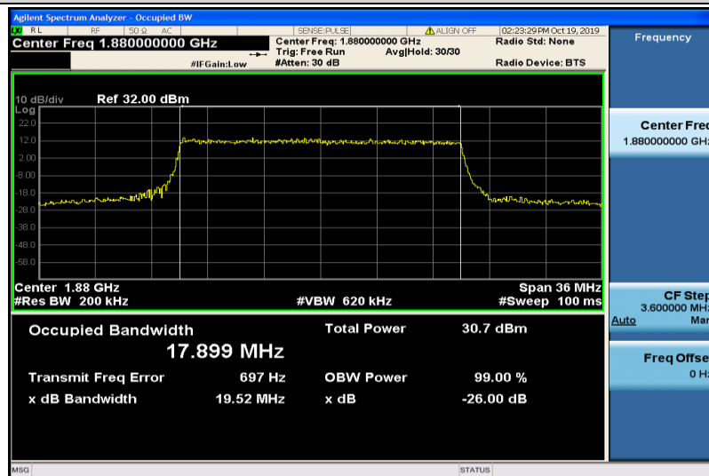
Band2-20MHz-16QAM-18900-100RB#0-17.899
