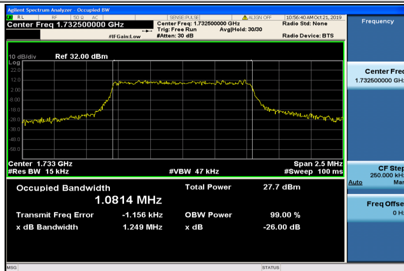
Band4-1.4MHz-QPSK-20175-6RB#0-1.0814
