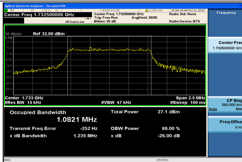
Band4-1.4MHz-16QAM-20175-6RB#0-1.0821
