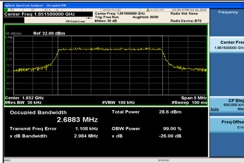
Band2-3MHz-16QAM-18615-15RB#0-2.6883
