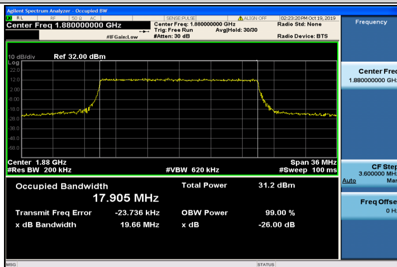
Band2-20MHz-QPSK-18900-100RB#0-17.905
