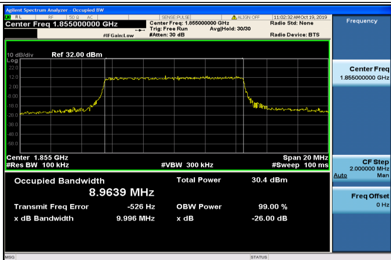
Band2-10MHz-16QAM-18650-50RB#0-8.9639
