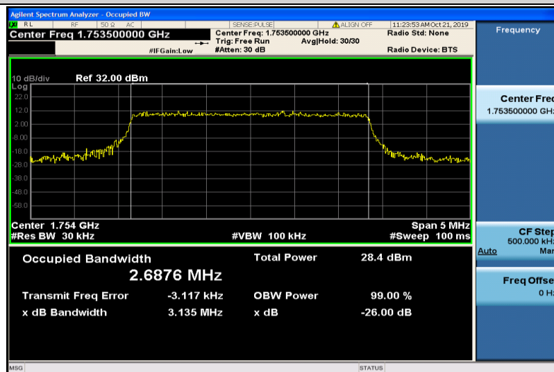
Band4-3MHz-16QAM-20385-15RB#0-2.6876
