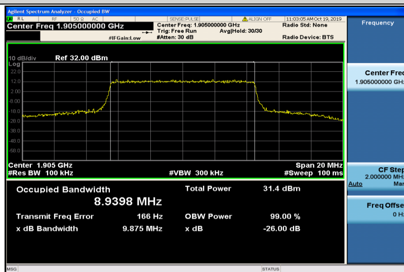
Band2-10MHz-QPSK-19150-50RB#0-8.9398
