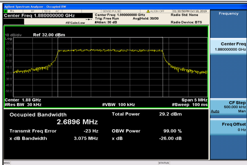
Band2-3MHz-QPSK-18900-15RB#0-2.6896
