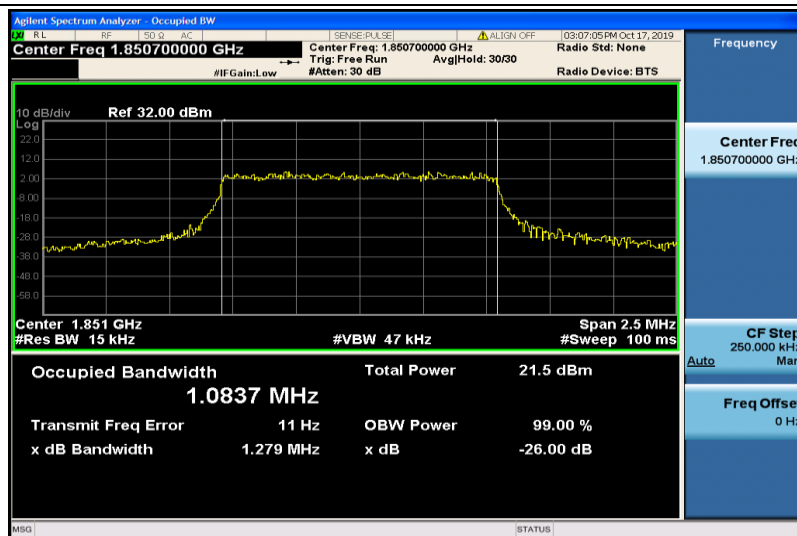
Band2-1.4MHz-QPSK-18607-6RB#0-1.0837
