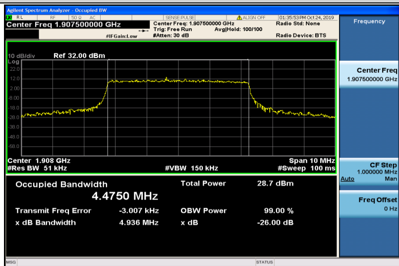
Band2-5MHz-16QAM-19175-25RB#0-4.4750
