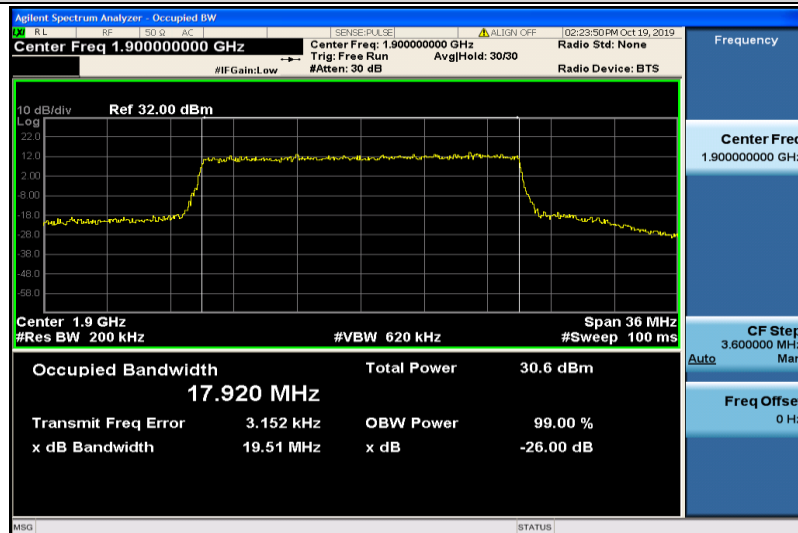
Band2-20MHz-16QAM-19100-100RB#0-17.920
