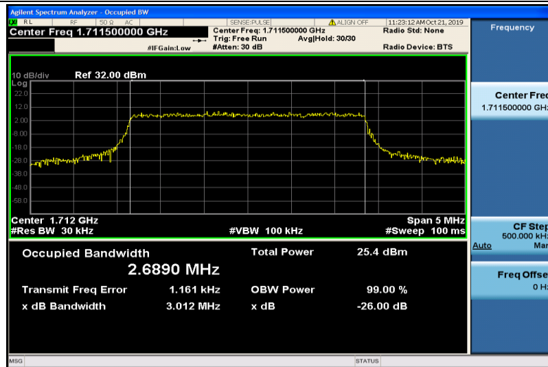
Band4-3MHz-16QAM-19965-15RB#0-2.6890
