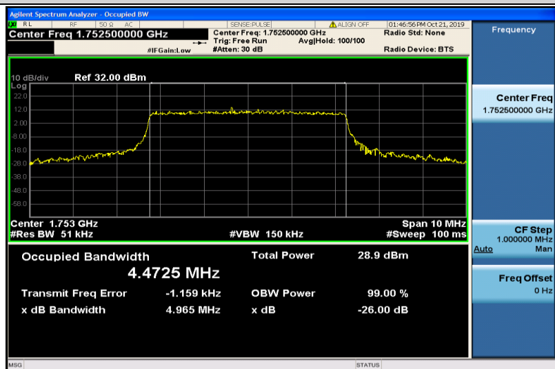
Band4-5MHz-16QAM-20375-25RB#0-4.4725
