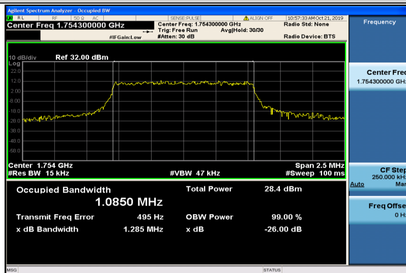
Band4-1.4MHz-QPSK-20393-6RB#0-1.0850
