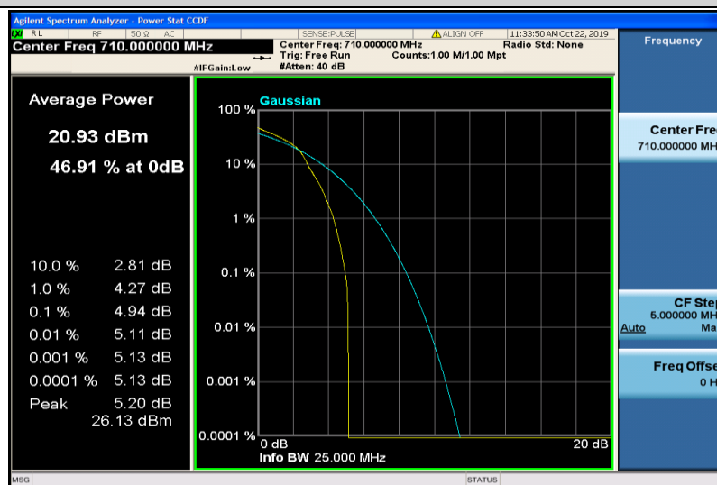
Band17-10MHz-16QAM-23790-1RB#0
