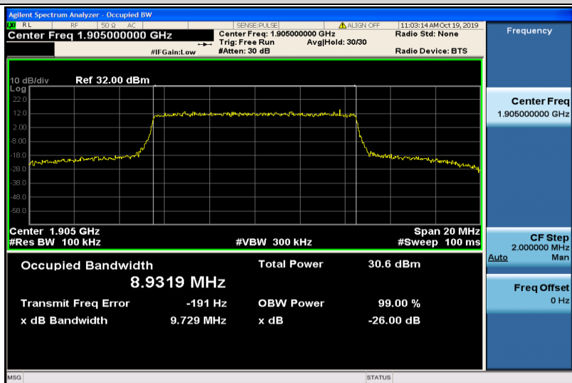
Band2-10MHz-16QAM-19150-50RB#0-8.9319
