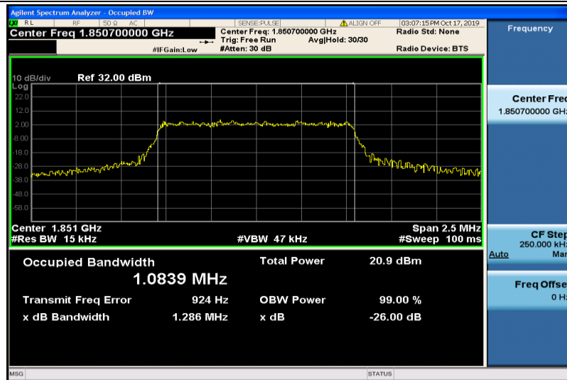
Band2-1.4MHz-16QAM-18607-6RB#0-1.0839
