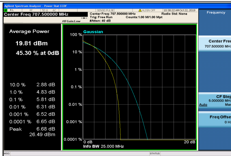
Band12-10MHz-16QAM-23095-50RB#0
