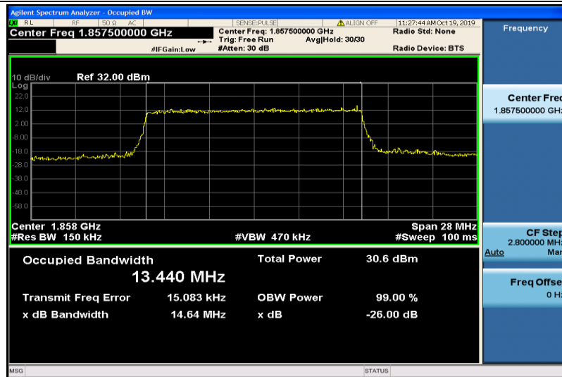
Band2-15MHz-16QAM-18675-75RB#0-13.440
