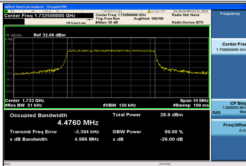
Band4-5MHz-QPSK-20175-25RB#0-4.4760
