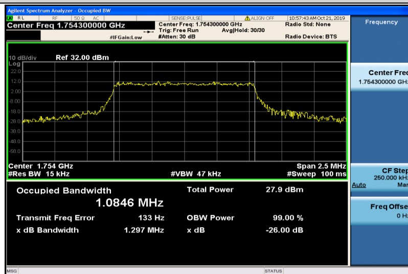
Band4-1.4MHz-16QAM-20393-6RB#0-1.0846
