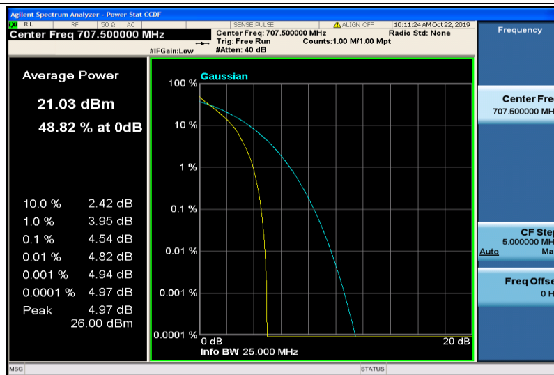
Band12-3MHz-QPSK-23095-15RB#0
