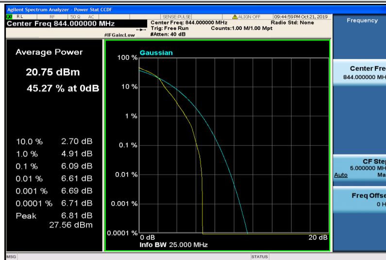
Band5-10MHz-16QAM-20600-1RB#0
