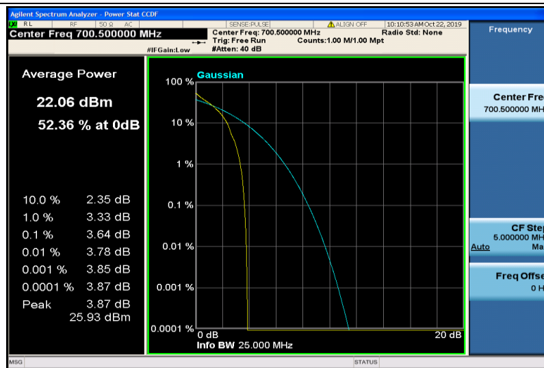
Band12-3MHz-QPSK-23025-1RB#0
