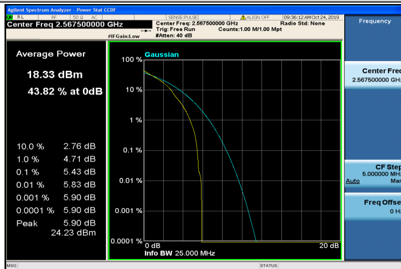
Band7-5MHz-QPSK-21425-1RB#0
