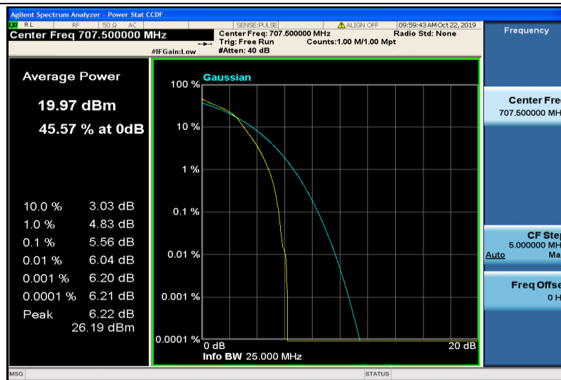
Band12-1.4MHz-16QAM-23095-6RB#0
