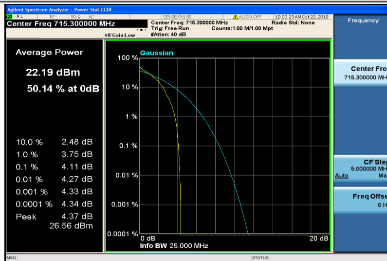
Band12-1.4MHz-QPSK-23173-1RB#0
