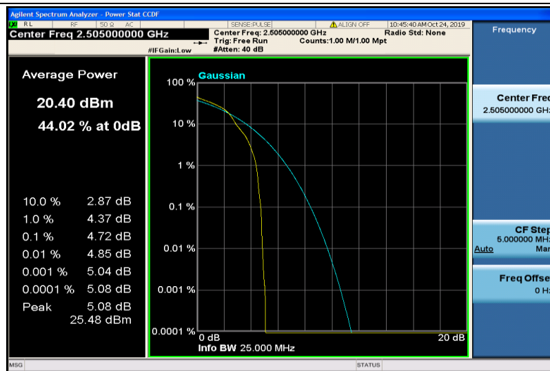
Band7-10MHz-16QAM-20800-1RB#0
