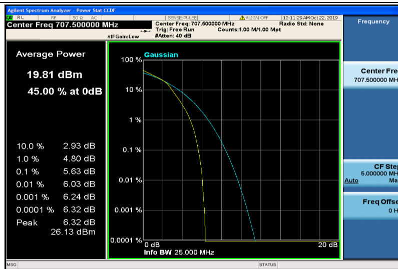
Band12-3MHz-16QAM-23095-15RB#0
