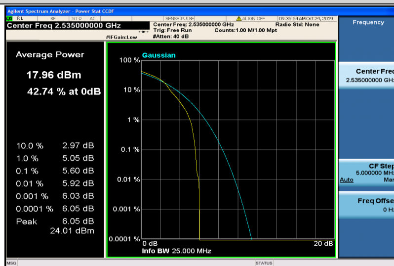
Band7-5MHz-16QAM-21100-1RB#0
