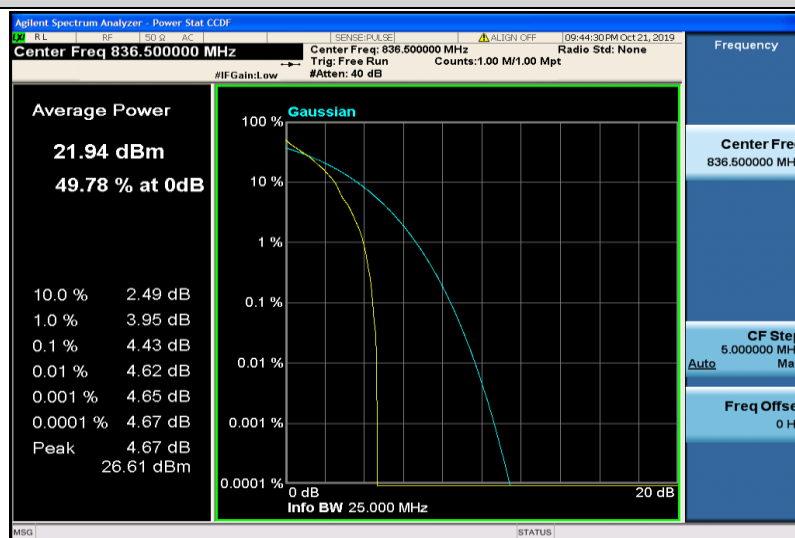
Band5-10MHz-QPSK-20525-1RB#0
