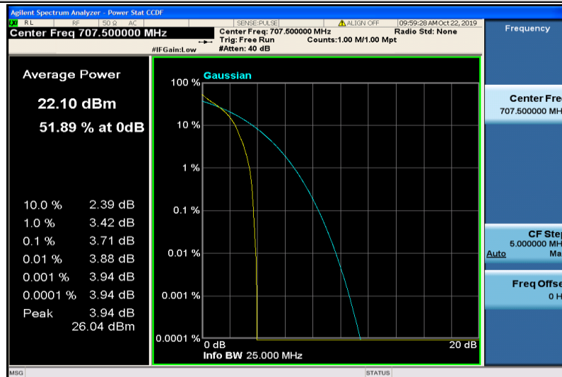
Band12-1.4MHz-QPSK-23095-1RB#0
