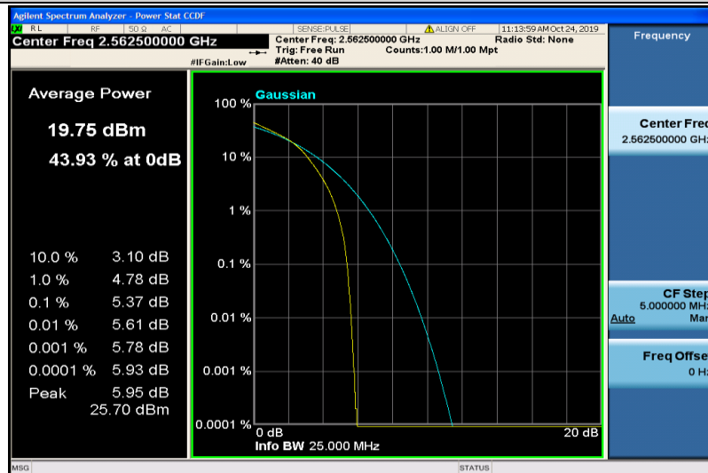
Band7-15MHz-16QAM-21375-75RB#0
