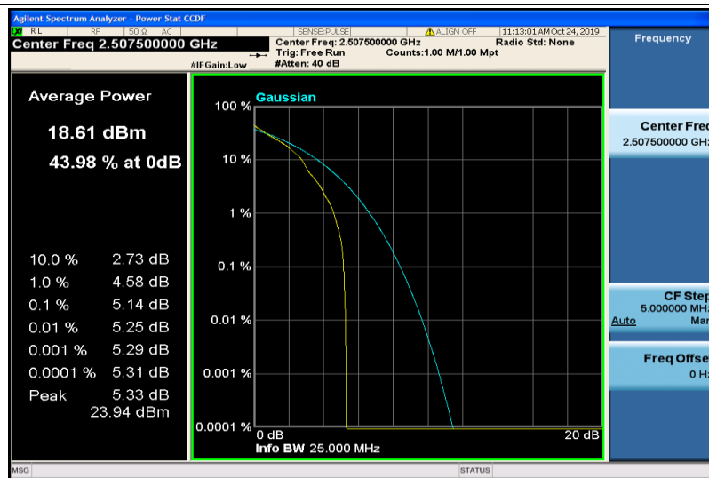
Band7-15MHz-QPSK-20825-1RB#0
