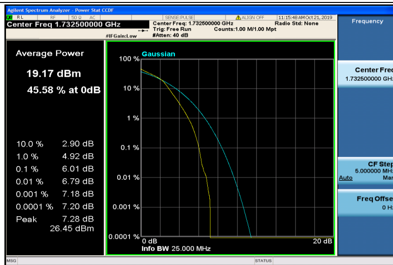
Band4-1.4MHz-16QAM-20175-6RB#0
