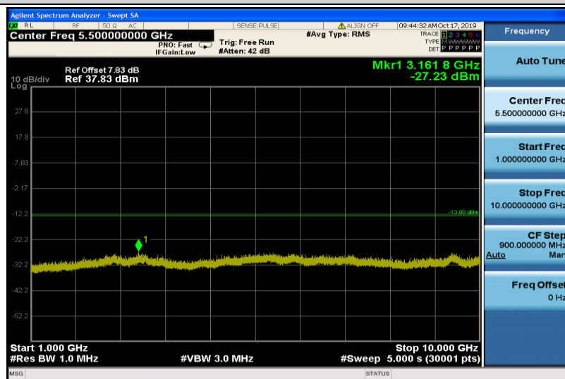
GSM850-128-1000~10000
