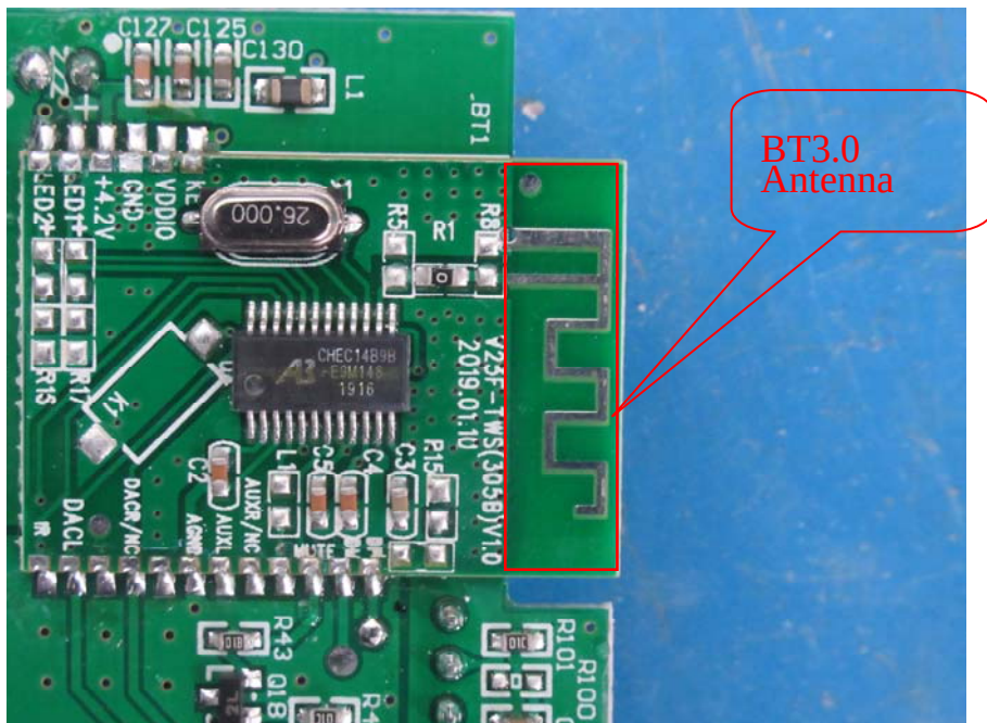
EUT – PCB-1 Top Chip View
