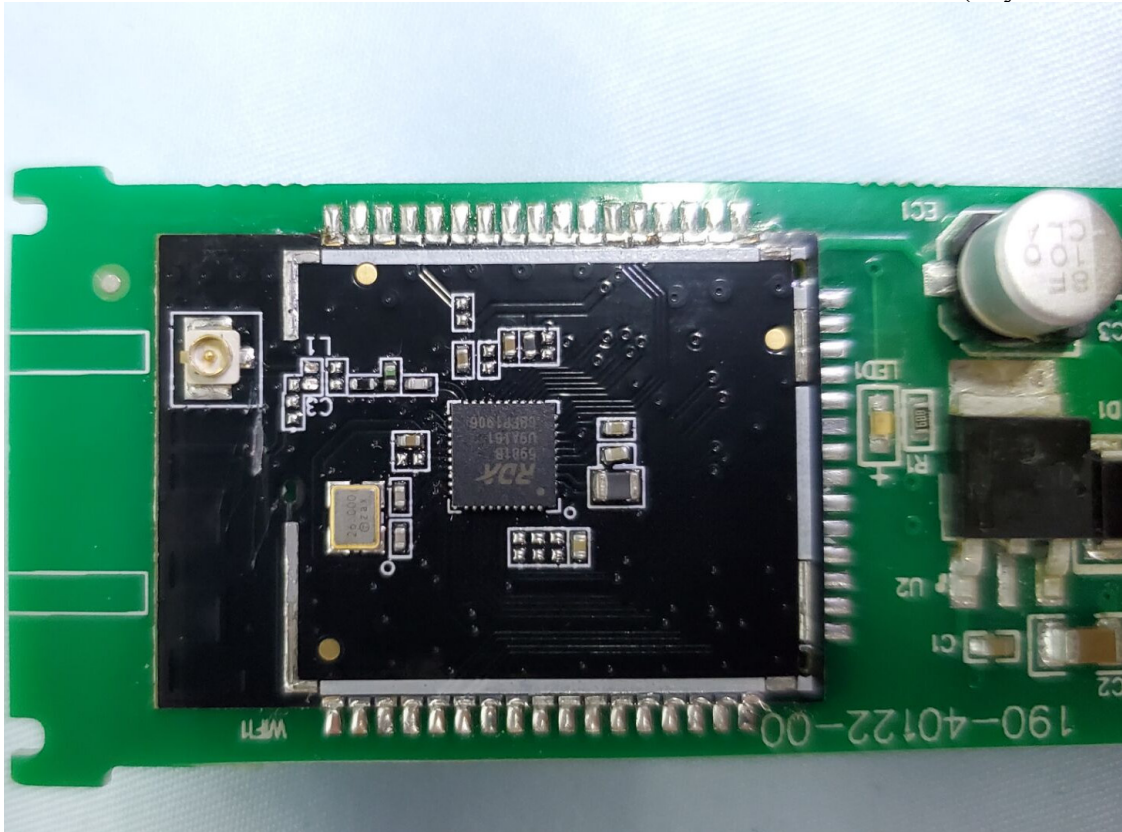
Figure 7 PCB Board (Crystal Oscillator)
