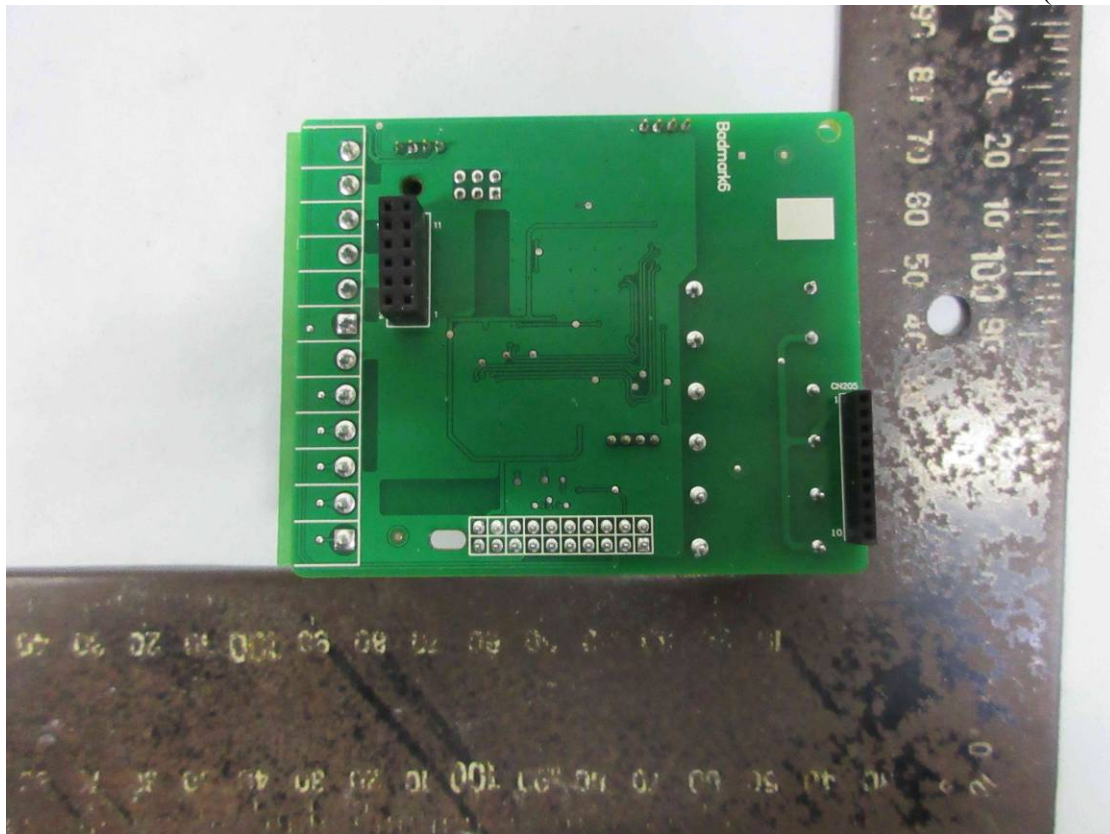
Figure 10 PCB Board (Solder Side)
