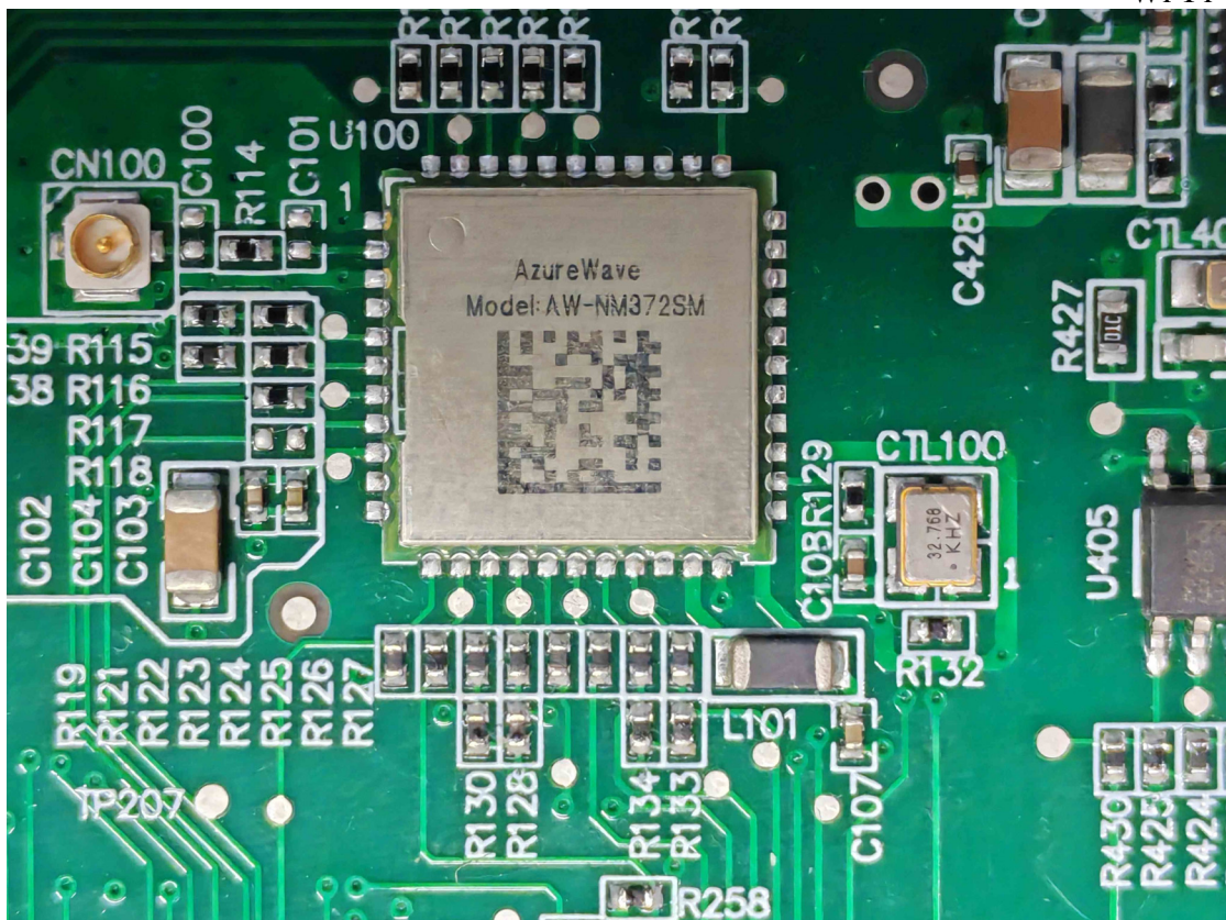
Figure 8 Wi-Fi Module
