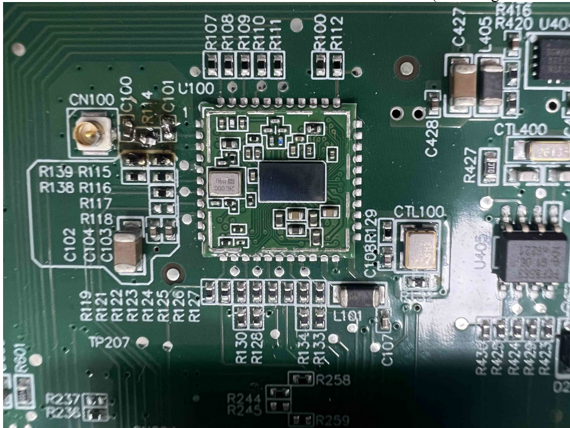
Figure 9 Wi-Fi Module(Shielding Cover Removed)
