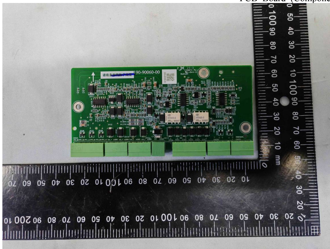
Figure 2 PCB Board (Component Side)
