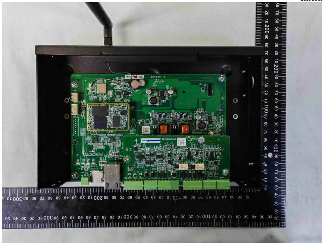
Figure 1 Internal View
