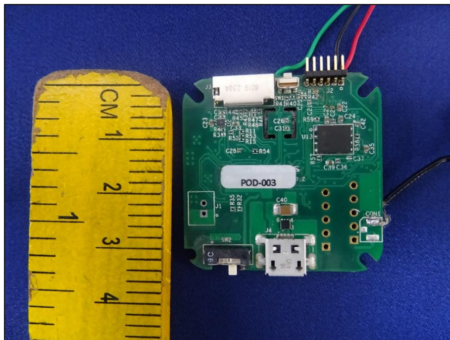
Photo 4: Dimensional View of PCB (Length)
