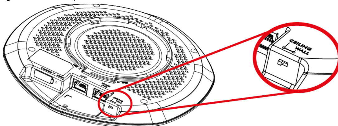
Figure 175 WAC Physical Antenna Switch
