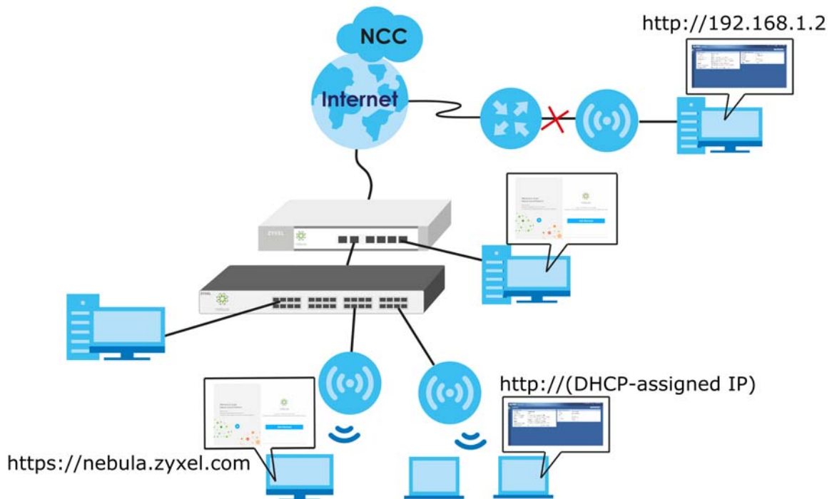
Figure 179 Cloud Mode Application
