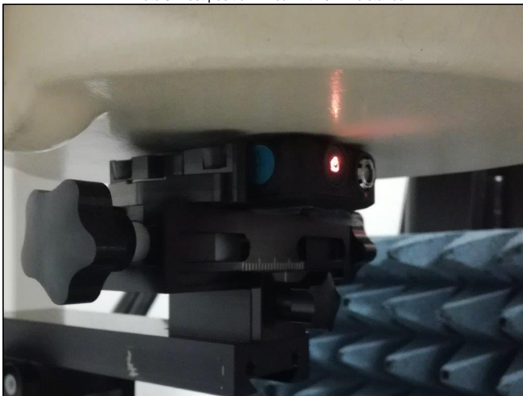
Photo 8: Test position - Rear with 0mm distance
