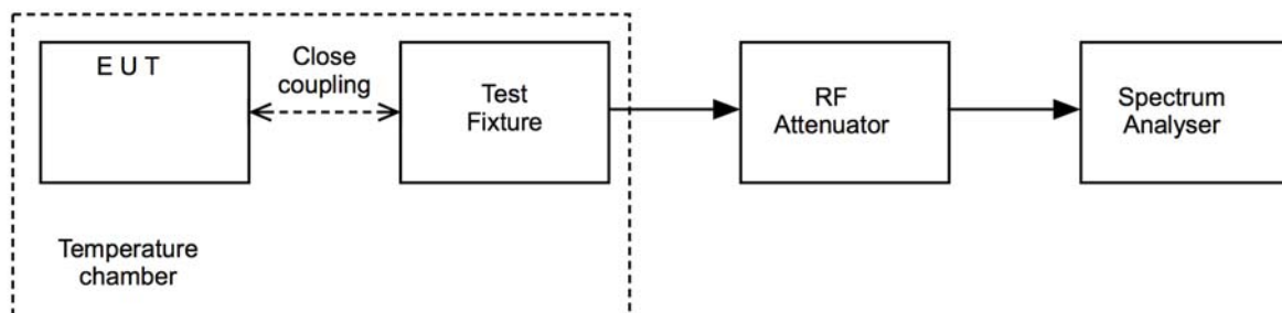
Figure v Test Setup
