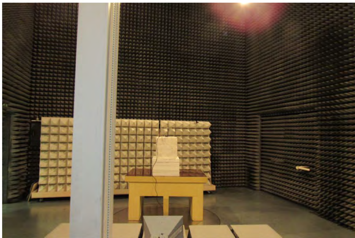
Testsetup above 1 GHz
