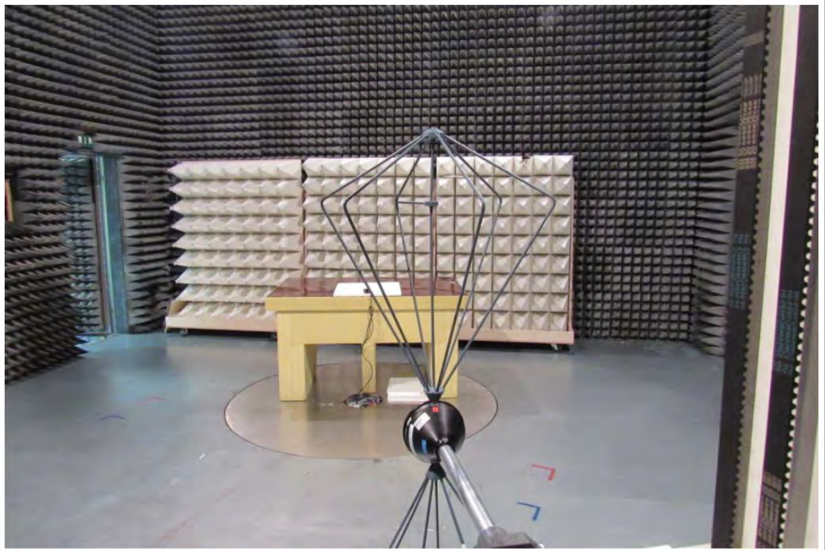
Testsetup above 30 MHz
