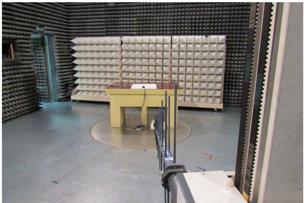
Testsetup above 200 MHz
