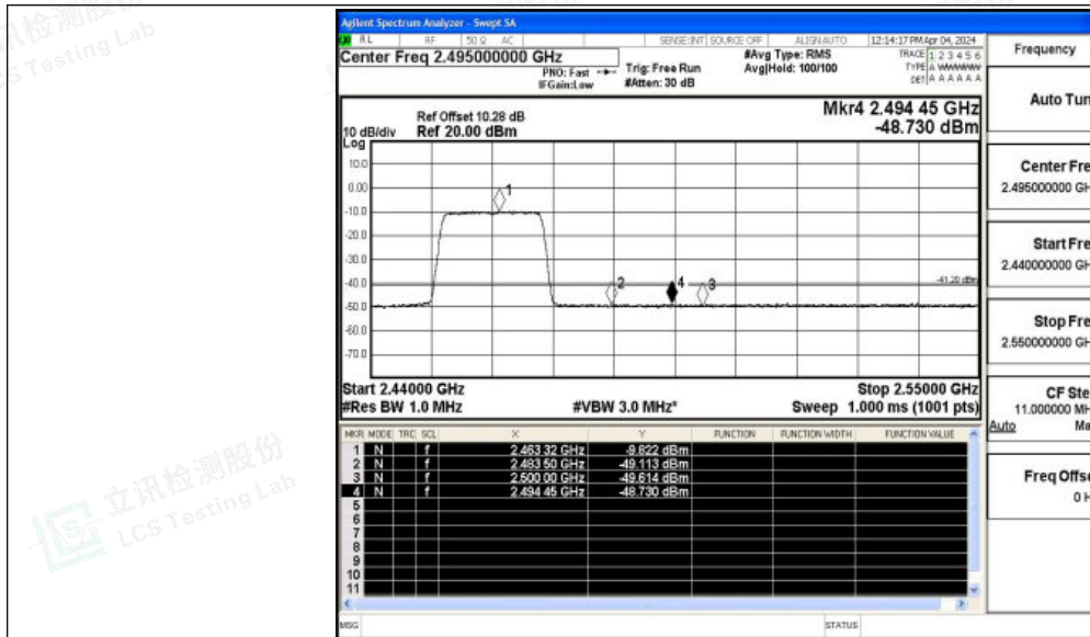
11N20SISO_Ant1_High_2462_Peak
