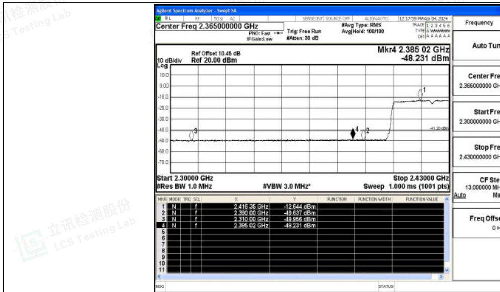
11N40SISO_Ant1_Low_2422_Peak
