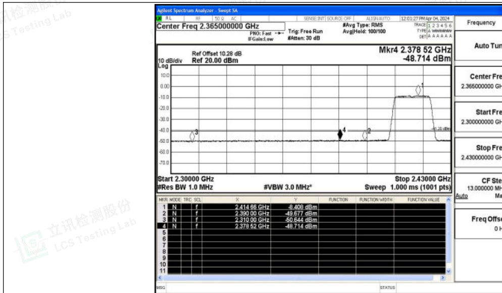
11G_Ant1_Low_2412_Peak
