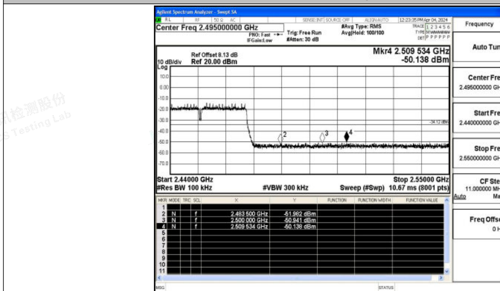
11N40SISO_Ant1_High_2452
