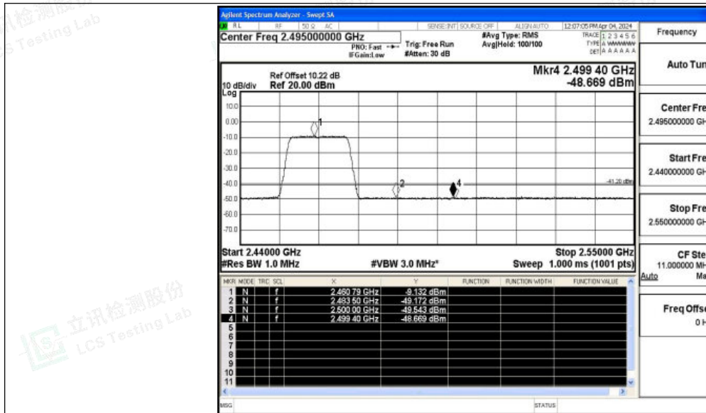
11G_Ant1_High_2462_Peak
