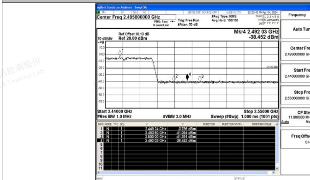
11N40SISO_Ant1_High_2452_Peak
