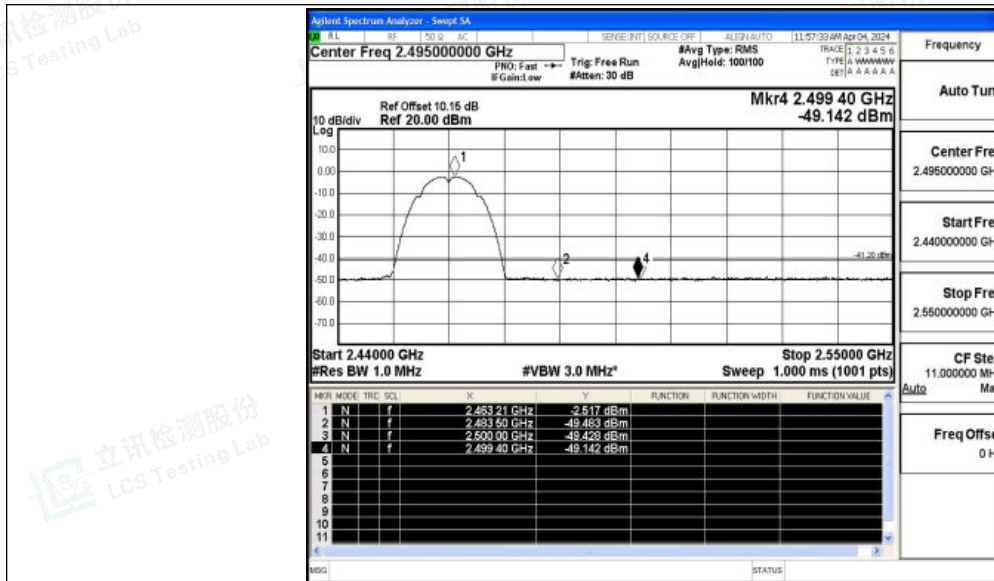
11B_Ant1_High_2462_Peak
