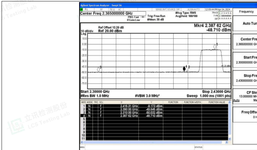
11N20SISO_Ant1_Low_2412_Peak
