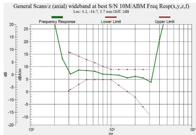
Figure C.9 Frequency Response of LTE B26
