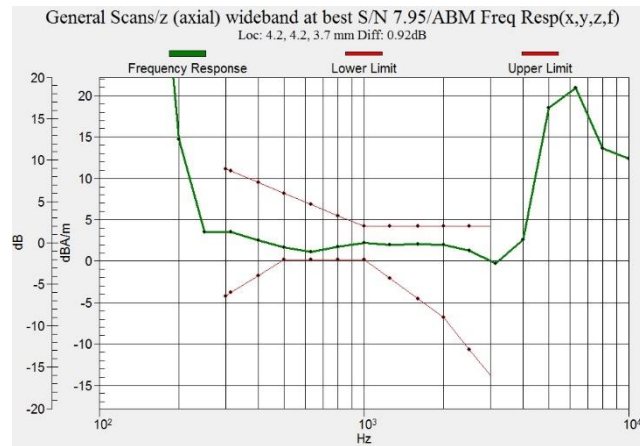
Figure C.16 Frequency Response of W1900 - OTT VoIP
