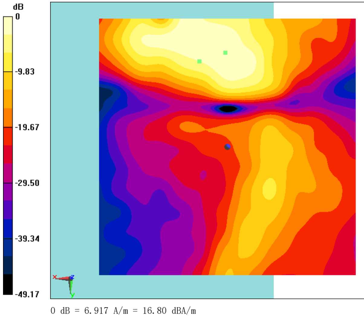
Fig B.38 T-Coil WiFi-2.4G
