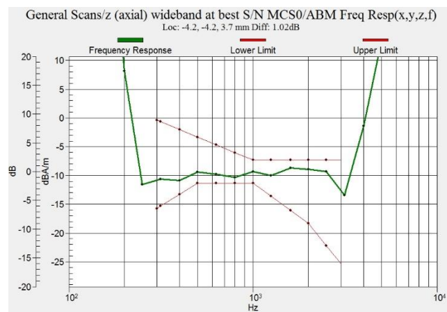
Figure C.14 Frequency Response of WiFi-5G
