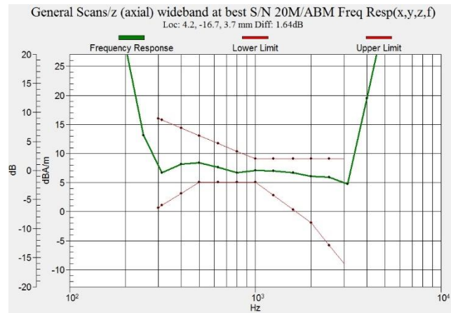
Figure C.7 Frequency Response of LTE B12
