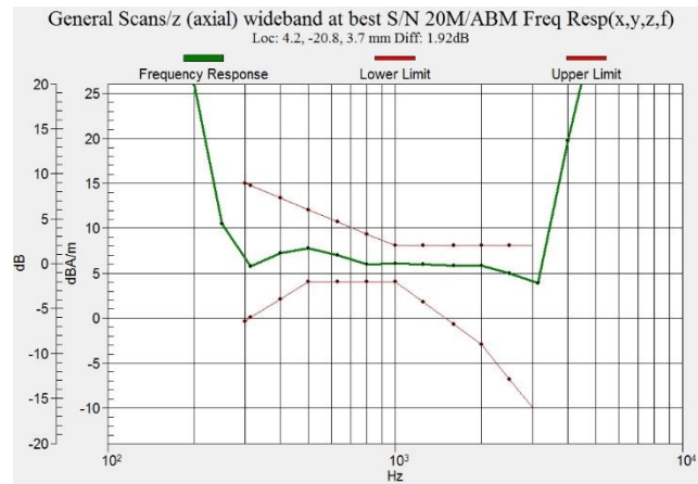
Figure C.10 Frequency Response of LTE B66
