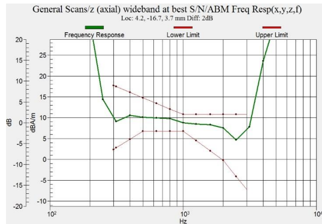
Figure C.20 Frequency Response of WiFi-5G - OTT VoIP
