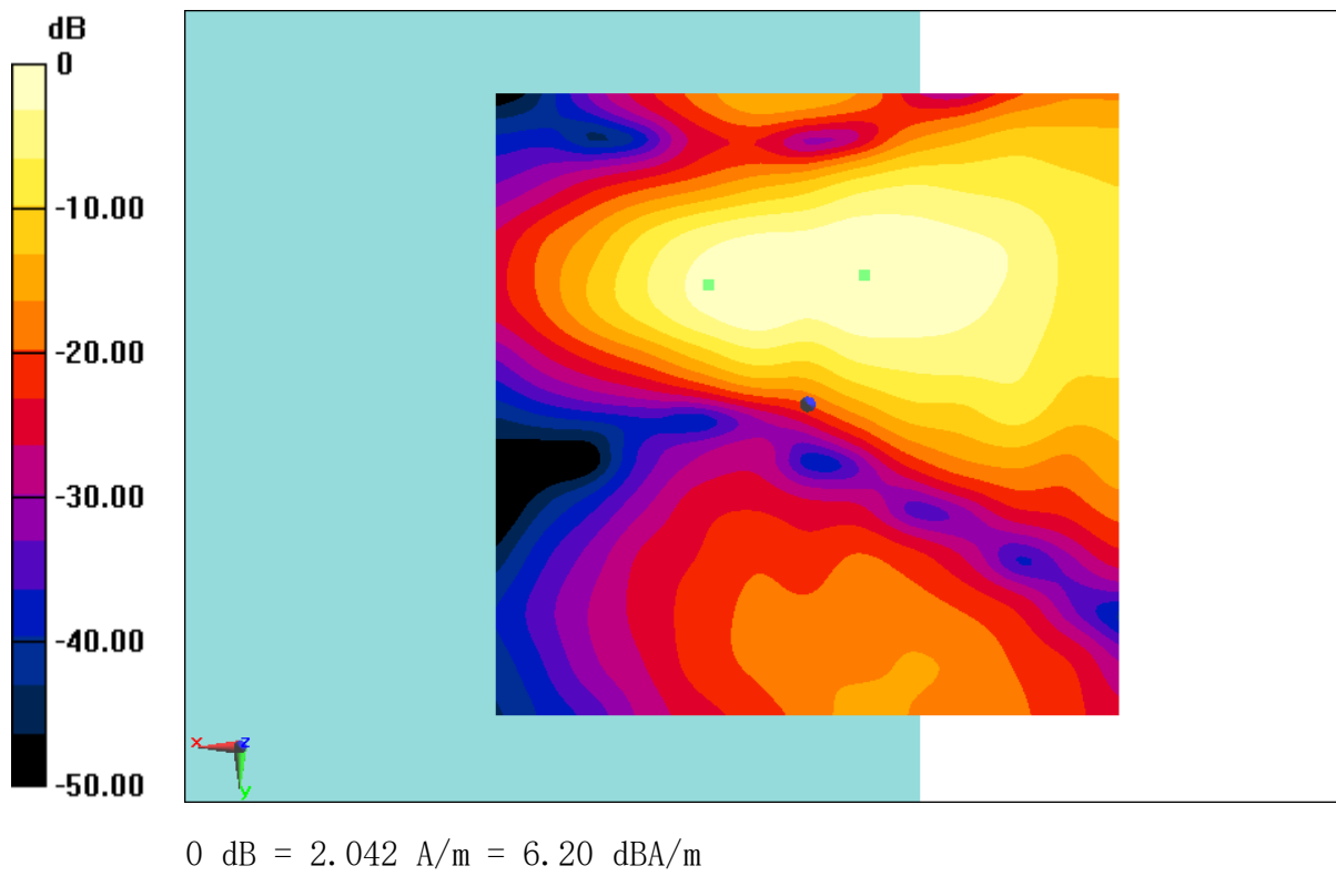
Fig B.15 T-Coil LTE B25
