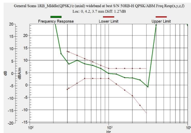
Figure C.17 Frequency Response of LTE B7 - OTT VoIP
