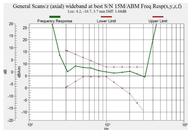
Figure C.12 Frequency Response of LTE B41
