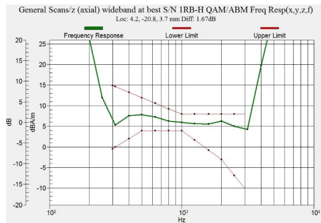
Figure C.8 Frequency Response of LTE B25
