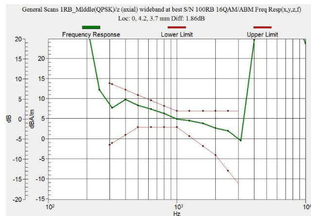
Figure C.18 Frequency Response of LTE B41 - OTT VoIP
