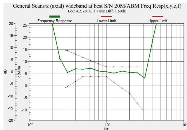
Figure C.6 Frequency Response of LTE B7
