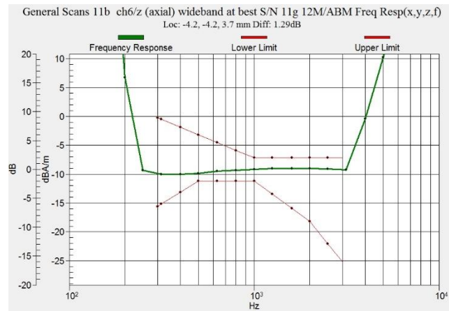
Figure C.13 Frequency Response of WiFi-2.4G
