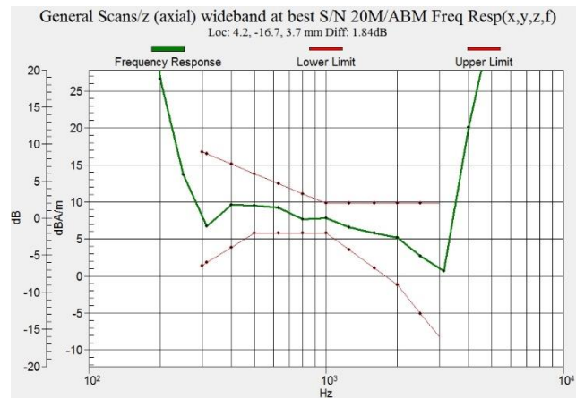
Figure C.11 Frequency Response of LTE B71
