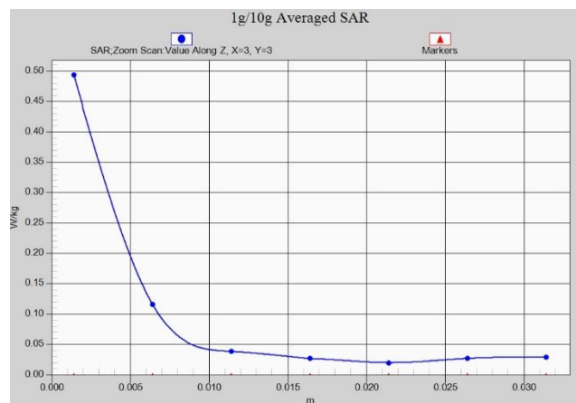
Fig. 1-30 Z-Scan at power reference point (WIFI 5G-Low)
