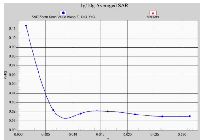
Fig. 1-31 Z-Scan at power reference point (WIFI 5G-Low)
