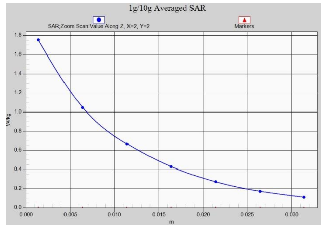
Fig. 1-16 Z-Scan at power reference point (LTE B25 MHz)
