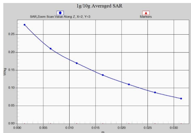
Fig. 1-18 Z-Scan at power reference point (LTE B26 MHz)
