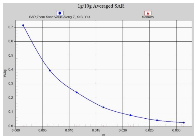
Fig. 1-20 Z-Scan at power reference point (LTE B41 MHz)
