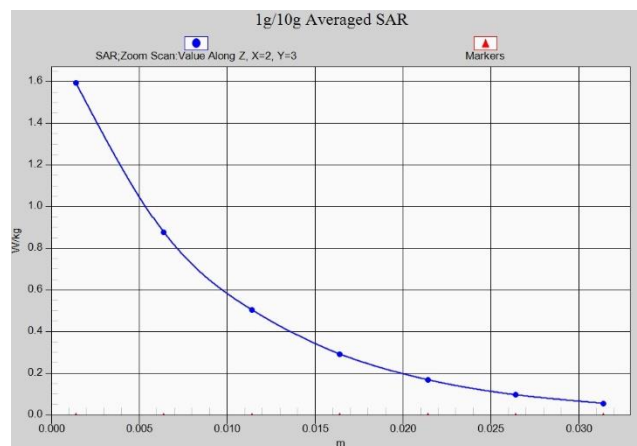
Fig. 1-15 Z-Scan at power reference point (LTE B25 MHz)
