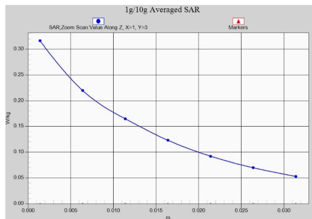
Fig. 1-24 Z-Scan at power reference point (LTE B71 MHz)
