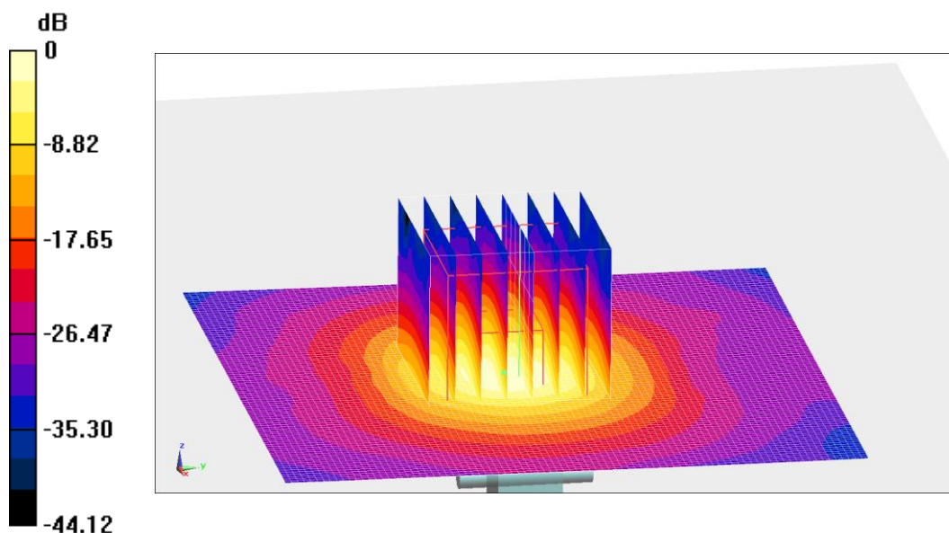
Fig.B.16 validation 5750 MHz 250mW
