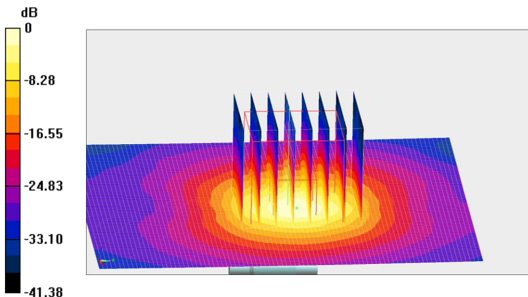
Fig.B.15 validation 5750 MHz 250mW
