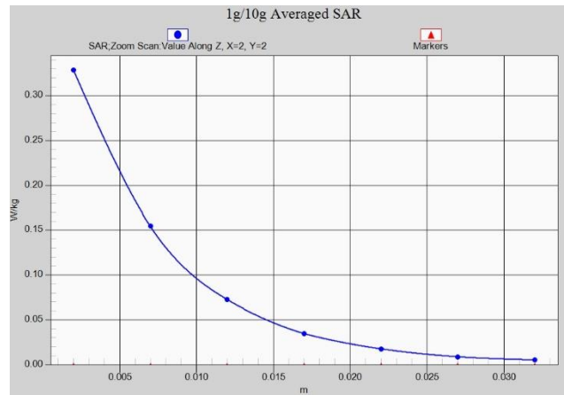
Fig. 1-28 Z-Scan at power reference point (WIFI 2.4G-Low)
