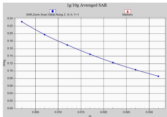
Fig. 1-23 Z-Scan at power reference point (LTE B71 MHz)
