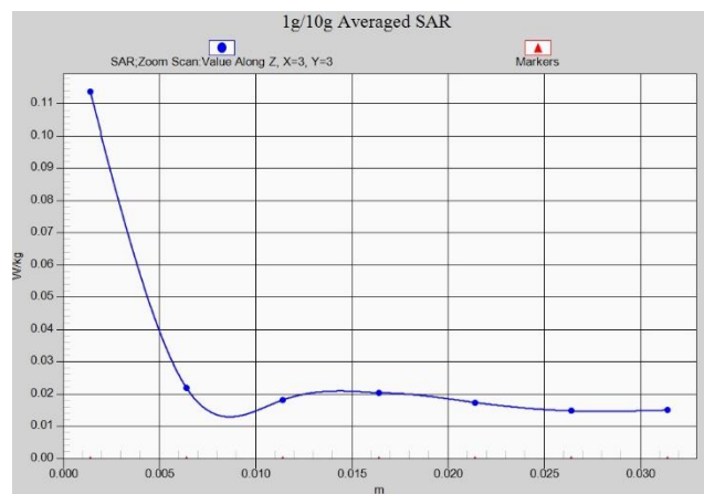
Fig. 1-29 Z-Scan at power reference point (WIFI 2.4G-Low)
