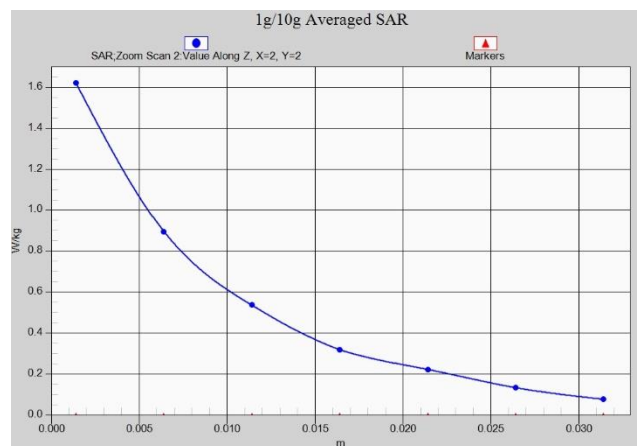
Fig. 1-21 Z-Scan at power reference point (LTE B66 MHz)
