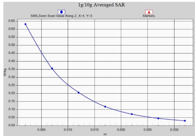
Fig. 1-19 Z-Scan at power reference point (LTE B41 MHz)
