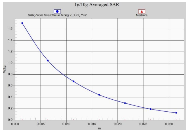
Fig. 1-22 Z-Scan at power reference point (LTE B66 MHz)
