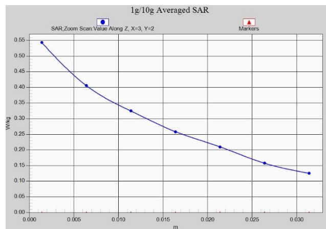
Fig. 1-14 Z-Scan at power reference point (LTE B12 MHz)
