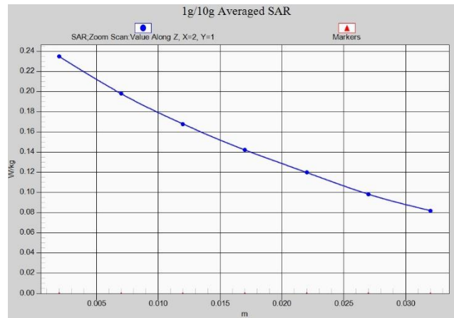
Fig. 1-13 Z-Scan at power reference point (LTE B12 MHz)
