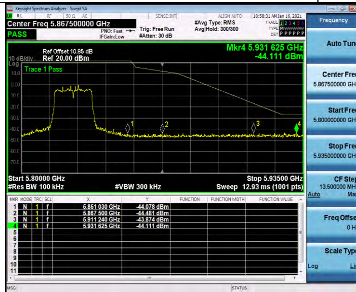
11AC20MIMO_Ant1_High_5825
