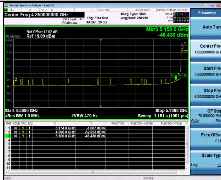
11N40MIMO_Ant1_Low_5190_Peak
