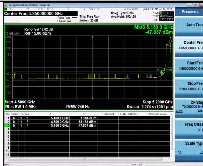
11AC20MIMO_Ant1_Low_5180_Peak
