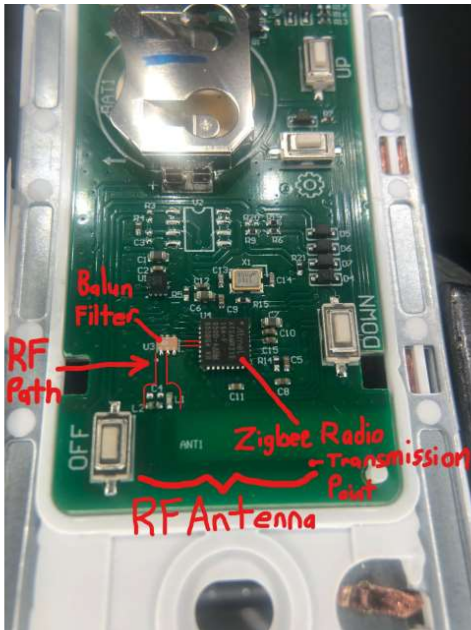
Legrand WNRL63 Zigbee Antenna View
