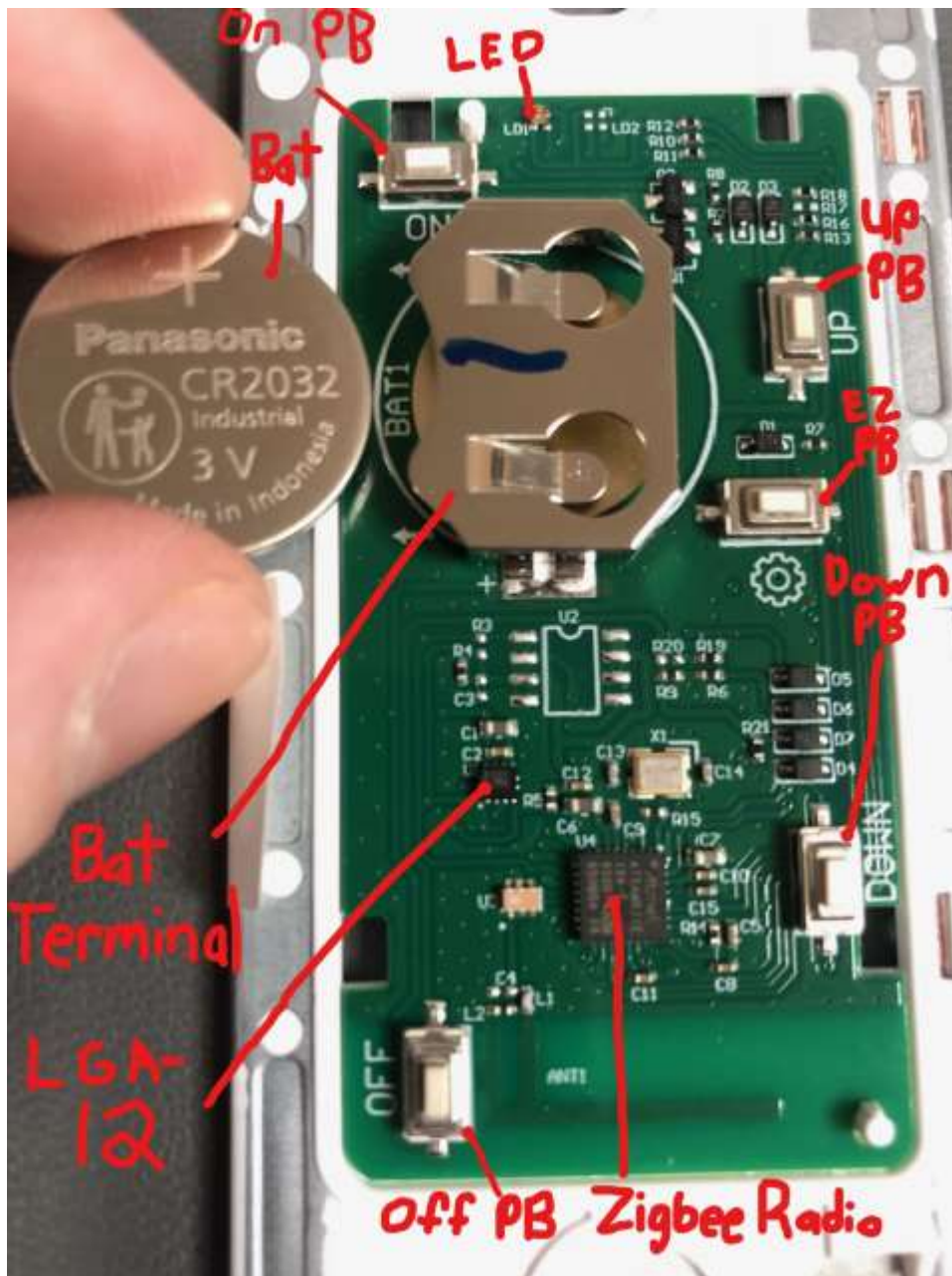
Legrand WNRL63 Switch PCB View
