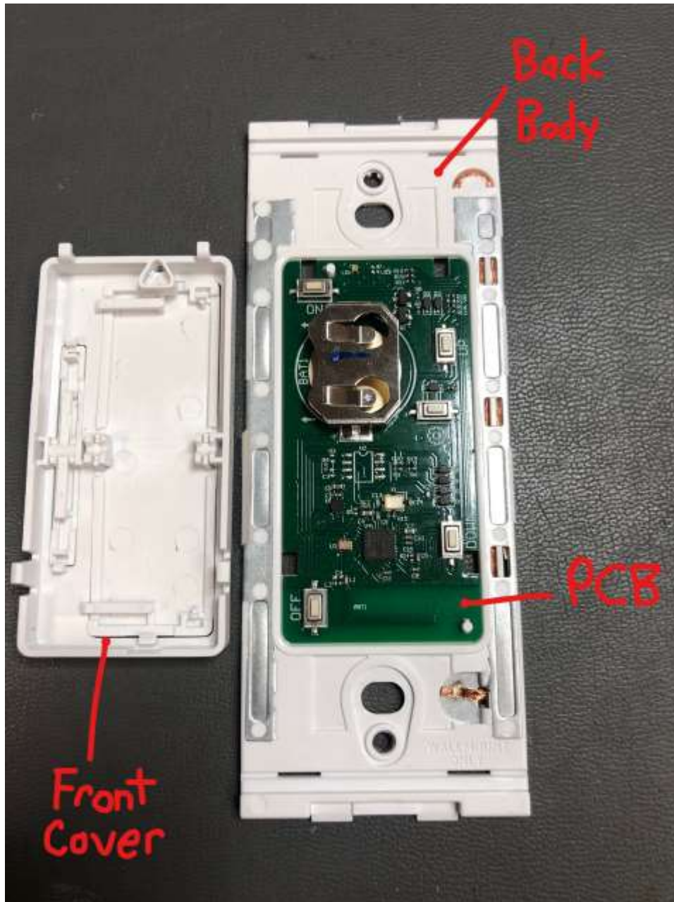
Legrand WNRL63 Switch Assembly View
