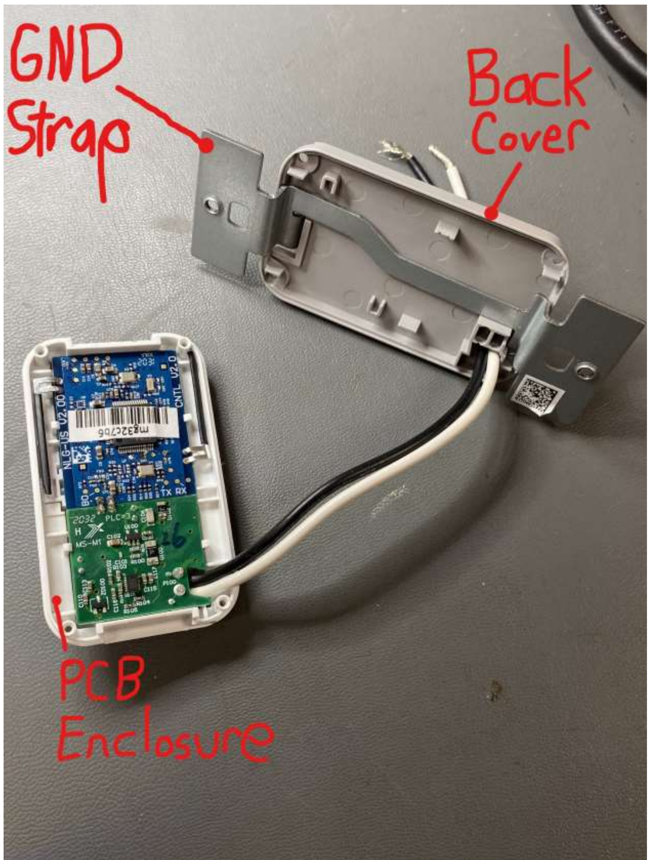
Figure 5: WNRH1 Assembly View
