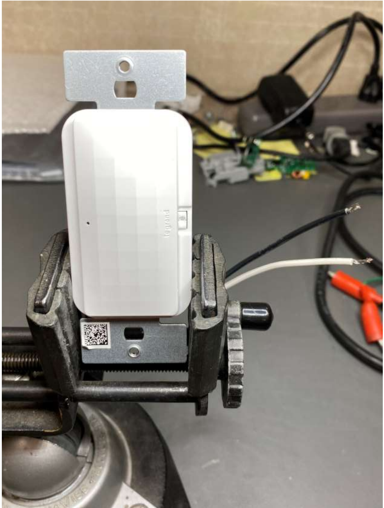
Figure 6: WNRH1 Assembled Device Front View
