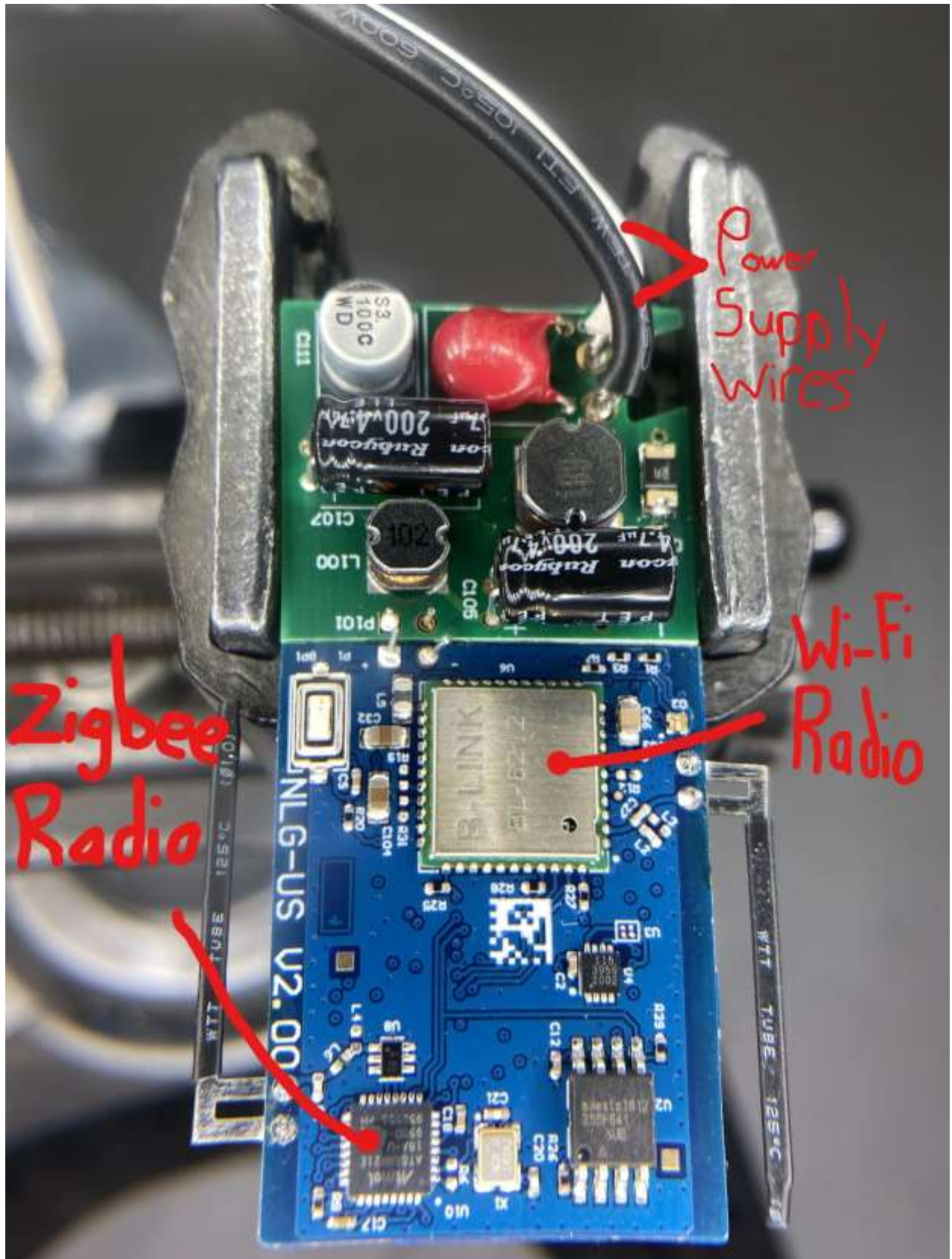
Figure 2: WNRH1 PCB Rear View
