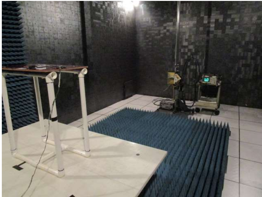
Radiated Emissions Test Setup 1 to 18 GHz
