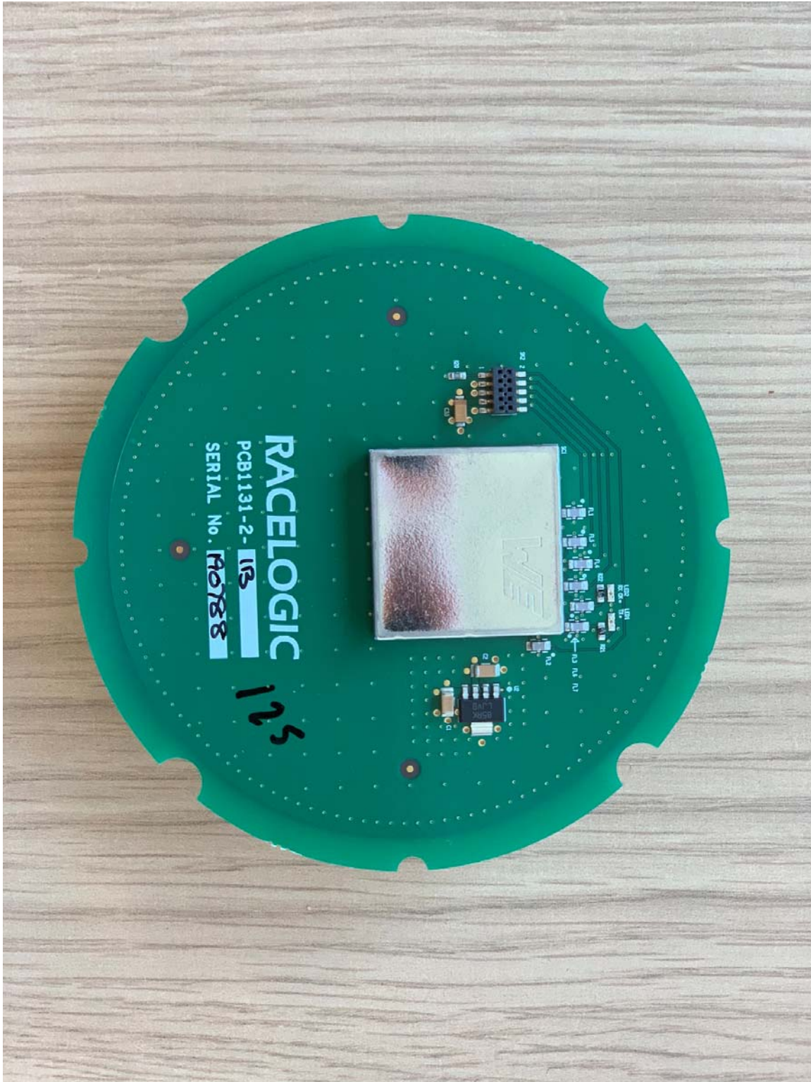
RF board component side – with shield
