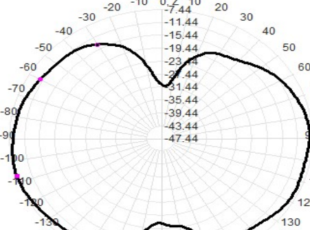
Gain(Peak):0.72dBi
