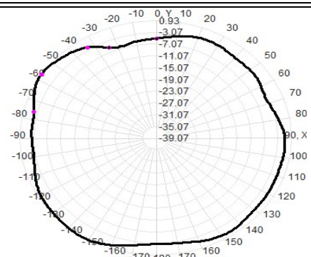
Efficiency:56.6%
