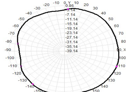
Efficiency:43.3%
