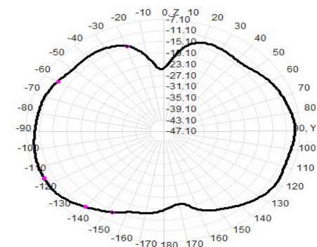
Gain(Peak):0.72dBi
