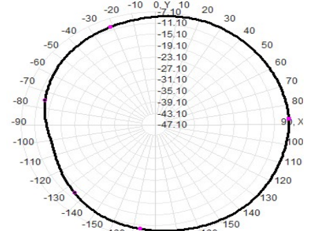
Efficiency:38.2%
