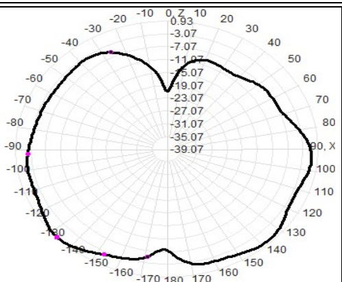
Gain(Peak):1.75dBi
