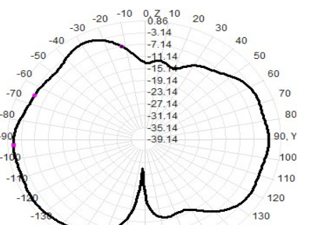
Gain(Peak)1.15dBi
