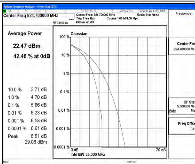
Band26-1.4MHz-QPSK-26915-6RB#0
