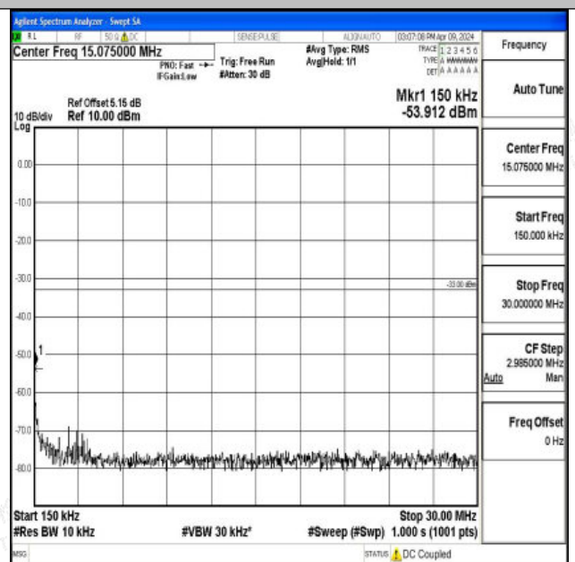
Band66_10MHz_QPSK_132622_1RB#0_0.15~30_0.15~30
