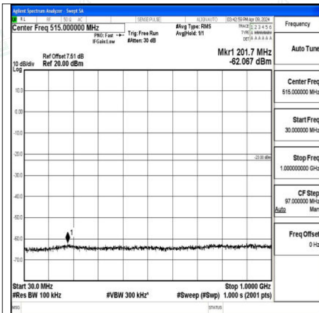
Band66_20MHz_QPSK_132072_1RB#0_30~1000_30~1000
