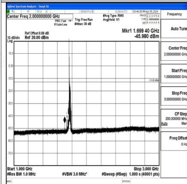
Band66_20MHz_16QAM_132572_1RB#0_1000~3000_10
