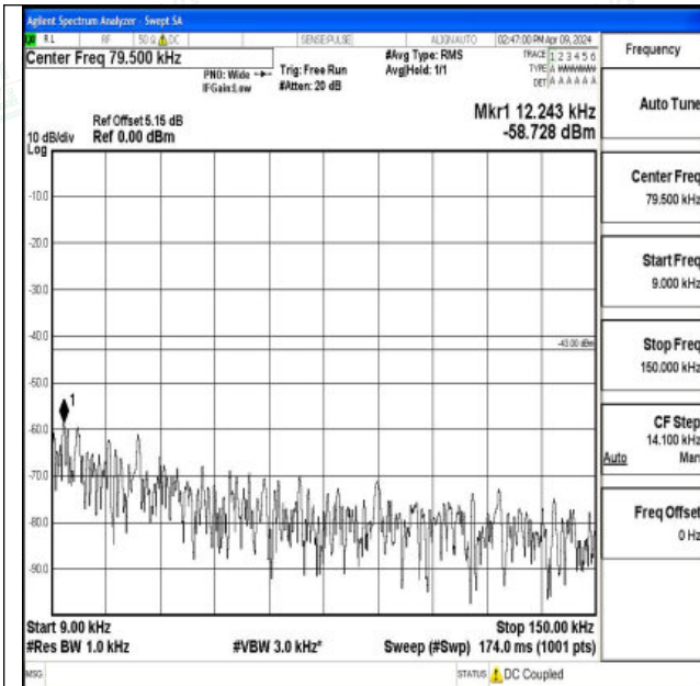
Band66_5MHz_QPSK_132647_1RB#0_0.009~0.15_0.009 ~0.15
