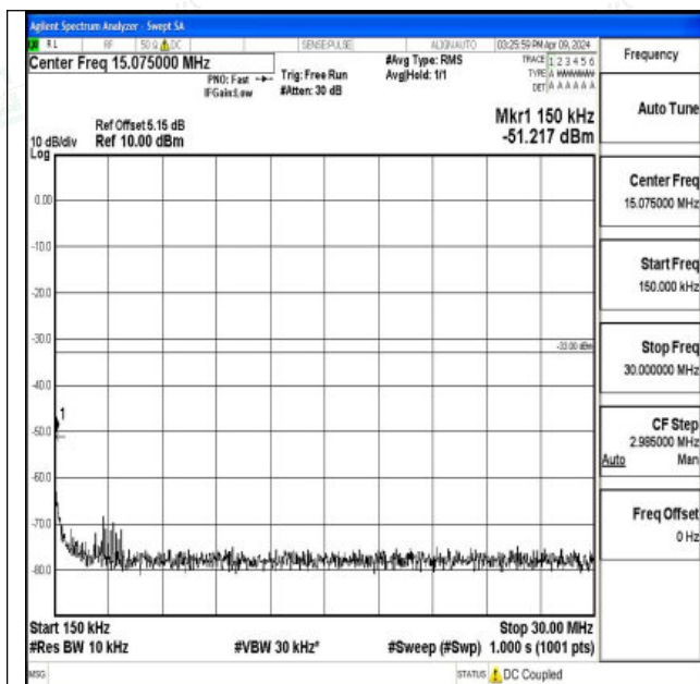
Band66_15MHz_16QAM_132322_1RB#0_0.15~30_0.15~30
