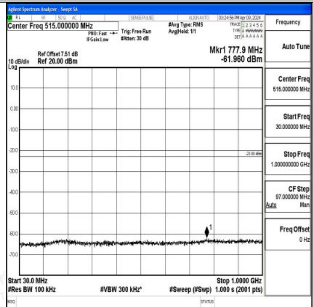
Band66_15MHz_16QAM_132047_1RB#0_30~1000_30~10 00
