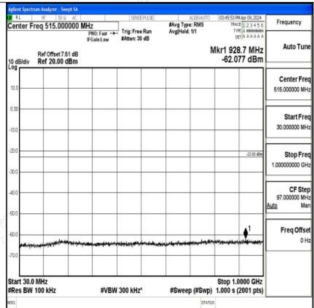
Band66_20MHz_16QAM_132572_1RB#0_30~1000_30~10
