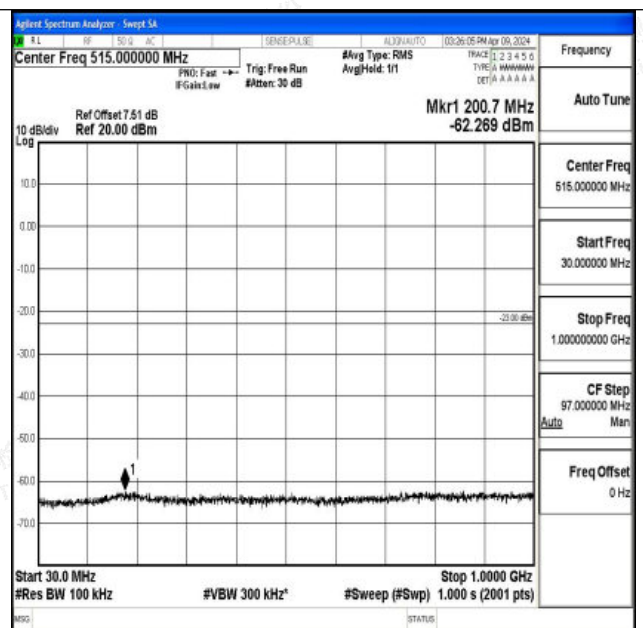
Band66_15MHz_16QAM_132322_1RB#0_30~1000_30~10
