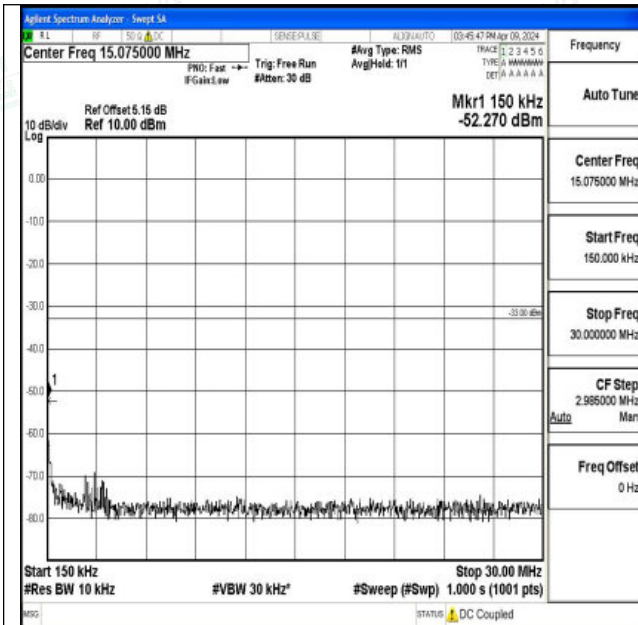
Band66_20MHz_16QAM_132572_1RB#0_0.15~30_0.15~30
