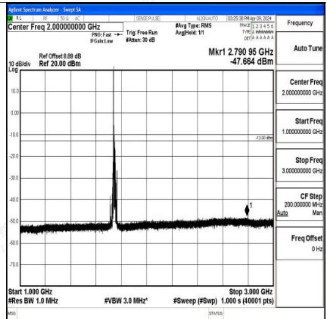
Band66_15MHz_QPSK_132322_1RB#0_1000~3000_1000 ~3000
