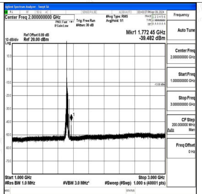
Band66_20MHz_QPSK_132072_1RB#0_1000~3000_1000~3000
