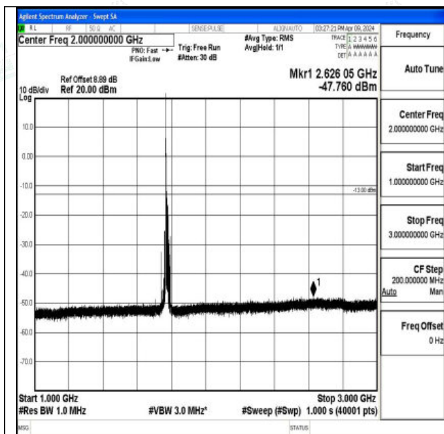
Band66_15MHz_16QAM_132597_1RB#0_1000~3000_10 00~3000
