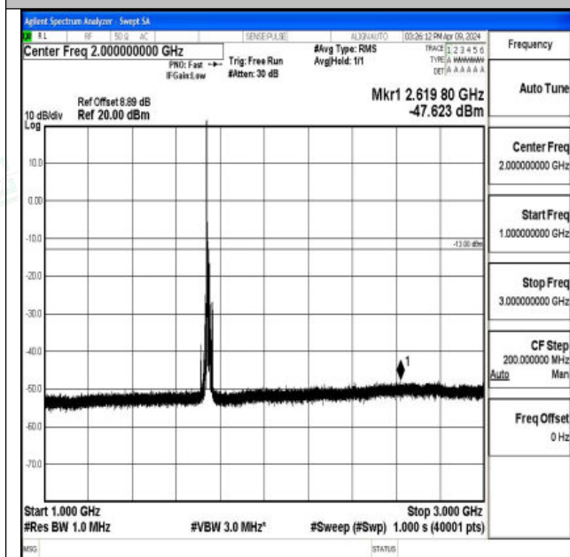
Band66_15MHz_16QAM_132322_1RB#0_1000~3000_10
