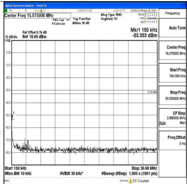
Band66_10MHz_QPSK_132322_1RB#0_0.15~30_0.15~30
