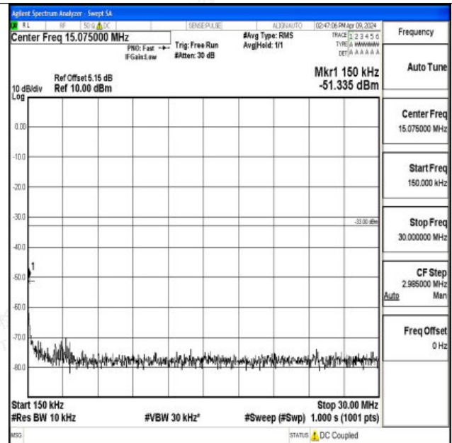
Band66_5MHz_QPSK_132647_1RB#0_0.15~30_0.15~30
