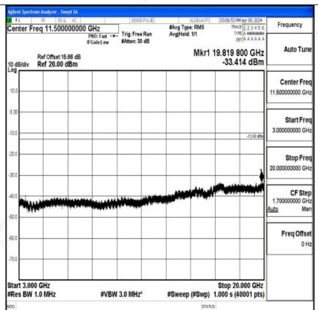
Band66_10MHz_16QAM_132322_1RB#0_3000~20000_30 00~20000
