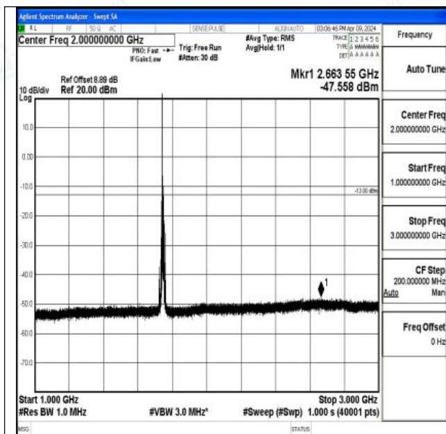
Band66_10MHz_16QAM_132322_1RB#0_1000~3000_10 00~3000
