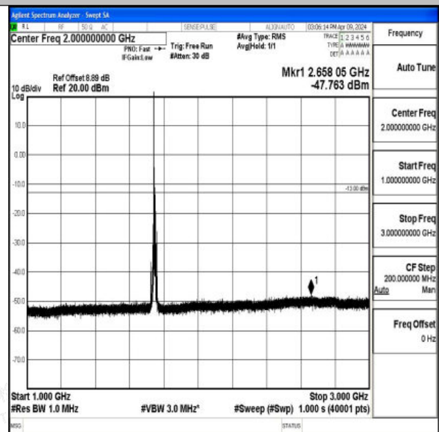
Band66_10MHz_QPSK_132322_1RB#0_1000~3000_1000 ~3000
