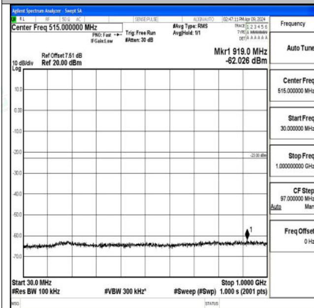
Band66_5MHz_QPSK_132647_1RB#0_30~1000_30~100 0
