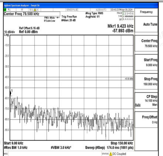
Band66_20MHz_16QAM_132072_1RB#0_0.009~0.15_0.009~0.15
