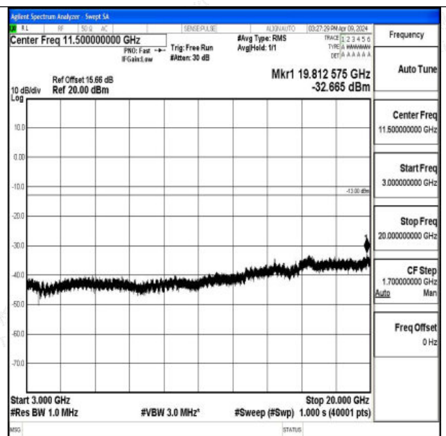
Band66_15MHz_16QAM_132597_1RB#0_3000~20000_30 00~20000
