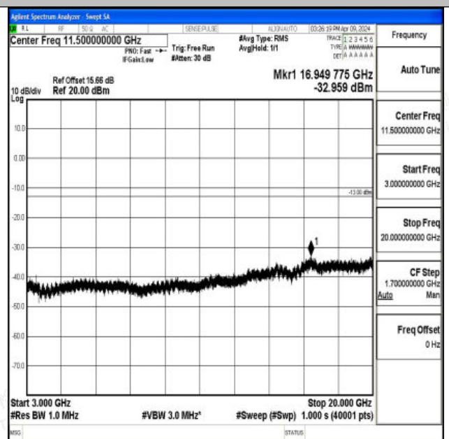
Band66_15MHz_16QAM_132322_1RB#0_3000~20000_30
