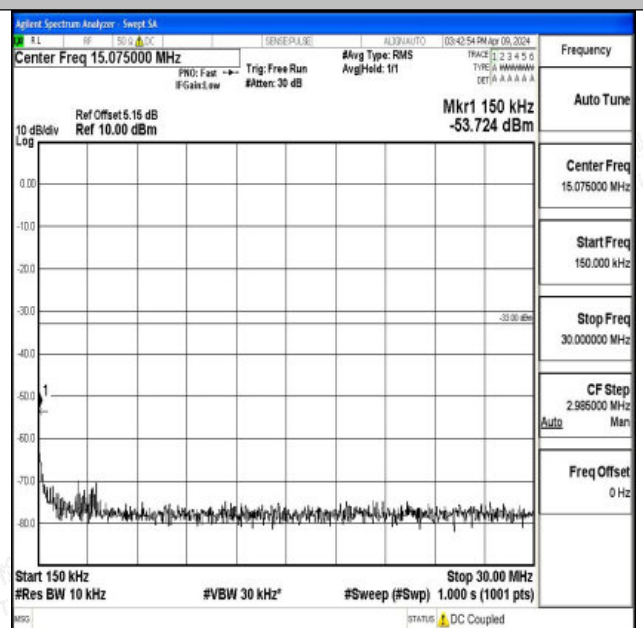
Band66_20MHz_QPSK_132072_1RB#0_0.15~30_0.15~30
