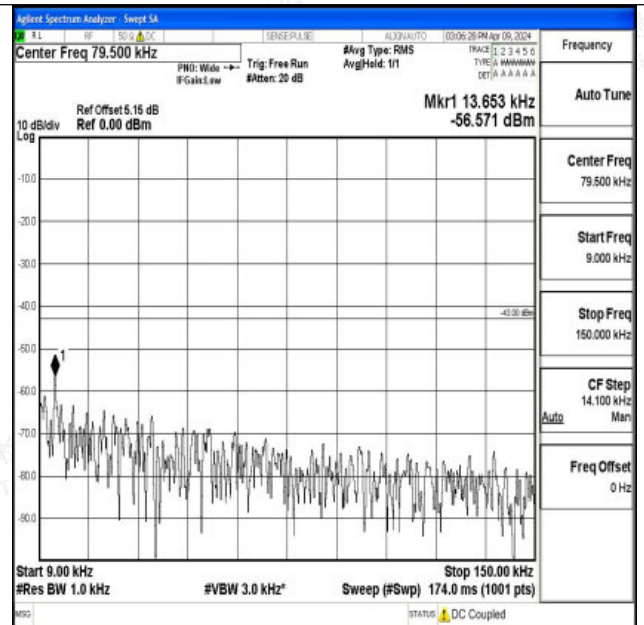
Band66_10MHz_16QAM_132322_1RB#0_0.009~0.15_0.00 9~0.15
