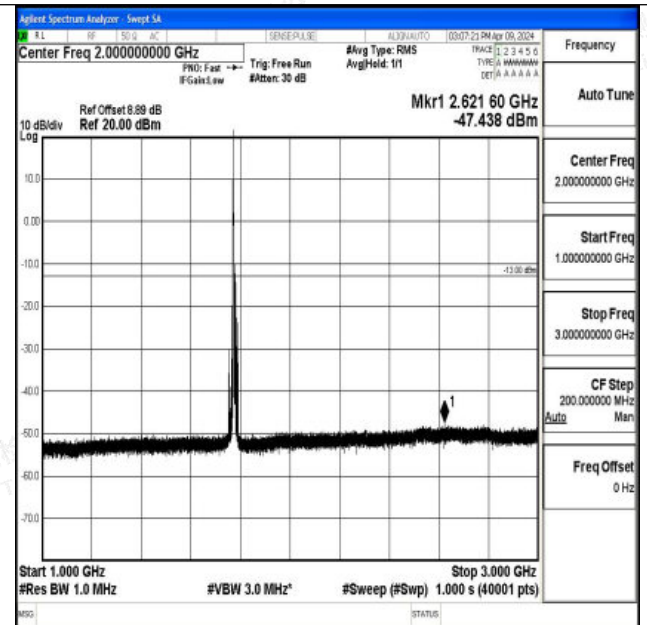
Band66_10MHz_QPSK_132622_1RB#0_1000~3000_1000~3000
