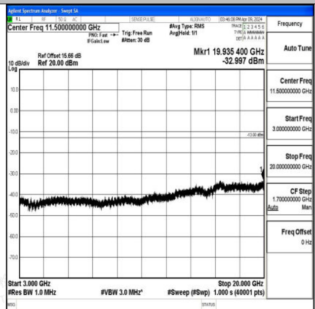
Band66_20MHz_16QAM_132572_1RB#0_3000~20000_30
