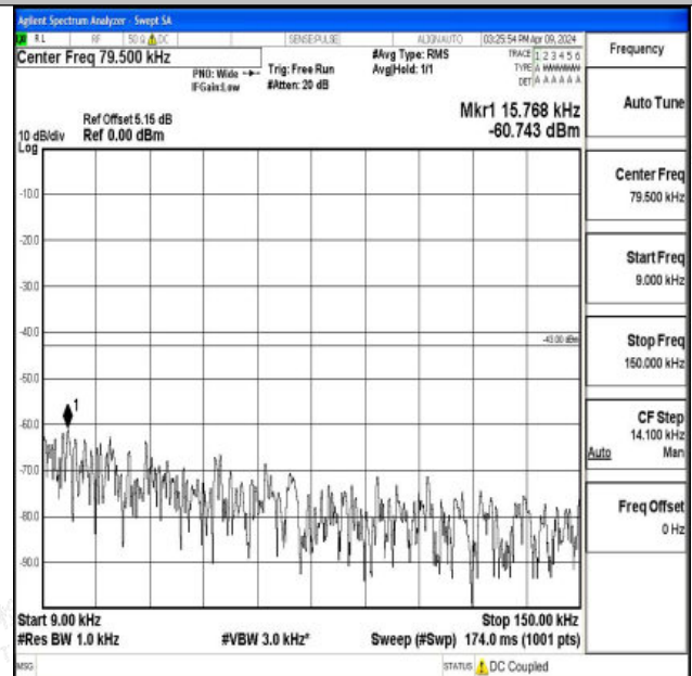
Band66_15MHz_16QAM_132322_1RB#0_0.009~0.15_0.00 9~0.15
