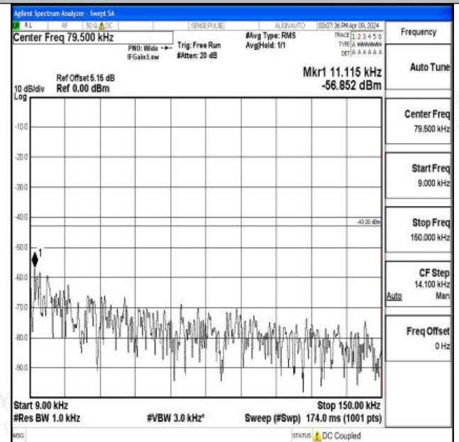
Band66_10MHz_16QAM_132622_1RB#0_0.009~0.15_0.009~0.15
