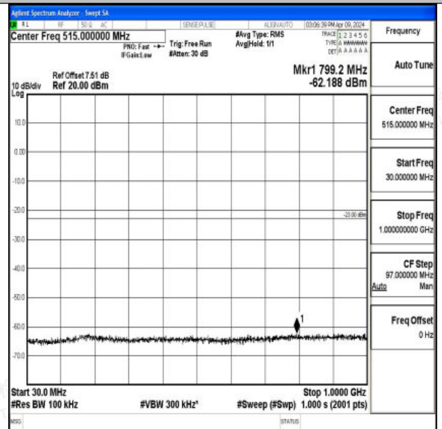
Band66_10MHz_16QAM_132322_1RB#0_30~1000_30~10 00
