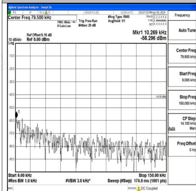
Band66_10MHz_QPSK_132622_1RB#0_0.009~0.15_0.00 9~0.15
