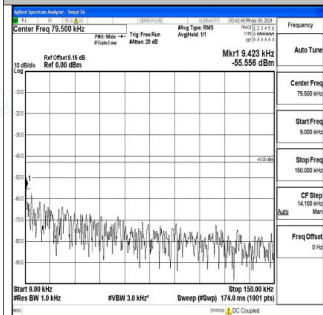
Band66_20MHz_QPSK_132072_1RB#0_0.009~0.15_0.00 9~0.15
