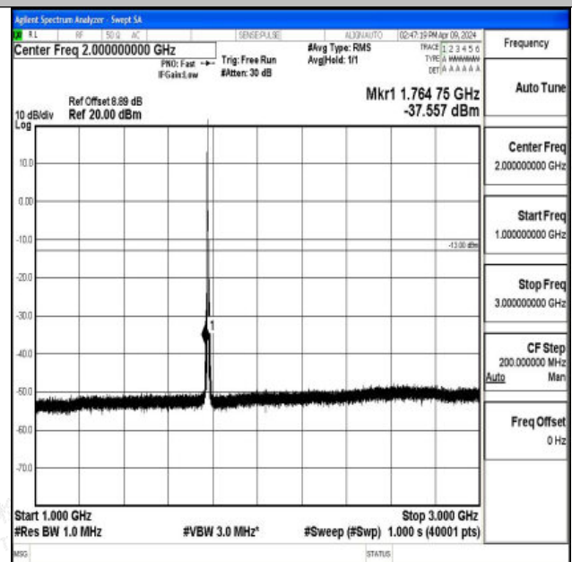
Band66_5MHz_QPSK_132647_1RB#0_1000~3000_1000~ 3000
