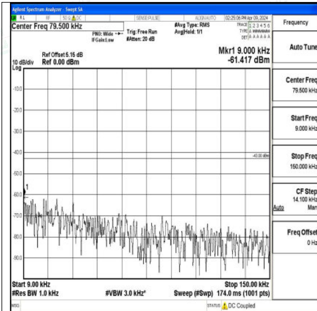
Band66_3MHz_QPSK_132322_1RB#0_0.009~0.15_0.009~0.15
