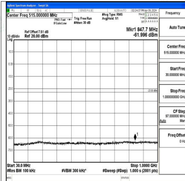
Band66_3MHz_QPSK_131987_1RB#0_30~1000_30~100
