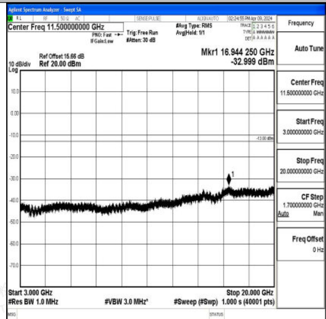
Band66_3MHz_16QAM_131987_1RB#0_3000~20000_300
