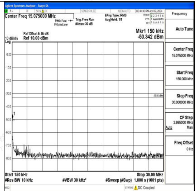
Band66_5MHz_QPSK_131997_1RB#0_0.15~30_0.15~30
