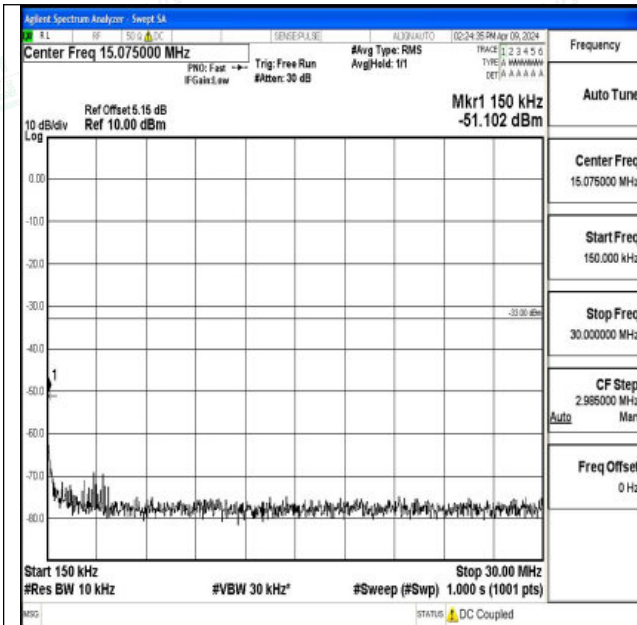
Band66_3MHz_16QAM_131987_1RB#0_0.15~30_0.15~3
