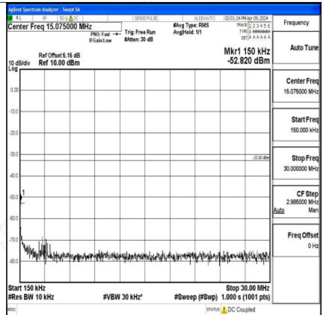
Band66_1.4MHz_QPSK_132665_1RB#0_0.15~30_0.15~30
