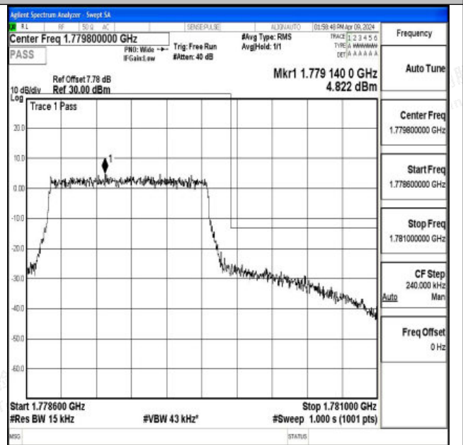
Band66_1.4MHz_16QAM_132665_6RB#0
