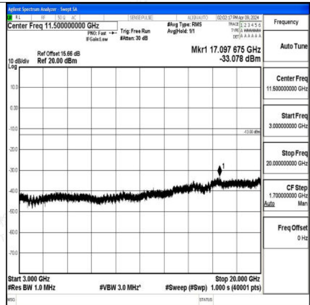
Band66_1.4MHz_16QAM_132665_1RB#0_3000~20000_30 00~20000
