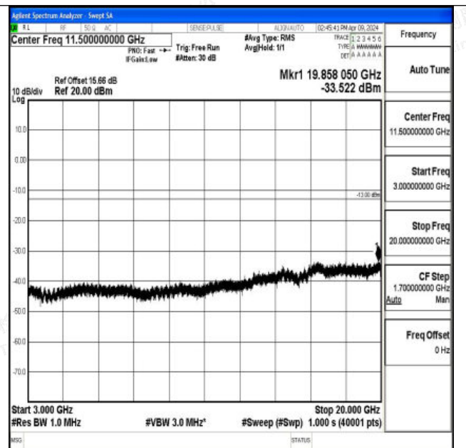
Band66_5MHz_16QAM_131997_1RB#0_3000~20000_300 0~20000
