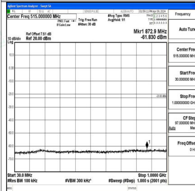
Band66_1.4MHz_QPSK_131979_1RB#0_30~1000_30~1000
