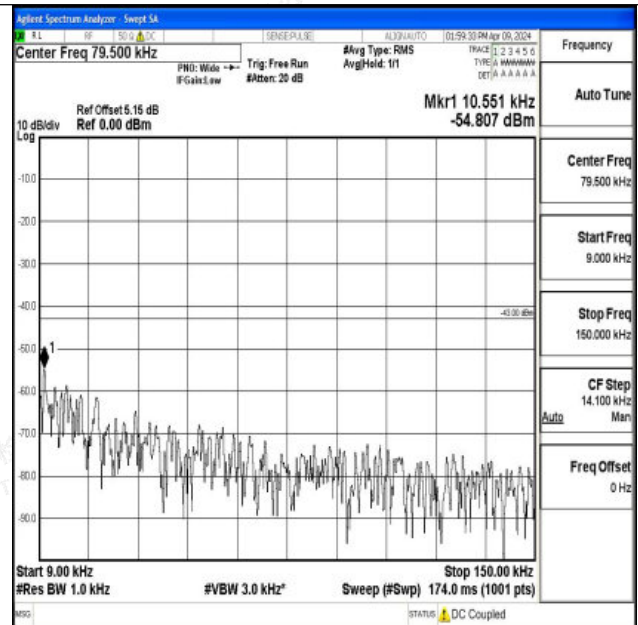
Band66_1.4MHz_16QAM_131979_1RB#0_0.009~0.15_0.0 09~0.15
