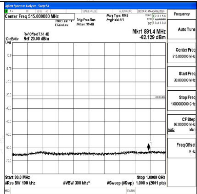
Band66_3MHz_16QAM_131987_1RB#0_30~1000_30~100
