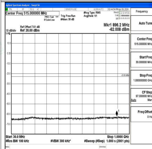
Band66_5MHz_QPSK_131997_1RB#0_30~1000_30~1000
