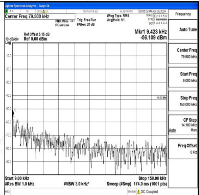
Band66_1.4MHz_16QAM_132665_1RB#0_0.009~0.15_0.0 09~0.15
