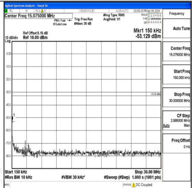
Band66_1.4MHz_QPSK_132322_1RB#0_0.15~30_0.15~30 0.15~30
