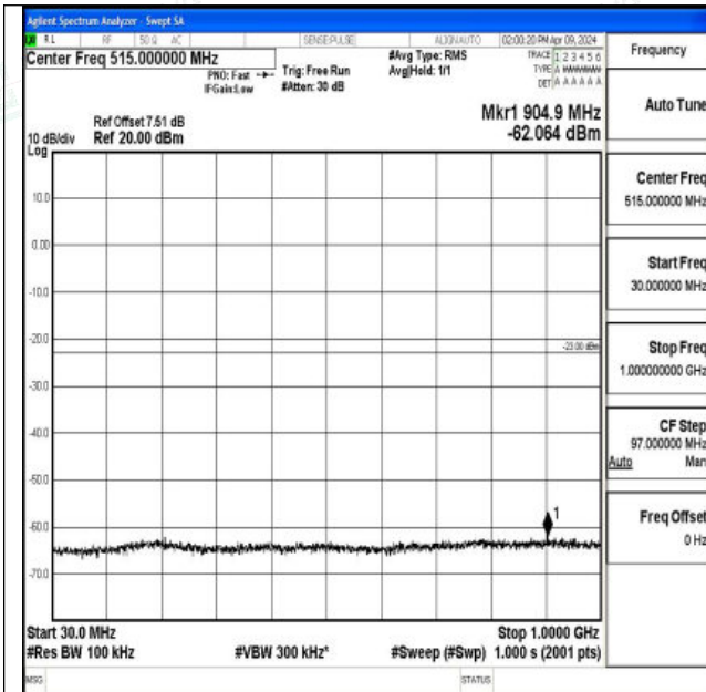
Band66_1.4MHz_QPSK_132322_1RB#0_30~1000_30~1000 00
