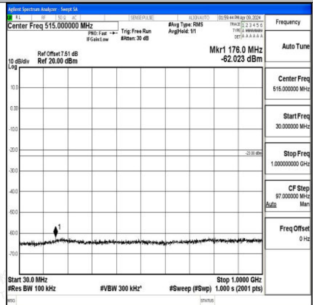
Band66_1.4MHz_16QAM_131979_1RB#0_30~1000_30~1 000
