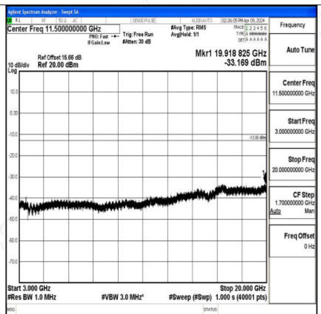
Band66_3MHz_16QAM_132322_1RB#0_3000~20000_300 0~20000
