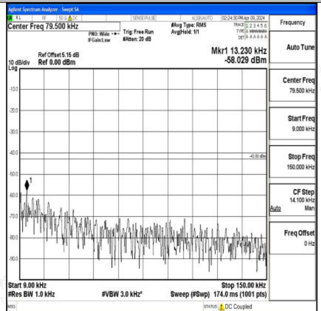
Band66_3MHz_16QAM_131987_1RB#0_0.009~0.15_0.009~0.15
