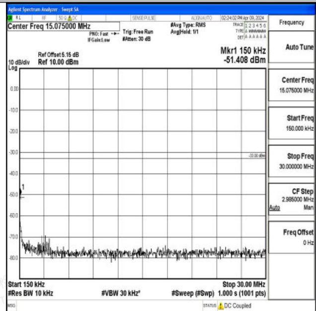
Band66_3MHz_QPSK_131987_1RB#0_0.15~30_0.15~30
