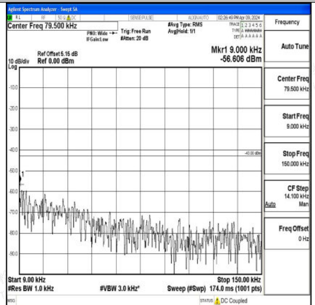
Band66_3MHz_16QAM_132657_1RB#0_0.009~0.15_0.009~0.15
