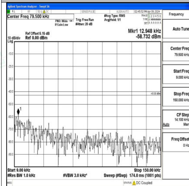
Band66_5MHz_QPSK_132322_1RB#0_0.009~0.15_0.009 ~0.15
