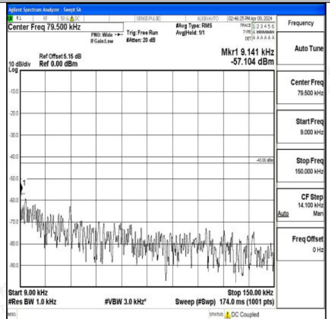
Band66_5MHz_16QAM_132322_1RB#0_0.009~0.15_0.009~0.15
