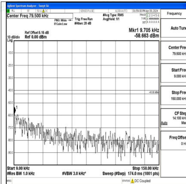
Band66_1.4MHz_QPSK_131979_1RB#0_0.009~0.15_0.09~0.15
