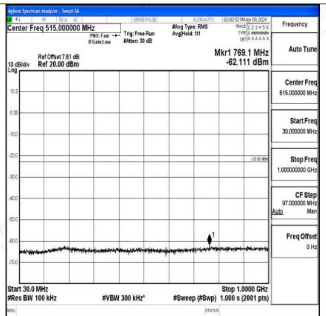
Band66_1.4MHz_16QAM_132322_1RB#0_30~1000_30~1000
