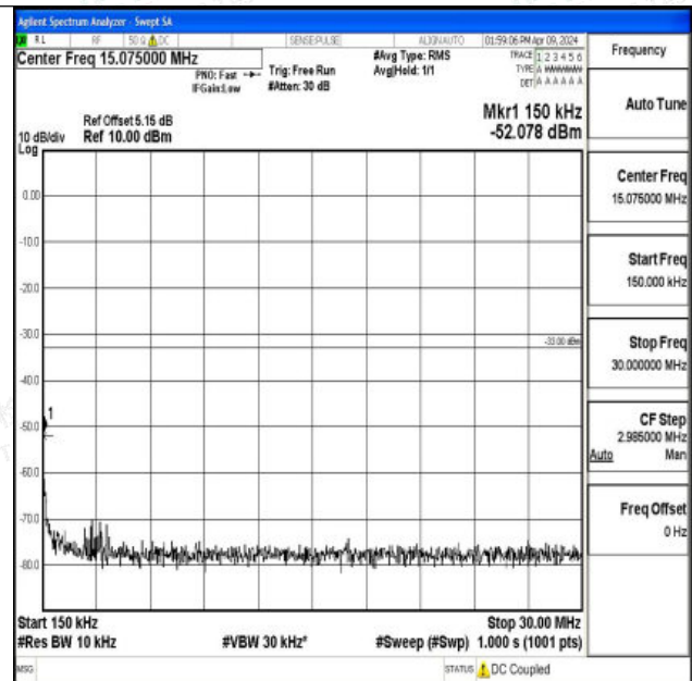
Band66_1.4MHz_QPSK_131979_1RB#0_0.15~30_0.15~30
