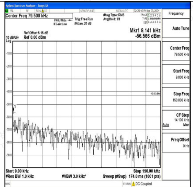
Band66_3MHz_16QAM_132322_1RB#0_0.009~0.15_0.009 ~0.15
