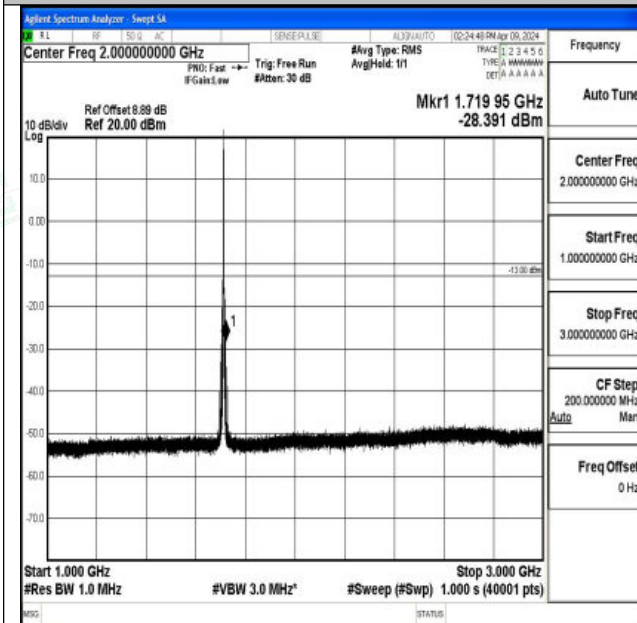
Band66_3MHz_16QAM_131987_1RB#0_1000~3000_100
