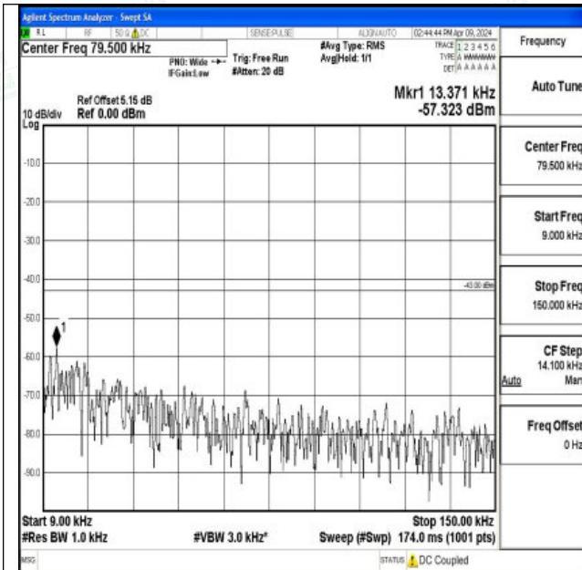
Band66_5MHz_QPSK_131997_1RB#0_0.009~0.15_0.009~0.15
