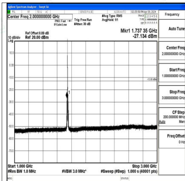
Band66_3MHz_16QAM_132322_1RB#0_1000~3000_100 0~3000
