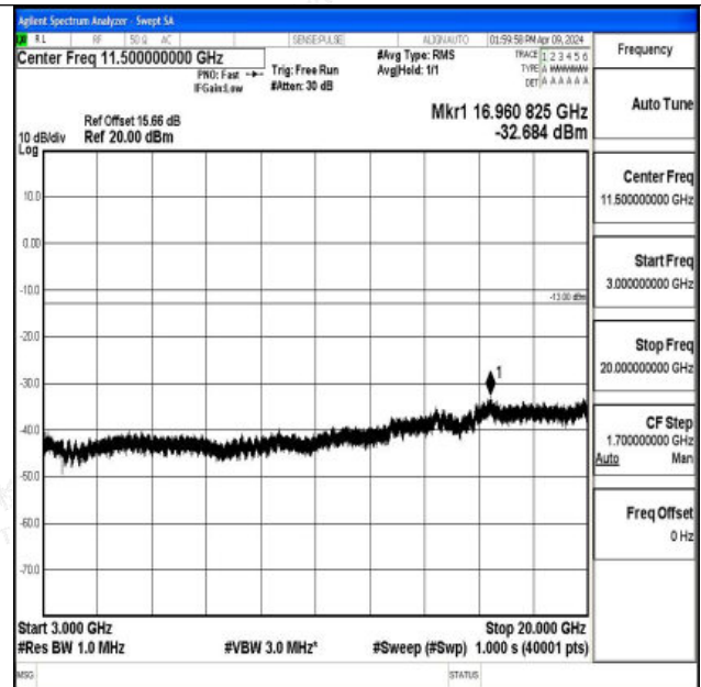
Band66_1.4MHz_16QAM_131979_1RB#0_3000~20000_30 00~20000
