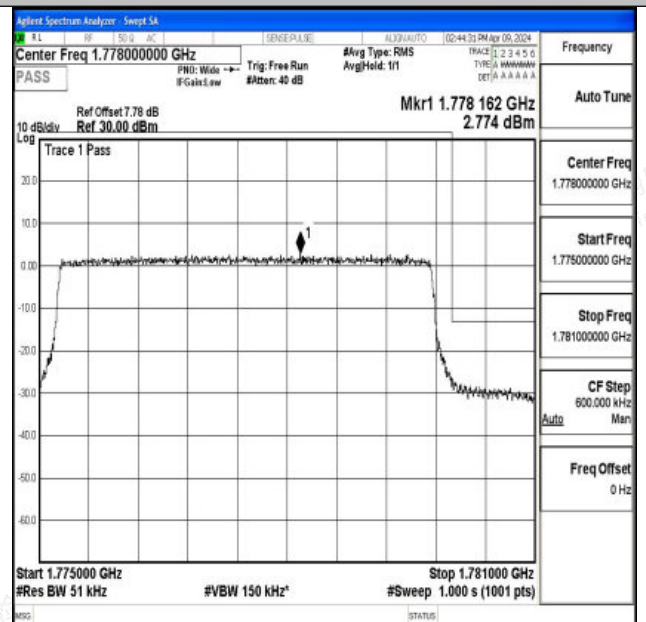
Band66_5MHz_16QAM_132647_25RB#0
