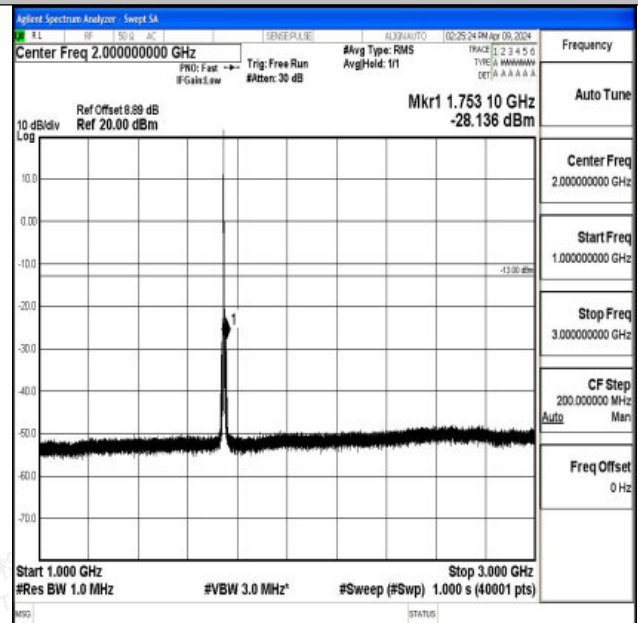
Band66_3MHz_QPSK_132322_1RB#0_1000~3000_1000~3000
