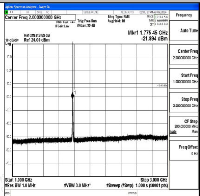
Band66_1.4MHz_QPSK_132665_1RB#0_1000~3000_1000~3000
