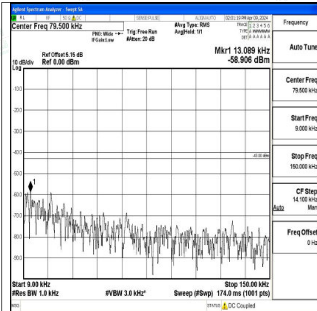
Band66_1.4MHz_QPSK_132665_1RB#0_0.009~0.15_0.09~0.15
