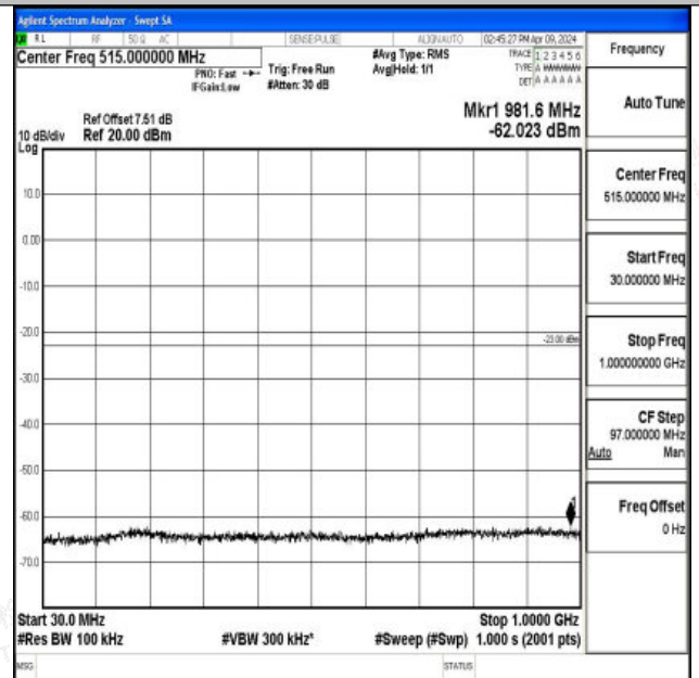
Band66_5MHz_16QAM_131997_1RB#0_30~1000_30~100 0
