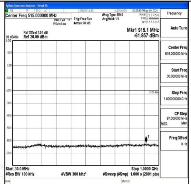
Band66_3MHz_16QAM_132322_1RB#0_30~1000_30~100 0
