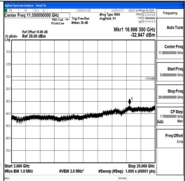
Band66_3MHz_16QAM_132657_1RB#0_3000~20000_300
