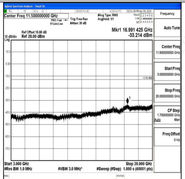
Band66_1.4MHz_16QAM_132322_1RB#0_3000~20000_3000~20000
