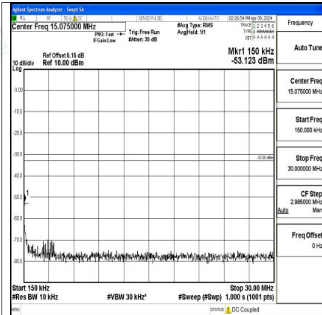
Band66_3MHz_16QAM_132657_1RB#0_0.15~30_0.15~3
