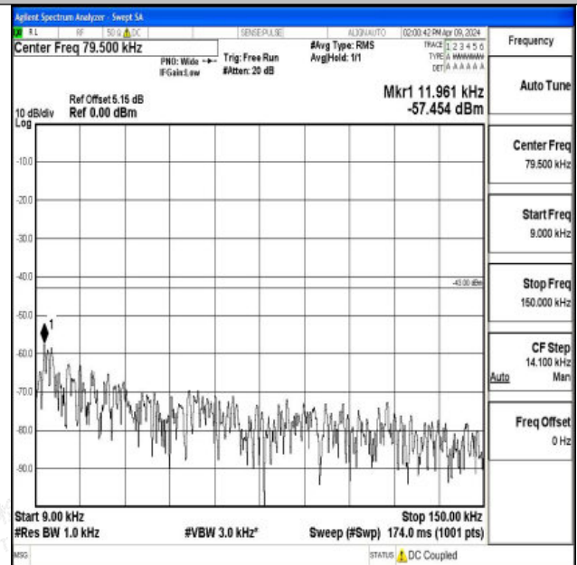
Band66_1.4MHz_16QAM_132322_1RB#0_0.009~0.15_0.009~0.15 09~0.15
