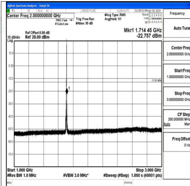
Band66_1.4MHz_16QAM_131979_1RB#0_1000~3000_10 00~3000
