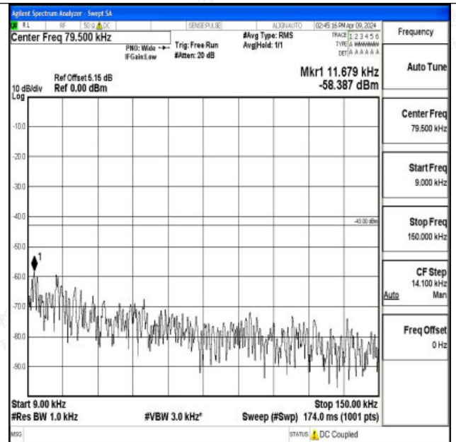
Band66_5MHz_16QAM_131997_1RB#0_0.009~0.15_0.009 ~0.15
