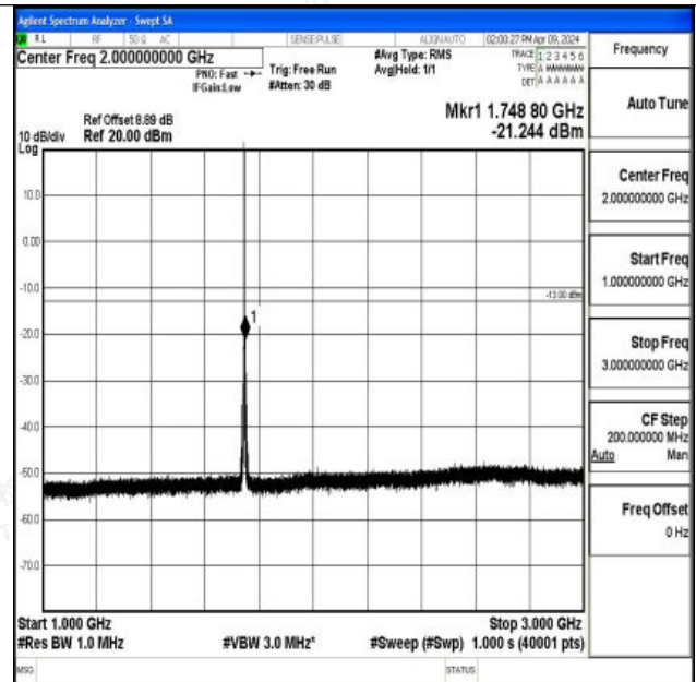
Band66_1.4MHz_QPSK_132322_1RB#0_1000~3000_1000~3000 ~3000
