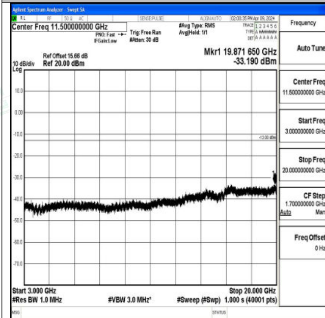
Band66_1.4MHz_QPSK_132322_1RB#0_3000~20000_3000~20000 00~20000
