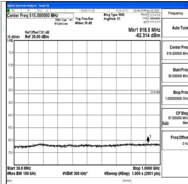
Band66_5MHz_QPSK_132322_1RB#0_30~1000_30~100
