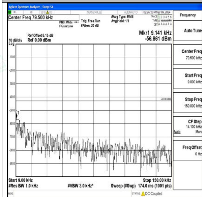
Band66_3MHz_QPSK_132657_1RB#0_0.009~0.15_0.009 ~0.15
