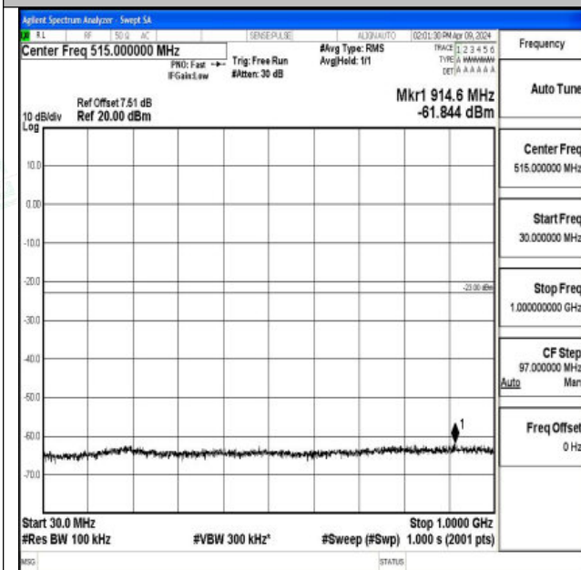
Band66_1.4MHz_QPSK_132665_1RB#0_30~1000_30~1000
