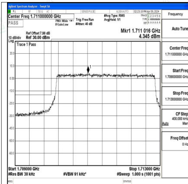
Band66_3MHz_QPSK_131987_15RB#0
