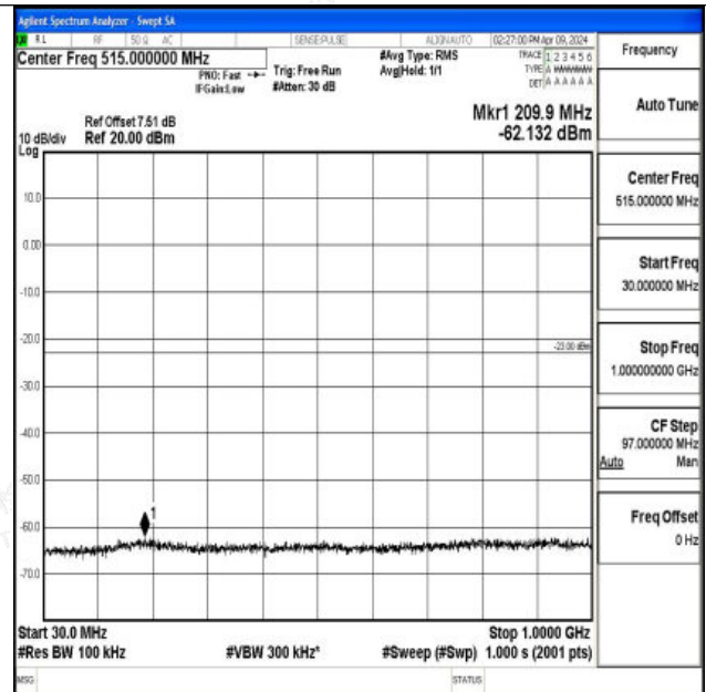
Band66_3MHz_16QAM_132657_1RB#0_30~1000_30~100
