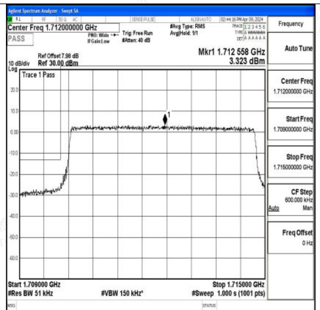
Band66_5MHz_16QAM_131997_25RB#0
