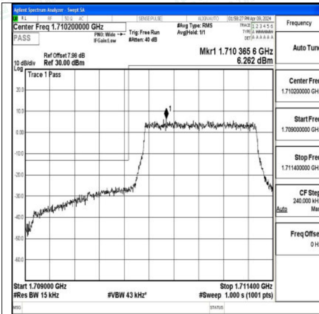
Band66_1.4MHz_QPSK_131979_6RB#0
