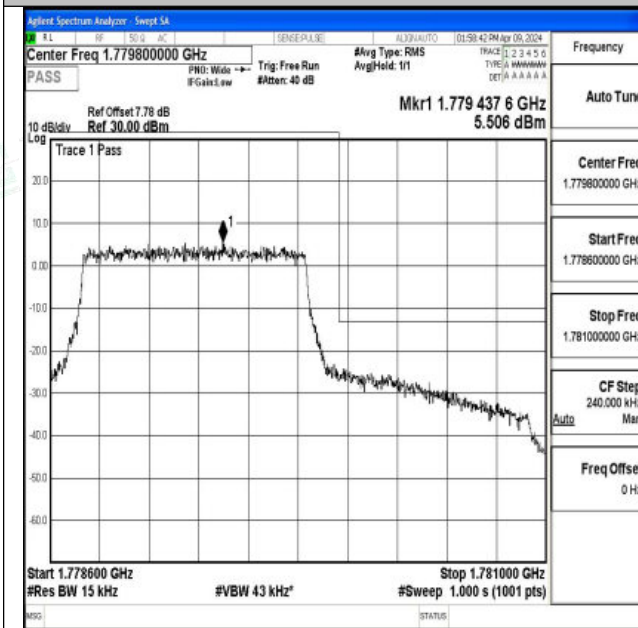
Band66_1.4MHz_QPSK_132665_6RB#0
