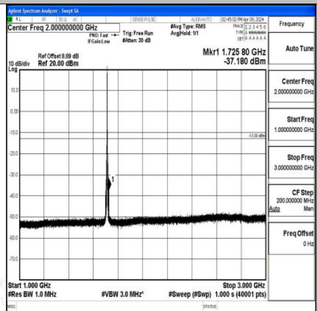
Band66_5MHz_QPSK_131997_1RB#0_1000~3000_1000~3000
