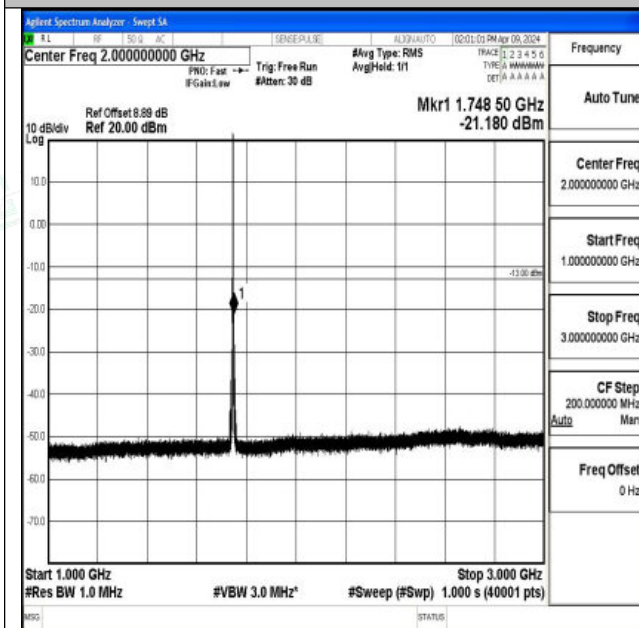
Band66_1.4MHz_16QAM_132322_1RB#0_1000~3000_1000~3000
