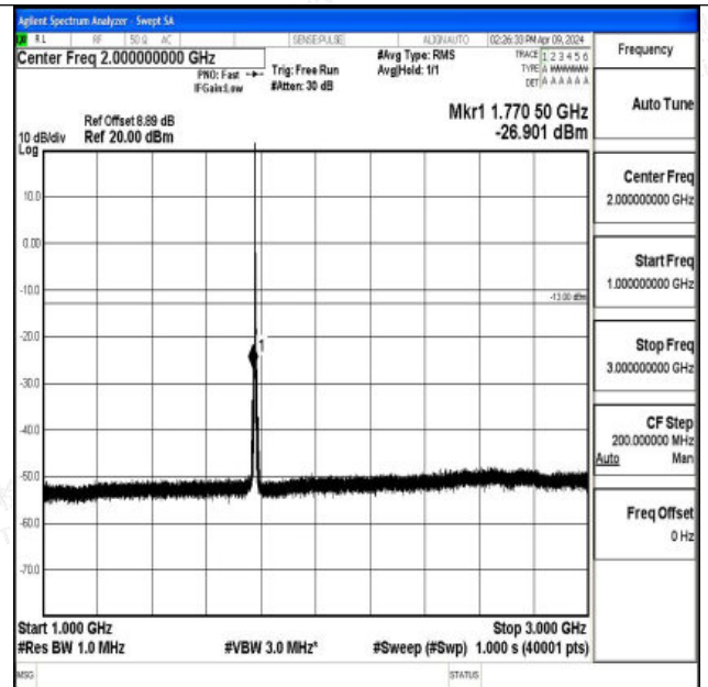
Band66_3MHz_QPSK_132657_1RB#0_1000~3000_1000~3000
