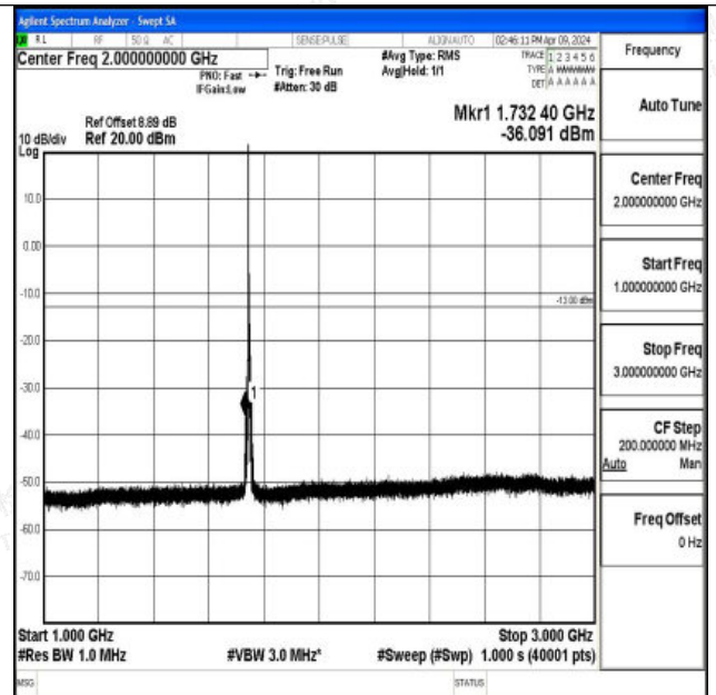
Band66_5MHz_QPSK_132322_1RB#0_1000~3000_1000~3000
