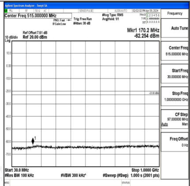
Band66_1.4MHz_16QAM_132665_1RB#0_30~1000_30~1 000
