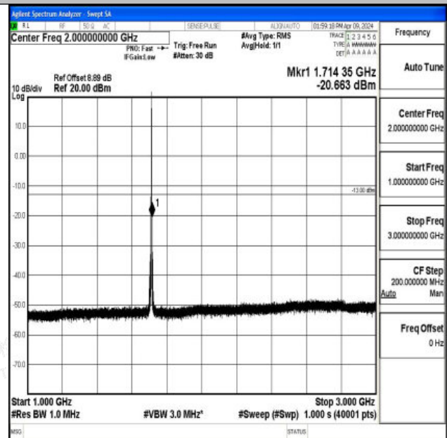
Band66_1.4MHz_QPSK_131979_1RB#0_1000~3000_1000~3000
