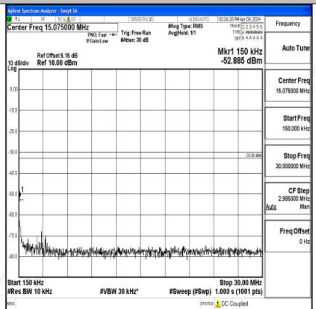
Band66_3MHz_QPSK_132657_1RB#0_0.15~30_0.15~30
