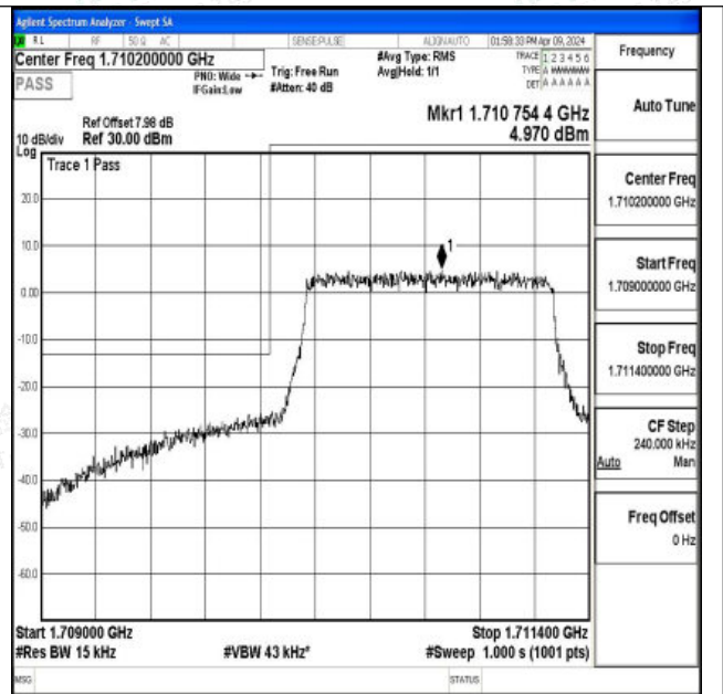
Band66_1.4MHz_16QAM_131979_6RB#0
