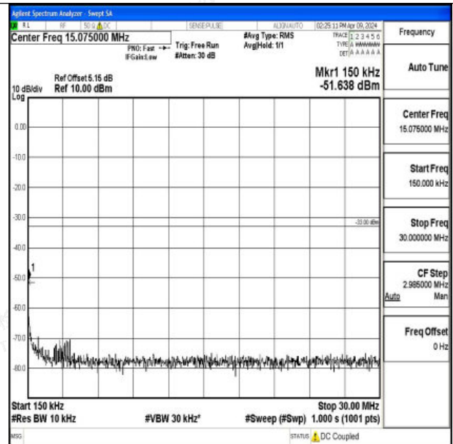
Band66_3MHz_QPSK_132322_1RB#0_0.15~30_0.15~30
