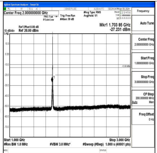
Band66_3MHz_QPSK_131987_1RB#0_1000~3000_1000~3000
