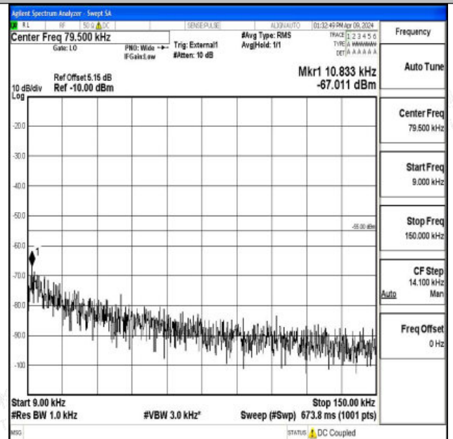
Band41_20MHz_16QAM_39750_1RB#0_0.009~0.15_0.009~0.15
