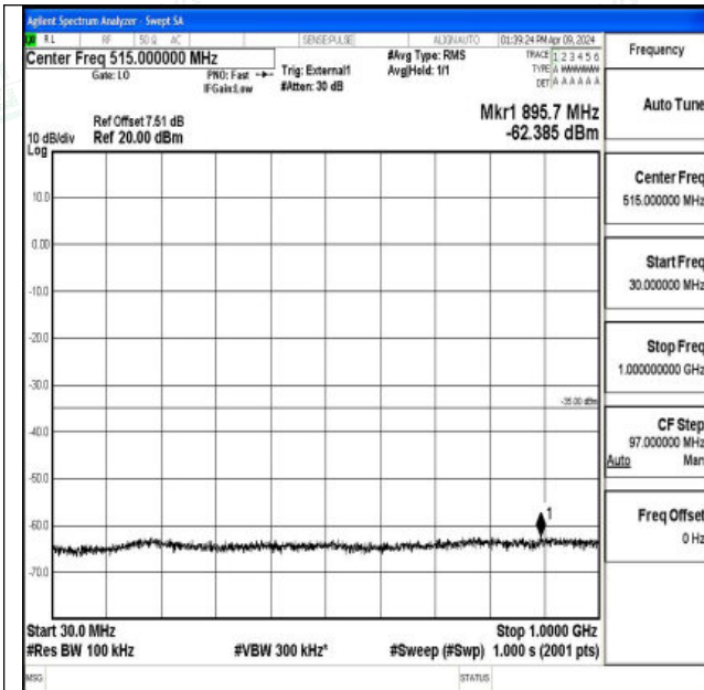
Band41_20MHz_QPSK_41490_1RB#0_30~1000_30~100
