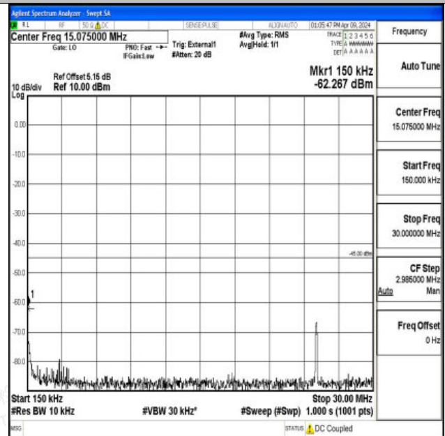
Band41_15MHz_QPSK_40620_1RB#0_0.15~30_0.15~30
