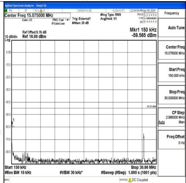
Band41_10MHz_QPSK_40620_1RB#0_0.15~30_0.15~30
