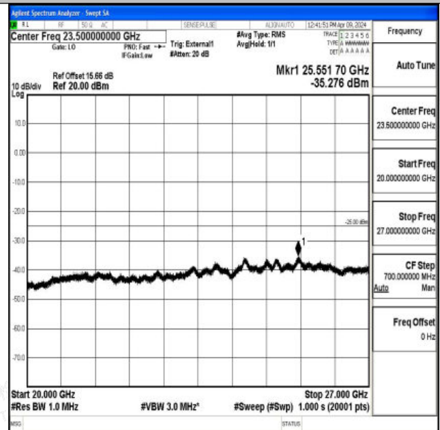
Band41_10MHz_16QAM_41540_1RB#0_20000~27000_20
