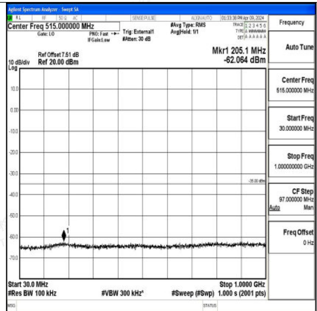
Band41_20MHz_16QAM_39750_1RB#0_30~1000_30~100
