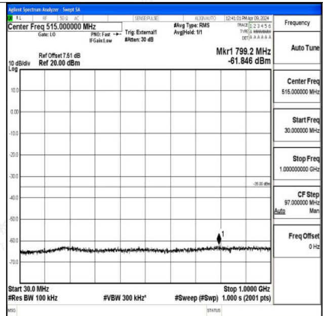
Band41_10MHz_16QAM_41540_1RB#0_30~1000_30~100
