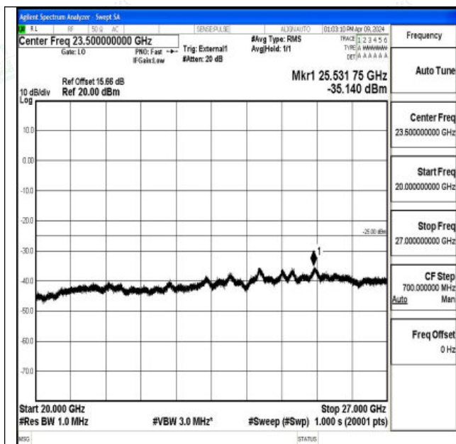
Band41_15MHz_QPSK_39725_1RB#0_20000~27000_20000~27000
