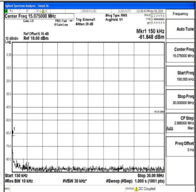
Band41_10MHz_QPSK_41540_1RB#0_0.15~30_0.15~30
