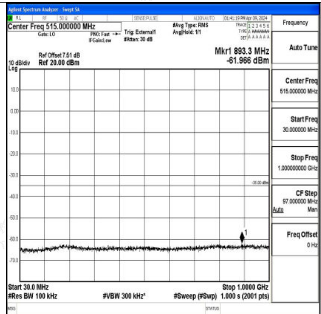
Band41_20MHz_16QAM_41490_1RB#0_30~1000_30~100
