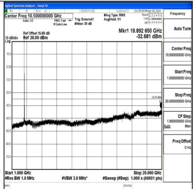
Band41_20MHz_QPSK_40620_1RB#0_1000~20000_1000 ~20000
