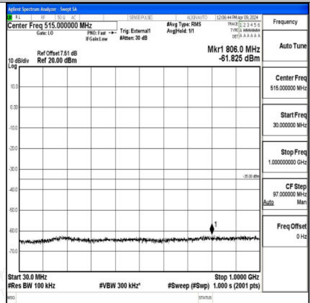
Band41_5MHz_16QAM_41565_1RB#0_30~1000_30~1000
