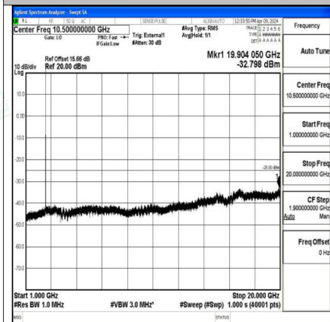
Band41_10MHz_16QAM_39700_1RB#0_1000~20000_1000~20000
