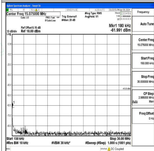
Band41_15MHz_16QAM_39725_1RB#0_0.15~30_0.15~30
