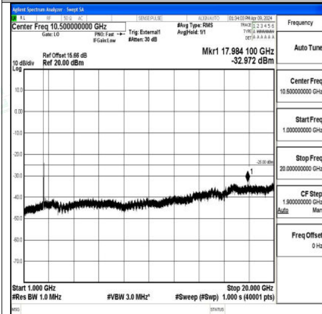
Band41_20MHz_16QAM_39750_1RB#0_1000~20000_10
