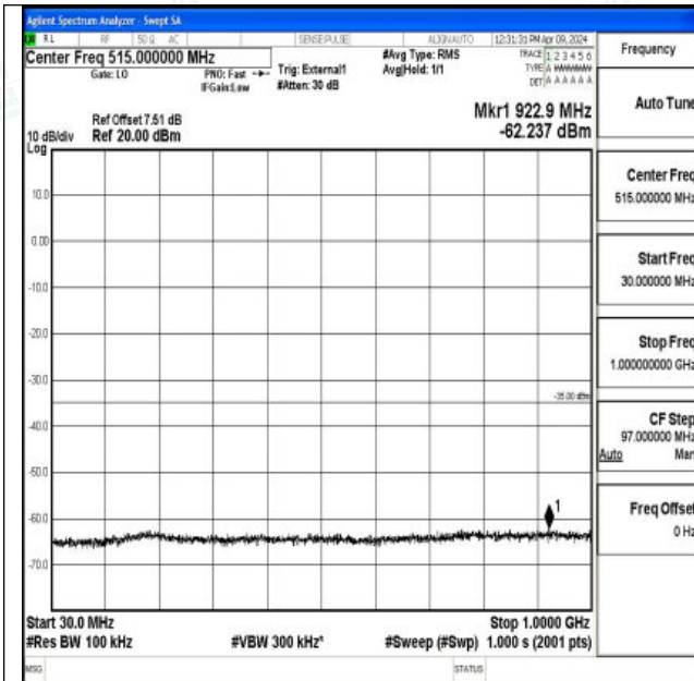
Band41_10MHz_QPSK_39700_1RB#0_30~1000_30~100
