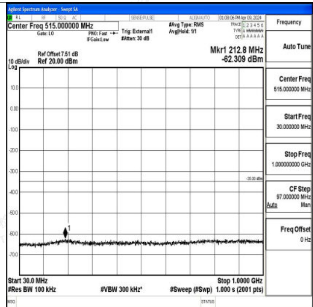
Band41_15MHz_16QAM_40620_1RB#0_30~1000_30~100
