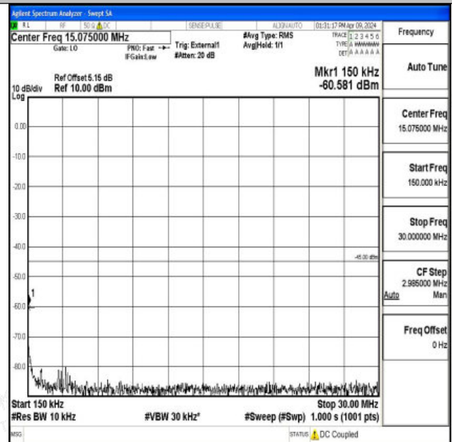
Band41_20MHz_QPSK_39750_1RB#0_0.15~30_0.15~30
