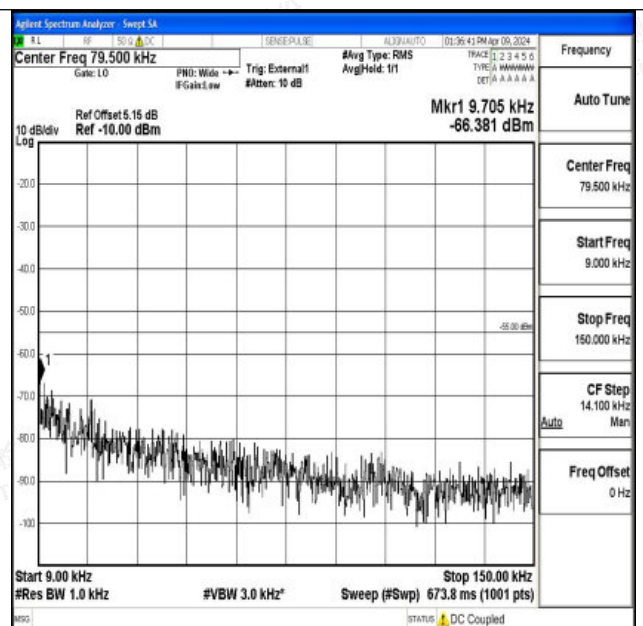
Band41_20MHz_16QAM_40620_1RB#0_0.009~0.15_0.009 ~0.15
