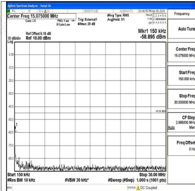
Band41_20MHz_16QAM_41490_1RB#0_0.15~30_0.15~3
