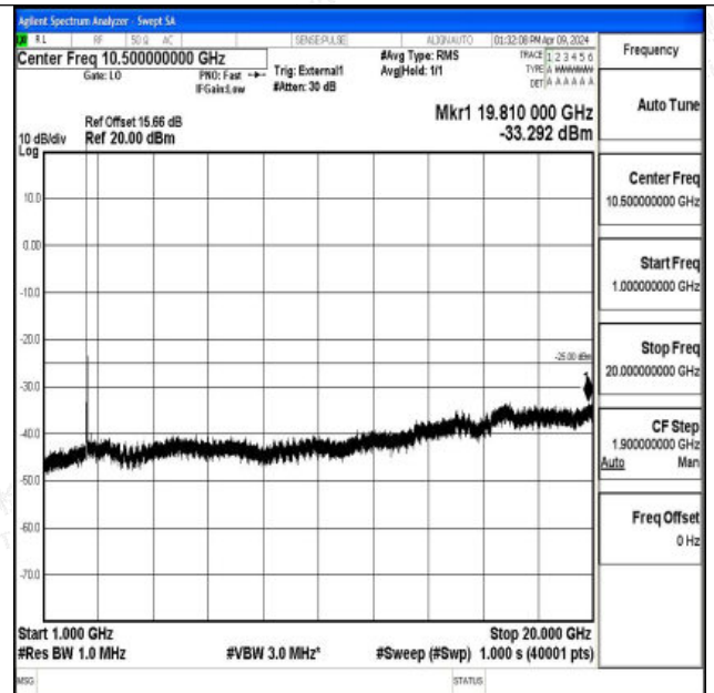
Band41_20MHz_QPSK_39750_1RB#0_1000~20000_1000~20000
