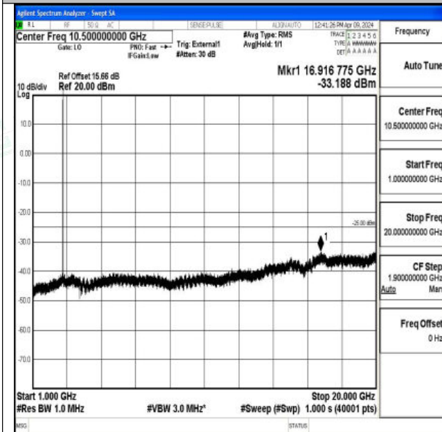
Band41_10MHz_16QAM_41540_1RB#0_1000~20000_10
