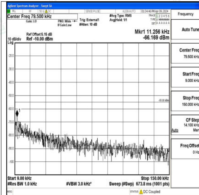
Band41_20MHz_QPSK_40620_1RB#0_0.009~0.15_0.009 ~0.15
