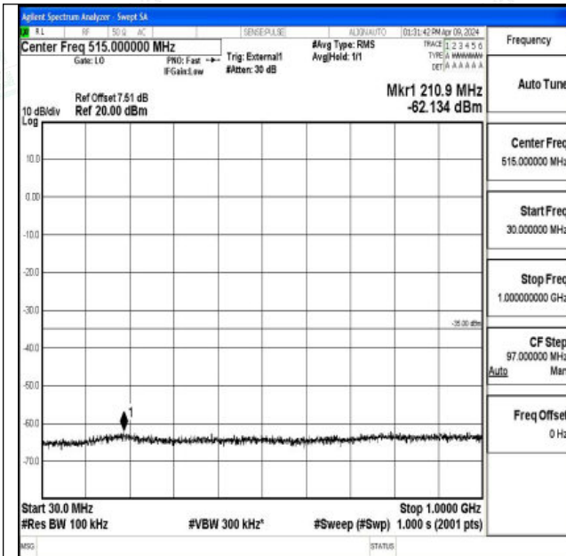
Band41_20MHz_QPSK_39750_1RB#0_30~1000_30~100
