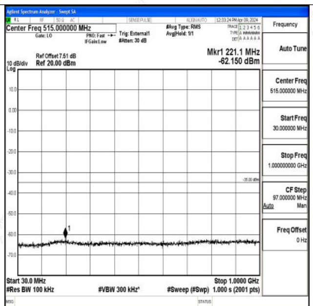
Band41_10MHz_16QAM_39700_1RB#0_30~1000_30~100
