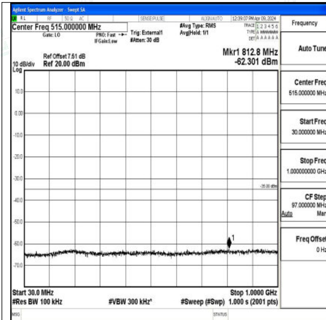
Band41_10MHz_QPSK_41540_1RB#0_30~1000_30~100
