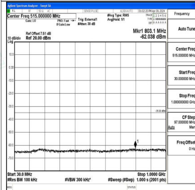
Band41_15MHz_QPSK_39725_1RB#0_30~1000_30~100 0
