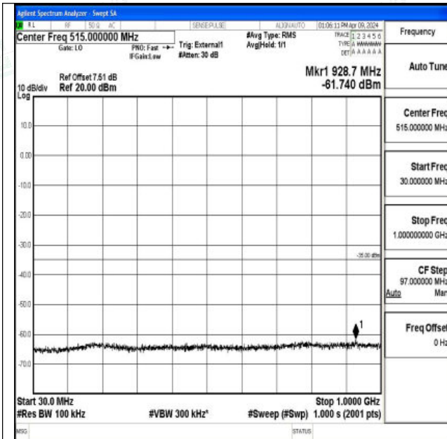
Band41_15MHz_QPSK_40620_1RB#0_30~1000_30~100
