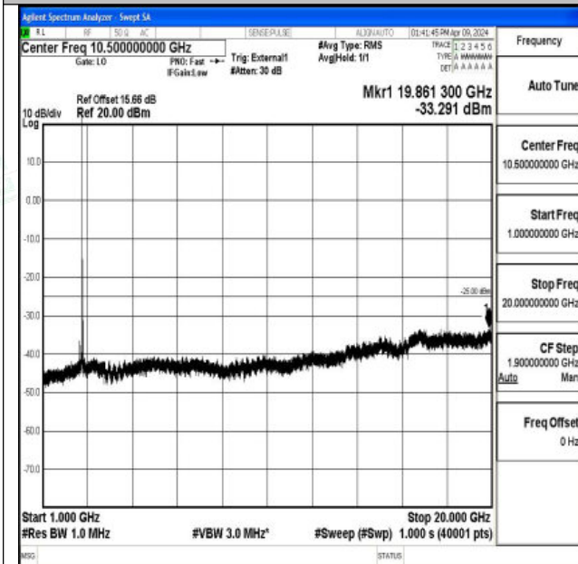
Band41_20MHz_16QAM_41490_1RB#0_1000~20000_10
