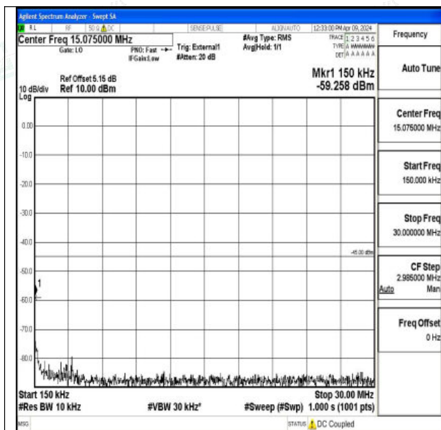
Band41_10MHz_16QAM_39700_1RB#0_0.15~30_0.15~3
