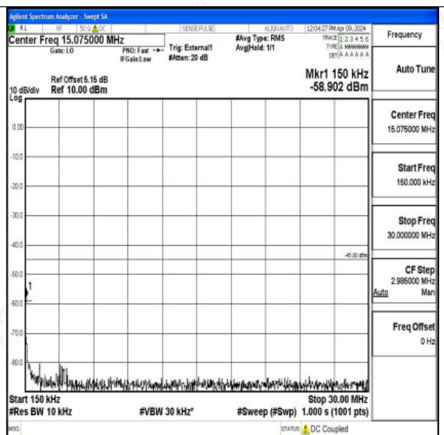
Band41_5MHz_QPSK_41565_1RB#0_0.15~30_0.15~30
