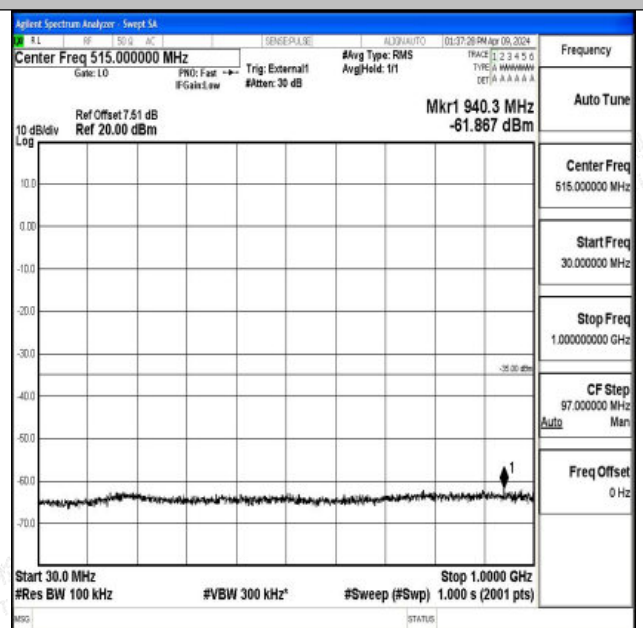
Band41_20MHz_16QAM_40620_1RB#0_30~1000_30~1000
