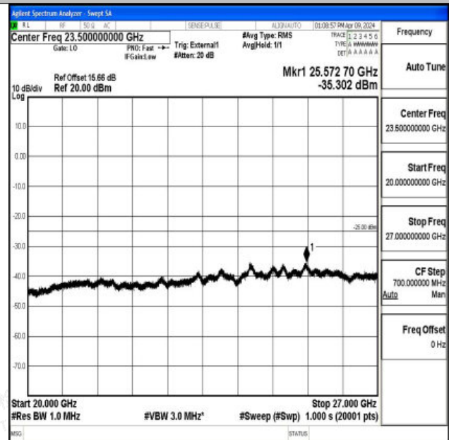
Band41_15MHz_16QAM_40620_1RB#0_20000~27000_20000~27000
