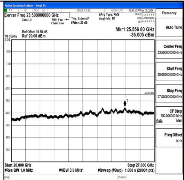
Band41_20MHz_16QAM_41490_1RB#0_20000~27000_20
