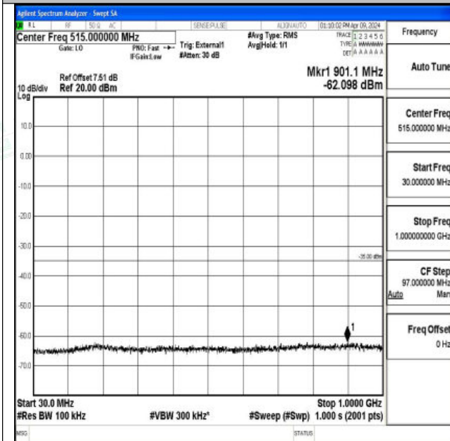
Band41_15MHz_QPSK_41515_1RB#0_30~1000_30~100 0
