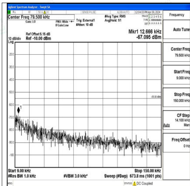
Band41_5MHz_QPSK_41565_1RB#0_0.009~0.15_0.009~0.15
