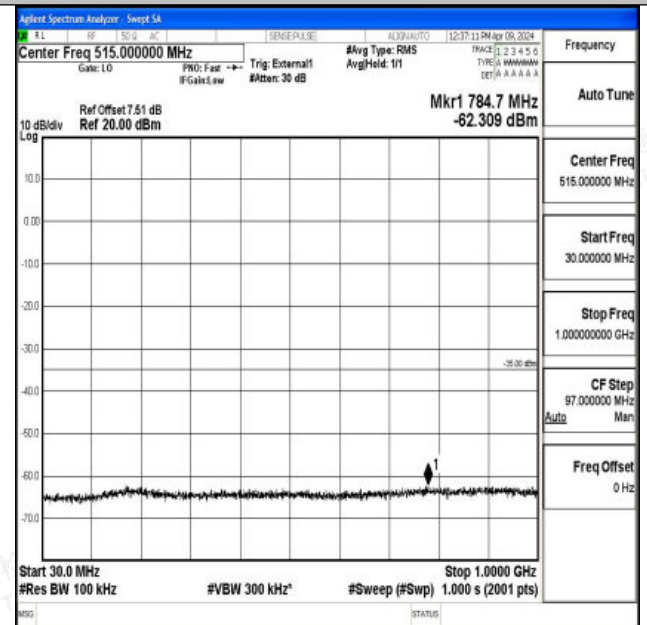
Band41_10MHz_16QAM_40620_1RB#0_30~1000_30~1000
