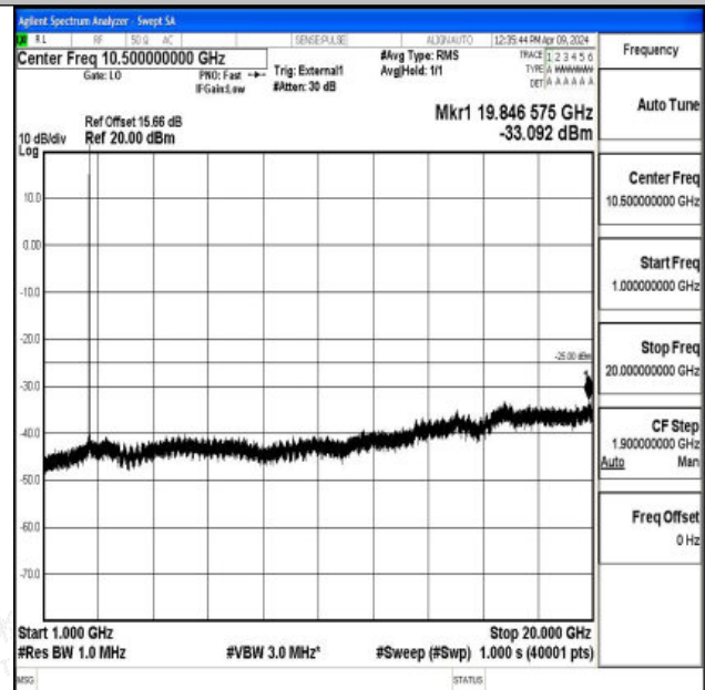
Band41_10MHz_QPSK_40620_1RB#0_1000~20000_1000~20000
