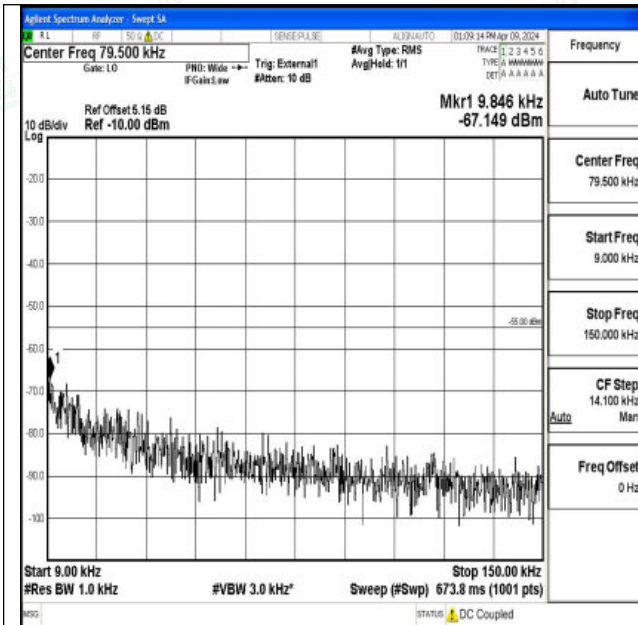
Band41_15MHz_QPSK_41515_1RB#0_0.009~0.15_0.009 ~0.15
