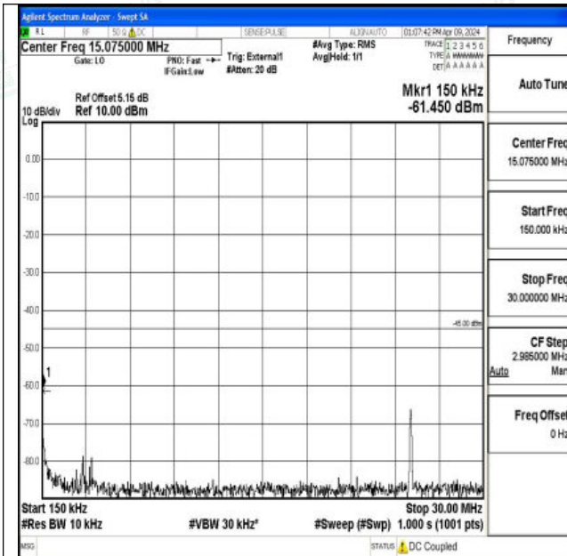
Band41_15MHz_16QAM_40620_1RB#0_0.15~30_0.15~3
