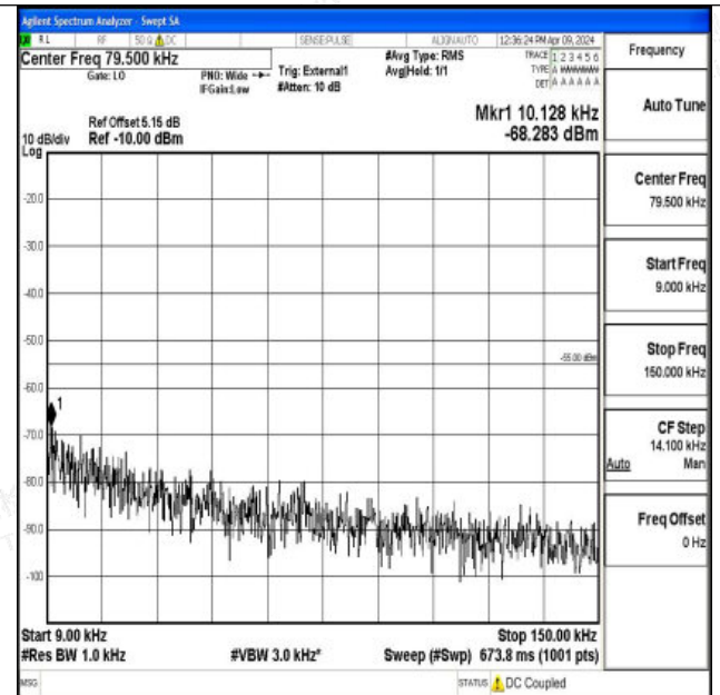
Band41_10MHz_16QAM_40620_1RB#0_0.009~0.15_0.009~0.15
