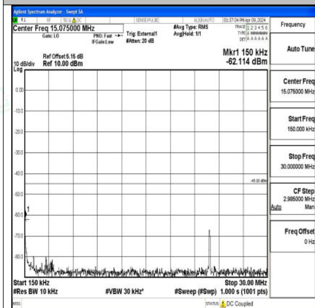
Band41_20MHz_16QAM_40620_1RB#0_0.15~30_0.15~30
