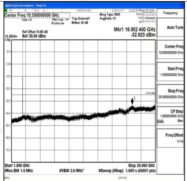
Band41_10MHz_QPSK_39700_1RB#0_1000~20000_1000~20000
