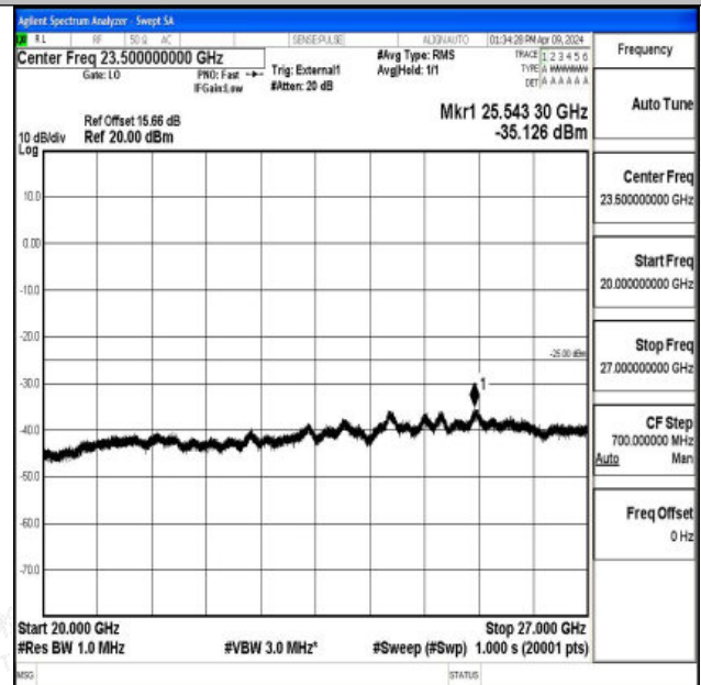
Band41_20MHz_16QAM_39750_1RB#0_20000~27000_20
