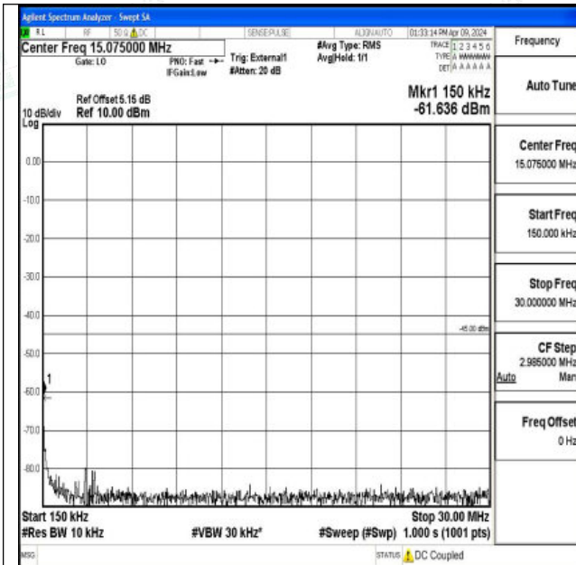
Band41_20MHz_16QAM_39750_1RB#0_0.15~30_0.15~3
