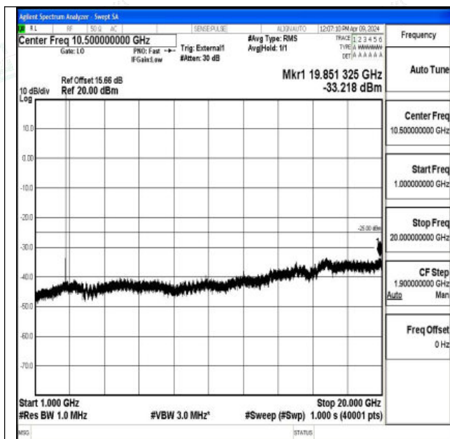
Band41_5MHz_16QAM_41565_1RB#0_1000~20000_100 0~20000
