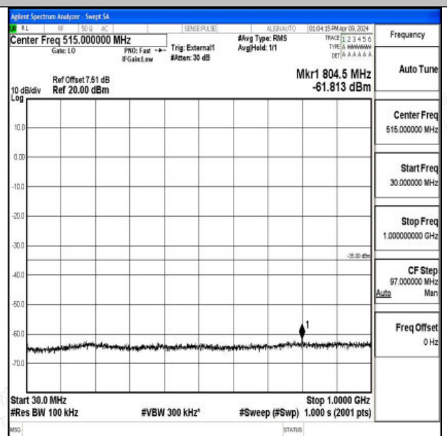
Band41_15MHz_16QAM_39725_1RB#0_30~1000_30~1000
