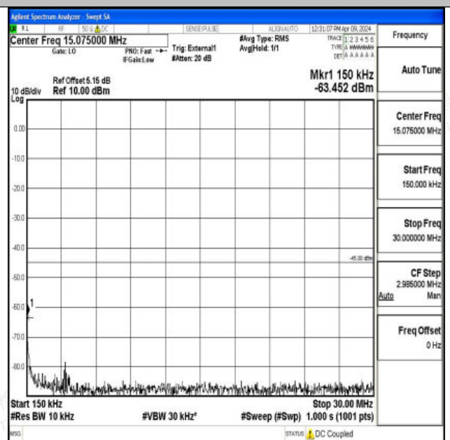
Band41_10MHz_QPSK_39700_1RB#0_0.15~30_0.15~30
