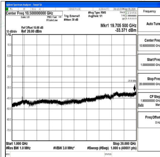
Band41_15MHz_16QAM_41515_1RB#0_1000~20000_10 00~20000
