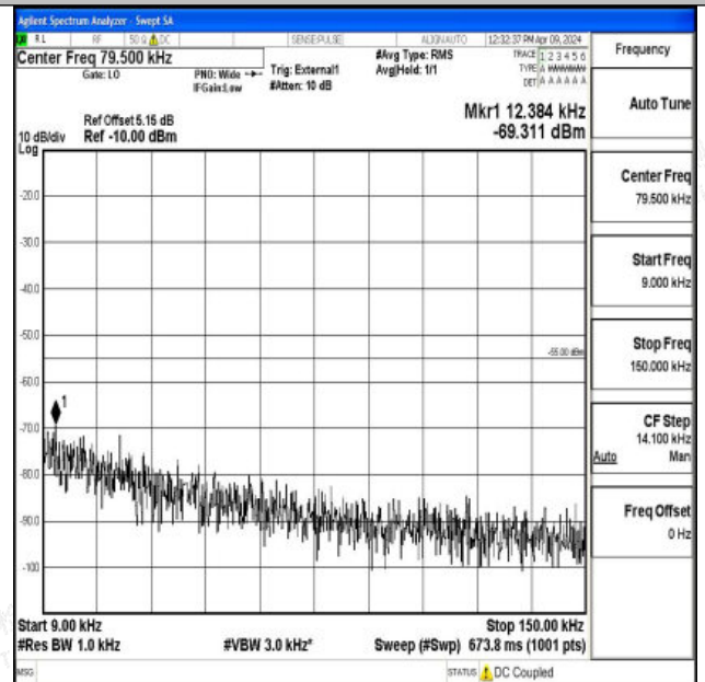
Band41_10MHz_16QAM_39700_1RB#0_0.009~0.15_0.009~0.15
