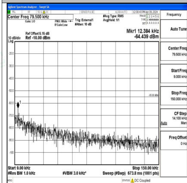
Band41_10MHz_QPSK_39700_1RB#0_0.009~0.15_0.009 ~0.15
