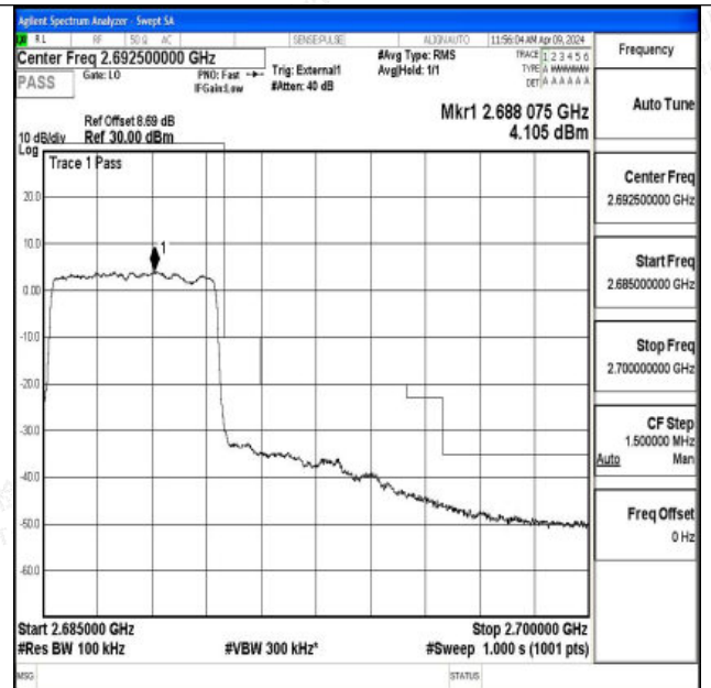
Band41_5MHz_16QAM_41565_25RB#0
