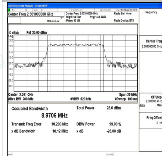
Band41-10MHz-QPSK-39700-50RB#0-PASS
