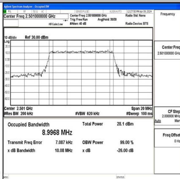
Band41-10MHz-16QAM-39700-50RB#0-PASS
