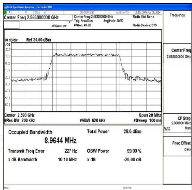
Band41-10MHz-16QAM-40620-50RB#0-PASS
