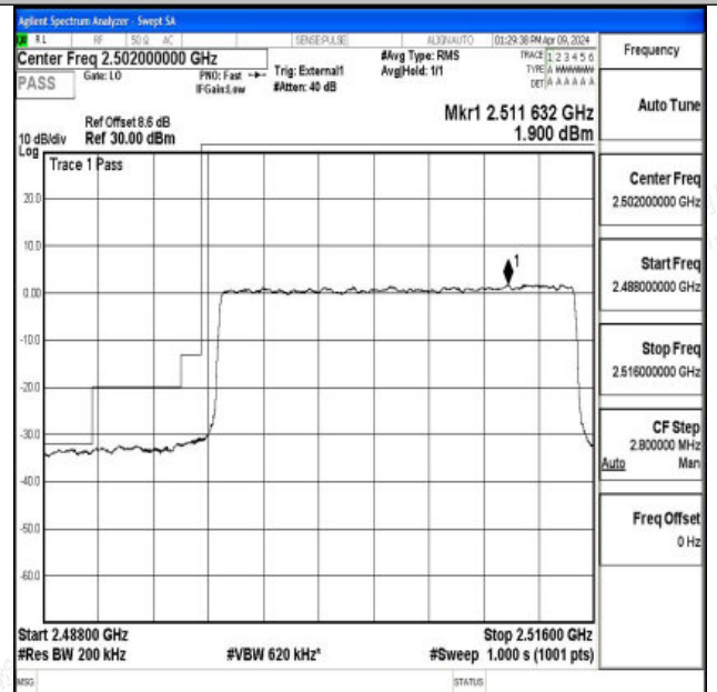
Band41_20MHz_16QAM_39750_100RB#0
