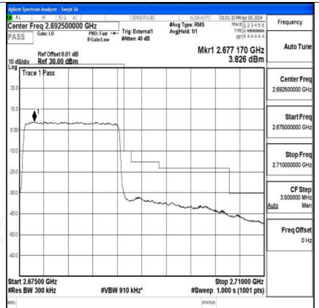
Band41_15MHz_16QAM_41515_75RB#0
