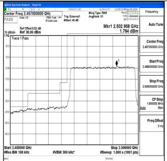
Band41_10MHz_16QAM_39700_50RB#0
