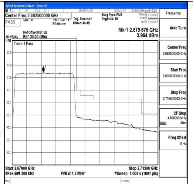
Band41_20MHz_16QAM_41490_100RB#0
