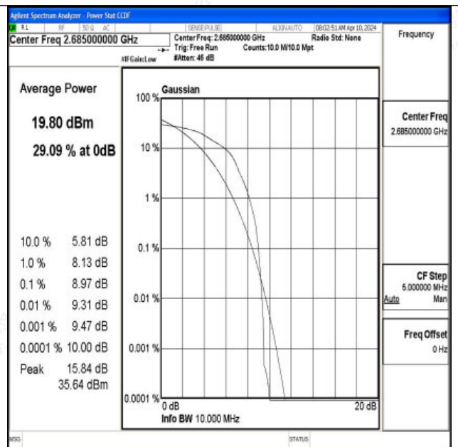
Band41-10MHz-16QAM-41540-1RB#0-PASS
