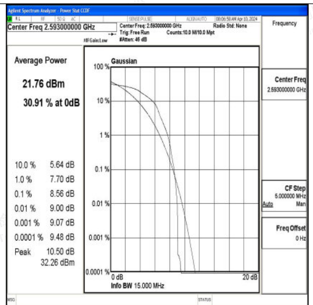
Band41-15MHz-16QAM-40620-1RB#0-PASS
