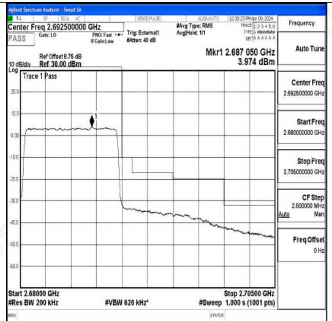
Band41_10MHz_16QAM_41540_50RB#0
