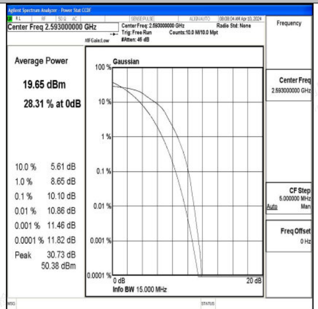
Band41-15MHz-16QAM-40620-75RB#0-PASS
