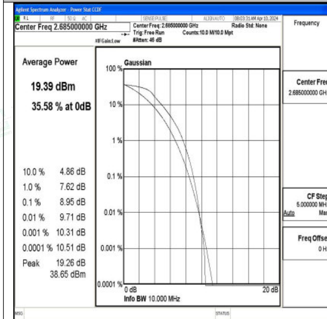
Band41-10MHz-QPSK-41540-50RB#0-PASS
