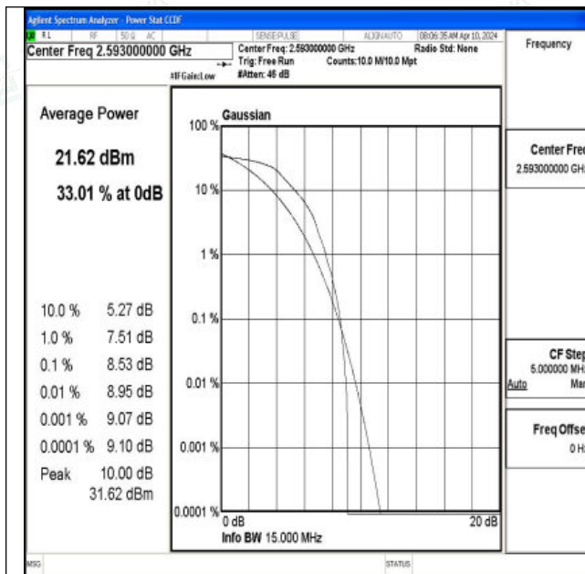
Band41-15MHz-QPSK-40620-1RB#0-PASS
