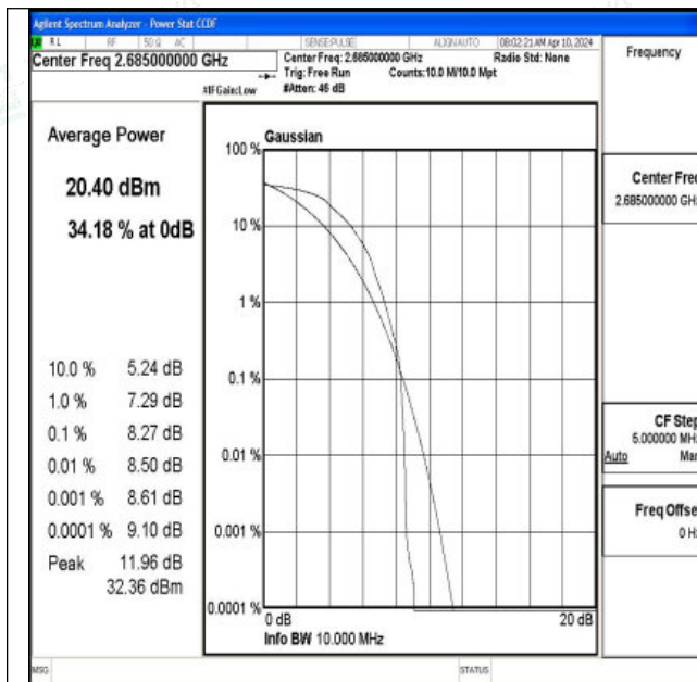
Band41-10MHz-QPSK-41540-1RB#0-PASS
