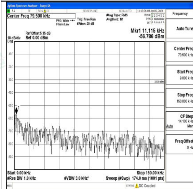
Band26_10MHz_QPSK_26990_1RB#0_0.009~0.15_0.009 ~0.15
