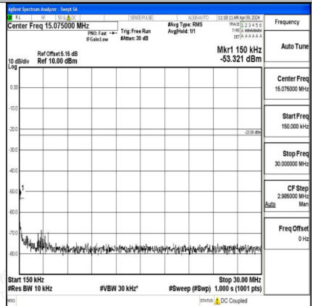
Band26_10MHz_QPSK_26990_1RB#0_0.15~30_0.15~30
