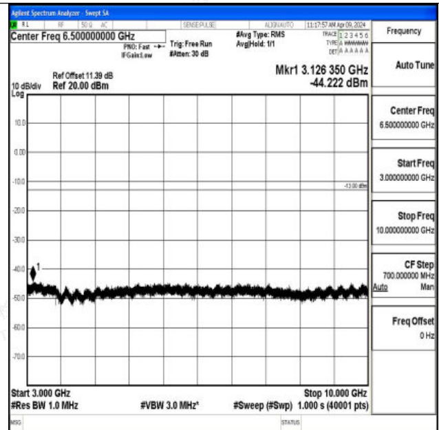
Band26_10MHz_16QAM_26915_1RB#0_3000~10000_300 0~10000
