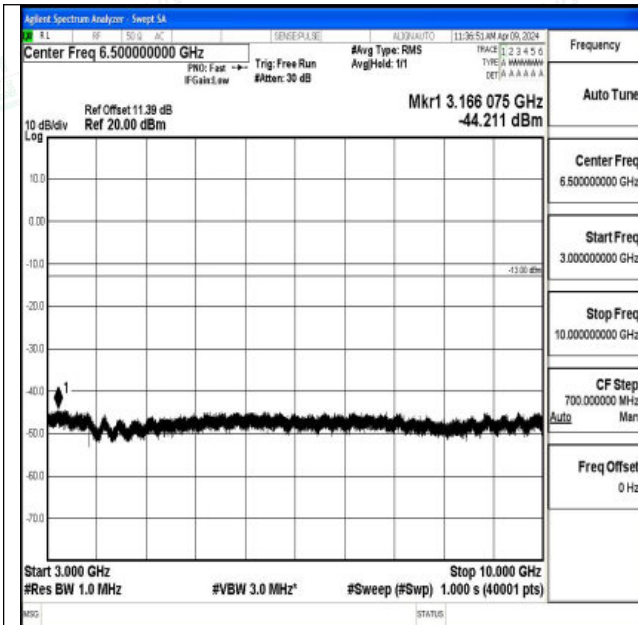
Band26_15MHz_QPSK_26965_1RB#0_3000~10000_300 0~10000
