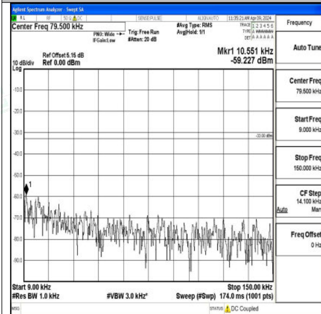
Band26_15MHz_QPSK_26915_1RB#0_0.009~0.15_0.009 ~0.15
