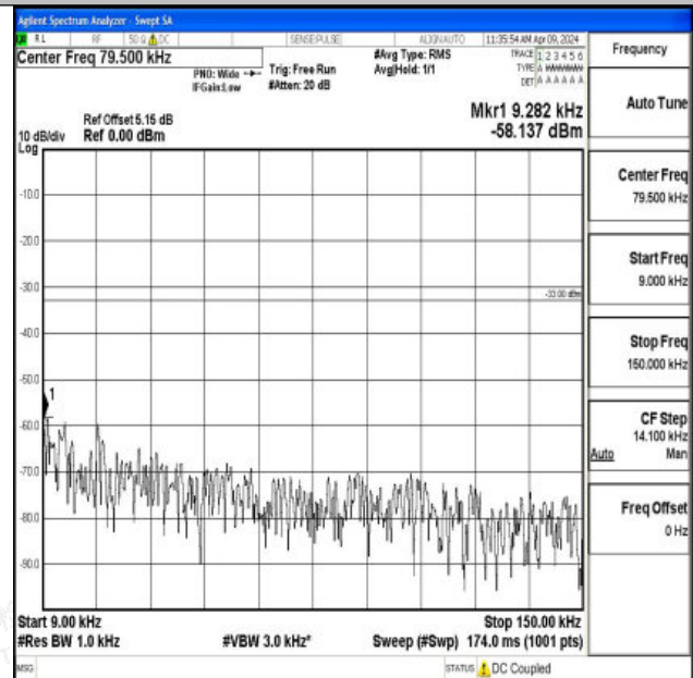
Band26_15MHz_16QAM_26915_1RB#0_0.009~0.15_0.009~0.15
