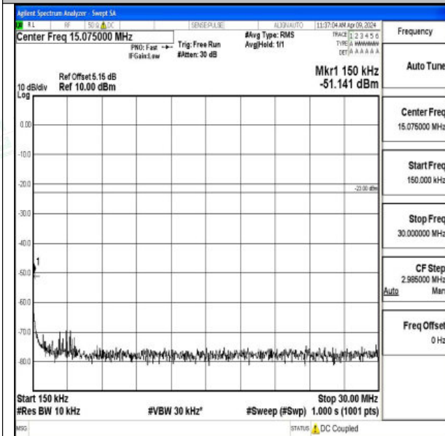
Band26_15MHz_16QAM_26965_1RB#0_0.15~30_0.15~3 0
