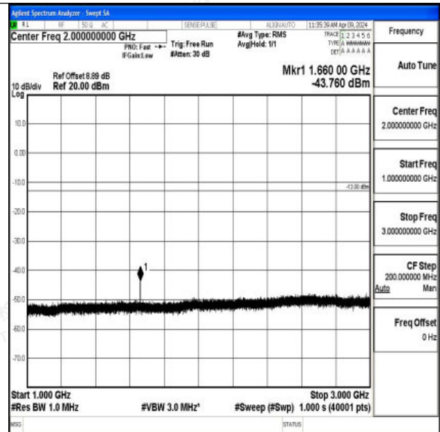
Band26_15MHz_QPSK_26915_1RB#0_1000~3000_1000~3000
