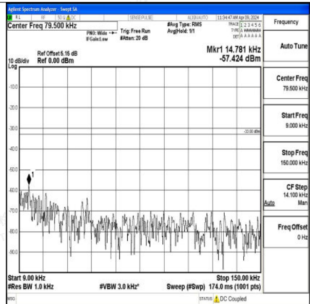
Band26_15MHz_16QAM_26865_1RB#0_0.009~0.15_0.009 ~0.15
