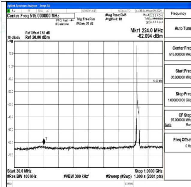
Band26_15MHz_QPSK_26915_1RB#0_30~1000_30~100
