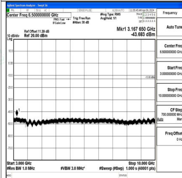
Band26_15MHz_QPSK_26915_1RB#0_3000~10000_3000~10000
