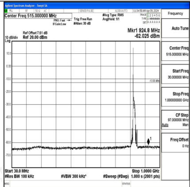
Band26_15MHz_16QAM_26865_1RB#0_30~1000_30~100 0
