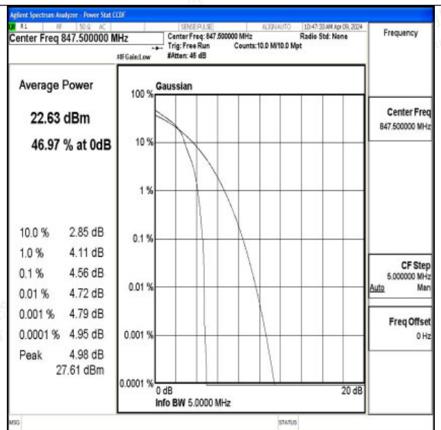
26(824-849)-3MHz-16QAM-27025-1RB#0-PASS
