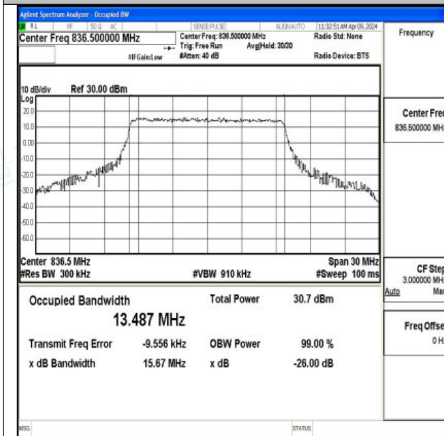
26(824-849)-15MHz-QPSK-26915-75RB#0-PASS
