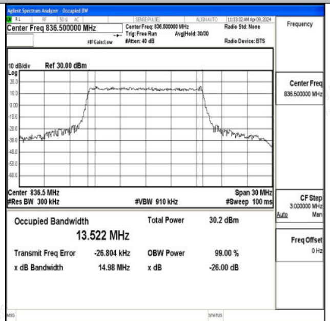
26(824-849)-15MHz-16QAM-26915-75RB#0-PASS
