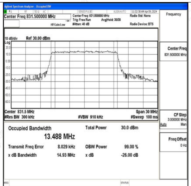
26(824-849)-15MHz-16QAM-26865-75RB#0-PASS
