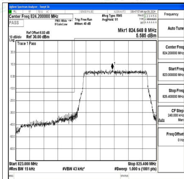
Band26 1.4MHz QPSK 26797 6RB#0
