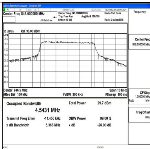
26(824-849)-5MHz-16QAM-27015-25RB#0-PASS
