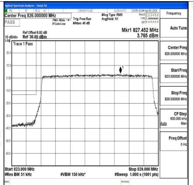
Band26_5MHz_16QAM_26815_25RB#0
