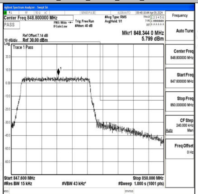
Band26 1.4MHz 16QAM 27033 6RB#0
