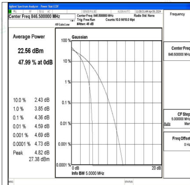
26(824-849)-5MHz-QPSK-27015-1RB#0-PASS
