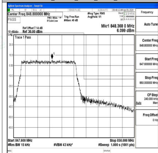
Band26 1.4MHz QPSK 27033 6RB#0
