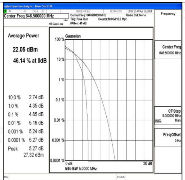
26(824-849)-5MHz-16QAM-27015-1RB#0-PASS
