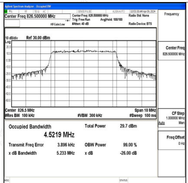
26(824-849)-5MHz-16QAM-26815-25RB#0-PASS
