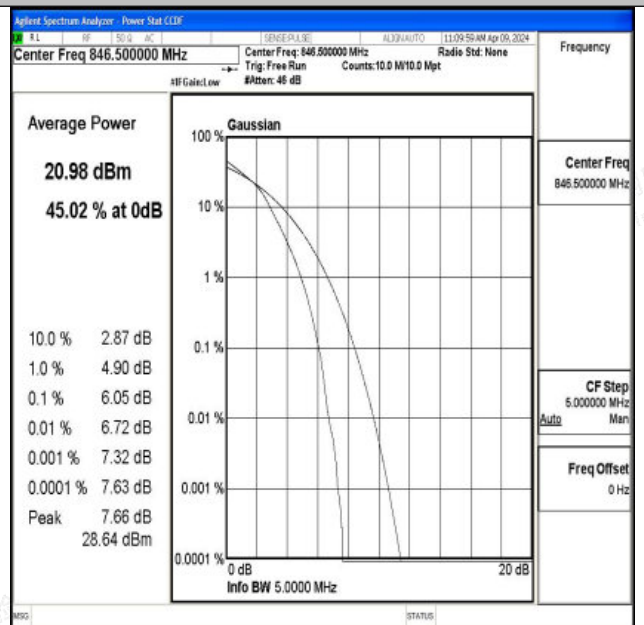
26(824-849)-5MHz-16QAM-27015-25RB#0-PASS
