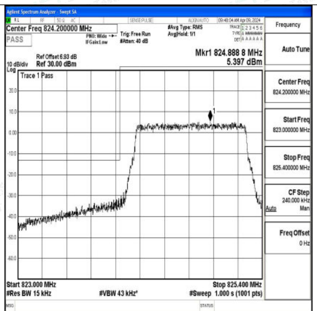
Band26 1.4MHz 16QAM 26797 6RB#0
