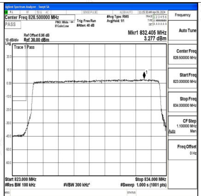
Band26_10MHz_16QAM_26840_50RB#0
