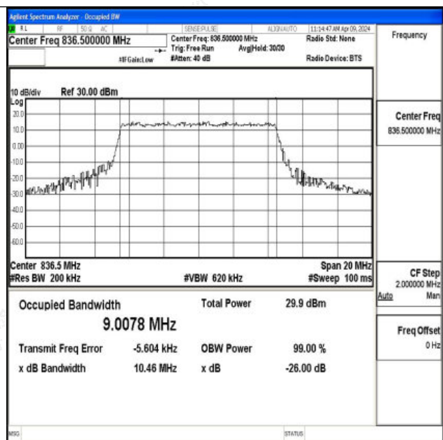
26(824-849)-10MHz-16QAM-26915-50RB#0-PASS
