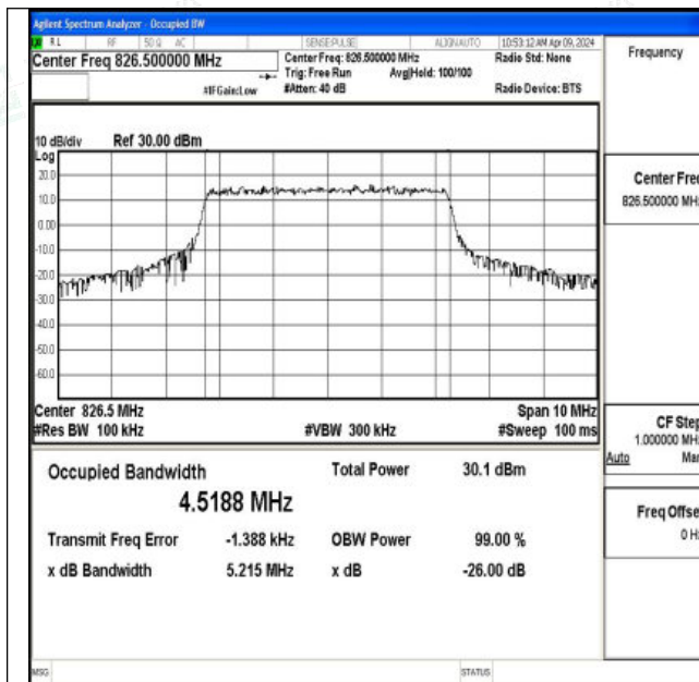
26(824-849)-5MHz-QPSK-26815-25RB#0-PASS
