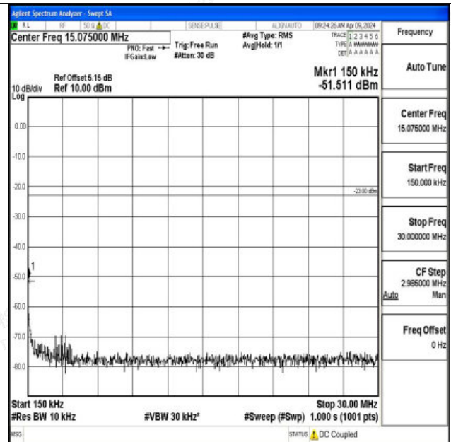
Band26_5MHz_QPSK_26765_1RB#0_0.15~30_0.15~30
