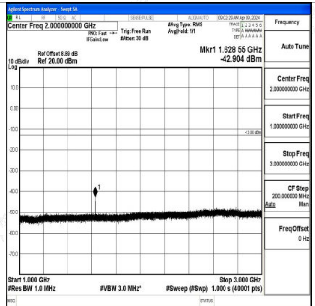
Band26_3MHz_QPSK_26705_1RB#0_1000~3000_1000~3000
