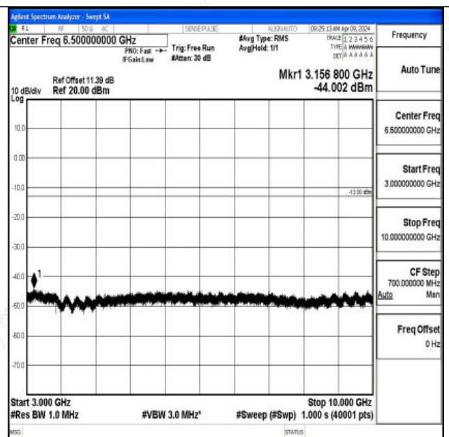
Band26_5MHz_16QAM_26765_1RB#0_3000~10000_3000 ~10000
