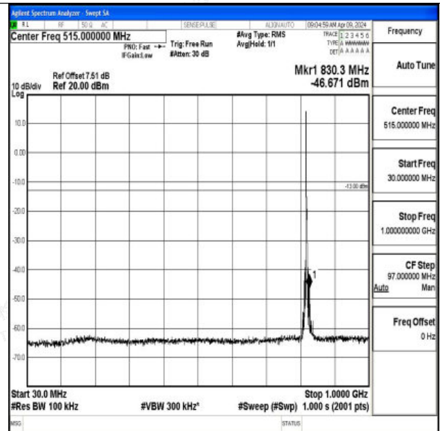
Band26_3MHz_16QAM_26775_1RB#0_30~1000_30~1000
