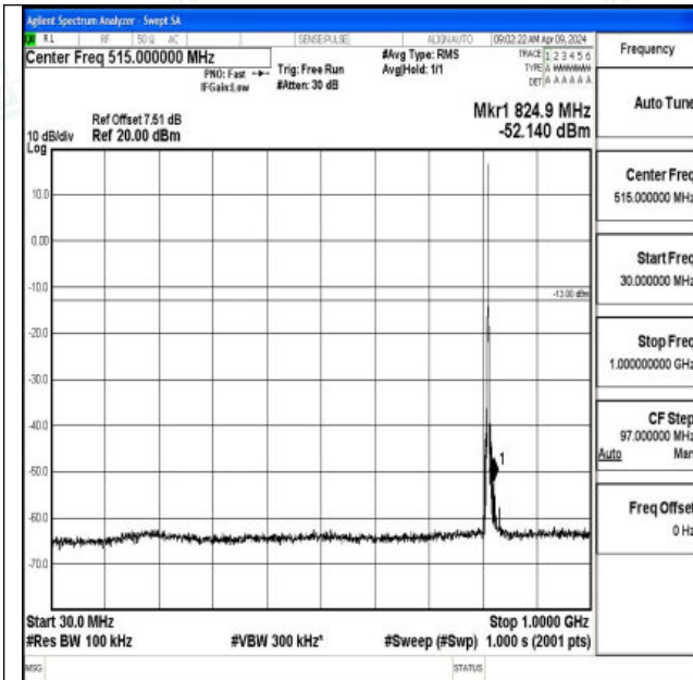
Band26_3MHz_QPSK_26705_1RB#0_30~1000_30~1000
