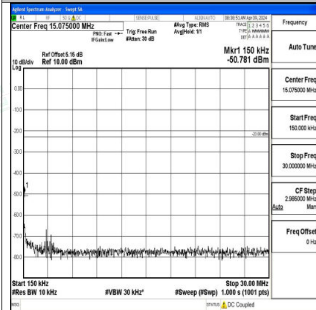
Band26_1.4MHz_16QAM_26783_1RB#0_0.15~30_0.15~3 0
