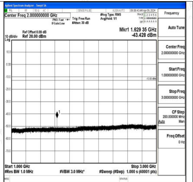
Band26_10MHz_QPSK_26740_1RB#0_1000~3000_1000~3000
