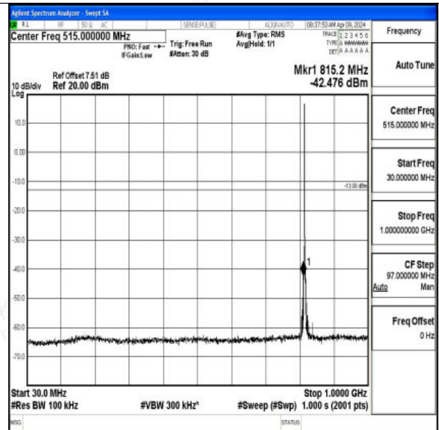
Band26_1.4MHz_16QAM_26740_1RB#0_30~1000_30~10
