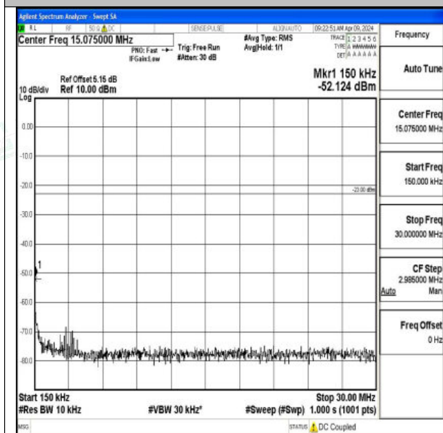
Band26_5MHz_16QAM_26715_1RB#0_0.15~30_0.15~30
