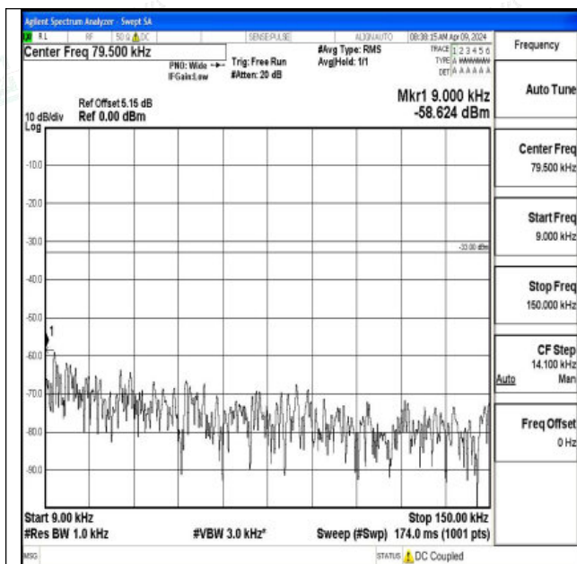
Band26_1.4MHz_QPSK_26783_1RB#0_0.009~0.15_0.00 9~0.15
