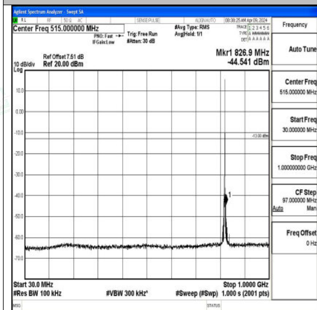
Band26_1.4MHz_QPSK_26783_1RB#0_30~1000_30~100 0
