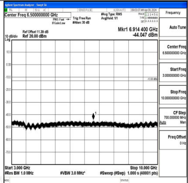
Band26_3MHz_16QAM_26705_1RB#0_3000~10000_3000 ~10000
