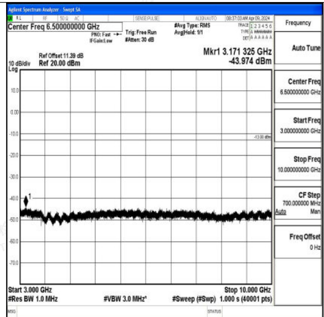
Band26_1.4MHz_16QAM_26697_1RB#0_3000~10000_300 0~10000
