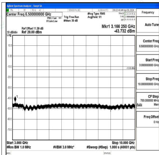
Band26_5MHz_QPSK_26715_1RB#0_3000~10000_3000~10000
