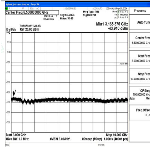
Band26_3MHz_QPSK_26775_1RB#0_3000~10000_3000~10000
