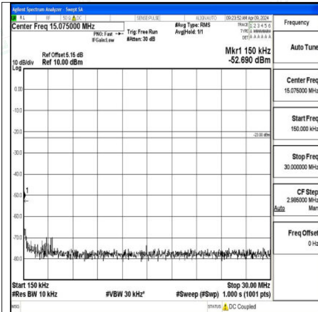
Band26_5MHz_16QAM_26740_1RB#0_0.15~30_0.15~30
