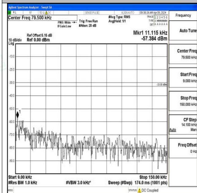
Band26_10MHz_QPSK_26740_1RB#0_0.009~0.15_0.009 ~0.15
