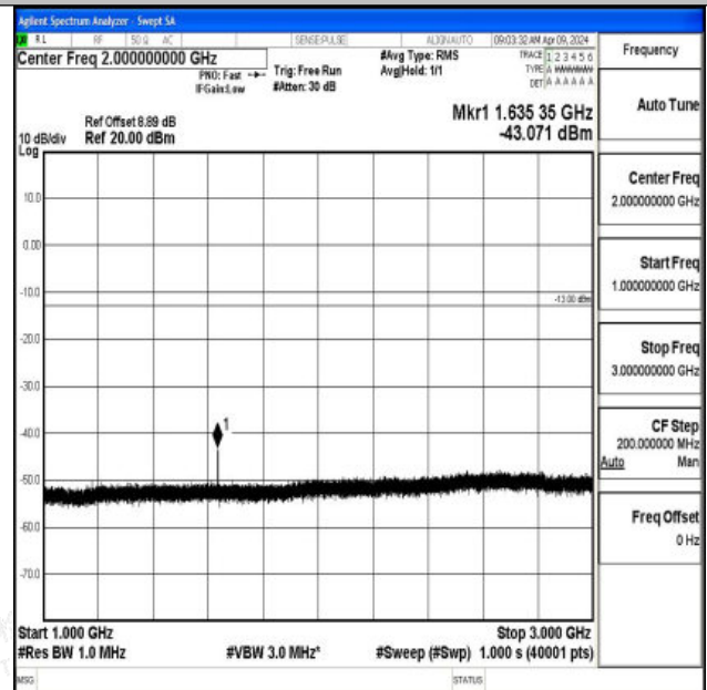
Band26_3MHz_QPSK_26740_1RB#0_1000~3000_1000~3000
