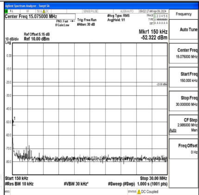
Band26_3MHz_QPSK_26705_1RB#0_0.15~30_0.15~30
