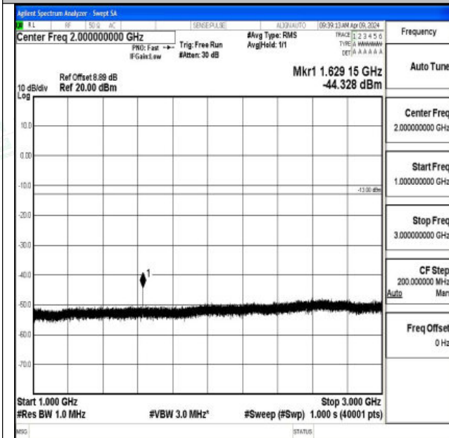
Band26_10MHz_16QAM_26740_1RB#0_1000~3000_100
