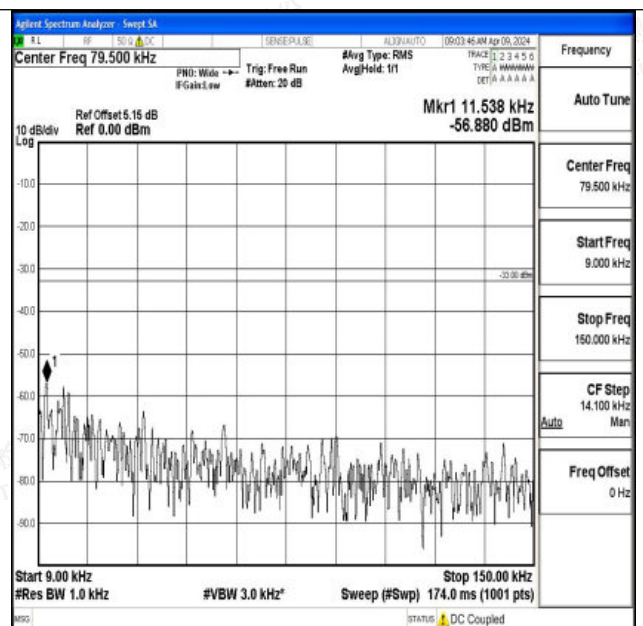
Band26_3MHz_16QAM_26740_1RB#0_0.009~0.15_0.009~0.15
