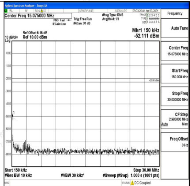
Band26_3MHz_QPSK_26740_1RB#0_0.15~30_0.15~30
