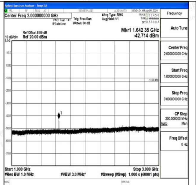
Band26_3MHz_QPSK_26775_1RB#0_1000~3000_1000~3000
