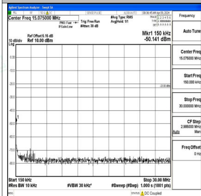
Band26_1.4MHz_16QAM_26697_1RB#0_0.15~30_0.15~3 0
