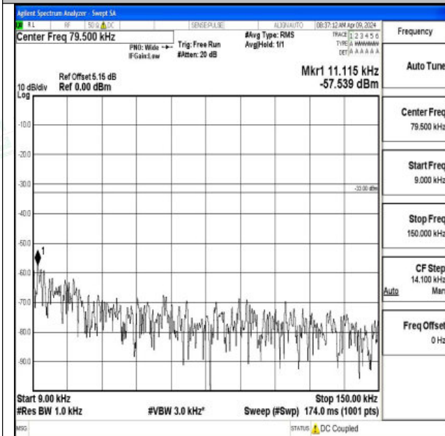
Band26_1.4MHz_QPSK_26740_1RB#0_0.009~0.15_0.00 9~0.15
