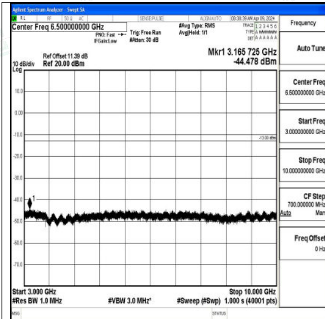
Band26_1.4MHz_QPSK_26783_1RB#0_3000~10000_300 0~10000
