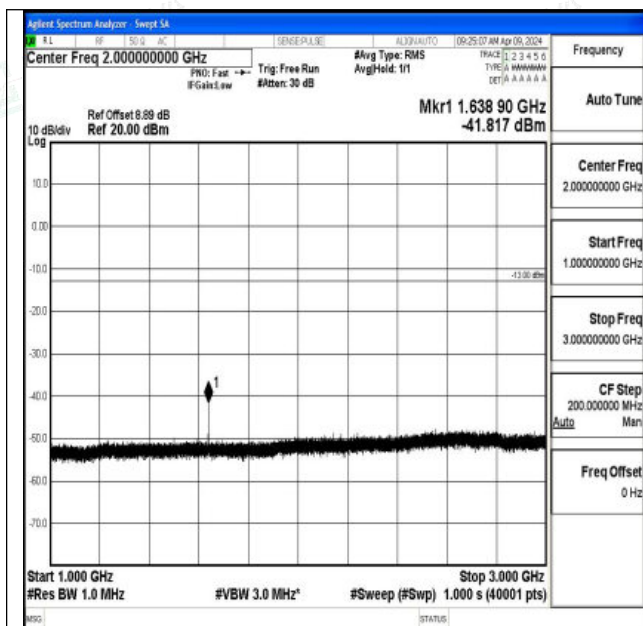
Band26_5MHz_16QAM_26765_1RB#0_1000~3000_1000 ~3000
