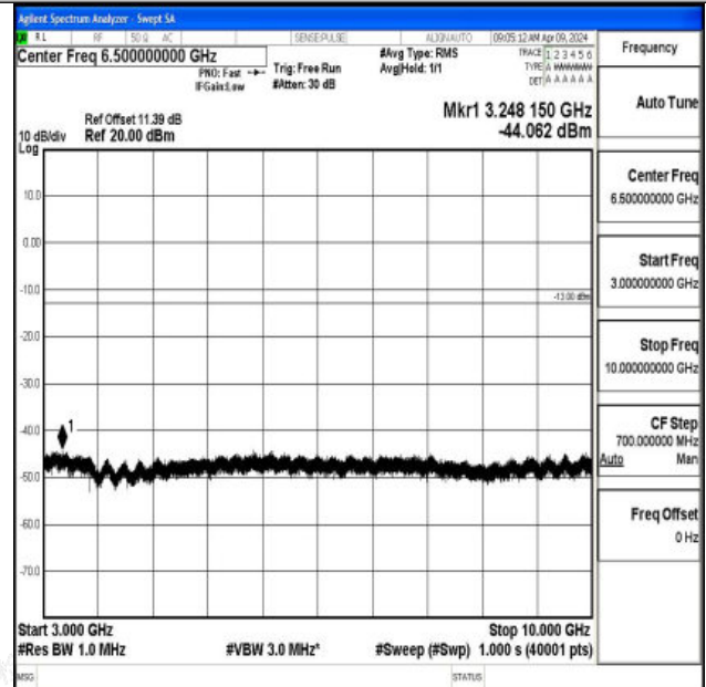
Band26_3MHz_16QAM_26775_1RB#0_3000~10000_3000 ~10000
