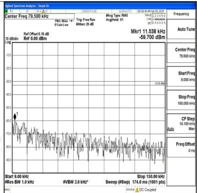
Band26_1.4MHz_16QAM_26783_1RB#0_0.009~0.15_0.00 9~0.15
