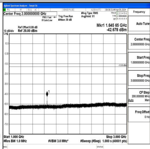
Band26_1.4MHz_QPSK_26783_1RB#0_1000~3000_1000~ 3000
