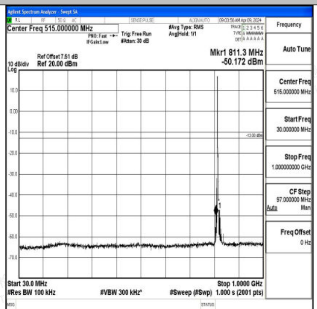
Band26_3MHz_16QAM_26740_1RB#0_30~1000_30~1000
