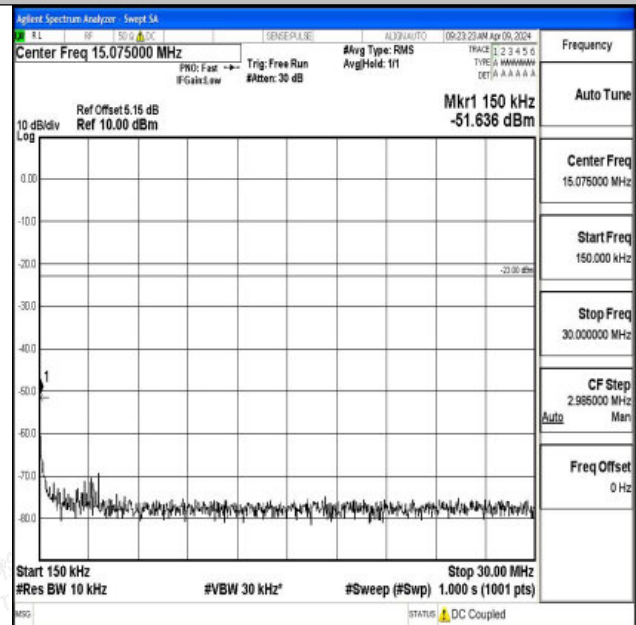
Band26_5MHz_QPSK_26740_1RB#0_0.15~30_0.15~30
