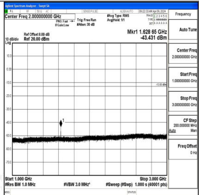
Band26_5MHz_QPSK_26715_1RB#0_1000~3000_1000~3000
