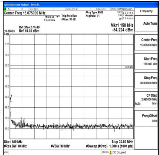
Band26_5MHz_QPSK_26715_1RB#0_0.15~30_0.15~30
