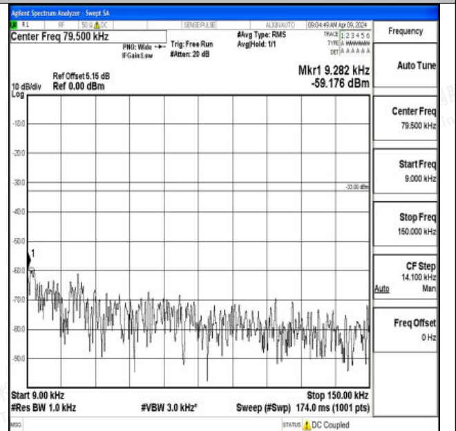
Band26_3MHz_16QAM_26775_1RB#0_0.009~0.15_0.009~0.15
