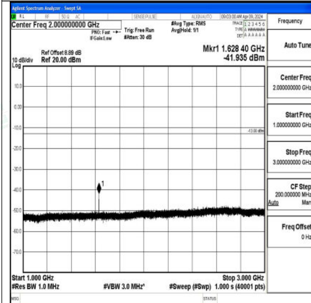
Band26_3MHz_16QAM_26705_1RB#0_1000~3000_1000 ~3000
