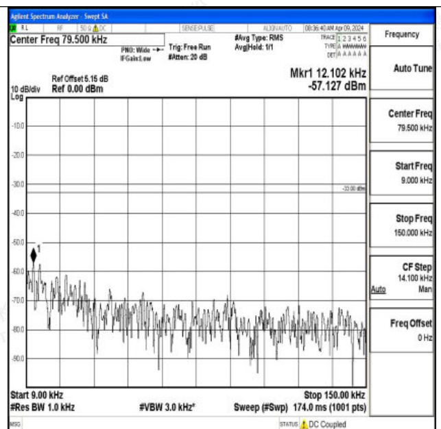
Band26_1.4MHz_16QAM_26697_1RB#0_0.009~0.15_0.00 9~0.15
