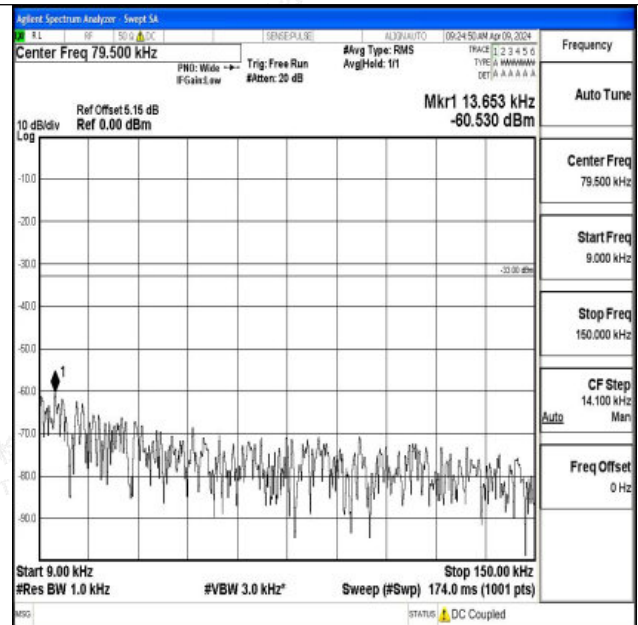
Band26_5MHz_16QAM_26765_1RB#0_0.009~0.15_0.009~0.15
