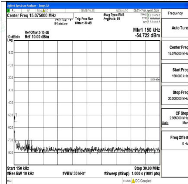
Band26_1.4MHz_16QAM_26740_1RB#0_0.15~30_0.15~3
