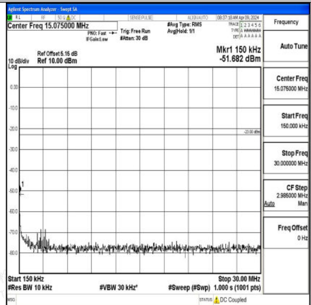
Band26_1.4MHz_QPSK_26740_1RB#0_0.15~30_0.15~30
