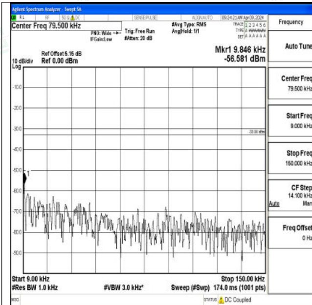
Band26_5MHz_QPSK_26765_1RB#0_0.009~0.15_0.009~0.15
