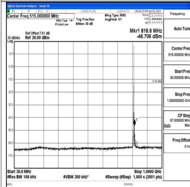
Band26_1.4MHz_QPSK_26697_1RB#0_30~1000_30~100 0
