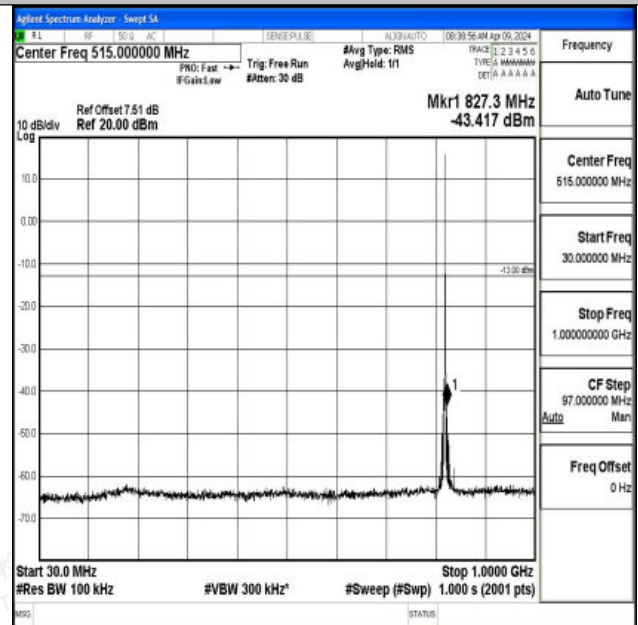
Band26_1.4MHz_16QAM_26783_1RB#0_30~1000_30~10 00
