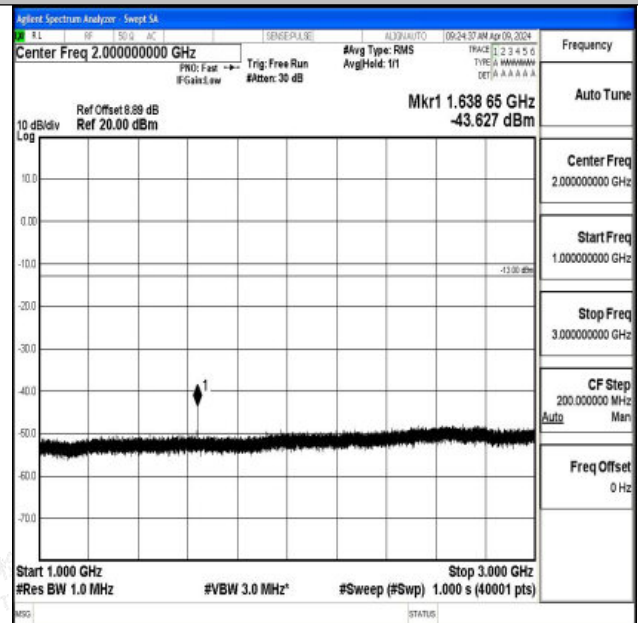
Band26_5MHz_QPSK_26765_1RB#0_1000~3000_1000~3000
