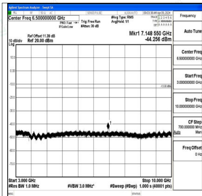
Band26_3MHz_QPSK_26740_1RB#0_3000~10000_3000~10000
