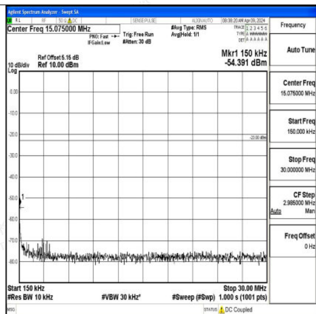
Band26_1.4MHz_QPSK_26783_1RB#0_0.15~30_0.15~30
