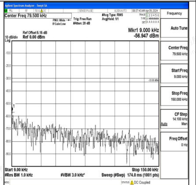
Band26_1.4MHz_16QAM_26740_1RB#0_0.009~0.15_0.009~0.15
