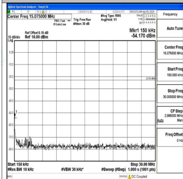
Band26_3MHz_16QAM_26740_1RB#0_0.15~30_0.15~30
