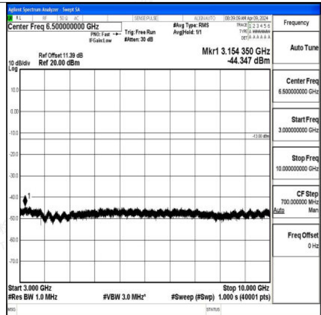
Band26_1.4MHz_16QAM_26783_1RB#0_3000~10000_300 0~10000
