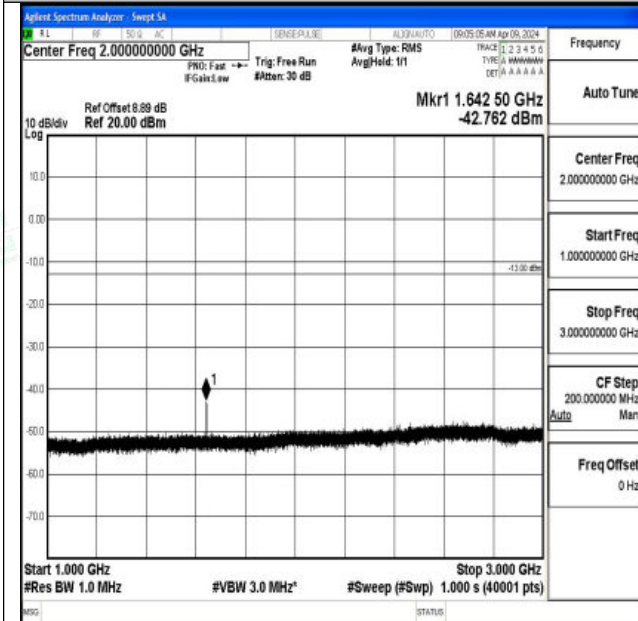
Band26_3MHz_16QAM_26775_1RB#0_1000~3000_1000 ~3000
