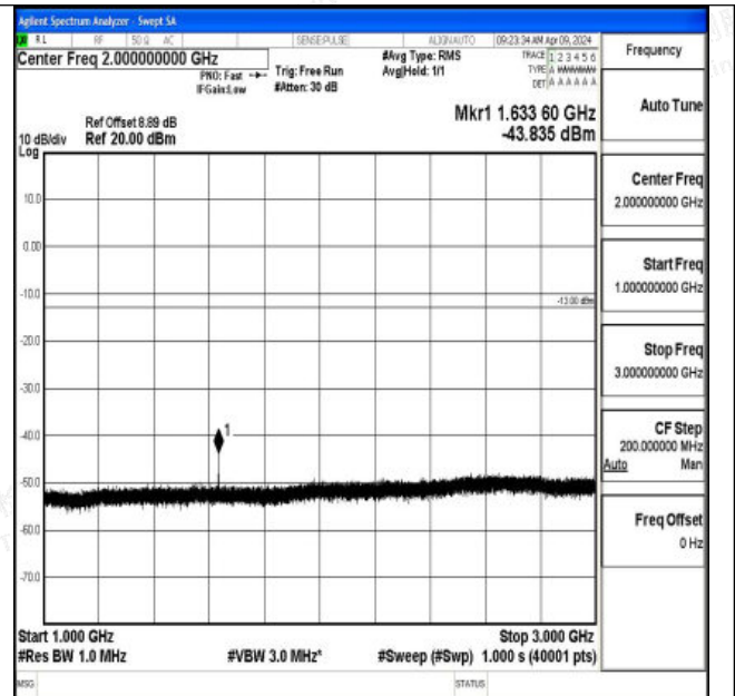
Band26_5MHz_QPSK_26740_1RB#0_1000~3000_1000~3000
