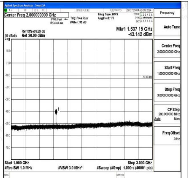
Band26_1.4MHz_QPSK_26740_1RB#0_1000~3000_1000~3000
