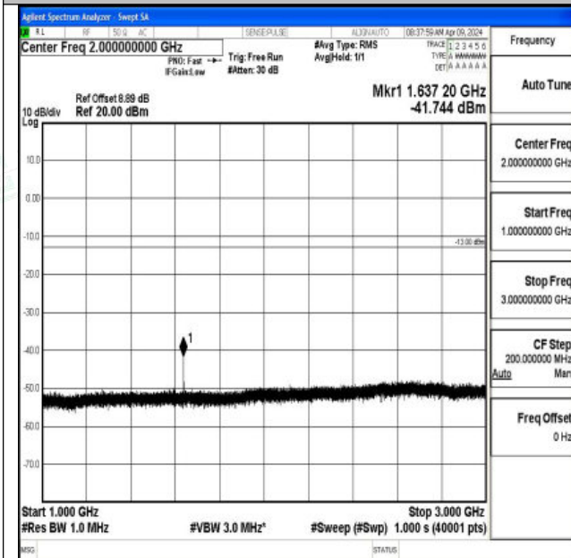
Band26_1.4MHz_16QAM_26740_1RB#0_1000~3000_100
