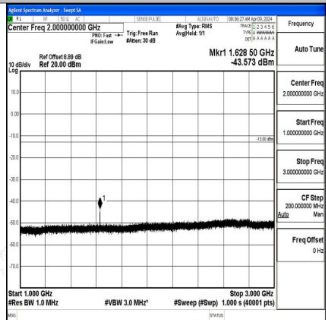
Band26_1.4MHz_QPSK_26697_1RB#0_1000~3000_1000~ 3000
