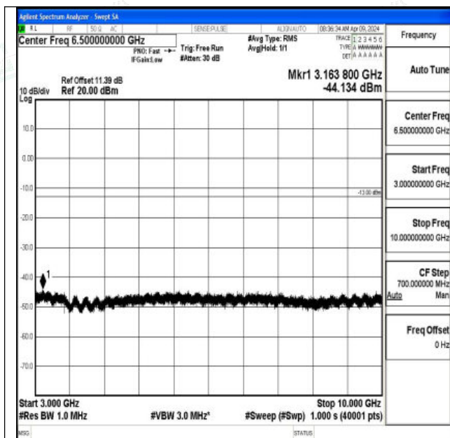
Band26_1.4MHz_QPSK_26697_1RB#0_3000~10000_300 0~10000
