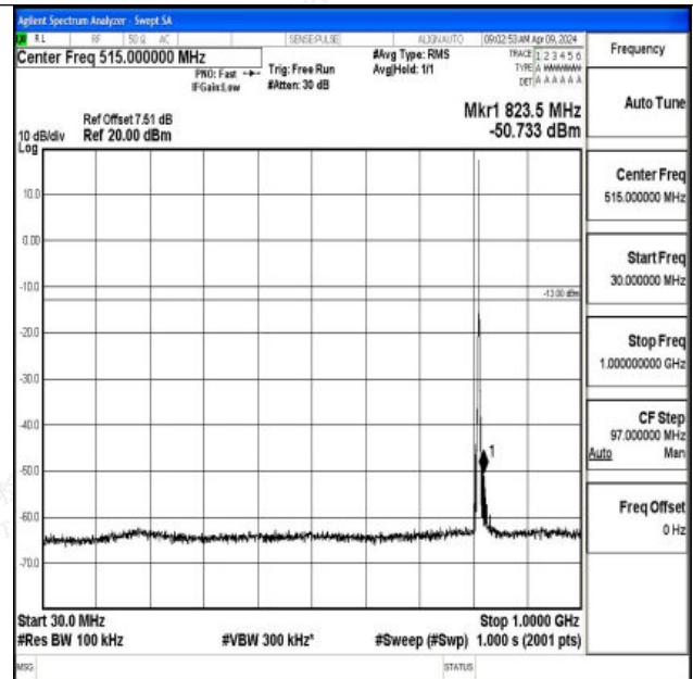
Band26_3MHz_16QAM_26705_1RB#0_30~1000_30~1000
