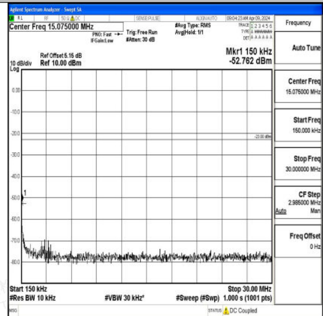
Band26_3MHz_QPSK_26775_1RB#0_0.15~30_0.15~30
