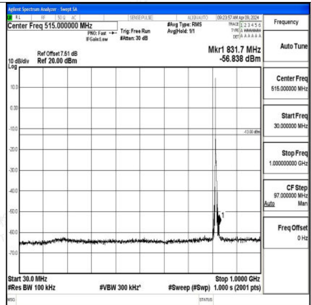
Band26_5MHz_16QAM_26740_1RB#0_30~1000_30~1000
