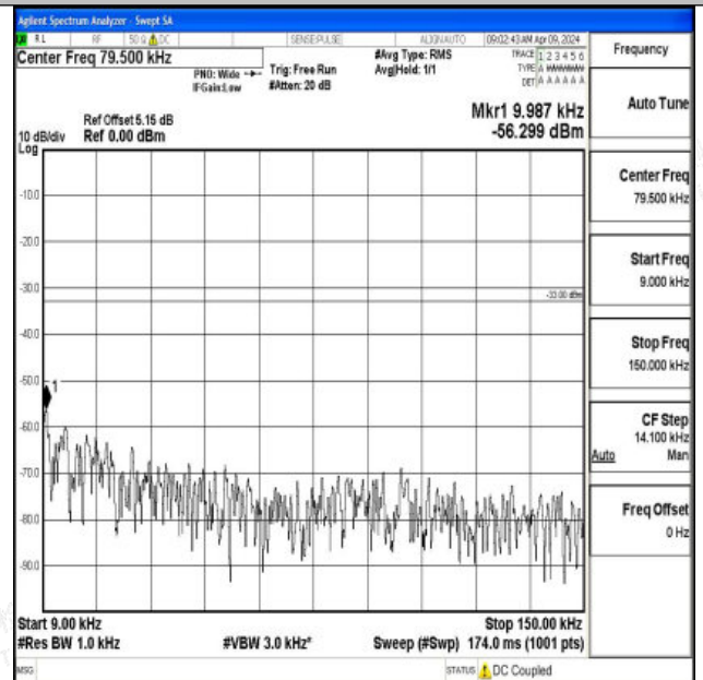
Band26_3MHz_16QAM_26705_1RB#0_0.009~0.15_0.009~0.15
