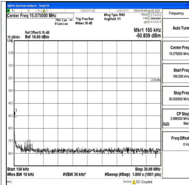
Band26_3MHz_16QAM_26775_1RB#0_0.15~30_0.15~30
