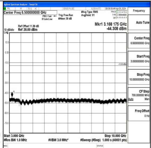
Band26_1.4MHz_16QAM_26740_1RB#0_3000~10000_300
