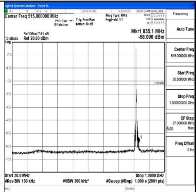
Band26_5MHz_16QAM_26765_1RB#0_30~1000_30~1000
