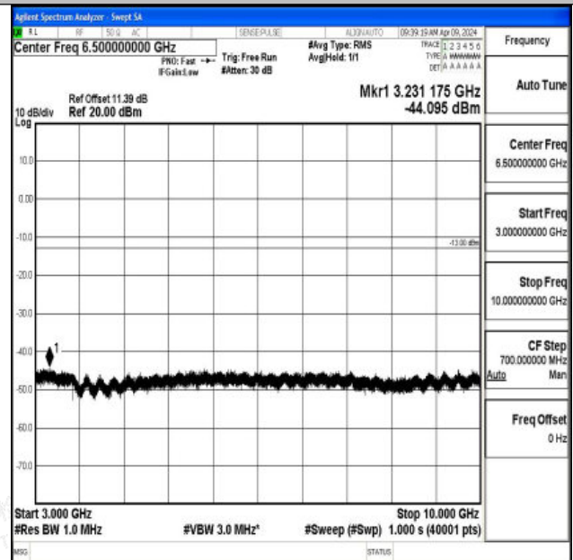
Band26_10MHz_16QAM_26740_1RB#0_3000~10000_300
