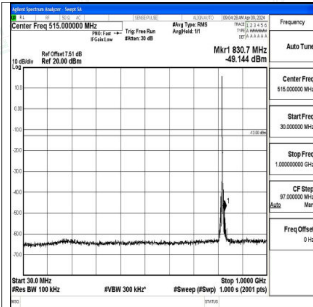
Band26_3MHz_QPSK_26775_1RB#0_30~1000_30~1000
