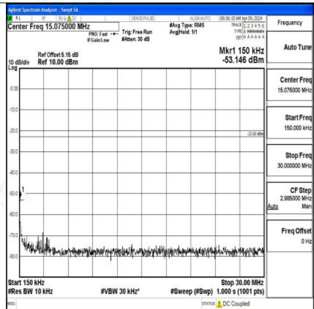
Band26_1.4MHz_QPSK_26697_1RB#0_0.15~30_0.15~30
