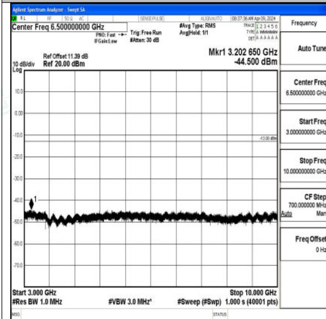
Band26_1.4MHz_QPSK_26740_1RB#0_3000~10000_3000~10000
