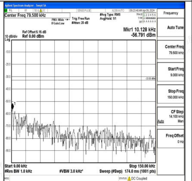
Band26_5MHz_16QAM_26740_1RB#0_0.009~0.15_0.009~0.15
