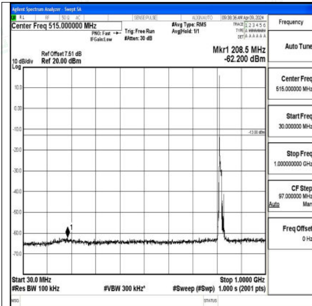
Band26_10MHz_QPSK_26740_1RB#0_30~1000_30~100
