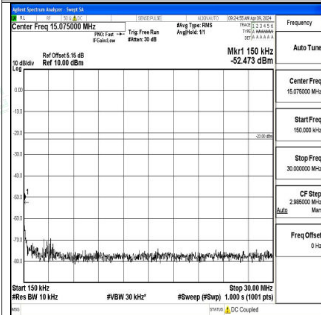
Band26_5MHz_16QAM_26765_1RB#0_0.15~30_0.15~30
