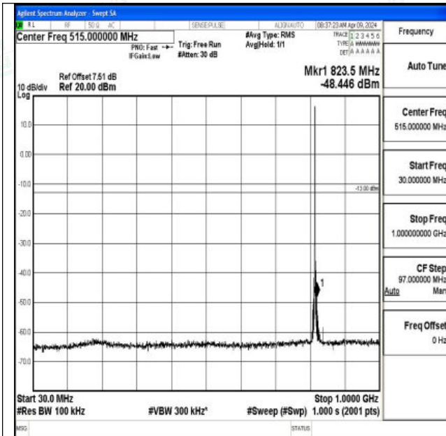
Band26_1.4MHz_QPSK_26740_1RB#0_30~1000_30~100
