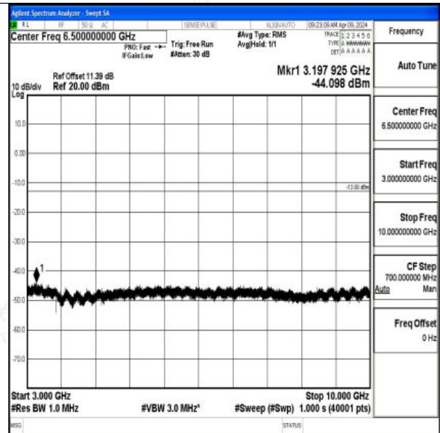
Band26_5MHz_16QAM_26715_1RB#0_3000~10000_3000 ~10000
