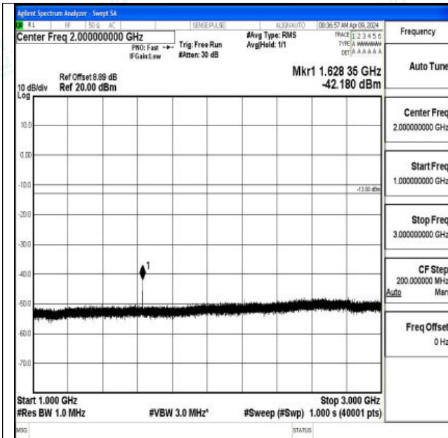
Band26_1.4MHz_16QAM_26697_1RB#0_1000~3000_100 0~3000
