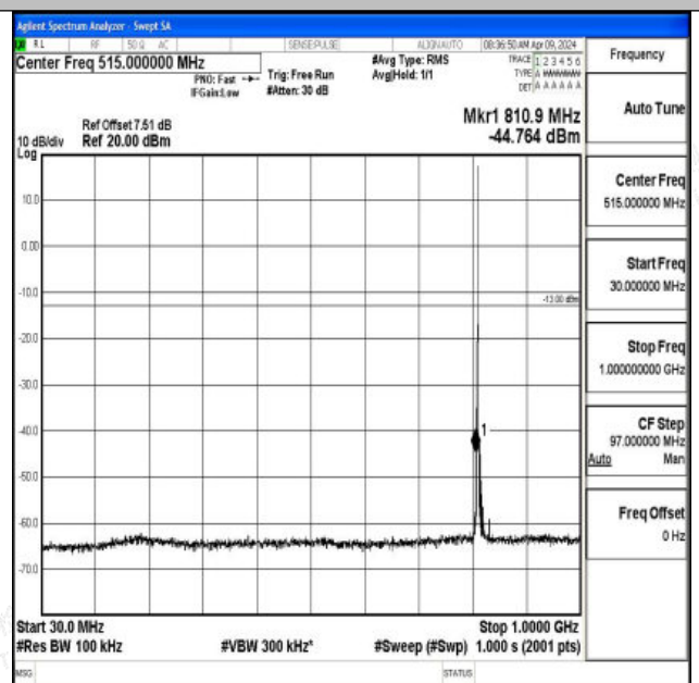
Band26_1.4MHz_16QAM_26697_1RB#0_30~1000_30~10 00
