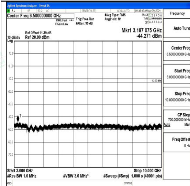
Band26_10MHz_QPSK_26740_1RB#0_3000~10000_3000~10000
