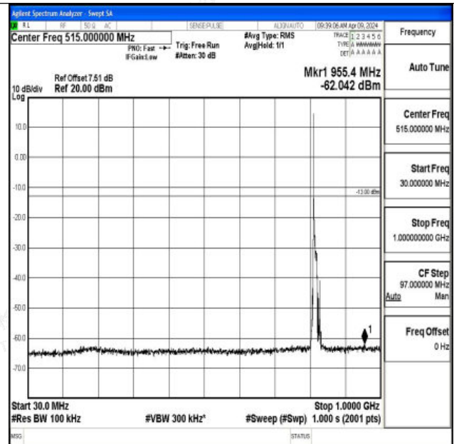
Band26_10MHz_16QAM_26740_1RB#0_30~1000_30~100
