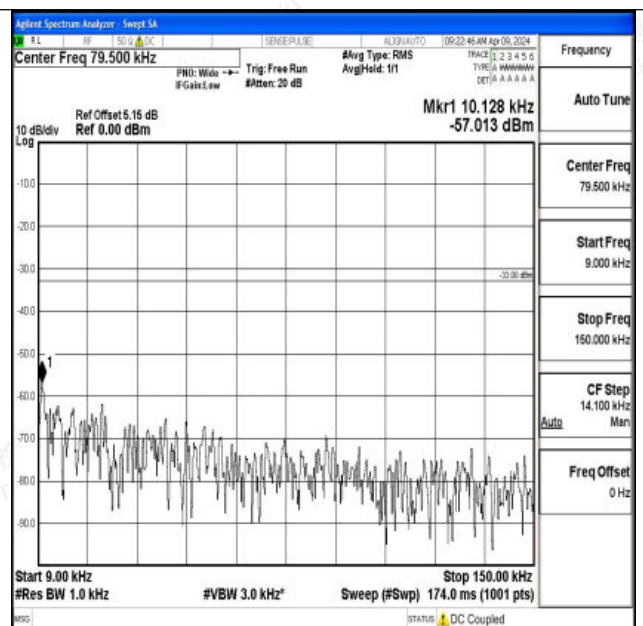
Band26_5MHz_16QAM_26715_1RB#0_0.009~0.15_0.009~0.15
