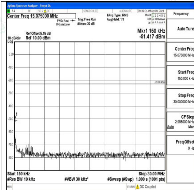
Band26_10MHz_16QAM_26740_1RB#0_0.15~30_0.15~3
