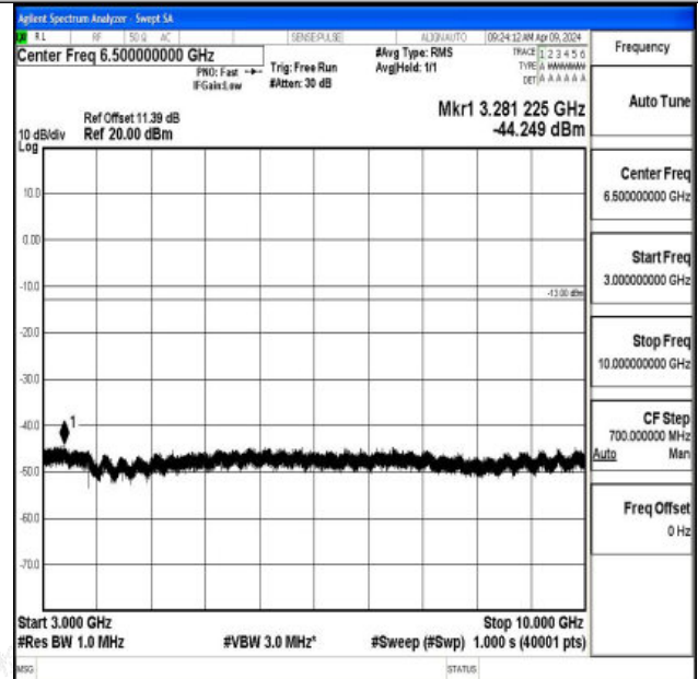
Band26_5MHz_16QAM_26740_1RB#0_3000~10000_3000~10000
