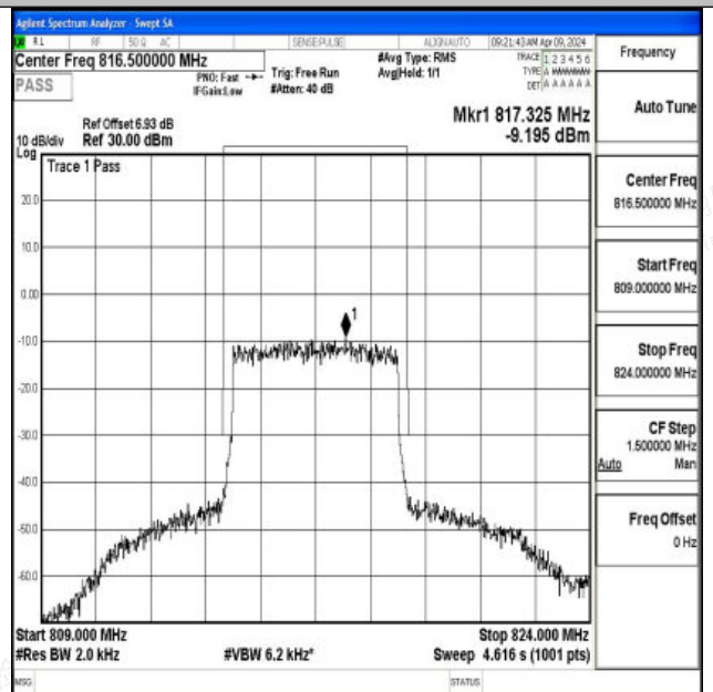
Band26_5MHz_16QAM_26715_25RB#0
