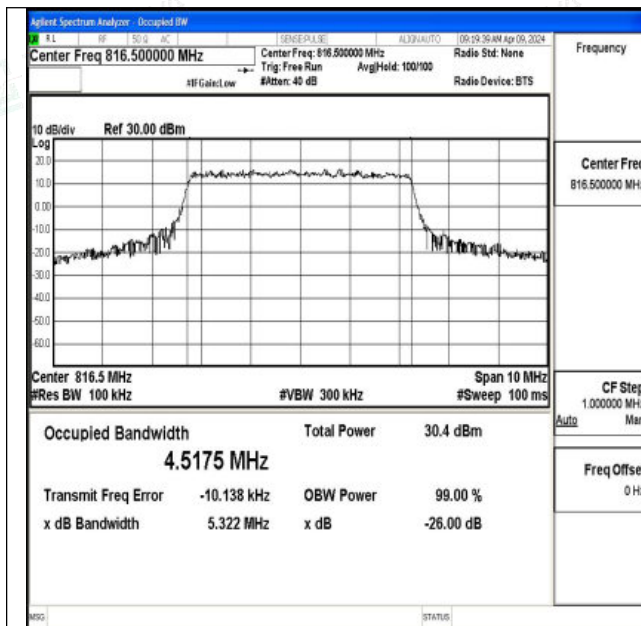
26(814-824)-5MHz-QPSK-26715-25RB#0-PASS
