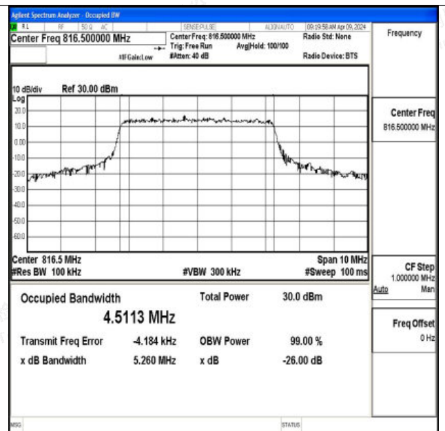
26(814-824)-5MHz-16QAM-26715-25RB#0-PASS
