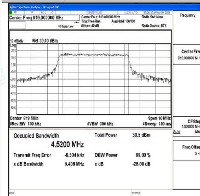
26(814-824)-5MHz-QPSK-26740-25RB#0-PASS
