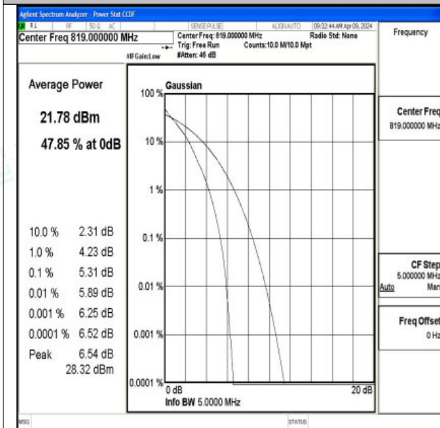
26(814-824)-5MHz-QPSK-26740-25RB#0-PASS
