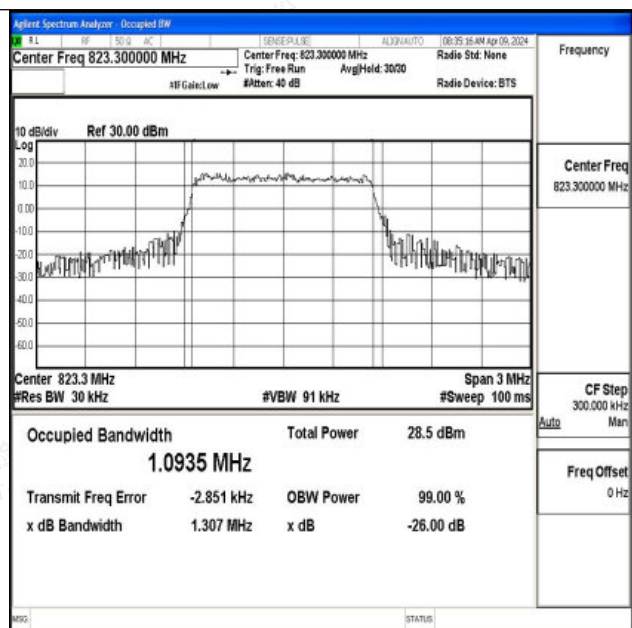
26(814-824)-1.4MHz-16QAM-26783-6RB#0-PASS
