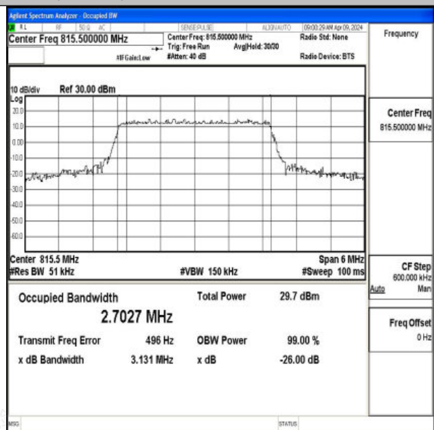
26(814-824)-3MHz-16QAM-26705-15RB#0-PASS
