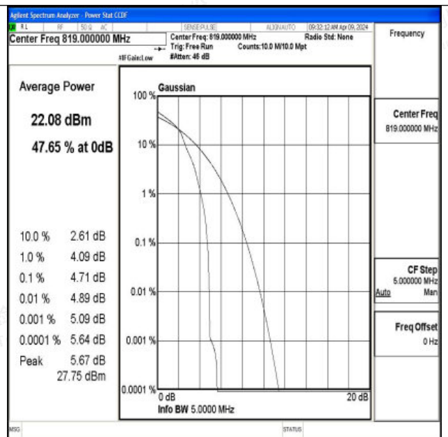
26(814-824)-5MHz-16QAM-26740-1RB#0-PASS
