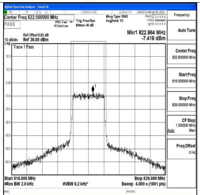
Band26_3MHz_16QAM_26775_15RB#0
