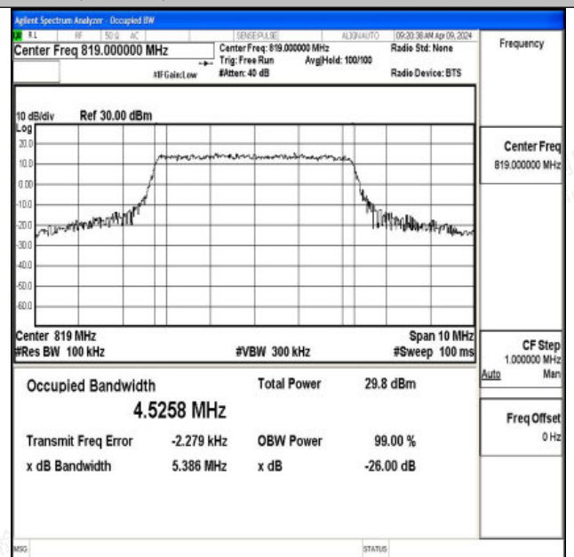
26(814-824)-5MHz-16QAM-26740-25RB#0-PASS
