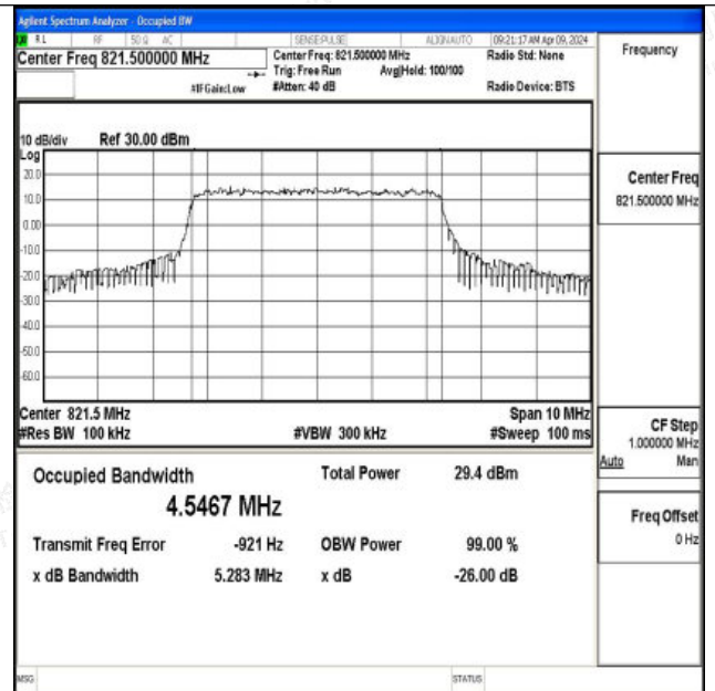
26(814-824)-5MHz-16QAM-26765-25RB#0-PASS
