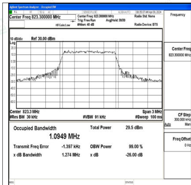
26(814-824)-1.4MHz-QPSK-26783-6RB#0-PASS
