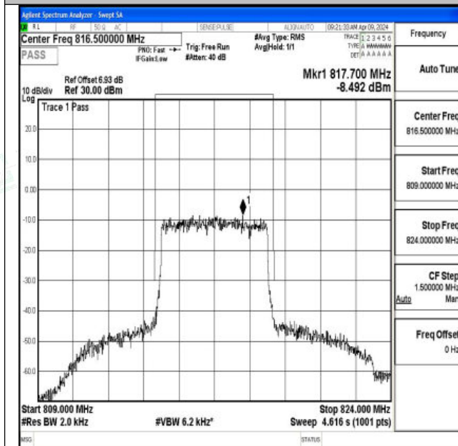
Band26_5MHz_QPSK_26715_25RB#0
