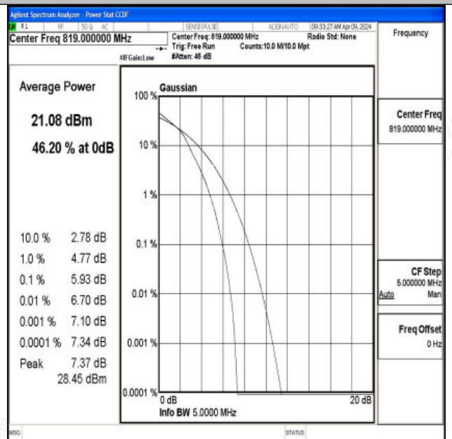
26(814-824)-5MHz-16QAM-26740-25RB#0-PASS
