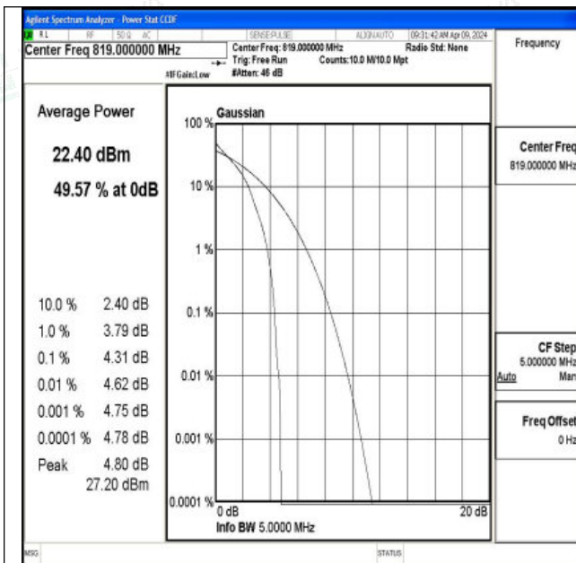
26(814-824)-5MHz-QPSK-26740-1RB#0-PASS
