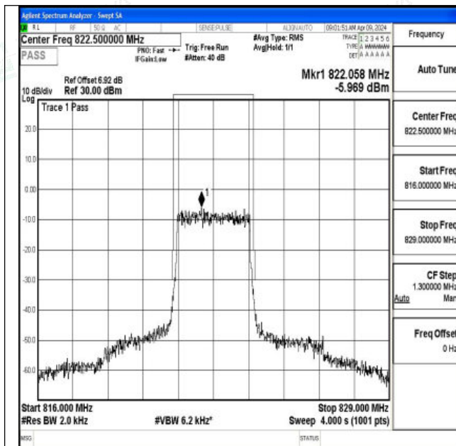
Band26_3MHz_QPSK_26775_15RB#0
