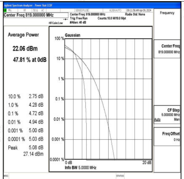
26(814-824)-3MHz-16QAM-26740-1RB#0-PASS
