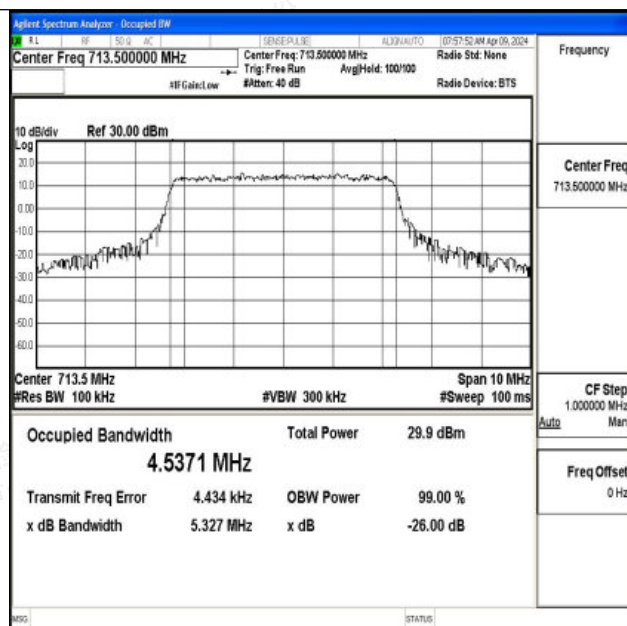
Band17-5MHz-16QAM-23825-25RB#0-PASS
