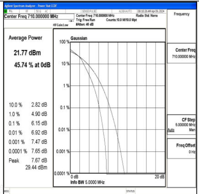
Band17-5MHz-16QAM-23790-25RB#0-PASS
