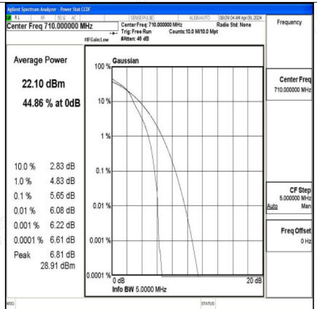
Band17-5MHz-16QAM-23790-1RB#0-PASS
