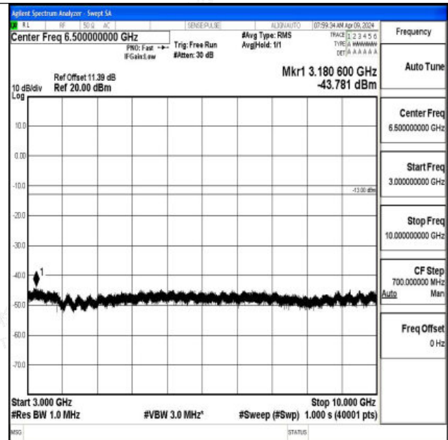
Band17_5MHz_16QAM_23755_1RB#0_3000~10000_3000 ~10000
