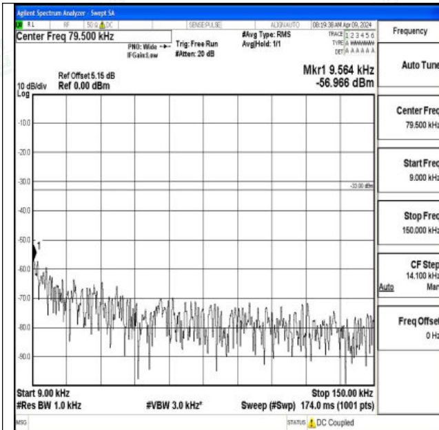
Band17_10MHz_QPSK_23790_1RB#0_0.009~0.15_0.009 ~0.15
