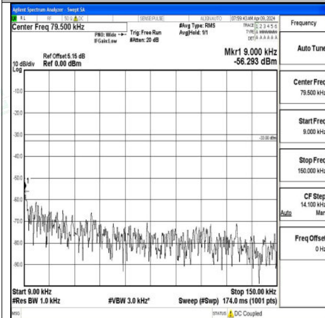
Band17_5MHz_QPSK_23790_1RB#0_0.009~0.15_0.009~ 0.15
