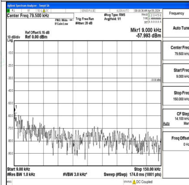
Band17_10MHz_QPSK_23780_1RB#0_0.009~0.15_0.009 ~0.15
