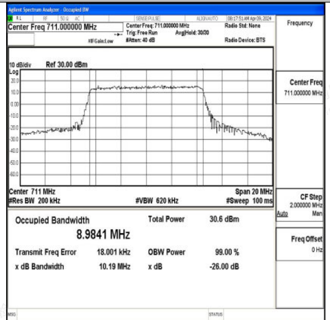
Band17-10MHz-16QAM-23800-50RB#0-PASS
