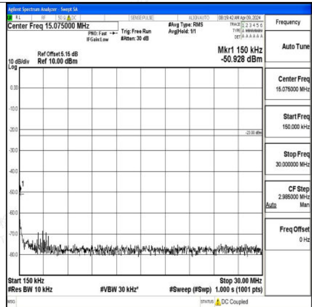
Band17_10MHz_QPSK_23790_1RB#0_0.15~30_0.15~30
