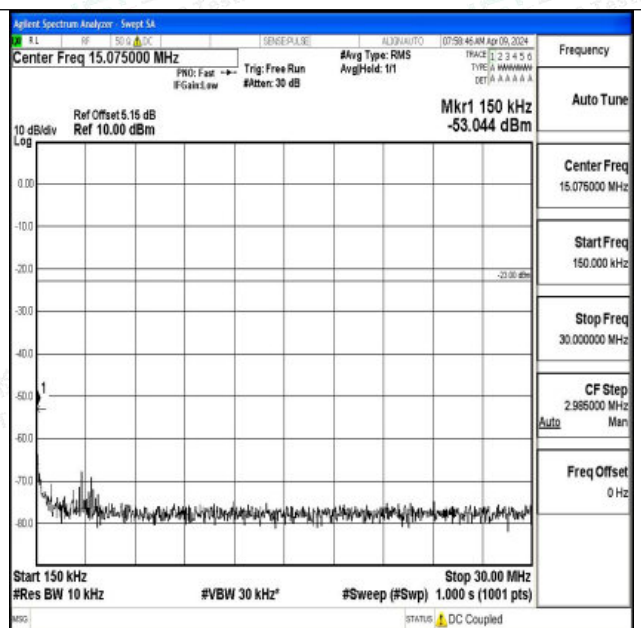
Band17_5MHz_QPSK_23755_1RB#0_0.15~30_0.15~30
