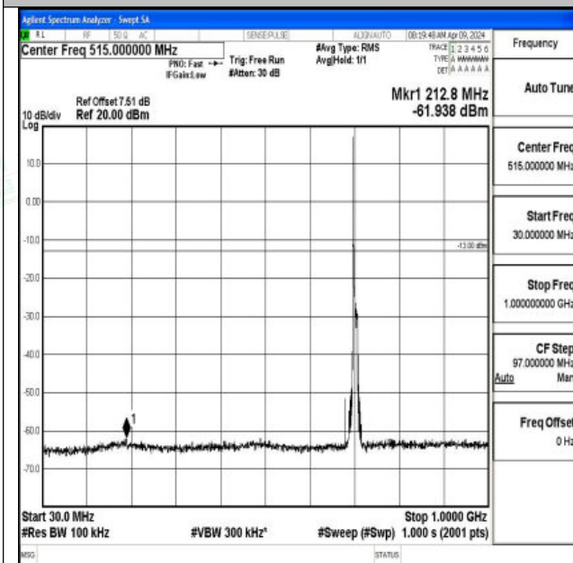
Band17_10MHz_QPSK_23790_1RB#0_30~1000_30~100 0
