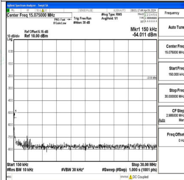
Band17_5MHz_16QAM_23825_1RB#0_0.15~30_0.15~30
