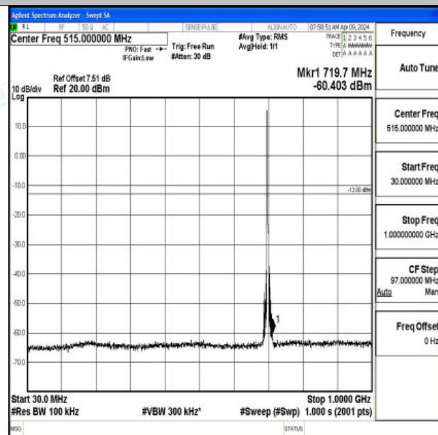
Band17_5MHz_QPSK_23755_1RB#0_30~1000_30~1000
