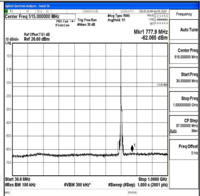
Band17_10MHz_16QAM_23790_1RB#0_30~1000_30~100 0
