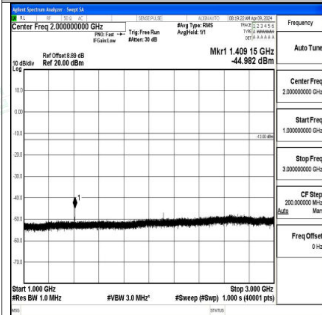
Band17_10MHz_16QAM_23780_1RB#0_1000~3000_100
