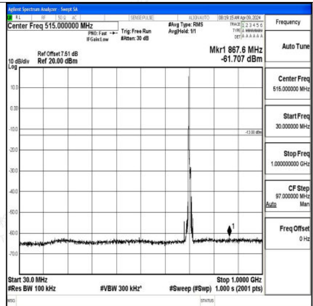
Band17_10MHz_16QAM_23780_1RB#0_30~1000_30~100
