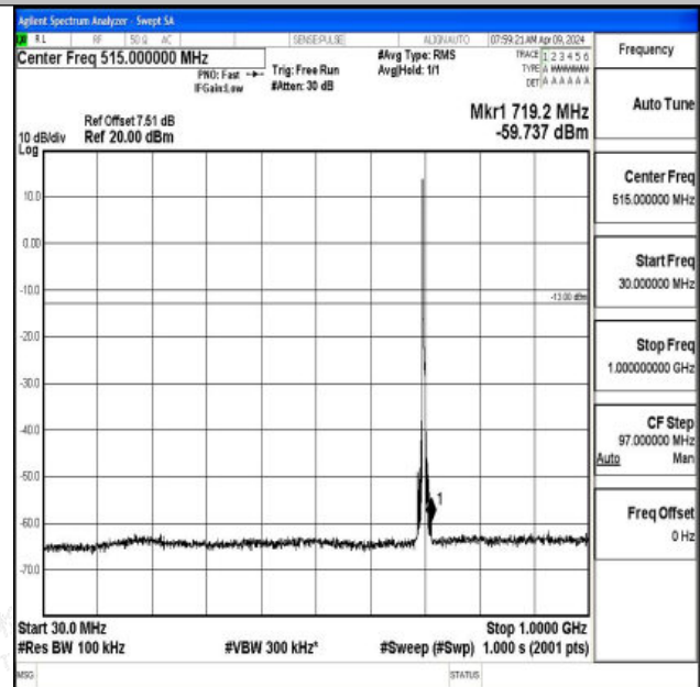
Band17_5MHz_16QAM_23755_1RB#0_30~1000_30~1000
