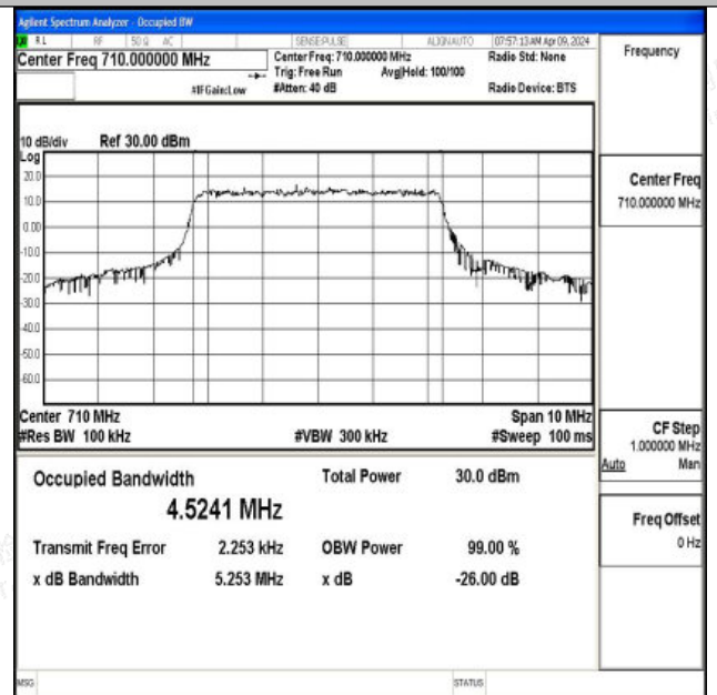
Band17-5MHz-16QAM-23790-25RB#0-PASS
