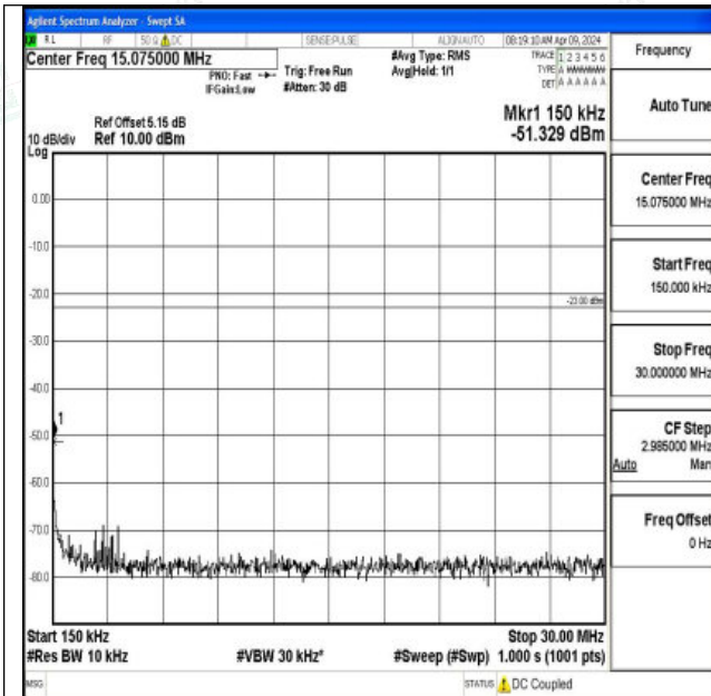
Band17_10MHz_16QAM_23780_1RB#0_0.15~30_0.15~3
