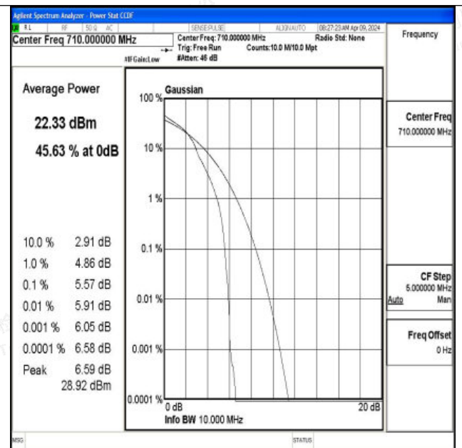
Band17-10MHz-16QAM-23790-1RB#0-PASS
