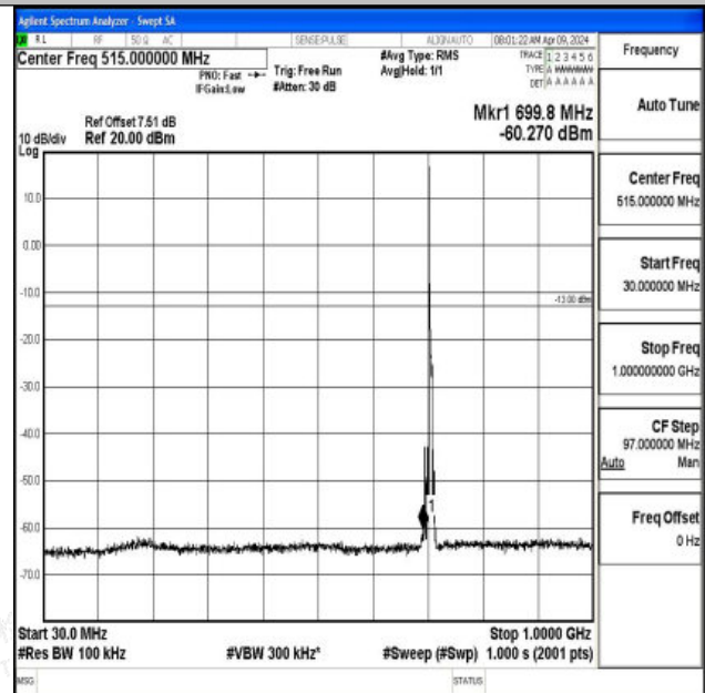
Band17_5MHz_16QAM_23825_1RB#0_30~1000_30~1000
