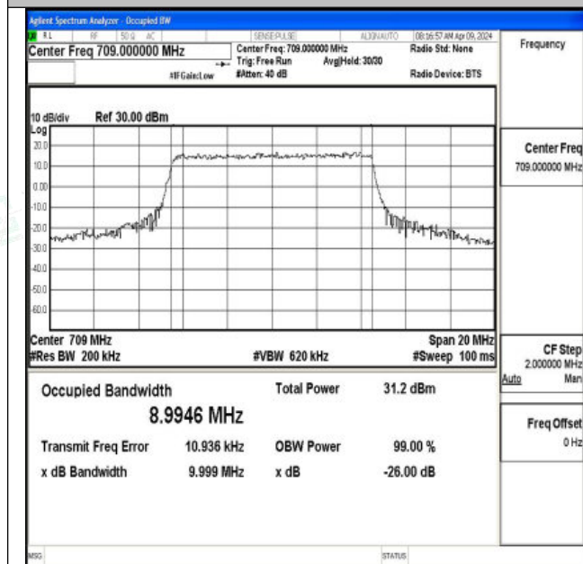
Band17-10MHz-QPSK-23780-50RB#0-PASS
