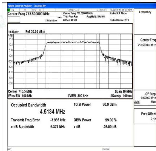
Band17-5MHz-QPSK-23825-25RB#0-PASS
