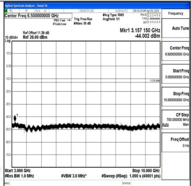
Band17_10MHz_16QAM_23780_1RB#0_3000~10000_300
