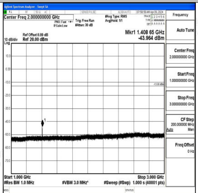
Band17_5MHz_QPSK_23755_1RB#0_1000~3000_1000~3000
