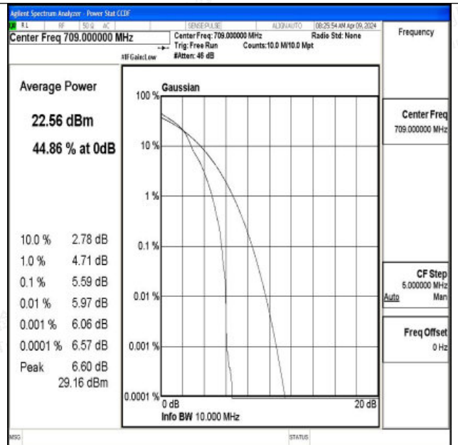
Band17-10MHz-16QAM-23780-1RB#0-PASS
