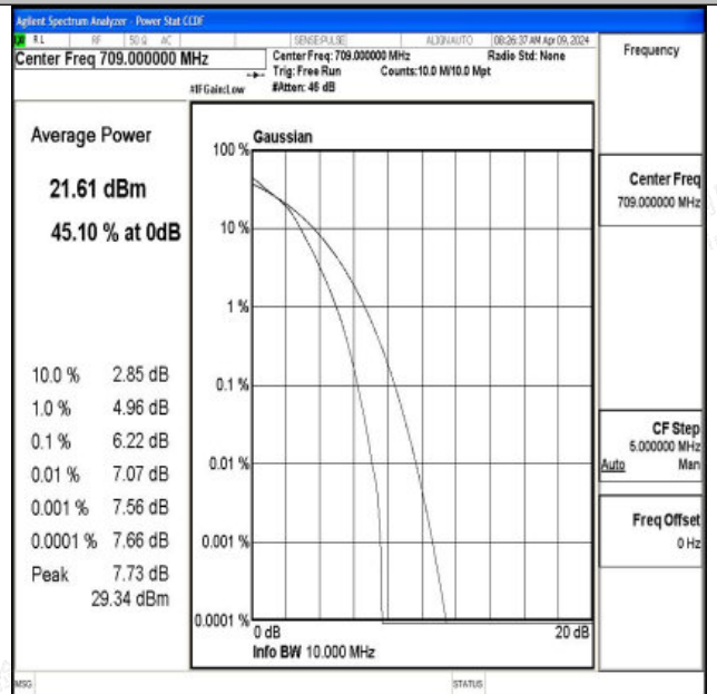
Band17-10MHz-16QAM-23780-50RB#0-PASS
