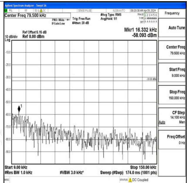
Band17_10MHz_16QAM_23790_1RB#0_0.009~0.15_0.009 ~0.15
