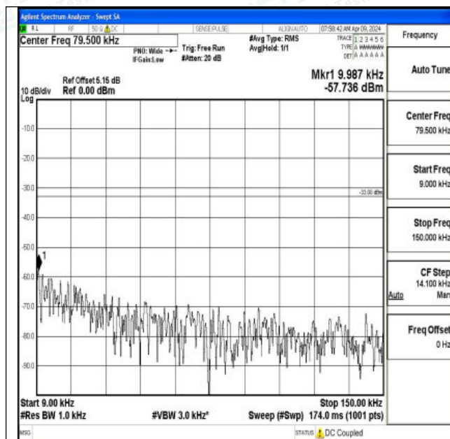
Band17_5MHz_QPSK_23755_1RB#0_0.009~0.15_0.009~0.15
