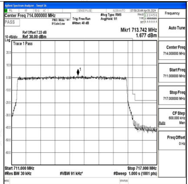
Band17_5MHz_16QAM_23825_25RB#0
