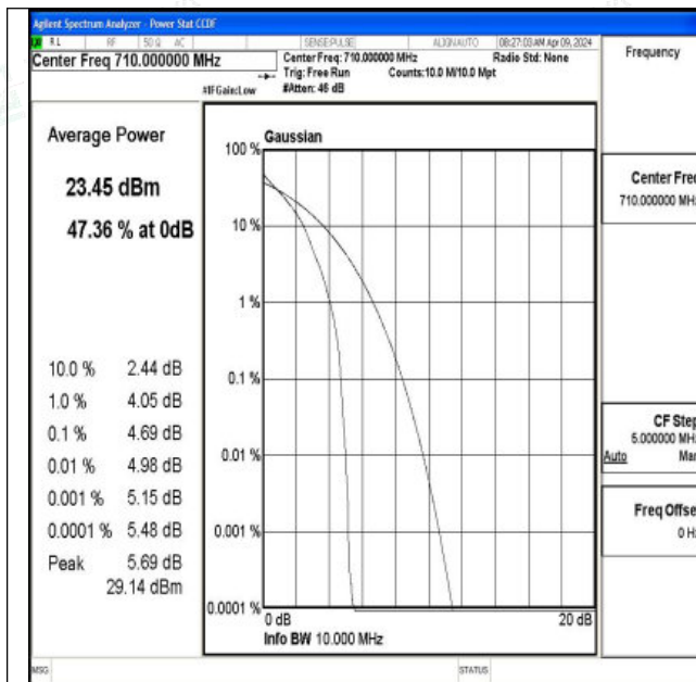
Band17-10MHz-QPSK-23790-1RB#0-PASS
