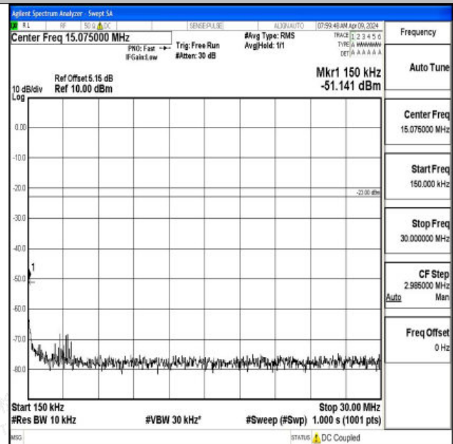
Band17_5MHz_QPSK_23790_1RB#0_0.15~30_0.15~30
