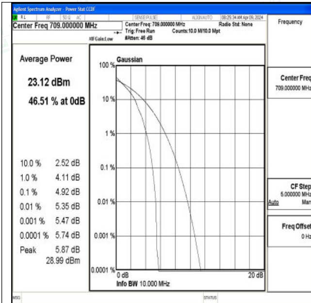
Band17-10MHz-QPSK-23780-1RB#0-PASS
