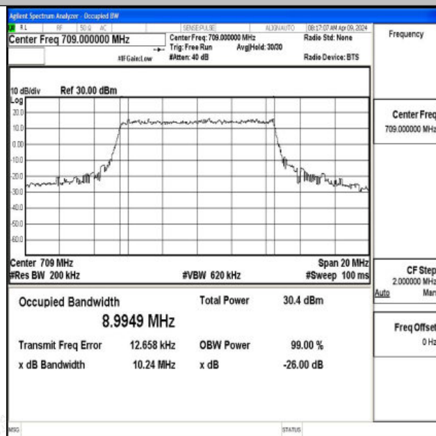
Band17-10MHz-16QAM-23780-50RB#0-PASS
