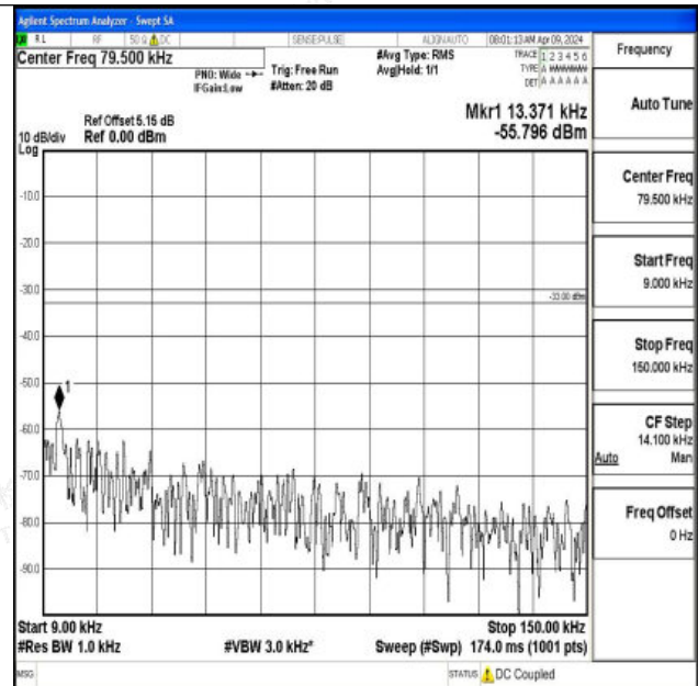
Band17_5MHz_16QAM_23825_1RB#0_0.009~0.15_0.009 ~0.15
