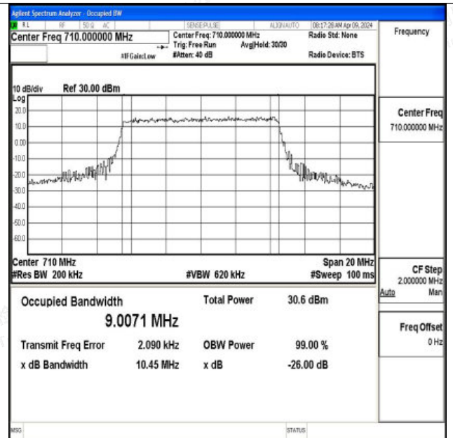
Band17-10MHz-16QAM-23790-50RB#0-PASS
