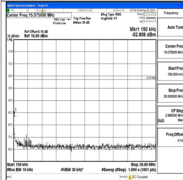
Band17_5MHz_16QAM_23755_1RB#0_0.15~30_0.15~30
