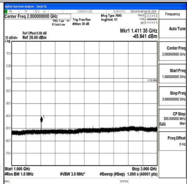
Band17_10MHz_QPSK_23790_1RB#0_1000~3000_1000~ 3000
