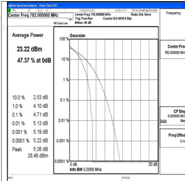
Band13-5MHz-QPSK-23230-1RB#0-PASS
