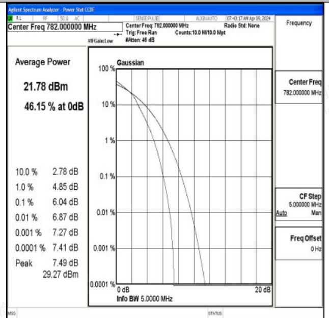
Band13-5MHz-16QAM-23230-25RB#0-PASS
