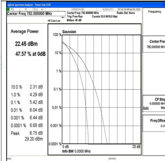
Band13-5MHz-QPSK-23230-25RB#0-PASS
