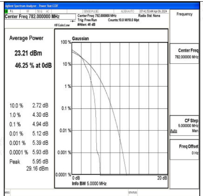
Band13-5MHz-16QAM-23230-1RB#0-PASS
