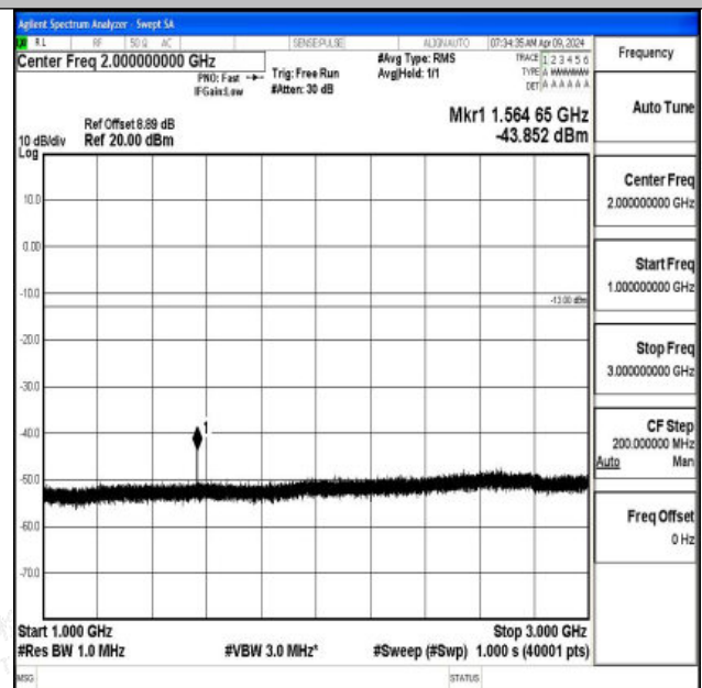
Band13_5MHz_QPSK_23255_1RB#0_1000~3000_1000~3000
