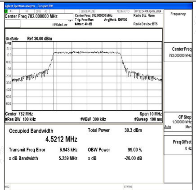
Band13-5MHz-16QAM-23230-25RB#0-PASS
