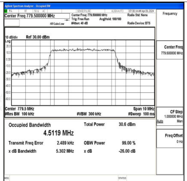
Band13-5MHz-16QAM-23205-25RB#0-PASS
