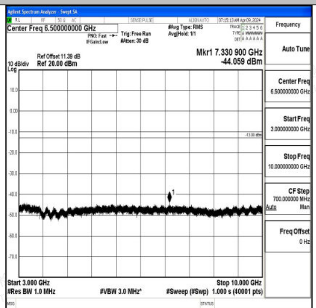
Band12_10MHz_16QAM_23060_1RB#0_3000~10000_300
