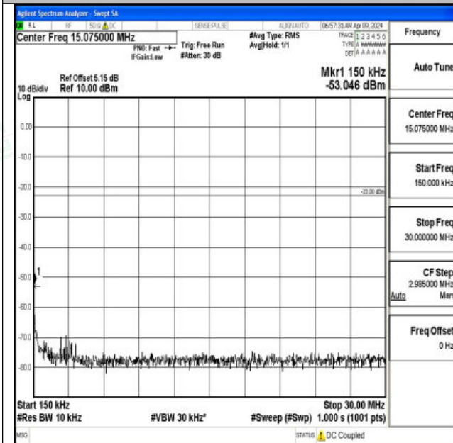
Band12_5MHz_16QAM_23155_1RB#0_0.15~30_0.15~30
