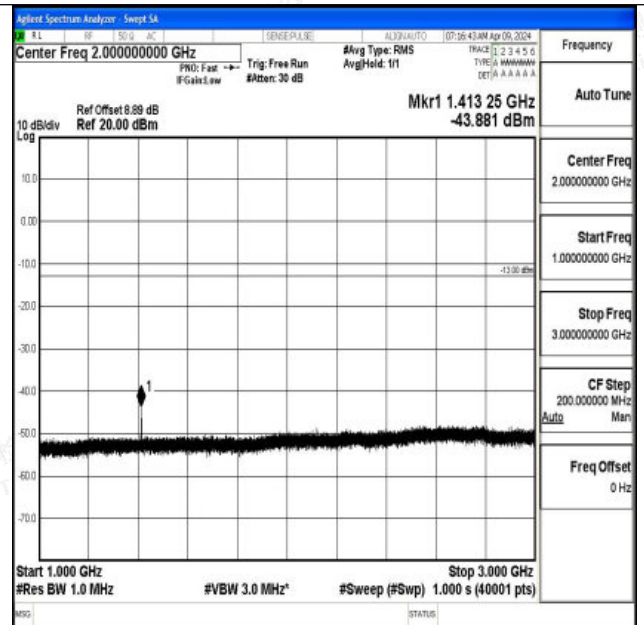
Band12_10MHz_QPSK_23130_1RB#0_1000~3000_1000~3000
