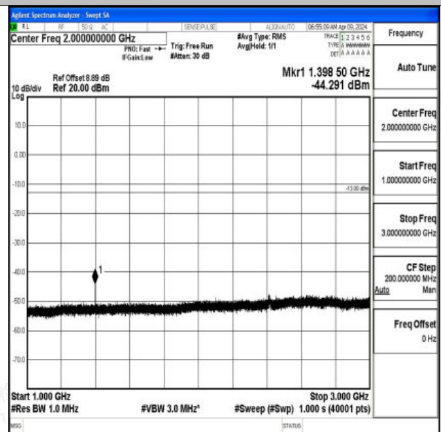
Band12_5MHz_QPSK_23035_1RB#0_1000~3000_1000~3000
