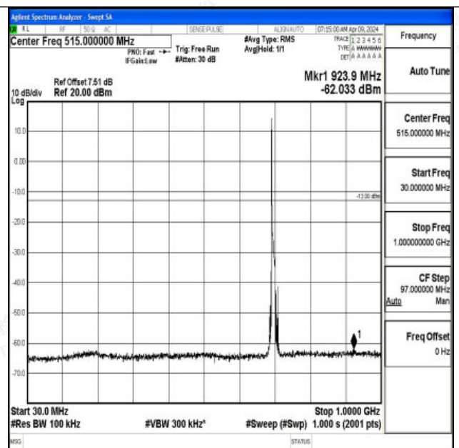
Band12_10MHz_16QAM_23060_1RB#0_30~1000_30~100
