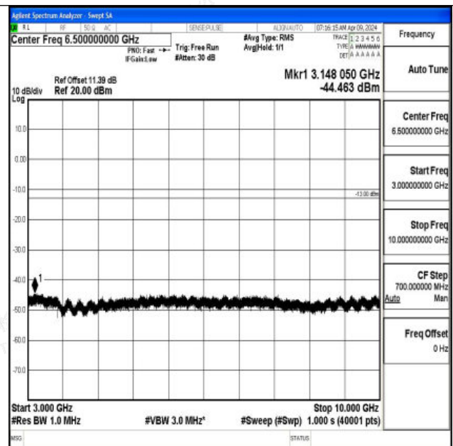
Band12_10MHz_16QAM_23095_1RB#0_3000~10000_300 0~10000
