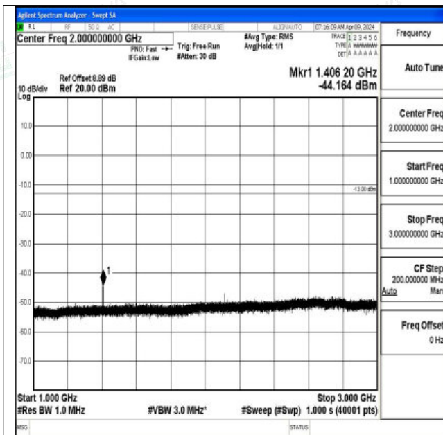
Band12_10MHz_16QAM_23095_1RB#0_1000~3000_100 0~3000
