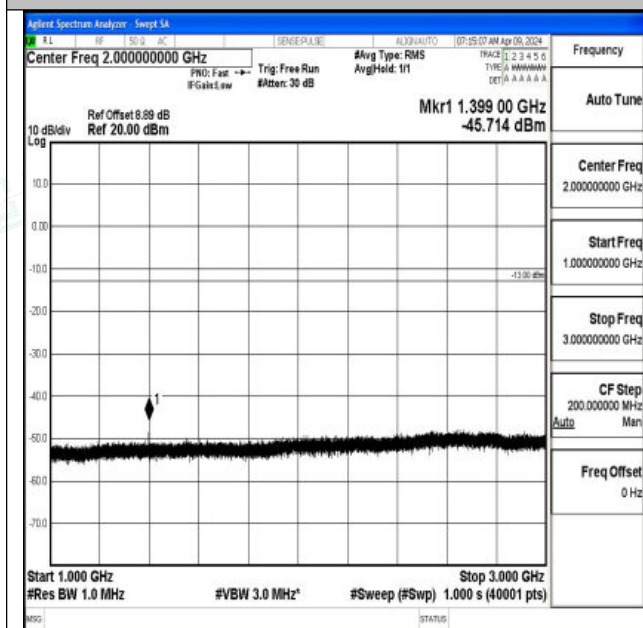
Band12_10MHz_16QAM_23060_1RB#0_1000~3000_100
