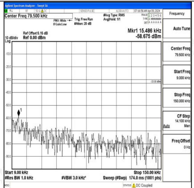
Band12_10MHz_16QAM_23130_1RB#0_0.009~0.15_0.009~0.15
