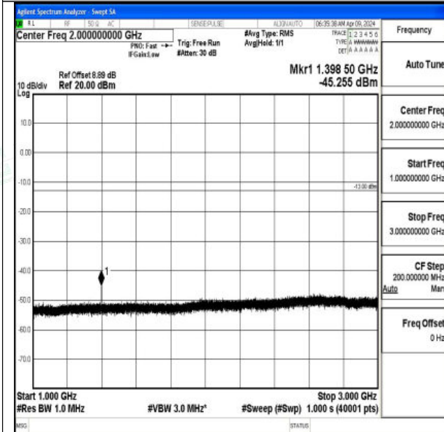
Band12_3MHz_16QAM_23025_1RB#0_1000~3000_1000~3000
