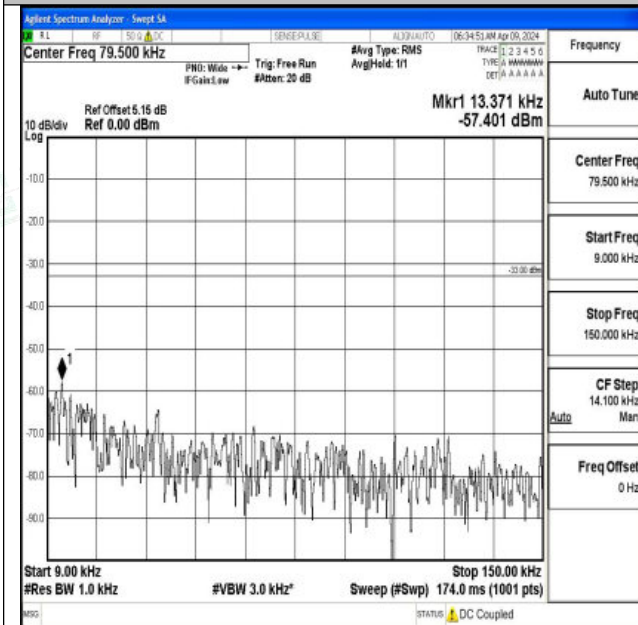
Band12_3MHz_QPSK_23025_1RB#0_0.009~0.15_0.009~0.15
