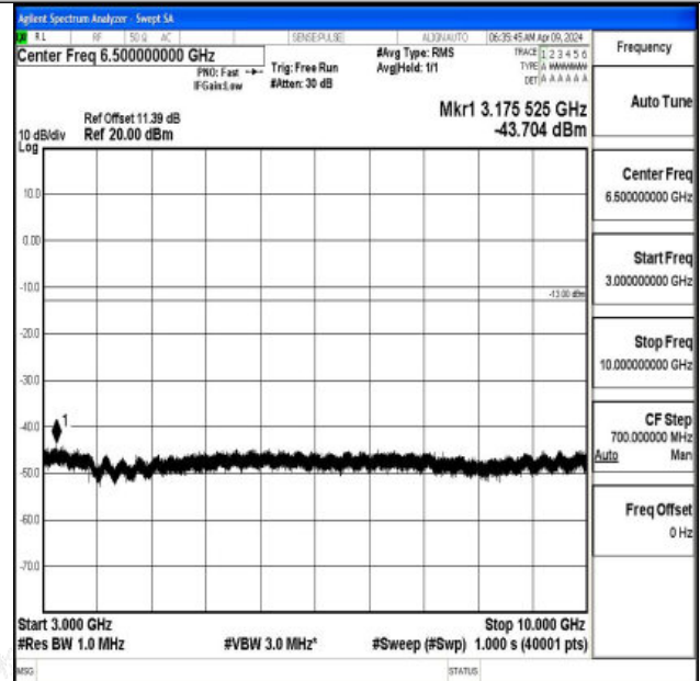
Band12_3MHz_16QAM_23025_1RB#0_3000~10000_3000~10000
