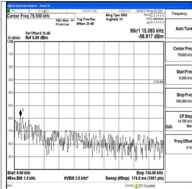
Band12_5MHz_QPSK_23155_1RB#0_0.009~0.15_0.009~0.15
