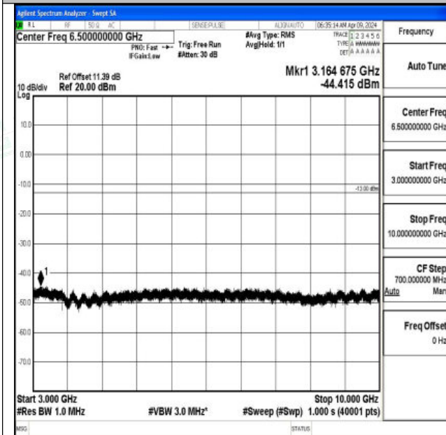
Band12_3MHz_QPSK_23025_1RB#0_3000~10000_3000~10000
