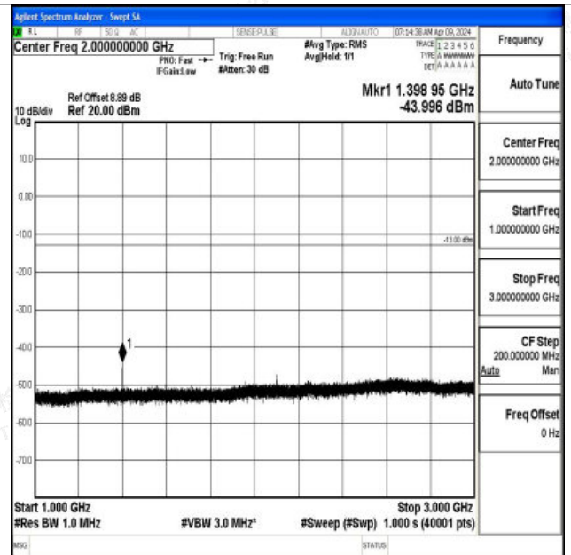
Band12_10MHz_QPSK_23060_1RB#0_1000~3000_1000~3000
