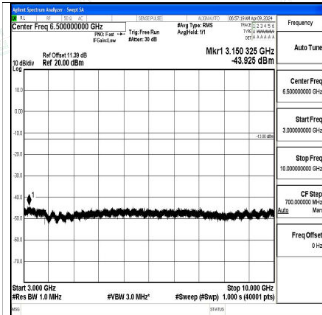
Band12_5MHz_QPSK_23155_1RB#0_3000~10000_3000 ~10000
