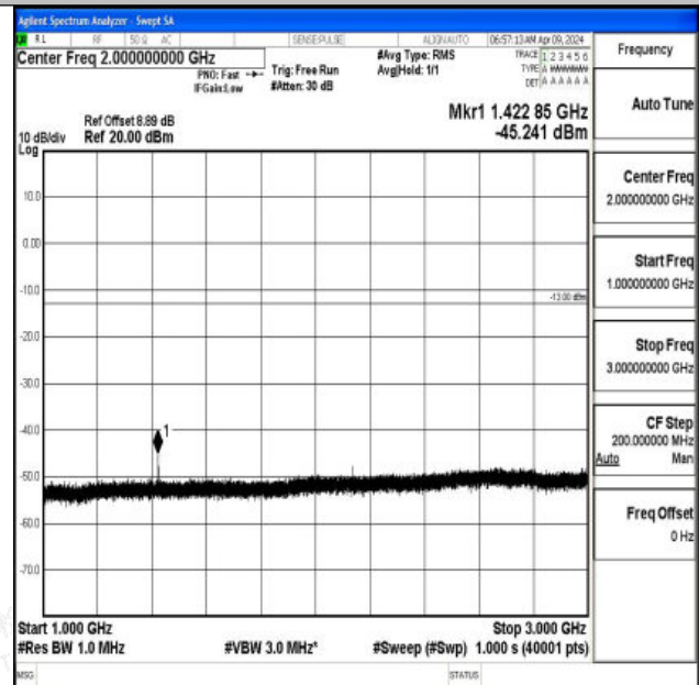
Band12_5MHz_QPSK_23155_1RB#0_1000~3000_1000~3000
