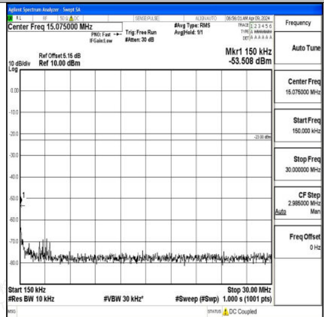
Band12_5MHz_QPSK_23095_1RB#0_0.15~30_0.15~30
