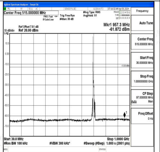
Band12_10MHz_16QAM_23095_1RB#0_30~1000_30~100 0
