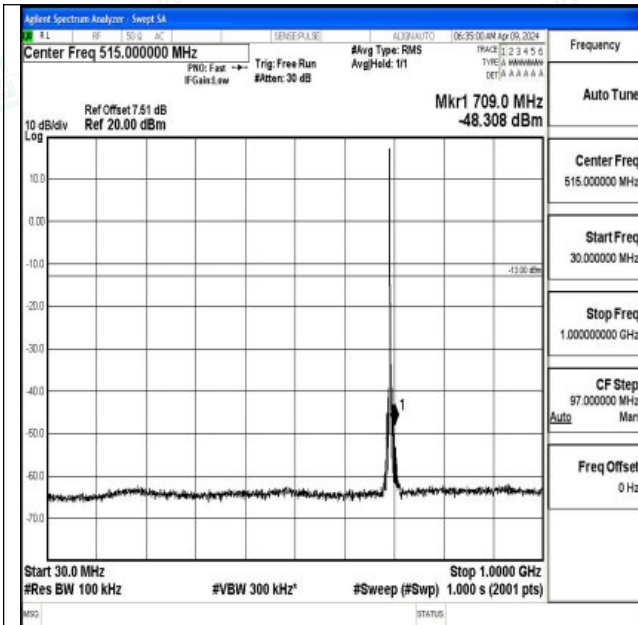
Band12_3MHz_QPSK_23025_1RB#0_30~1000_30~1000
