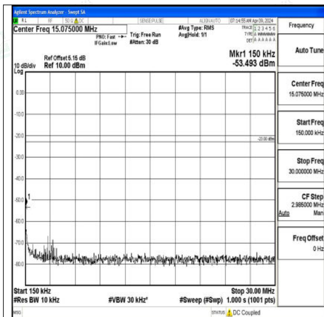
Band12_10MHz_16QAM_23060_1RB#0_0.15~30_0.15~3
