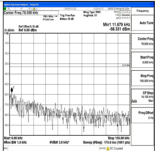
Band12_5MHz_16QAM_23035_1RB#0_0.009~0.15_0.009~0.15
