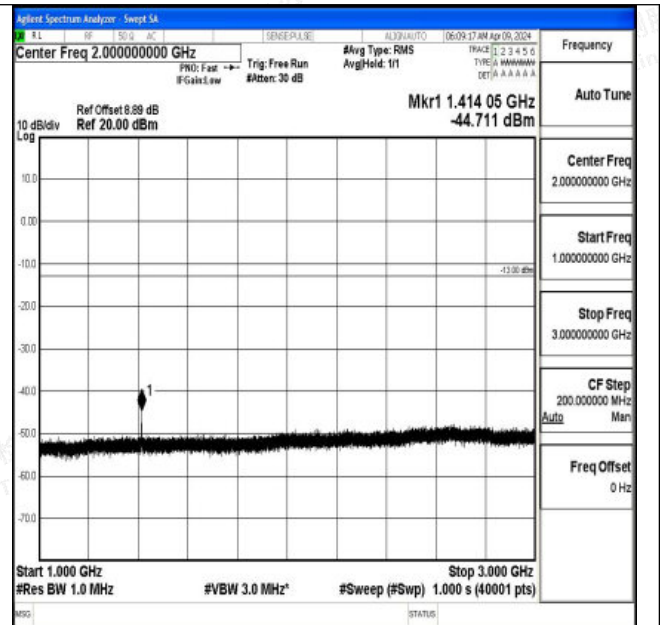
Band12_1.4MHz_QPSK_23095_1RB#0_1000~3000_1000~3000
