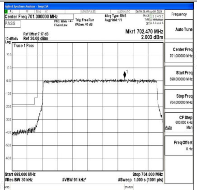
Band12_5MHz_16QAM_23035_25RB#0
