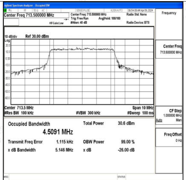
Band12-5MHz-16QAM-23155-25RB#0-PASS
