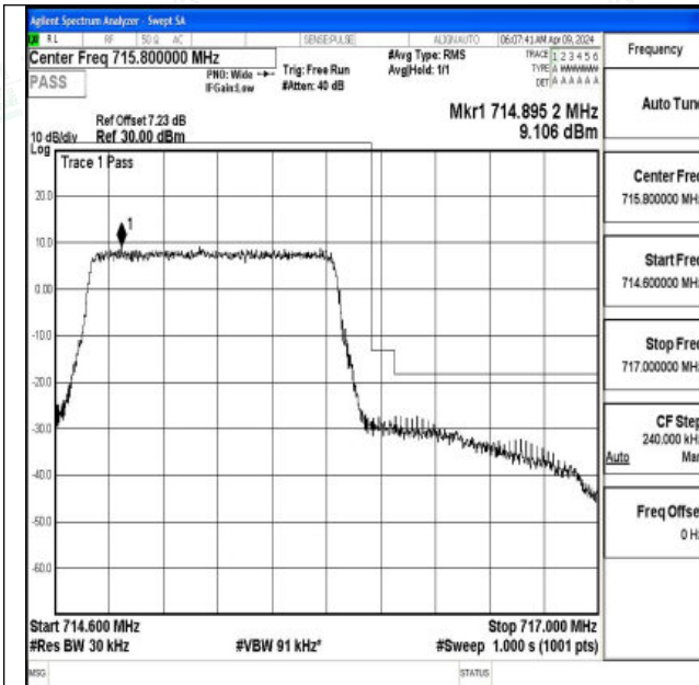
Band12_1.4MHz_QPSK_23173_6RB#0
