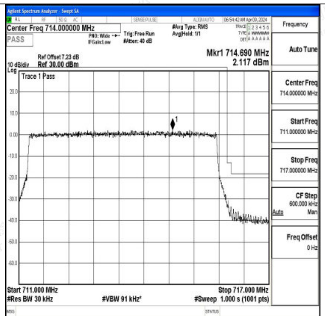
Band12_5MHz_16QAM_23155_25RB#0
