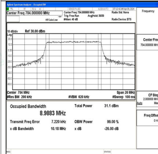
Band12-10MHz-QPSK-23060-50RB#0-PASS
