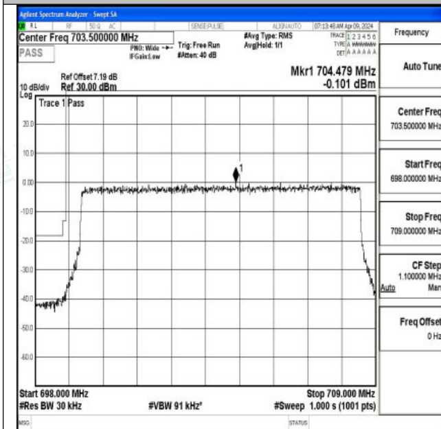
Band12_10MHz_QPSK_23060_50RB#0
