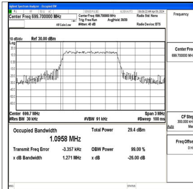
Band12-1.4MHz-QPSK-23017-6RB#0-PASS
