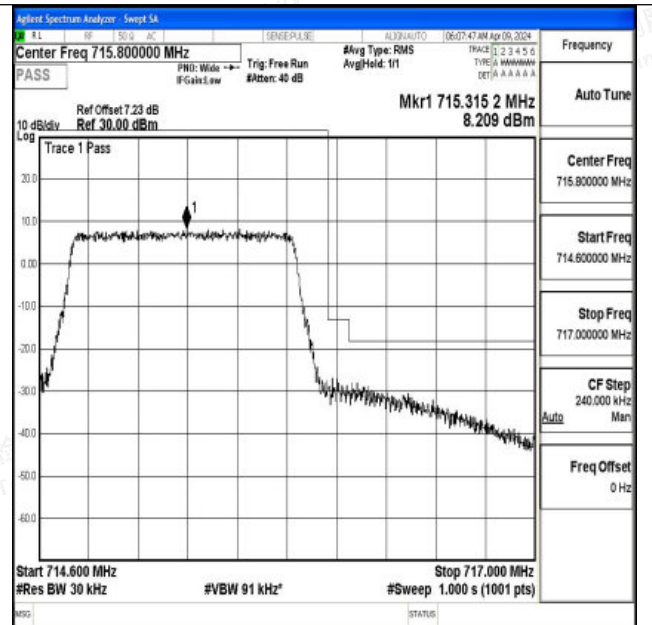
Band12_1.4MHz_16QAM_23173_6RB#0
