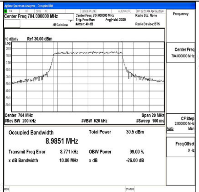
Band12-10MHz-16QAM-23060-50RB#0-PASS
