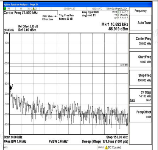
Band12_1.4MHz_16QAM_23095_1RB#0_0.009~0.15_0.009~0.15
