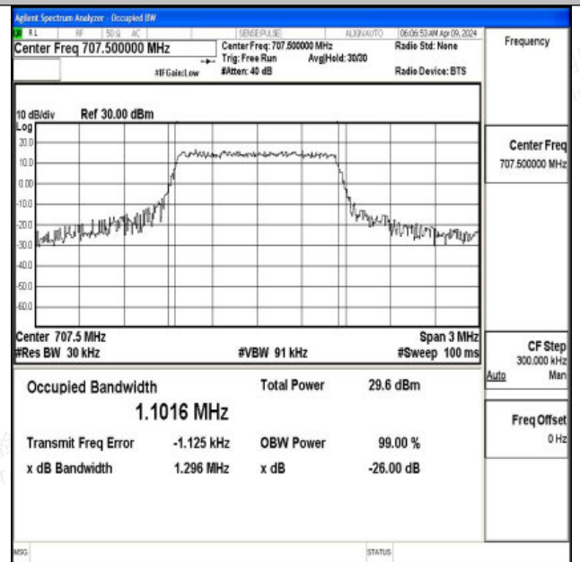
Band12-1.4MHz-16QAM-23095-6RB#0-PASS
