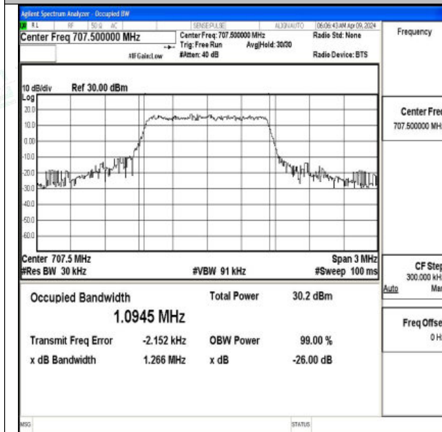
Band12-1.4MHz-QPSK-23095-6RB#0-PASS
