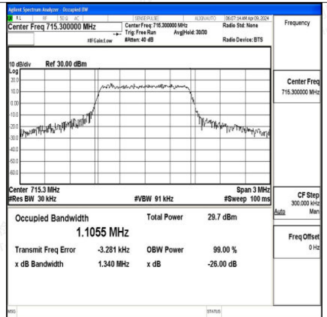
Band12-1.4MHz-16QAM-23173-6RB#0-PASS
