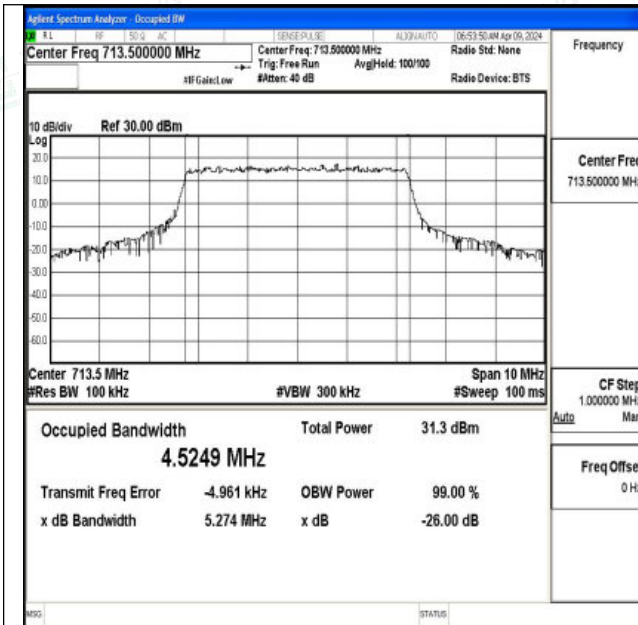
Band12-5MHz-QPSK-23155-25RB#0-PASS
