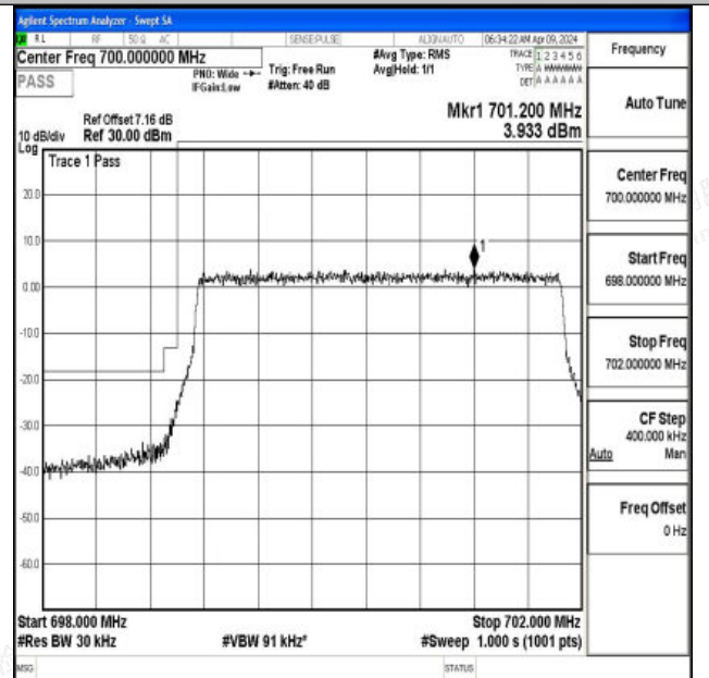
Band12_3MHz_16QAM_23025_15RB#0
