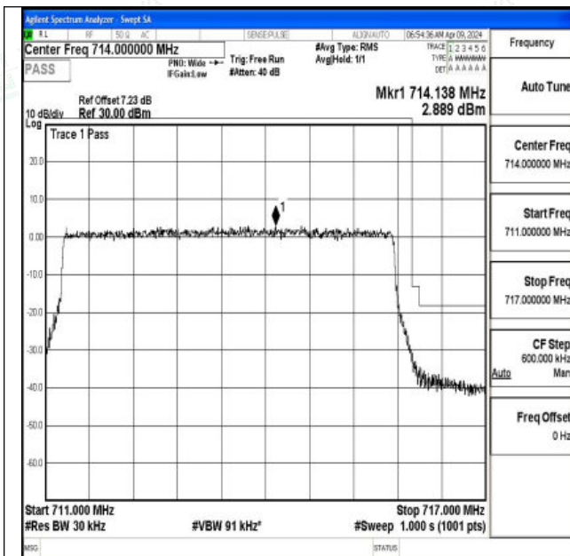
Band12_5MHz_QPSK_23155_25RB#0
