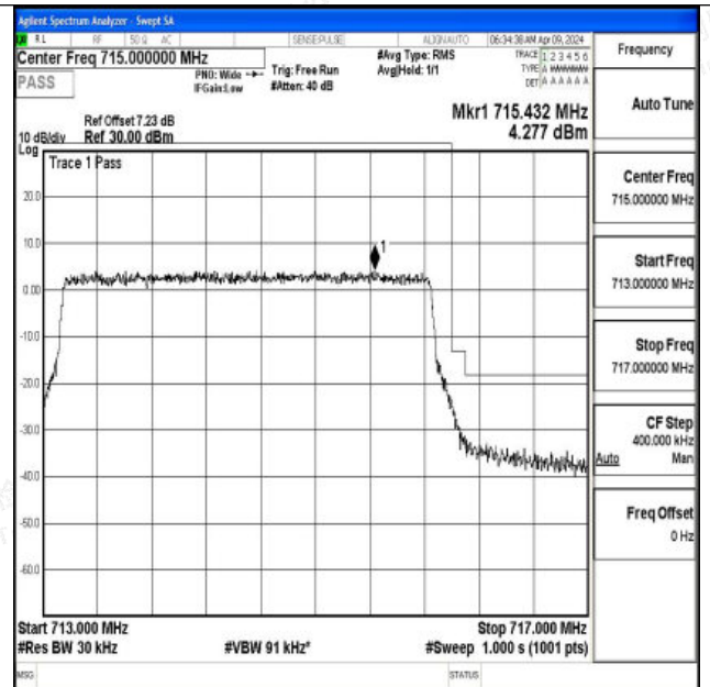
Band12_3MHz_16QAM_23165_15RB#0
