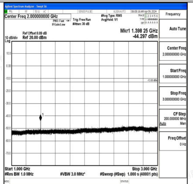
Band12_1.4MHz_QPSK_23017_1RB#0_1000~3000_1000~
