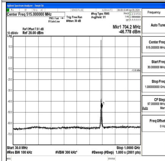
Band12_1.4MHz_QPSK_23017_1RB#0_30~1000_30~100
