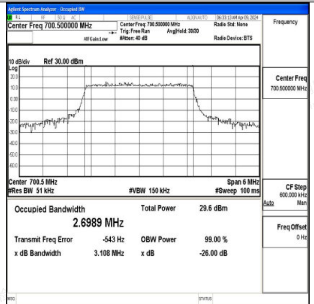
Band12-3MHz-16QAM-23025-15RB#0-PASS
