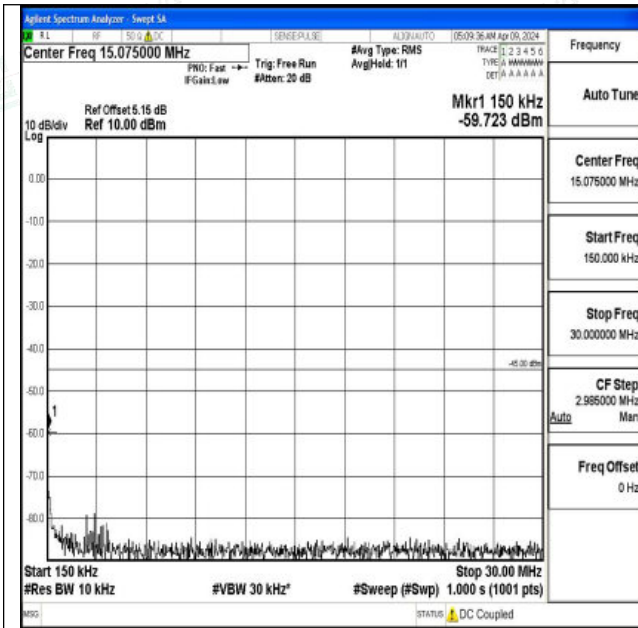
Band7_10MHz_16QAM_20800_1RB#0_0.15~30_0.15~30
