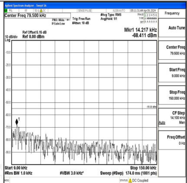
Band7_10MHz_16QAM_21400_1RB#0_0.009~0.15_0.009~0.15
