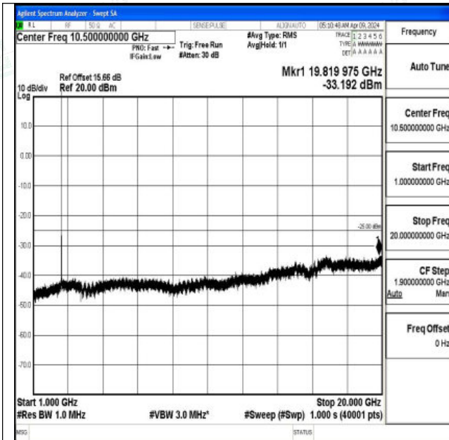
Band7_10MHz_16QAM_21100_1RB#0_1000~20000_100 0~20000
