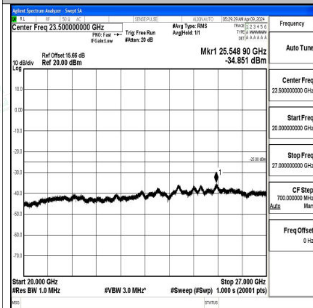
Band7_15MHz_QPSK_21100_1RB#0_20000~27000_20000~27000
