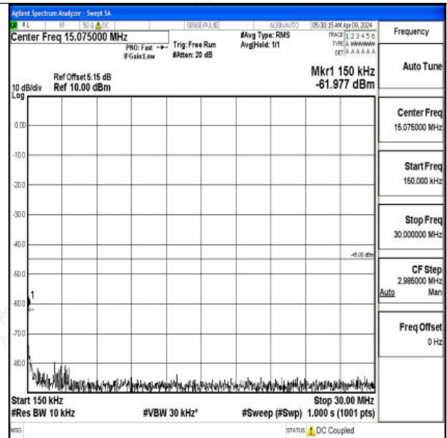
Band7_15MHz_QPSK_21375_1RB#0_0.15~30_0.15~30
