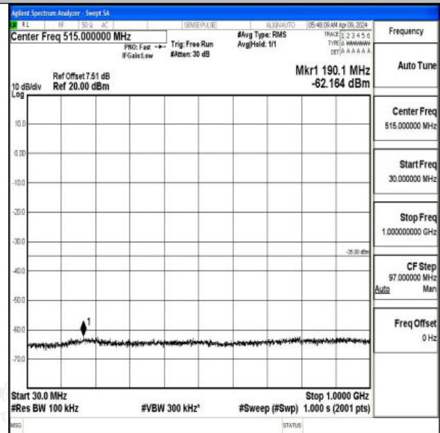
Band7_20MHz_16QAM_21100_1RB#0_30~1000_30~1000
