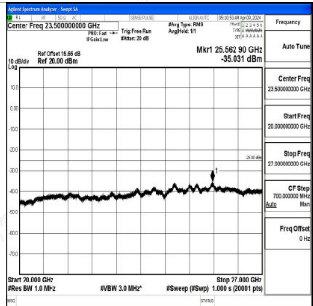
Band7_10MHz_16QAM_21100_1RB#0_20000~27000_200 00~27000
