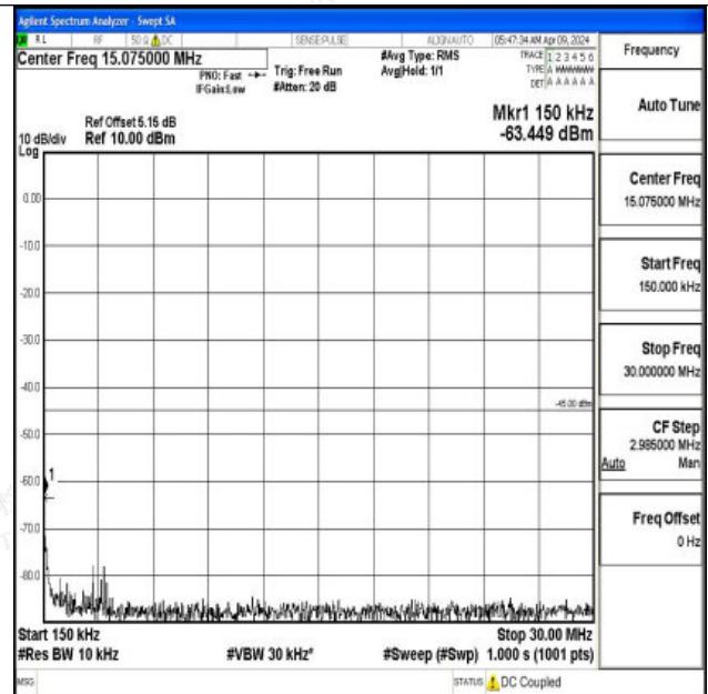
Band7_20MHz_QPSK_21100_1RB#0_0.15~30_0.15~30
