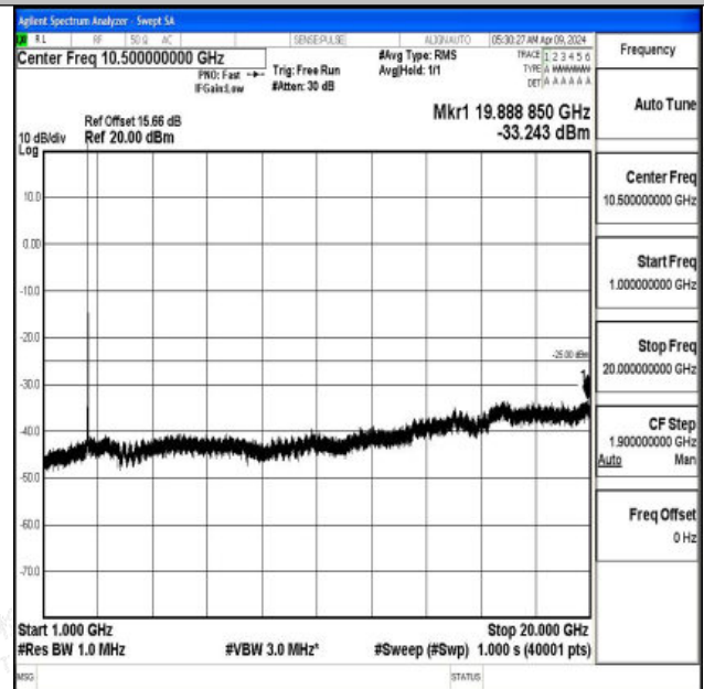
Band7_15MHz_QPSK_21375_1RB#0_1000~20000_1000~20000
