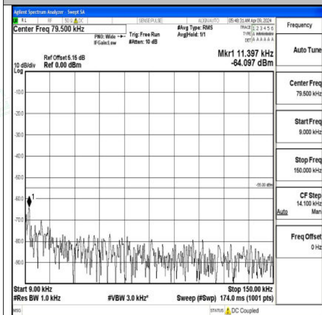
Band7_20MHz_QPSK_21350_1RB#0_0.009~0.15_0.009~0.15
