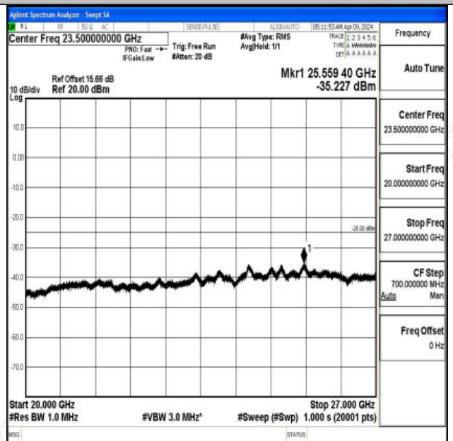
Band7_10MHz_16QAM_21400_1RB#0_20000~27000_20000~27000
