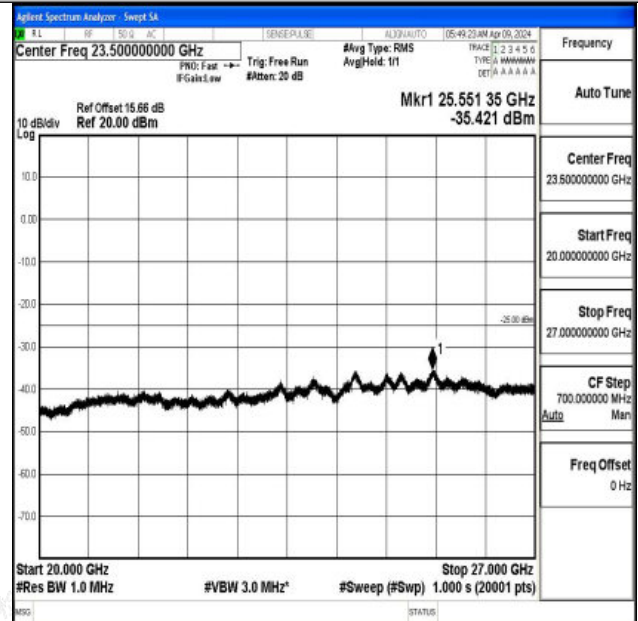
Band7_20MHz_16QAM_21350_1RB#0_20000~27000_200 00~27000
