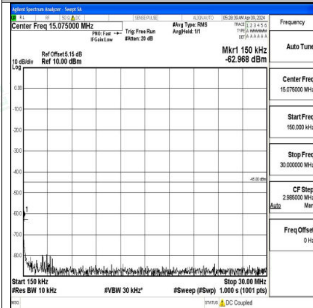
Band7_15MHz_16QAM_20825_1RB#0_0.15~30_0.15~30
