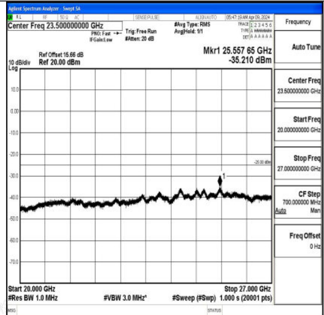
Band7_20MHz_16QAM_20850_1RB#0_20000~27000_20000~27000
