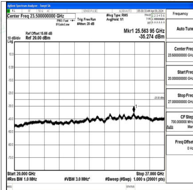
Band7_15MHz_QPSK_21375_1RB#0_20000~27000_2000~27000
