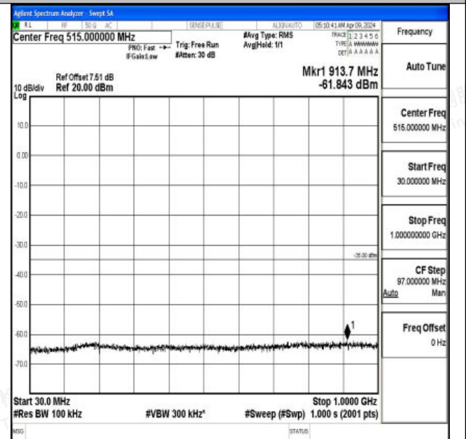
Band7_10MHz_16QAM_21100_1RB#0_30~1000_30~1000
