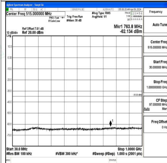
Band7_15MHz_QPSK_21375_1RB#0_30~1000_30~1000
