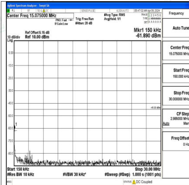
Band7_20MHz_16QAM_20850_1RB#0_0.15~30_0.15~30
