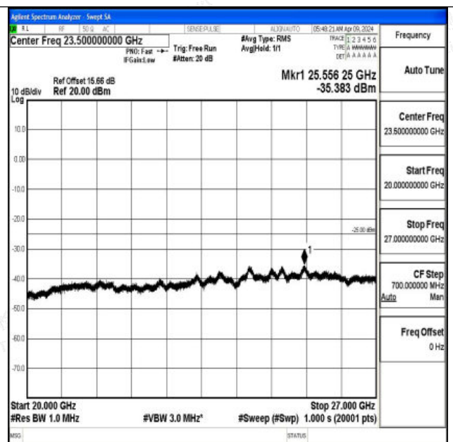
Band7_20MHz_16QAM_21100_1RB#0_20000~27000_200 00~27000
