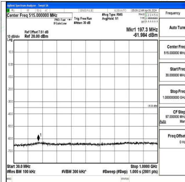
Band7_10MHz_QPSK_20800_1RB#0_30~1000_30~1000
