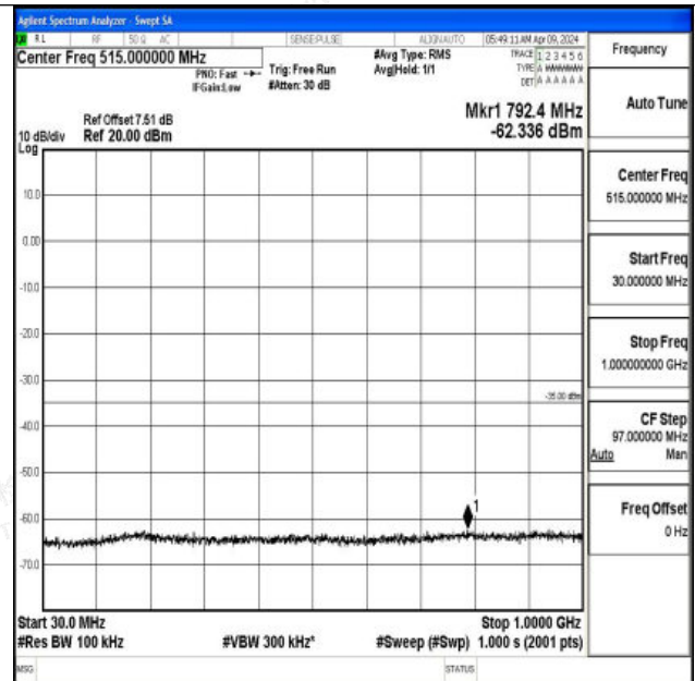
Band7_20MHz_16QAM_21350_1RB#0_30~1000_30~1000
