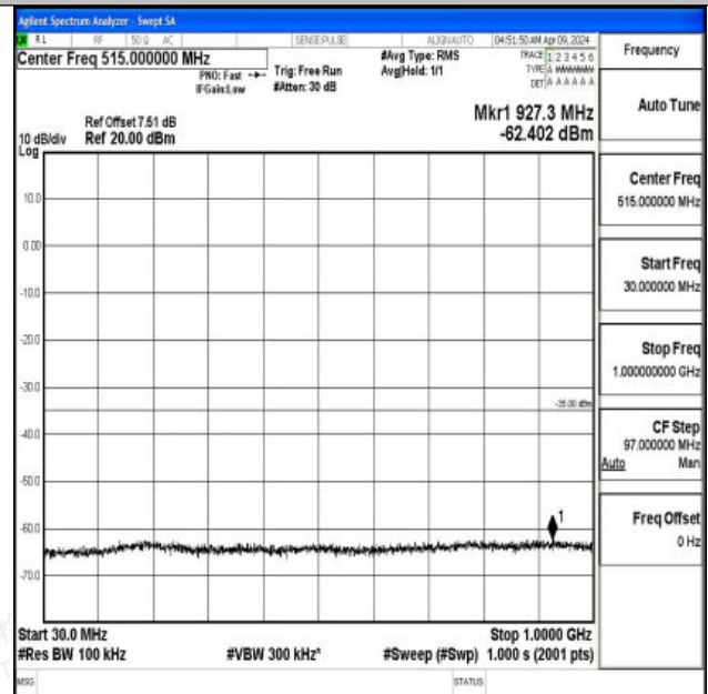
Band7_5MHz_16QAM_21425_1RB#0_30~1000_30~1000
