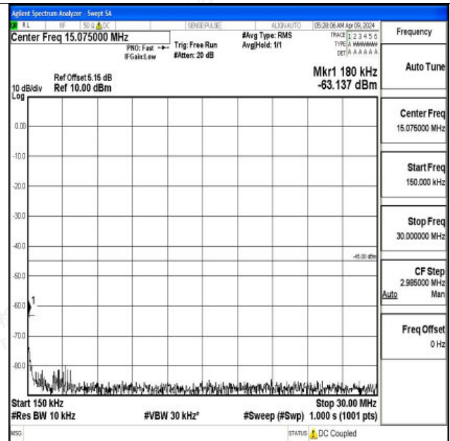
Band7_15MHz_QPSK_20825_1RB#0_0.15~30_0.15~30
