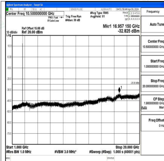
Band7_5MHz_16QAM_21425_1RB#0_1000~20000_1000~20000
