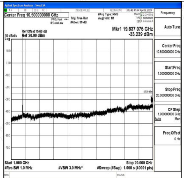
Band7_20MHz_QPSK_21350_1RB#0_1000~20000_1000~20000
