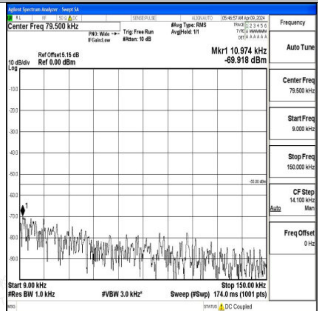
Band7_20MHz_16QAM_20850_1RB#0_0.009~0.15_0.009~0.15
