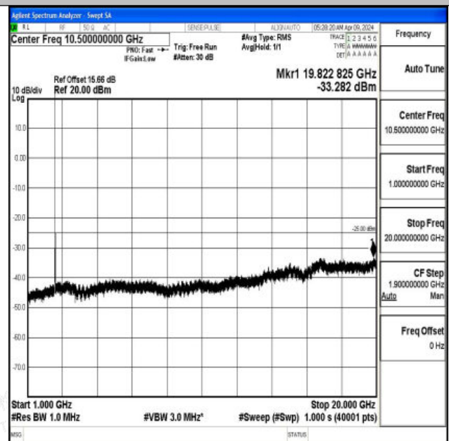
Band7_15MHz_QPSK_20825_1RB#0_1000~20000_1000~20000
