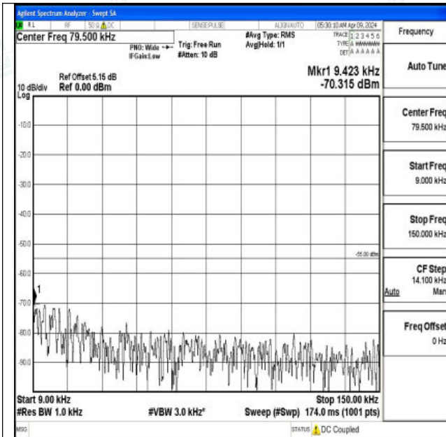
Band7_15MHz_QPSK_21375_1RB#0_0.009~0.15_0.009~0.15
