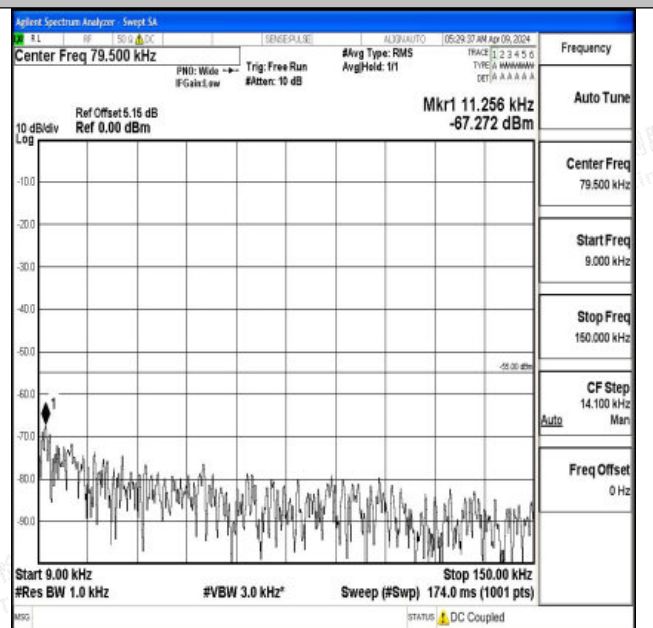
Band7_15MHz_16QAM_21100_1RB#0_0.009~0.15_0.009~0.15
