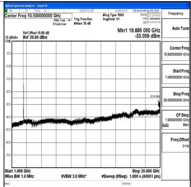
Band7_20MHz_QPSK_20850_1RB#0_1000~20000_1000~20000
