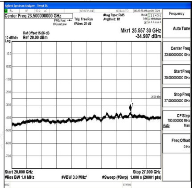
Band7_15MHz_16QAM_20825_1RB#0_20000~27000_200 00~27000
