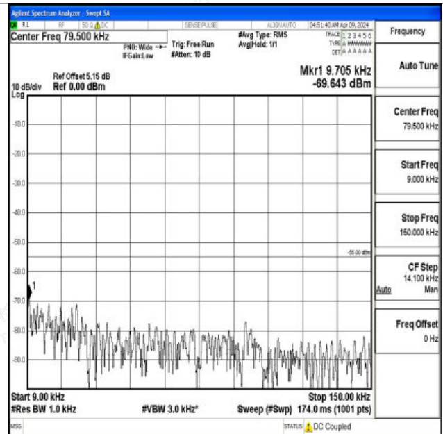
Band7_5MHz_16QAM_21425_1RB#0_0.009~0.15_0.009~ 0.15
