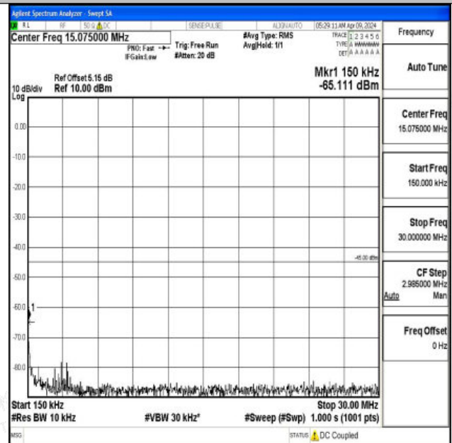
Band7_15MHz_QPSK_21100_1RB#0_0.15~30_0.15~30
