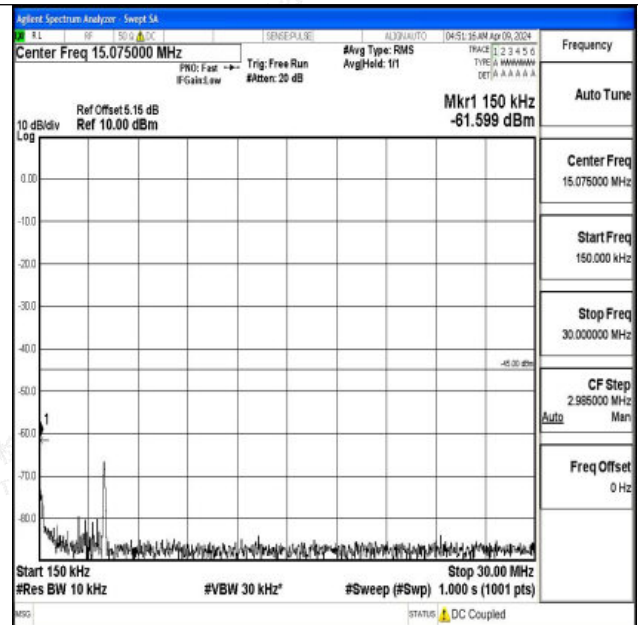
Band7_5MHz_QPSK_21425_1RB#0_0.15~30_0.15~30
