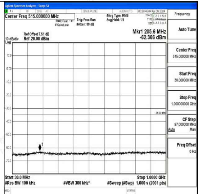
Band7_15MHz_16QAM_21100_1RB#0_30~1000_30~1000
