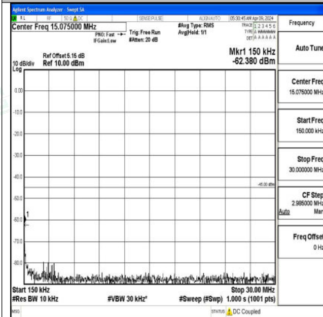
Band7_15MHz_16QAM_21375_1RB#0_0.15~30_0.15~30
