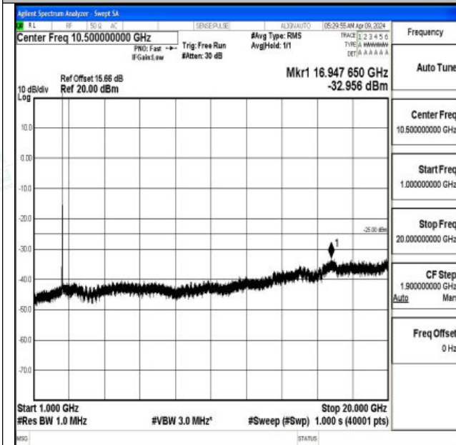
Band7_15MHz_16QAM_21100_1RB#0_1000~20000_100 0~20000
