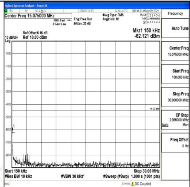
Band7_20MHz_QPSK_20850_1RB#0_0.15~30_0.15~30
