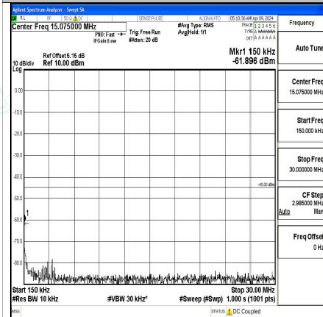
Band7_10MHz_16QAM_21100_1RB#0_0.15~30_0.15~30
