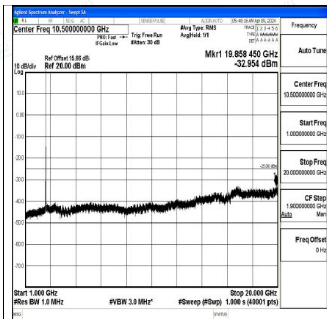
Band7_20MHz_16QAM_21100_1RB#0_1000~20000_100 0~20000
