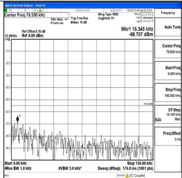
Band7_10MHz_16QAM_20800_1RB#0_0.009~0.15_0.009~0.15
