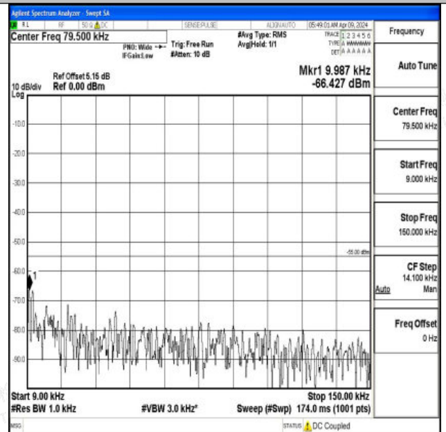
Band7_20MHz_16QAM_21350_1RB#0_0.009~0.15_0.009~0.15
