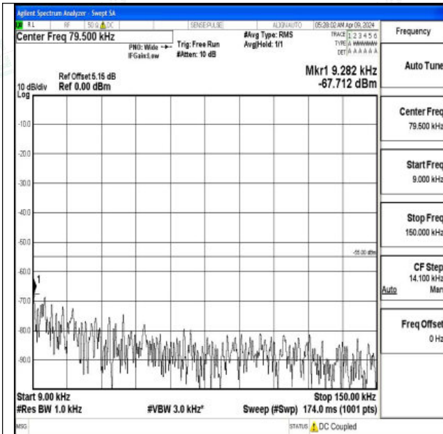
Band7_15MHz_QPSK_20825_1RB#0_0.009~0.15_0.009~0.15
