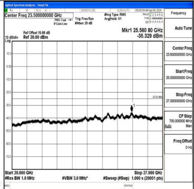
Band7_10MHz_16QAM_20800_1RB#0_20000~27000_200 00~27000
