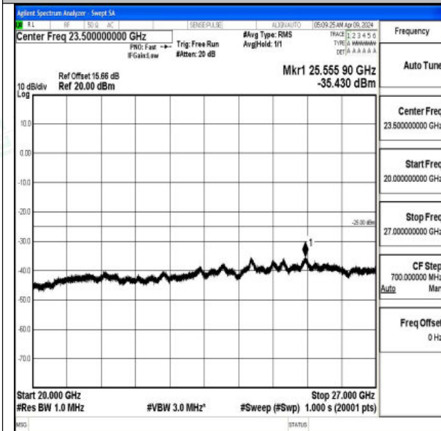
Band7_10MHz_QPSK_20800_1RB#0_20000~27000_20000~27000
