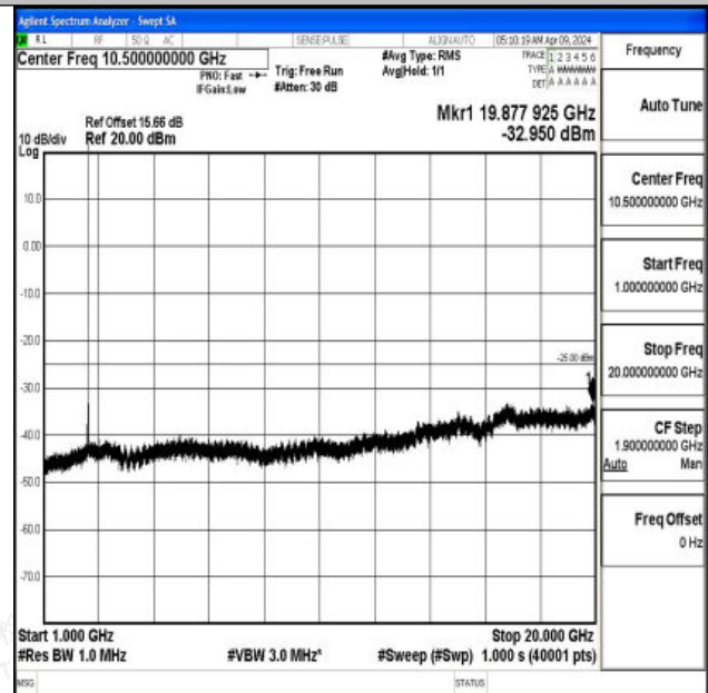
Band7_10MHz_QPSK_21100_1RB#0_1000~20000_1000~20000
