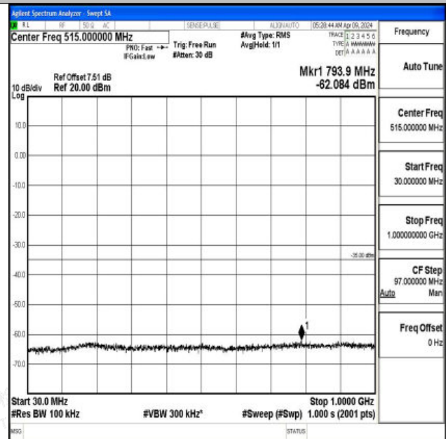
Band7_15MHz_16QAM_20825_1RB#0_30~1000_30~1000
