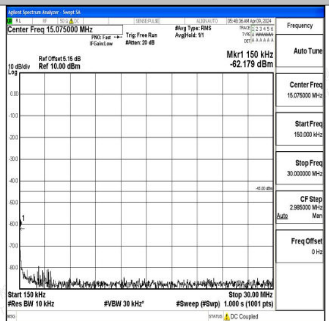
Band7_20MHz_QPSK_21350_1RB#0_0.15~30_0.15~30
