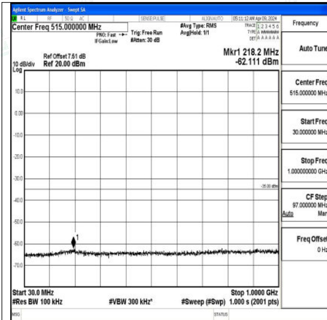
Band7_10MHz_QPSK_21400_1RB#0_30~1000_30~1000
