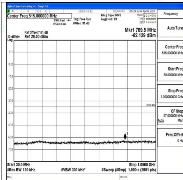
Band7_15MHz_QPSK_21100_1RB#0_30~1000_30~1000
