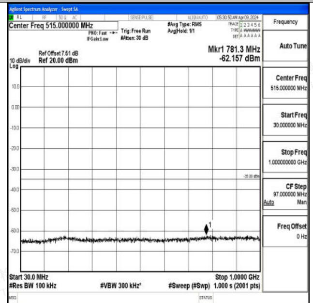
Band7_15MHz_16QAM_21375_1RB#0_30~1000_30~1000
