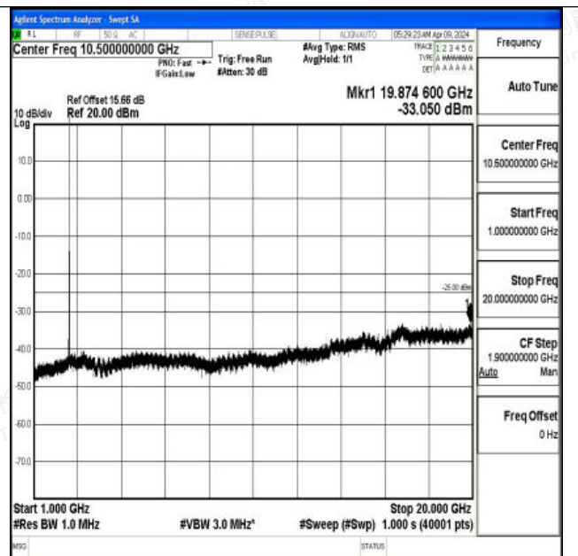
Band7_15MHz_QPSK_21100_1RB#0_1000~20000_1000~20000
