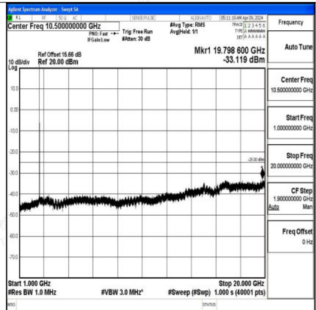
Band7_10MHz_QPSK_21400_1RB#0_1000~20000_1000~20000
