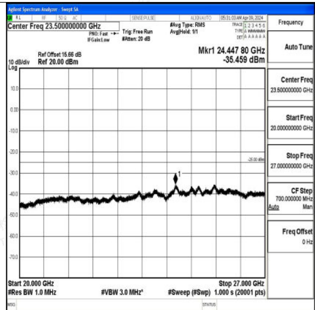
Band7_15MHz_16QAM_21375_1RB#0_20000~27000_200 00~27000
