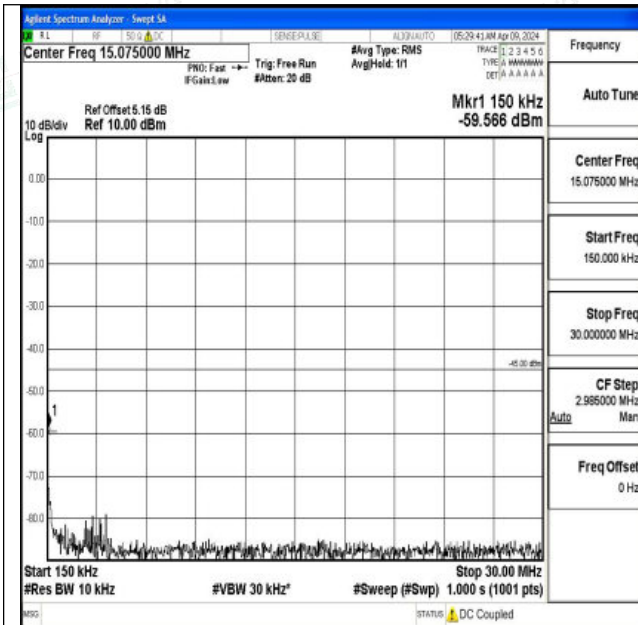
Band7_15MHz_16QAM_21100_1RB#0_0.15~30_0.15~30
