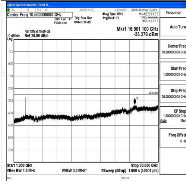
Band7_10MHz_16QAM_20800_1RB#0_1000~20000_100 0~20000
