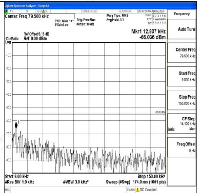
Band7_20MHz_16QAM_21100_1RB#0_0.009~0.15_0.009~0.15
