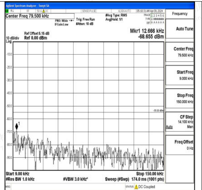
Band7_10MHz_16QAM_21100_1RB#0_0.009~0.15_0.009~0.15
