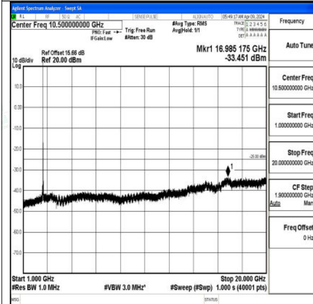
Band7_20MHz_16QAM_21350_1RB#0_1000~20000_100 0~20000
