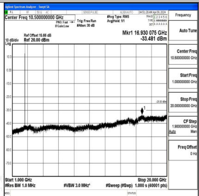
Band7_5MHz_QPSK_21425_1RB#0_1000~20000_1000~20000
