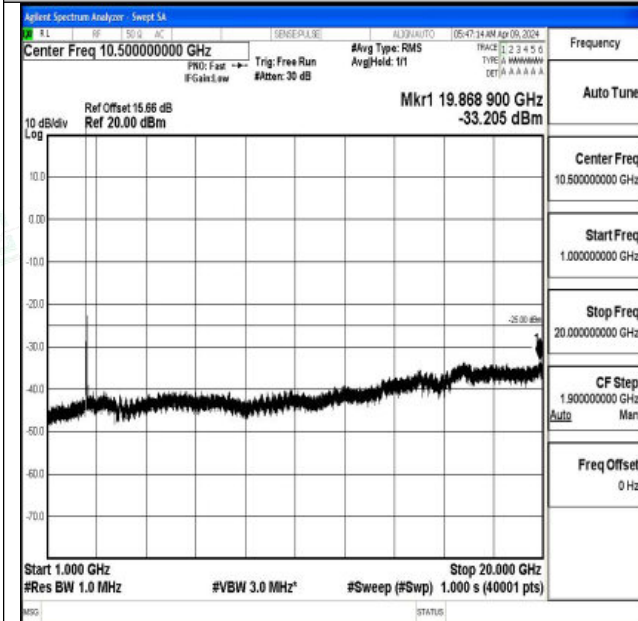
Band7_20MHz_16QAM_20850_1RB#0_1000~20000_1000~20000
