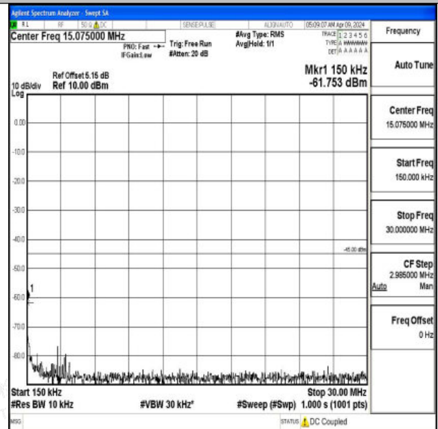
Band7_10MHz_QPSK_20800_1RB#0_0.15~30_0.15~30
