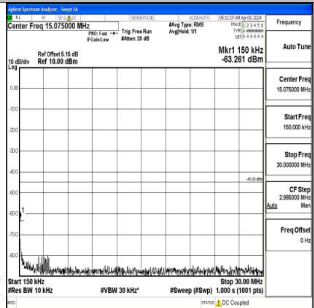
Band7_10MHz_QPSK_21400_1RB#0_0.15~30_0.15~30
