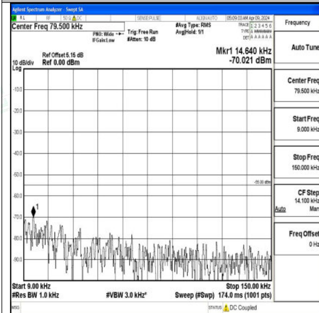
Band7_10MHz_QPSK_20800_1RB#0_0.009~0.15_0.009~0.15
