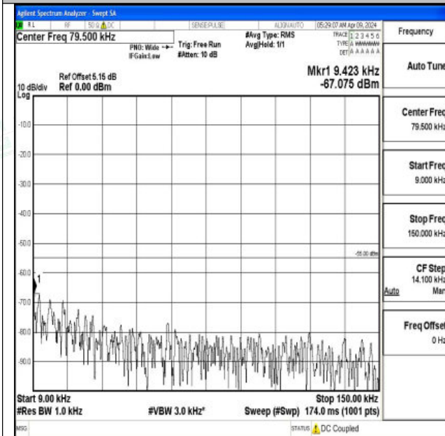
Band7_15MHz_QPSK_21100_1RB#0_0.009~0.15_0.009~0.15
