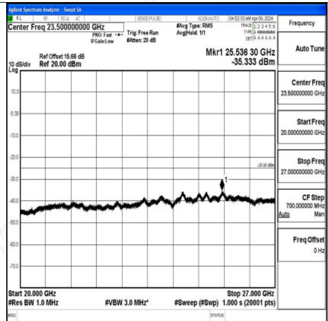
Band7_5MHz_16QAM_21425_1RB#0_20000~27000_2000~27000
