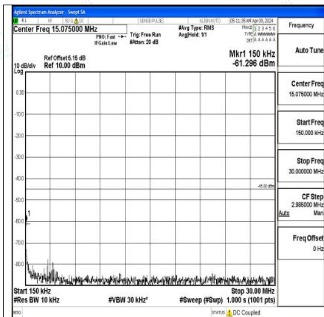
Band7_10MHz_16QAM_21400_1RB#0_0.15~30_0.15~30
