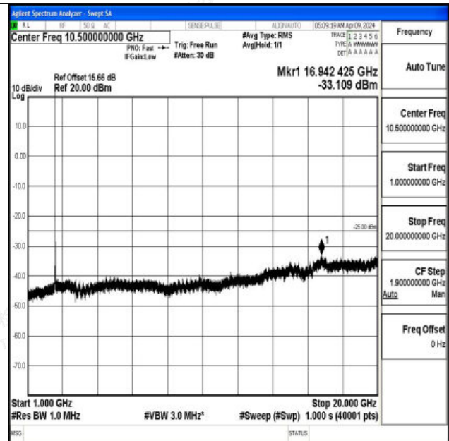
Band7_10MHz_QPSK_20800_1RB#0_1000~20000_1000~20000
