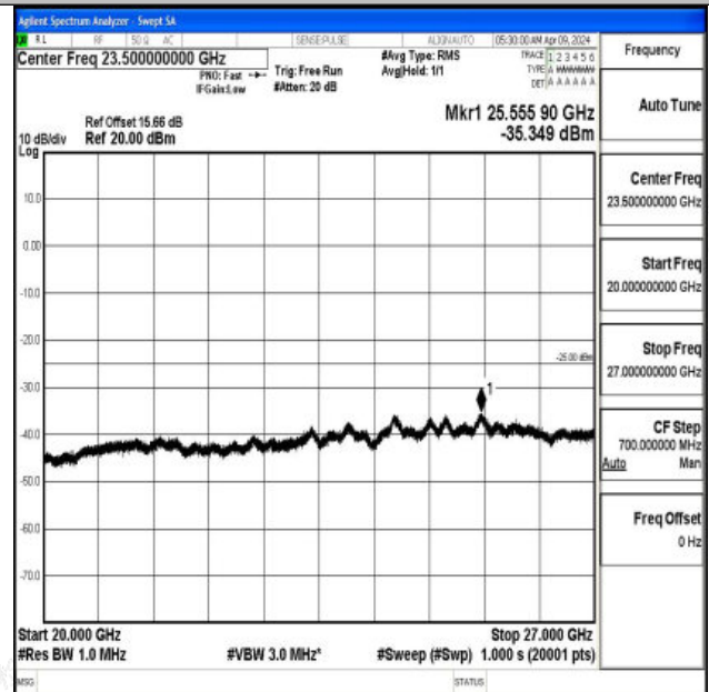
Band7_15MHz_16QAM_21100_1RB#0_20000~27000_200 00~27000
