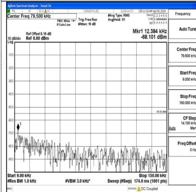
Band7_10MHz_QPSK_21400_1RB#0_0.009~0.15_0.009~0.15
