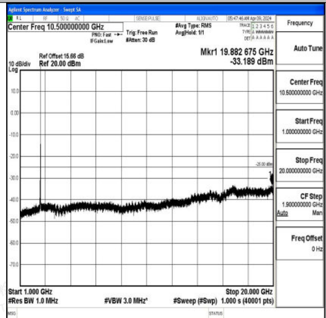
Band7_20MHz_QPSK_21100_1RB#0_1000~20000_1000~20000
