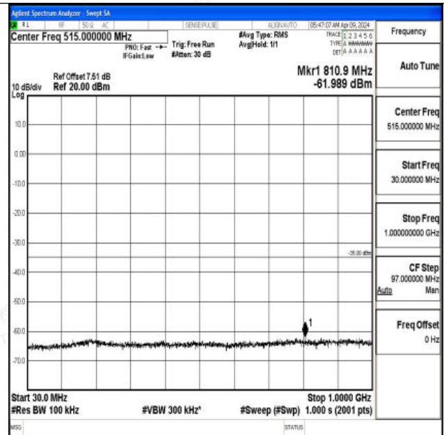
Band7_20MHz_16QAM_20850_1RB#0_30~1000_30~1000
