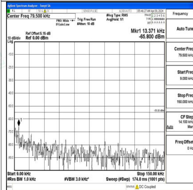
Band7_20MHz_QPSK_20850_1RB#0_0.009~0.15_0.009~0.15
