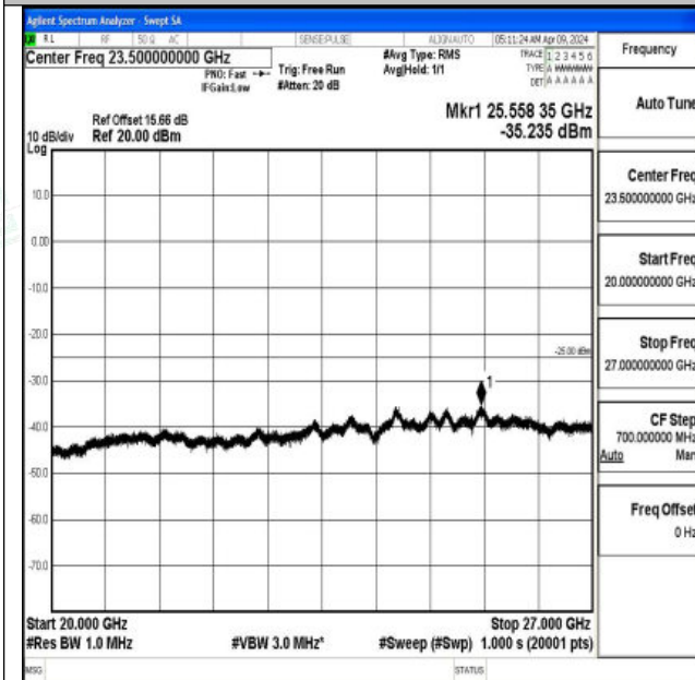
Band7_10MHz_QPSK_21400_1RB#0_20000~27000_20000~27000
