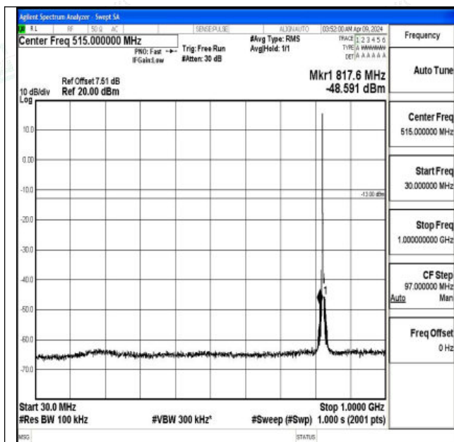
Band5_3MHz_QPSK_20415_1RB#0_30~1000_30~1000
