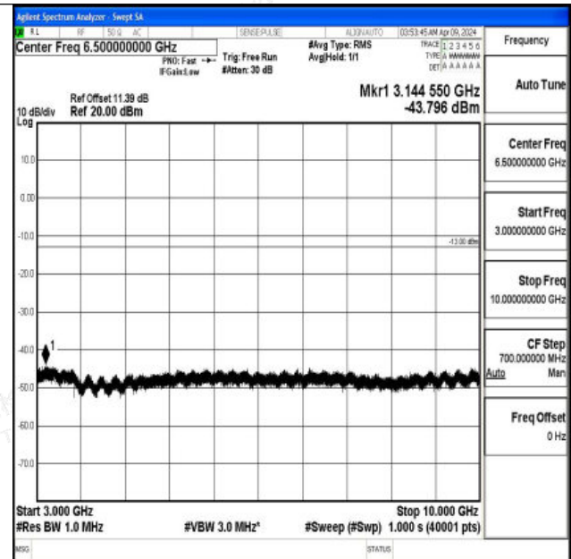
Band5_3MHz_16QAM_20525_1RB#0_3000~10000_3000~10000
