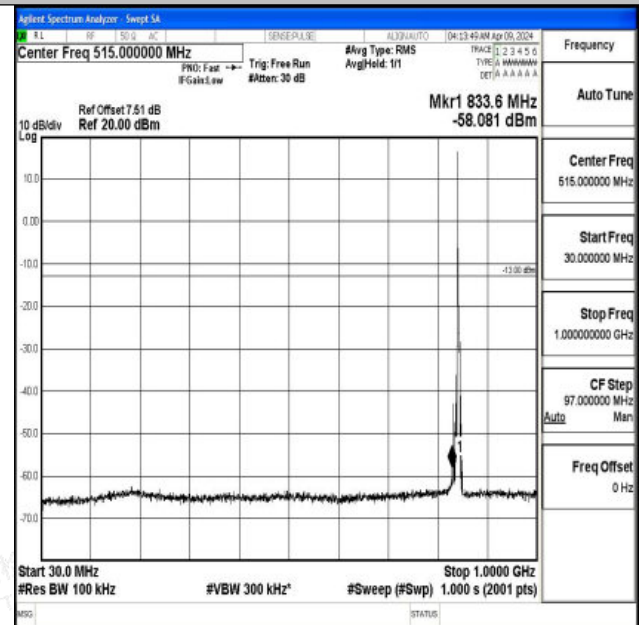
Band5_5MHz_16QAM_20625_1RB#0_30~1000_30~1000
