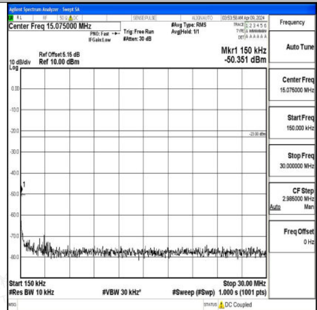
Band5_3MHz_QPSK_20635_1RB#0_0.15~30_0.15~30
