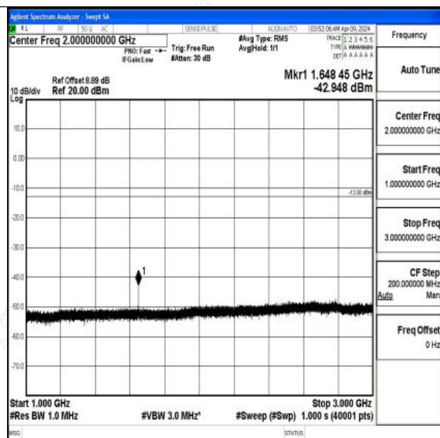
Band5_3MHz_QPSK_20415_1RB#0_1000~3000_1000~3000
