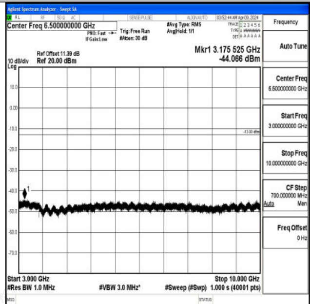
Band5_3MHz_16QAM_20415_1RB#0_3000~10000_3000~10000
