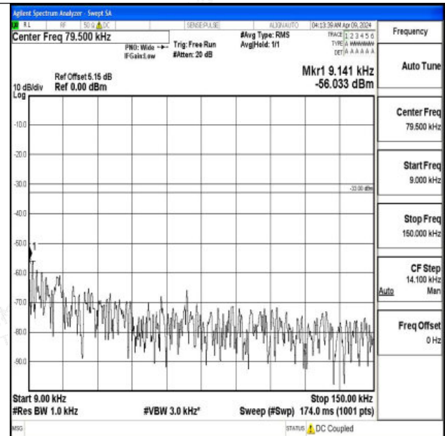
Band5_5MHz_16QAM_20625_1RB#0_0.009~0.15_0.009~0.15
