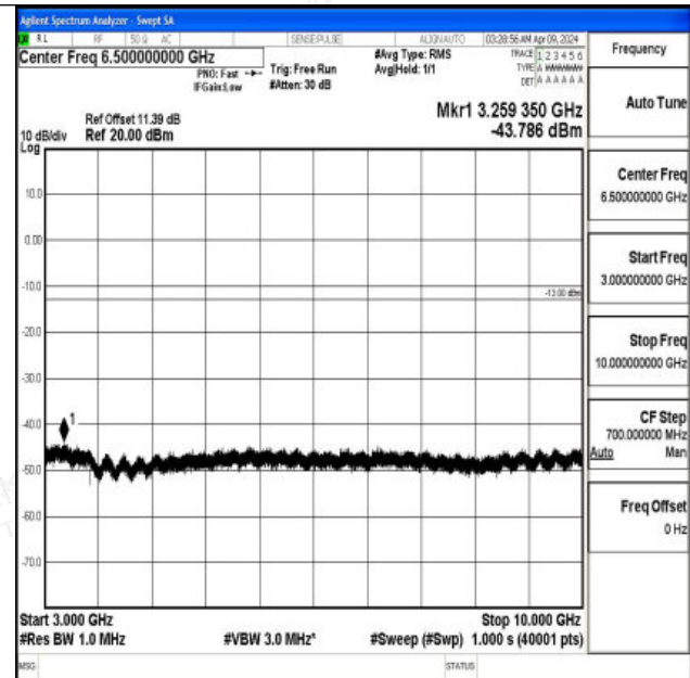
Band5_1.4MHz_16QAM_20643_1RB#0_3000~10000_3000 ~10000
