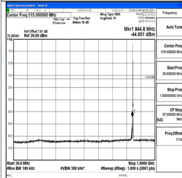
Band5_1.4MHz_QPSK_20643_1RB#0_30~1000_30~1000
