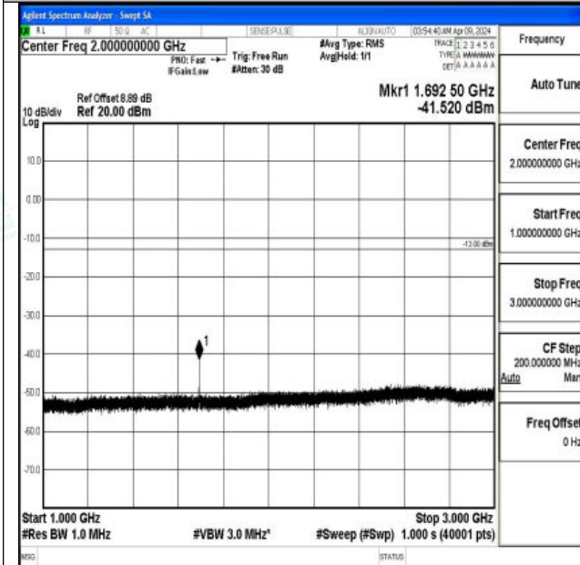
Band5_3MHz_16QAM_20635_1RB#0_1000~3000_1000~3000
