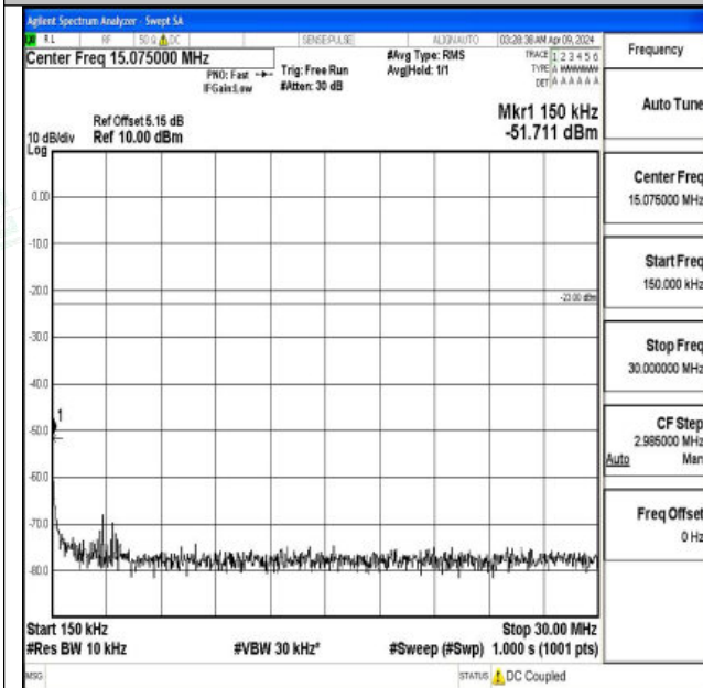
Band5_1.4MHz_16QAM_20643_1RB#0_0.15~30_0.15~30
