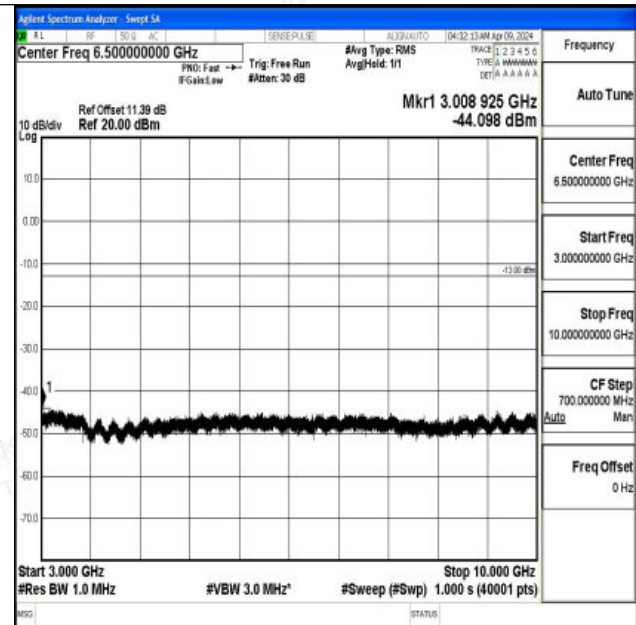
Band5_10MHz_16QAM_20525_1RB#0_3000~10000_3000 ~10000
