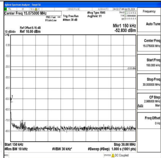
Band5_10MHz_QPSK_20600_1RB#0_0.15~30_0.15~30
