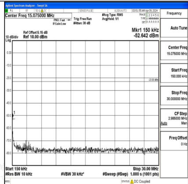
Band5_3MHz_QPSK_20415_1RB#0_0.15~30_0.15~30
