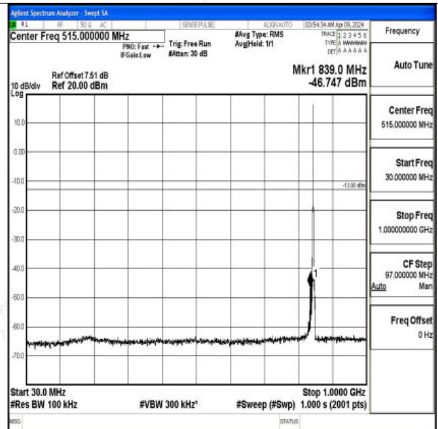
Band5_3MHz_16QAM_20635_1RB#0_30~1000_30~1000
