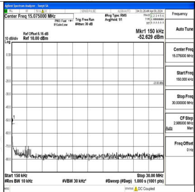
Band5_10MHz_QPSK_20525_1RB#0_0.15~30_0.15~30
