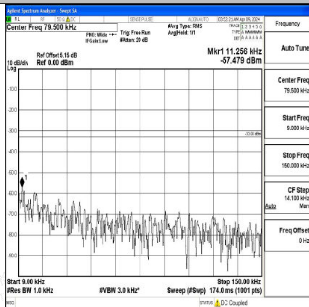
Band5_3MHz_16QAM_20415_1RB#0_0.009~0.15_0.009~0.15
