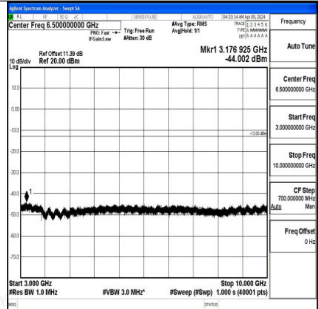
Band5_10MHz_16QAM_20600_1RB#0_3000~10000_3000 ~10000
