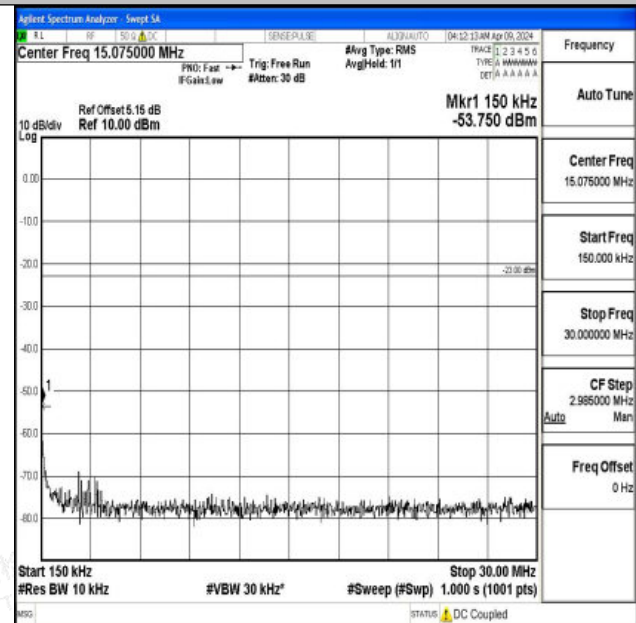
Band5_5MHz_QPSK_20525_1RB#0_0.15~30_0.15~30
