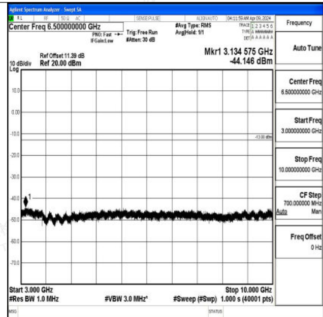
Band5_5MHz_16QAM_20425_1RB#0_3000~10000_3000~10000
