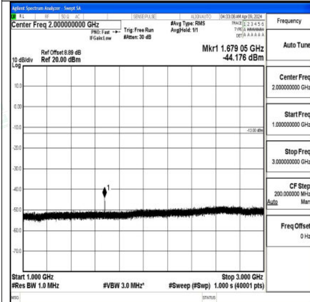
Band5_10MHz_16QAM_20600_1RB#0_1000~3000_1000 ~3000
