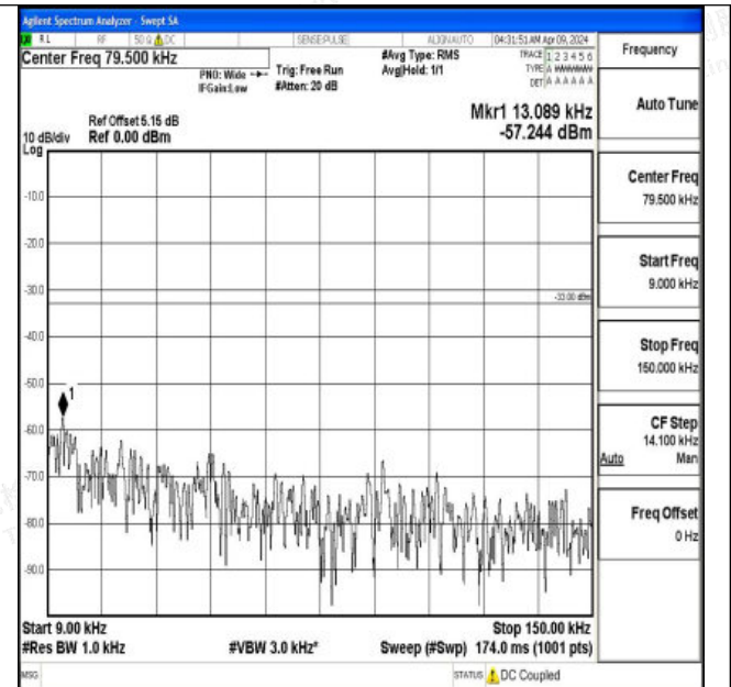
Band5_10MHz_16QAM_20525_1RB#0_0.009~0.15_0.009~0.15
