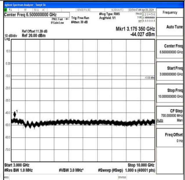
Band5_3MHz_16QAM_20635_1RB#0_3000~10000_3000~10000
