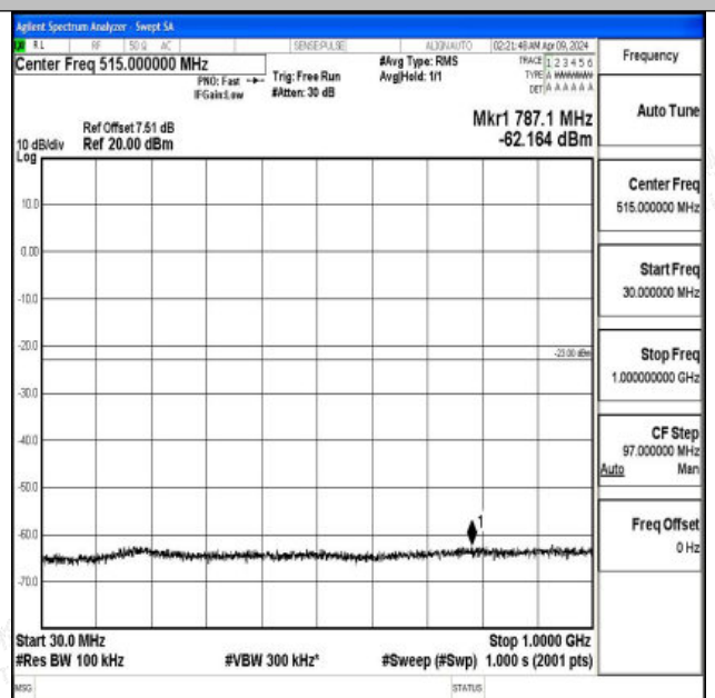
Band4 5MHz 16QAM 20375 1RB#0 30~1000 30~1000
