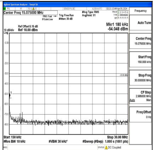
Band4_5MHz_QPSK_20375_1RB#0_0.15~30_0.15~30
