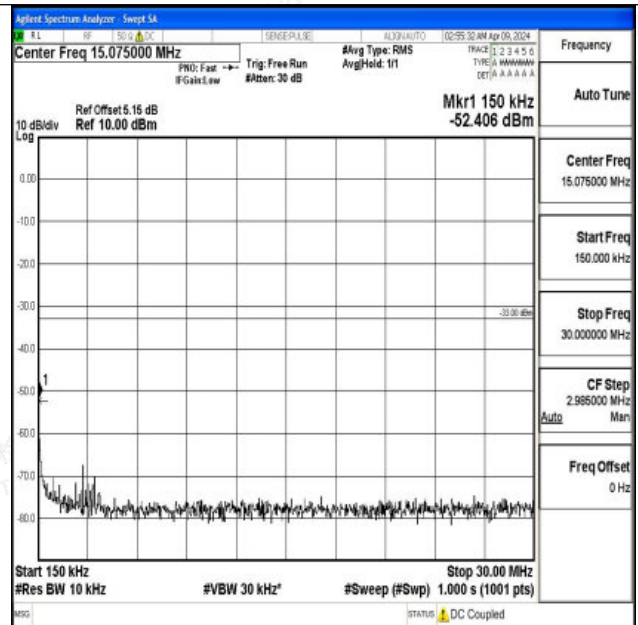
Band4_15MHz_QPSK_20325_1RB#0_0.15~30_0.15~30
