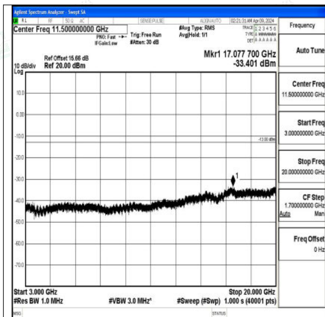
Band4_5MHz_QPSK_20375_1RB#0_3000~20000_3000~ 20000
