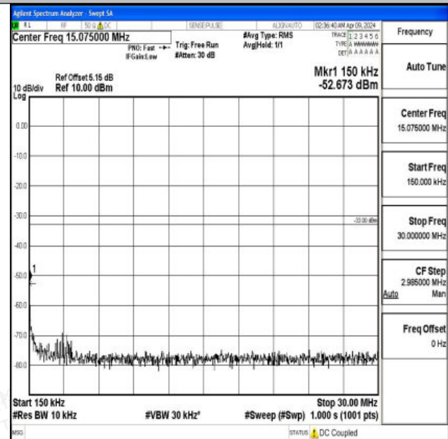
Band4_10MHz_QPSK_20000_1RB#0_0.15~30_0.15~30
