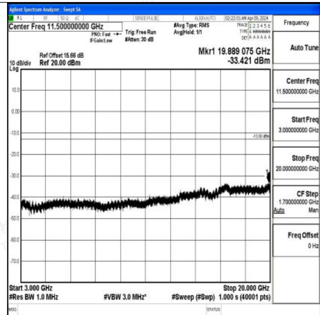
Band4_5MHz_16QAM_20375_1RB#0_3000~20000_3000~20000
