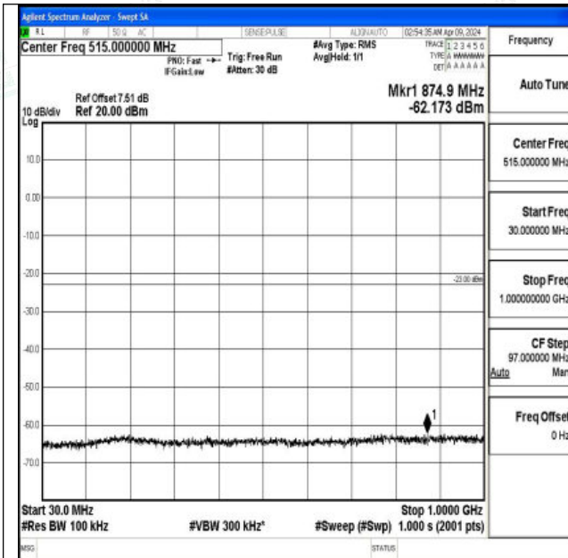
Band4_15MHz_QPSK_20175_1RB#0_30~1000_30~1000
