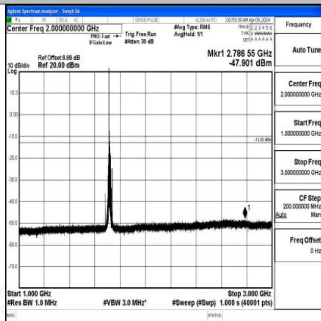
Band4_15MHz_QPSK_20025_1RB#0_1000~3000_1000~3000
