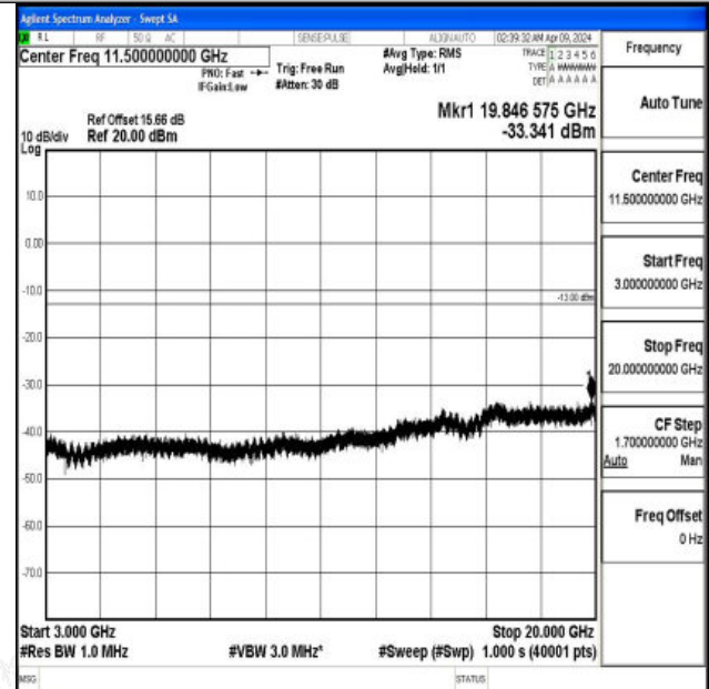
Band4_10MHz_16QAM_20350_1RB#0_3000~20000_3000~20000
