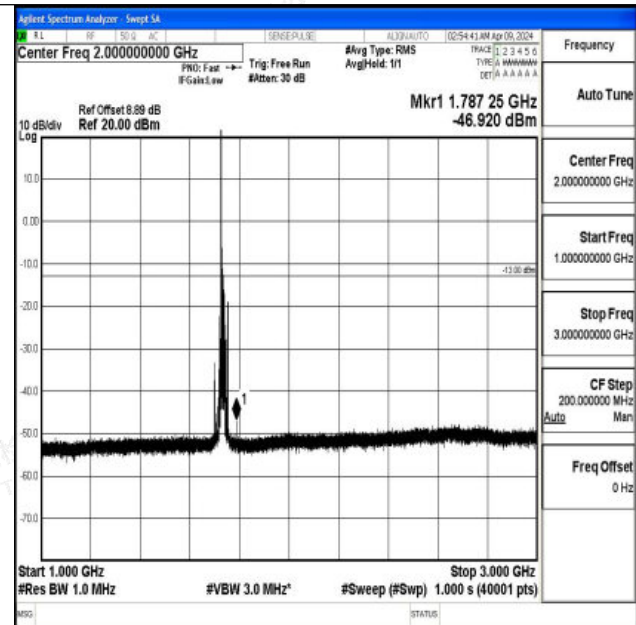
Band4_15MHz_QPSK_20175_1RB#0_1000~3000_1000~3000
