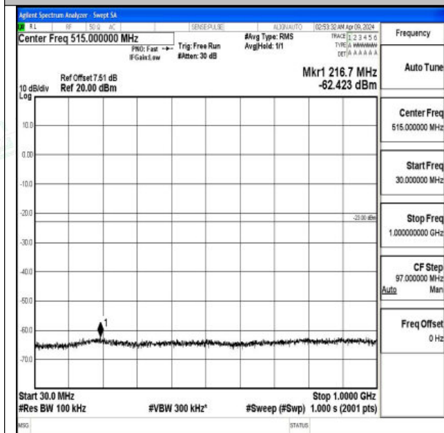
Band4_15MHz_QPSK_20025_1RB#0_30~1000_30~1000
