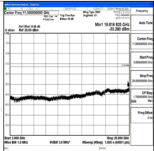
Band4_15MHz_16QAM_20025_1RB#0_3000~20000_3000 ~20000
