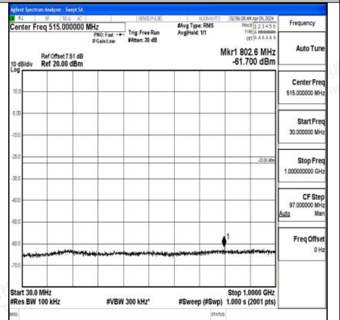
Band4_15MHz_16QAM_20325_1RB#0_30~1000_30~1000
