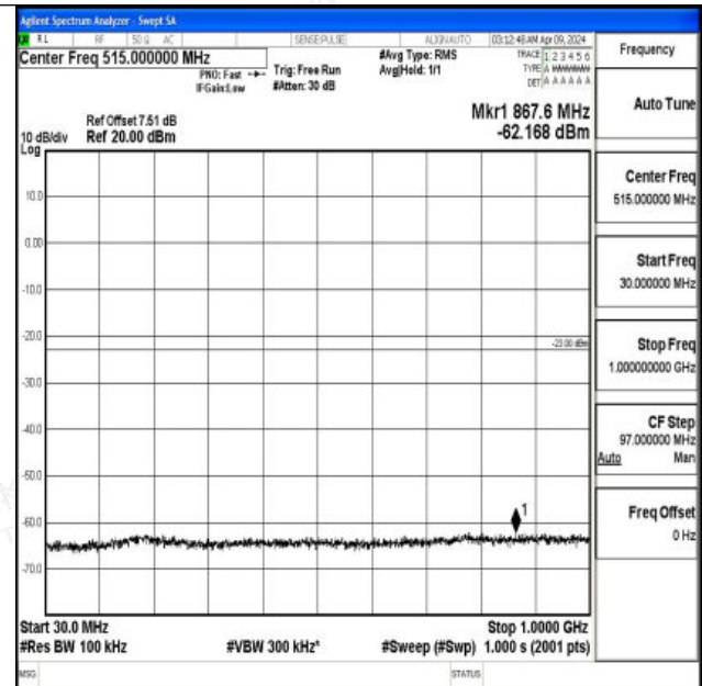
Band4_20MHz_16QAM_20300_1RB#0_30~1000_30~1000
