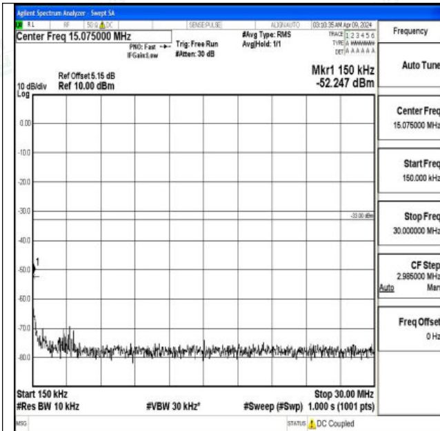
Band4_20MHz_16QAM_20050_1RB#0_0.15~30_0.15~30
