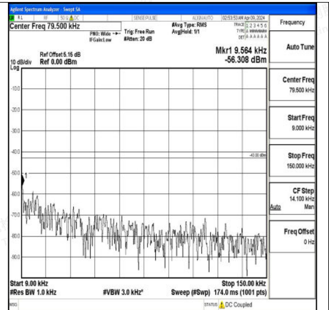
Band4_15MHz_16QAM_20025_1RB#0_0.009~0.15_0.009~0.15
