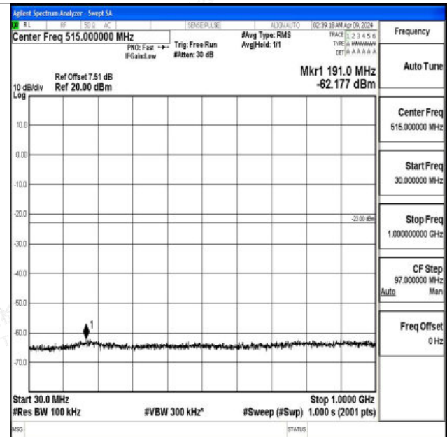
Band4_10MHz_16QAM_20350_1RB#0_30~1000_30~1000
