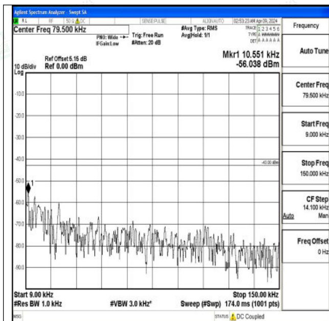
Band4_15MHz_QPSK_20025_1RB#0_0.009~0.15_0.009~0.15
