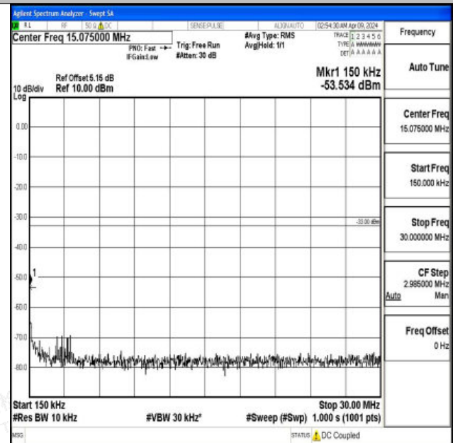
Band4_15MHz_QPSK_20175_1RB#0_0.15~30_0.15~30
