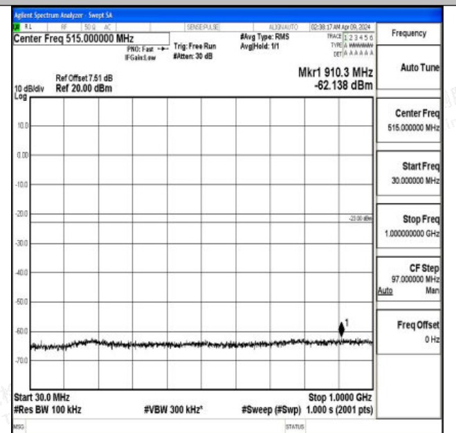
Band4_10MHz_16QAM_20175_1RB#0_30~1000_30~1000
