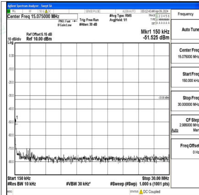
Band4_20MHz_16QAM_20300_1RB#0_0.15~30_0.15~30
