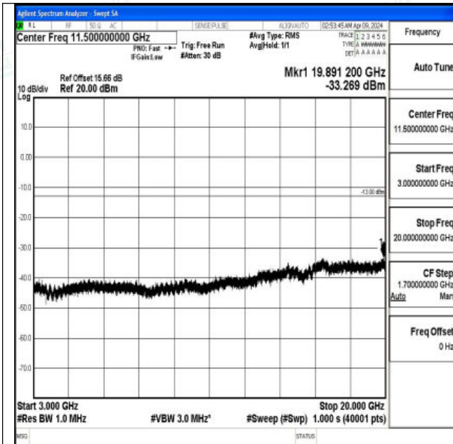
Band4_15MHz_QPSK_20025_1RB#0_3000~20000_3000~20000
