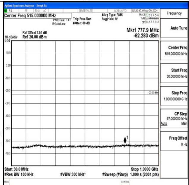
Band4_5MHz_16QAM_20175_1RB#0_30~1000_30~1000
