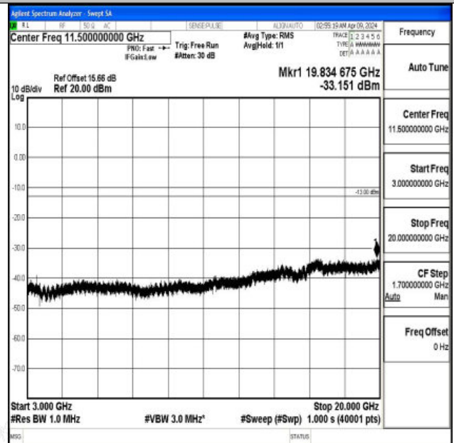
Band4_15MHz_16QAM_20175_1RB#0_3000~20000_3000~20000
