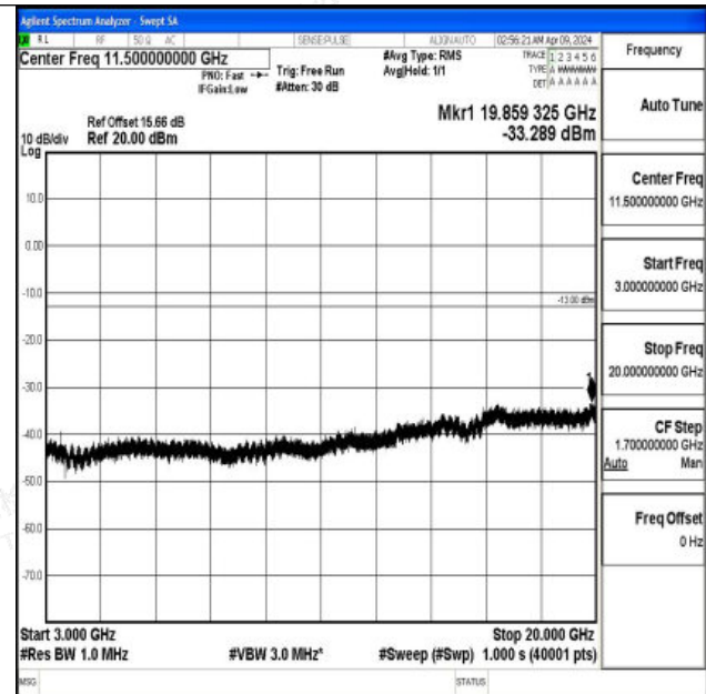
Band4_15MHz_16QAM_20325_1RB#0_3000~20000_3000 ~20000
