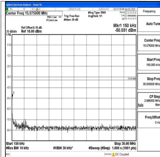
Band4_10MHz_16QAM_20000_1RB#0_0.15~30_0.15~30
