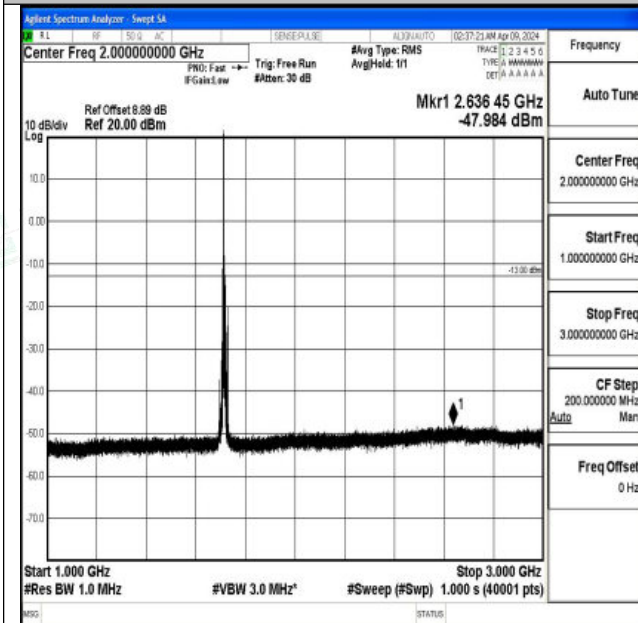
Band4_10MHz_16QAM_20000_1RB#0_1000~3000_1000~3000
