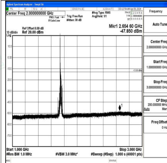
Band4_20MHz_16QAM_20300_1RB#0_1000~3000_1000~3000
