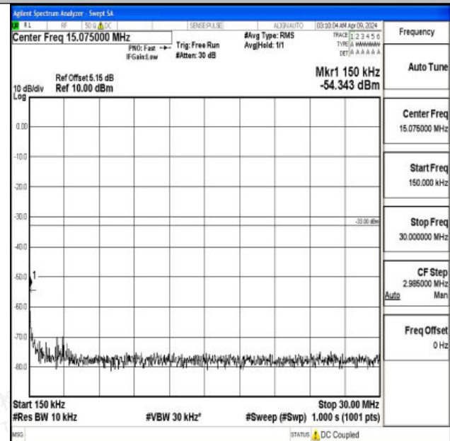
Band4_20MHz_QPSK_20050_1RB#0_0.15~30_0.15~30
