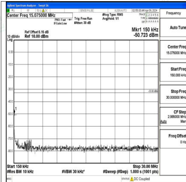
Band4_15MHz_16QAM_20175_1RB#0_0.15~30_0.15~30
