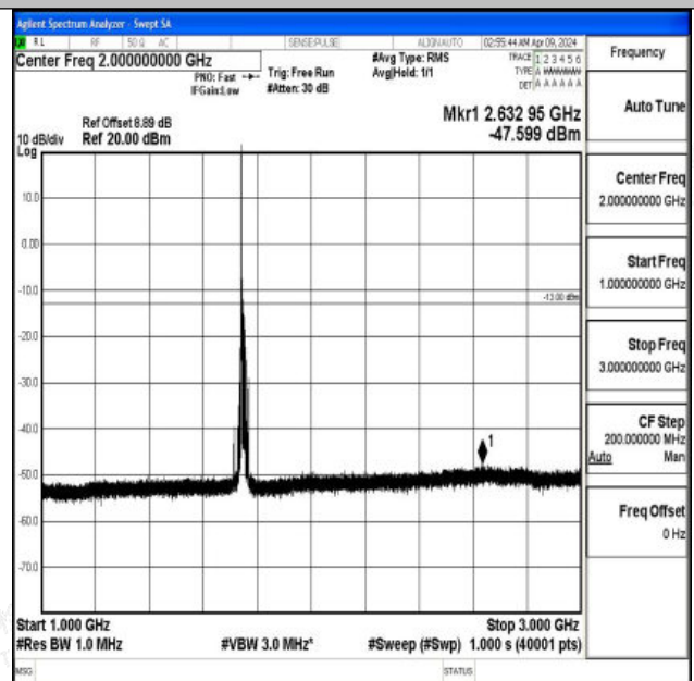
Band4_15MHz_QPSK_20325_1RB#0_1000~3000_1000~3000
