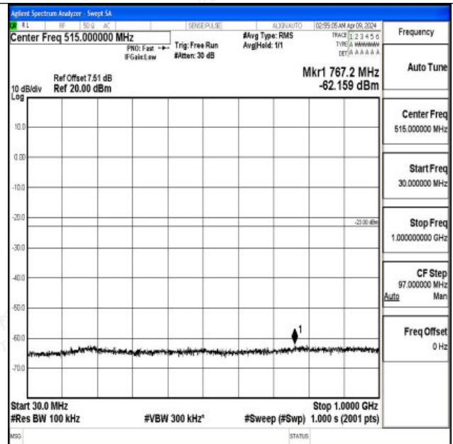
Band4_15MHz_16QAM_20175_1RB#0_30~1000_30~1000
