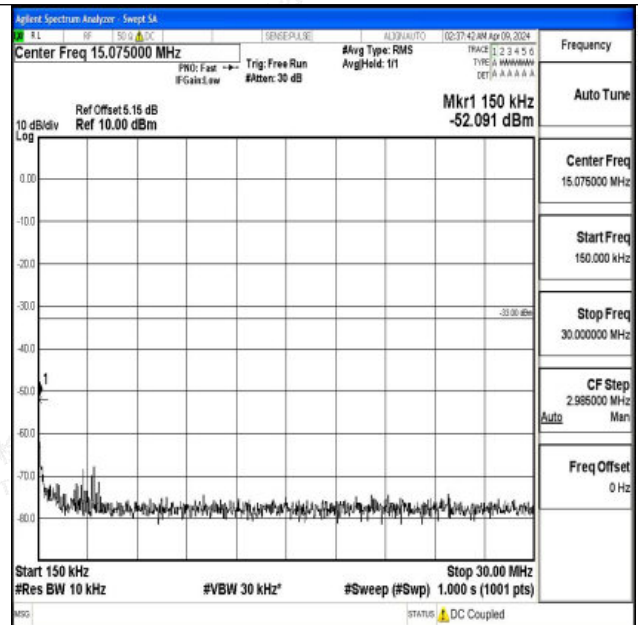
Band4_10MHz_QPSK_20175_1RB#0_0.15~30_0.15~30
