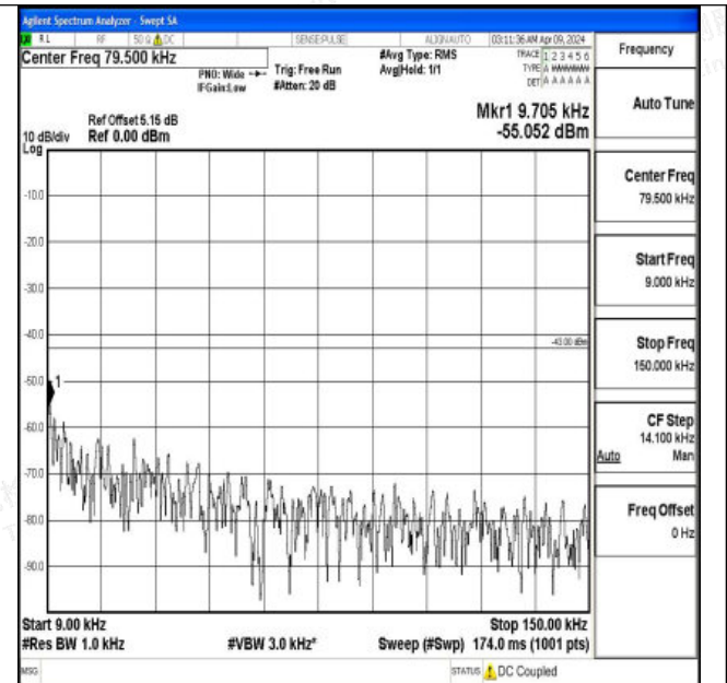
Band4_20MHz_16QAM_20175_1RB#0_0.009~0.15_0.009~0.15
