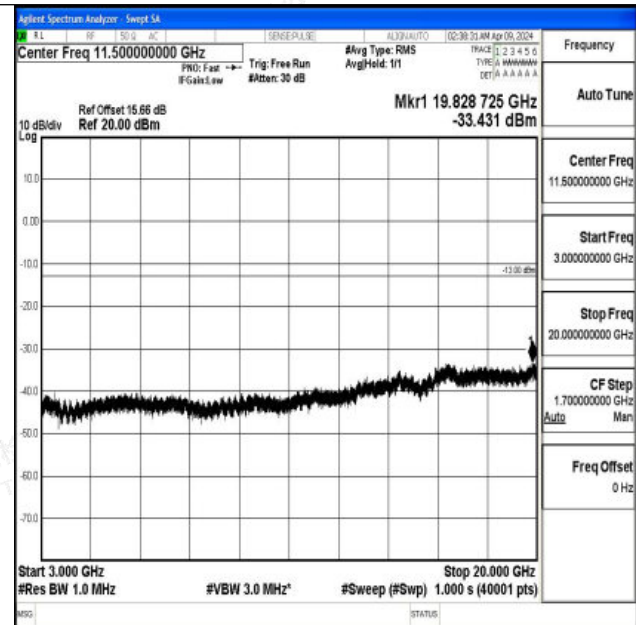
Band4_10MHz_16QAM_20175_1RB#0_3000~20000_3000 ~20000
