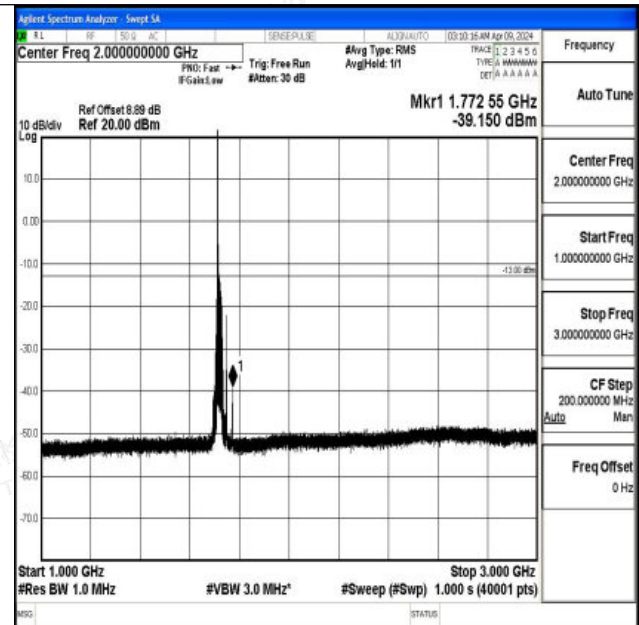
Band4_20MHz_QPSK_20050_1RB#0_1000~3000_1000~3000
