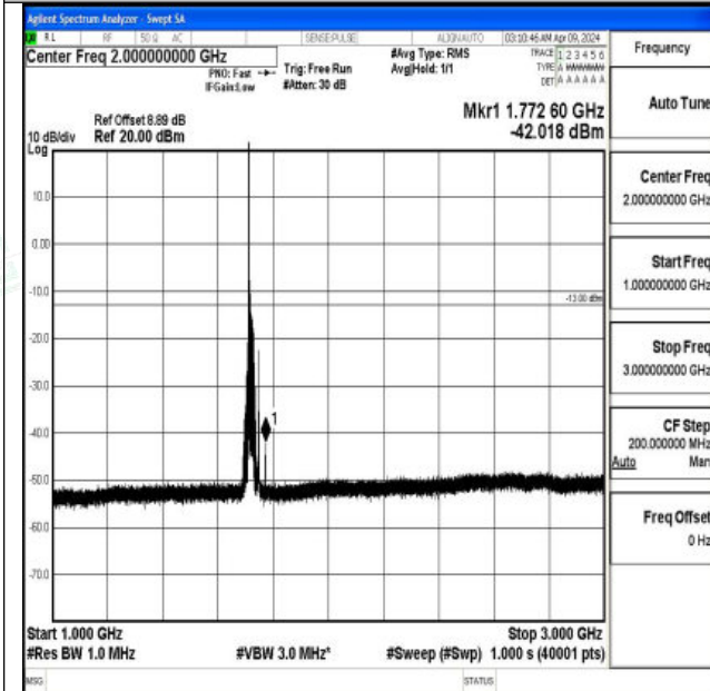
Band4_20MHz_16QAM_20050_1RB#0_1000~3000_1000~3000
