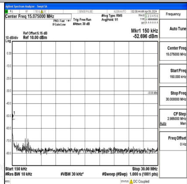
Band4_10MHz_QPSK_20350_1RB#0_0.15~30_0.15~30
