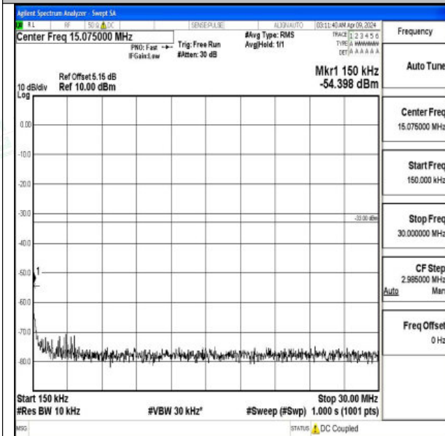
Band4_20MHz_16QAM_20175_1RB#0_0.15~30_0.15~30
