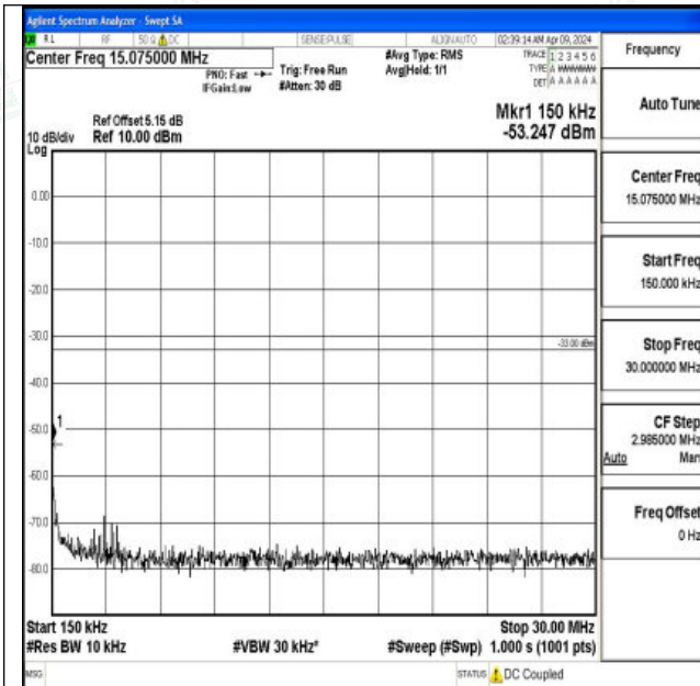
Band4_10MHz_16QAM_20350_1RB#0_0.15~30_0.15~30
