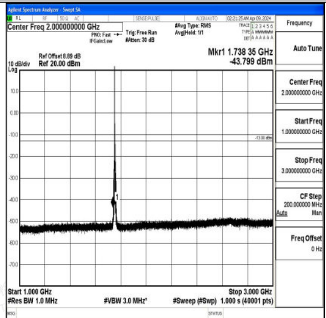
Band4_5MHz_QPSK_20375_1RB#0_1000~3000_1000~3000 00
