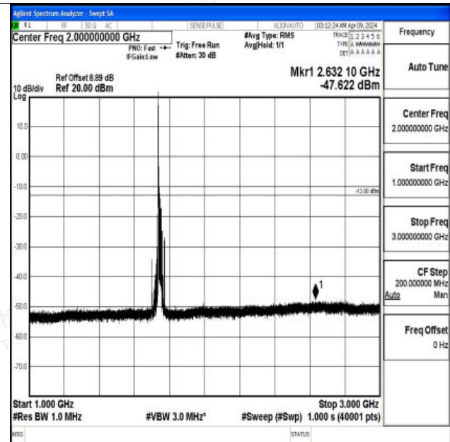
Band4_20MHz_QPSK_20300_1RB#0_1000~3000_1000~3000
