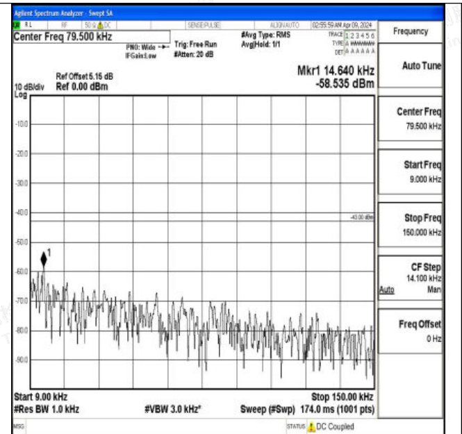
Band4_15MHz_16QAM_20325_1RB#0_0.009~0.15_0.009~0.15
