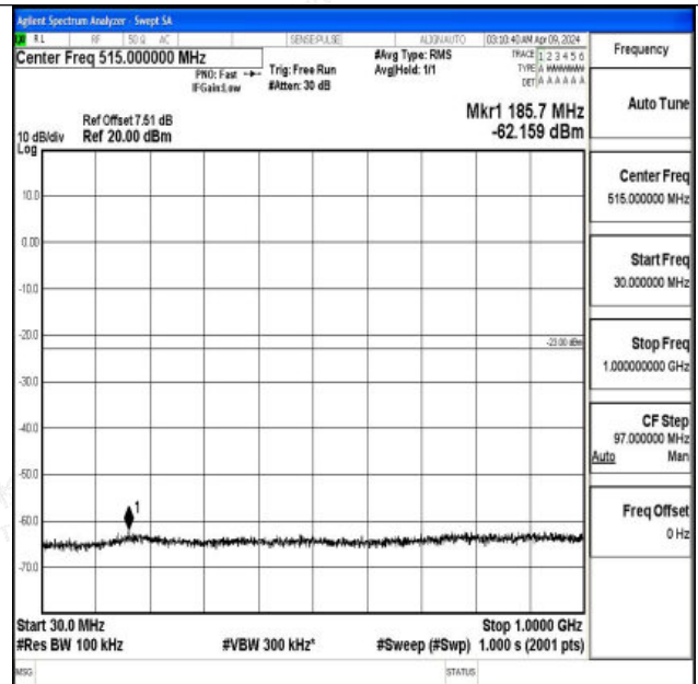
Band4_20MHz_16QAM_20050_1RB#0_30~1000_30~1000
