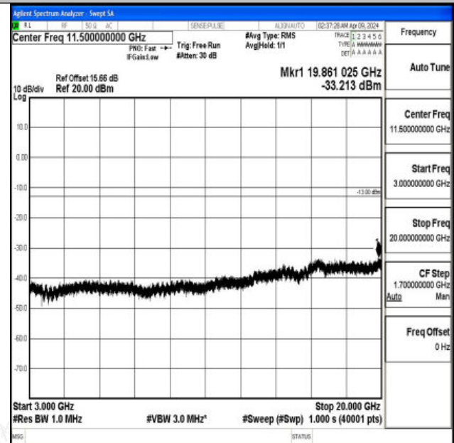
Band4_10MHz_16QAM_20000_1RB#0_3000~20000_3000~20000
