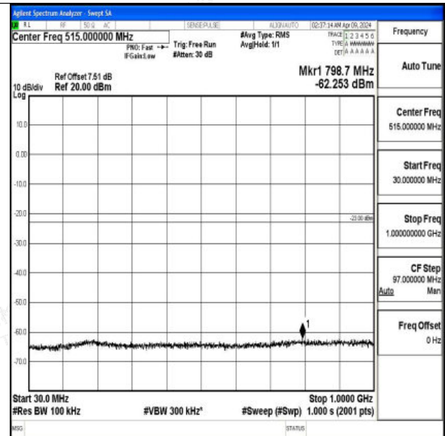
Band4_10MHz_16QAM_20000_1RB#0_30~1000_30~1000
