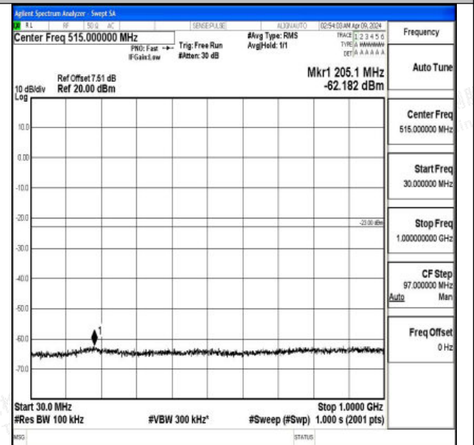
Band4_15MHz_16QAM_20025_1RB#0_30~1000_30~1000
