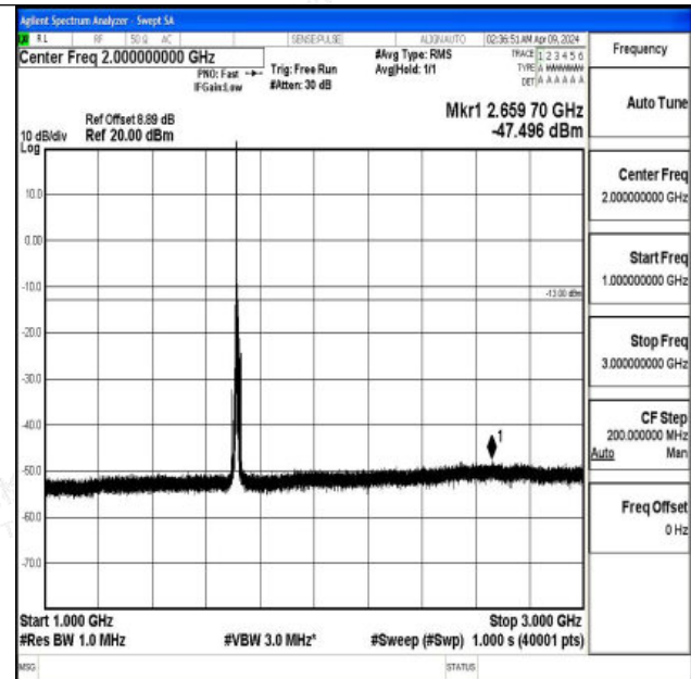
Band4_10MHz_QPSK_20000_1RB#0_1000~3000_1000~3000
