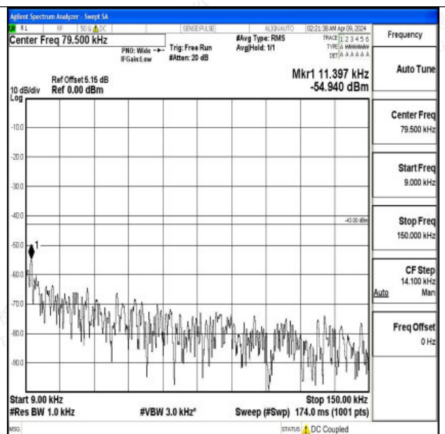
Band4_5MHz_16QAM_20375_1RB#0_0.009~0.15_0.009~0.15
