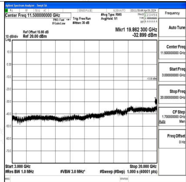
Band4_20MHz_16QAM_20175_1RB#0_3000~20000_3000 ~20000
