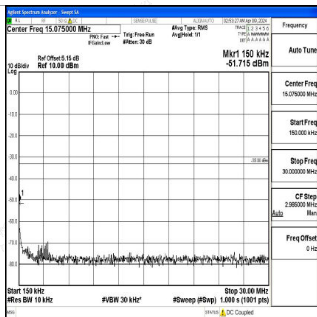
Band4_15MHz_QPSK_20025_1RB#0_0.15~30_0.15~30
