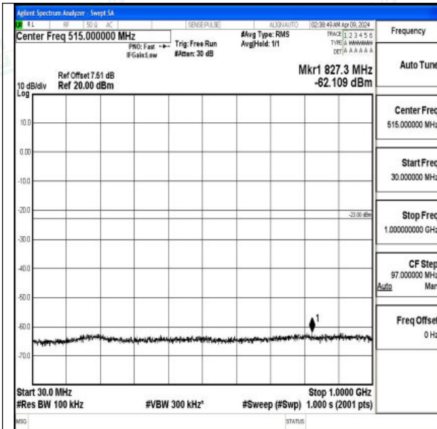
Band4_10MHz_QPSK_20350_1RB#0_30~1000_30~1000
