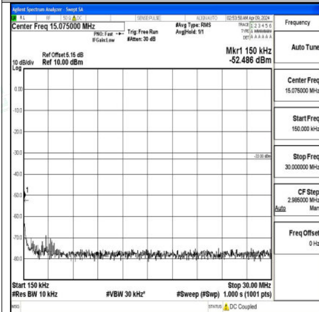
Band4_15MHz_16QAM_20025_1RB#0_0.15~30_0.15~30
