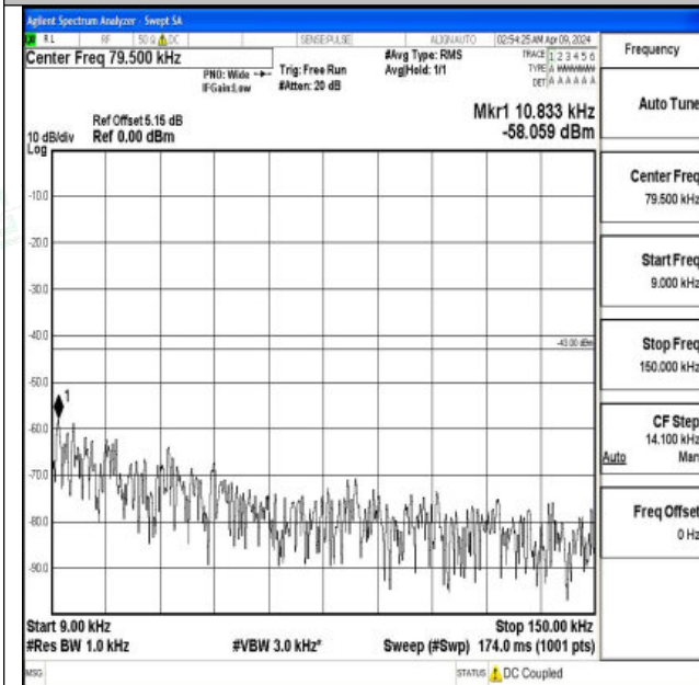
Band4_15MHz_QPSK_20175_1RB#0_0.009~0.15_0.009~ 0.15
