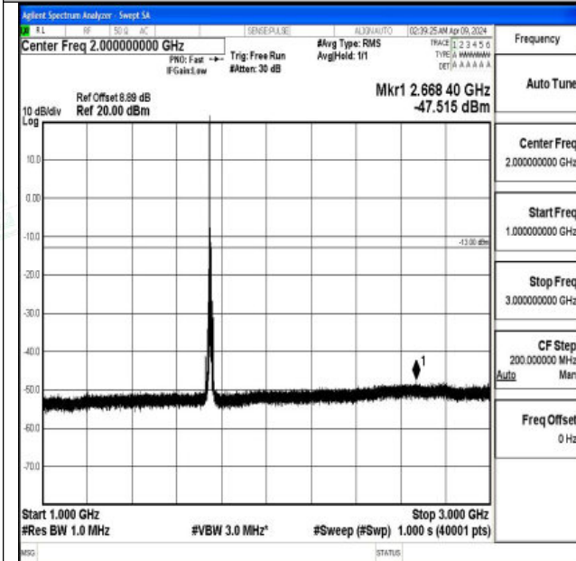
Band4_10MHz_16QAM_20350_1RB#0_1000~3000_1000~3000
