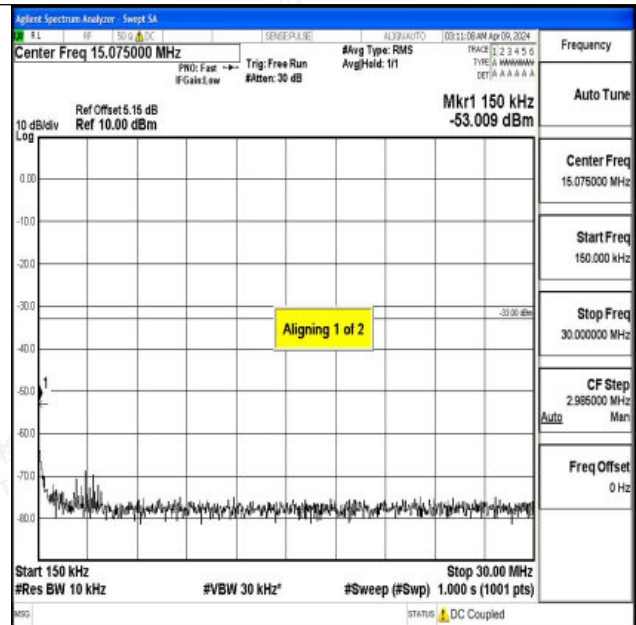
Band4_20MHz_QPSK_20175_1RB#0_0.15~30_0.15~30
