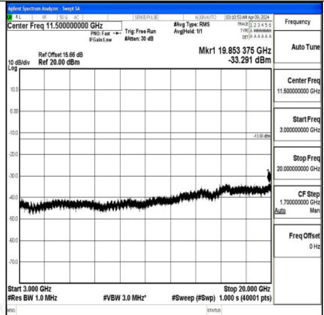
Band4_20MHz_16QAM_20050_1RB#0_3000~20000_3000~20000
