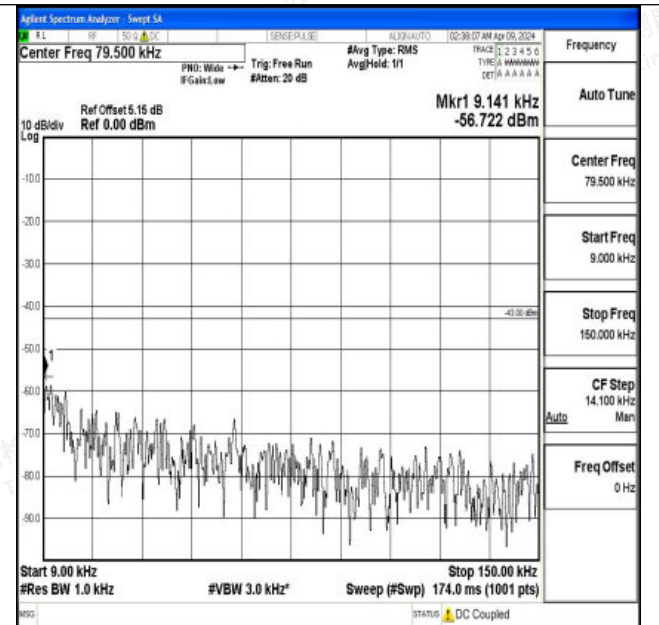
Band4_10MHz_16QAM_20175_1RB#0_0.009~0.15_0.009~0.15
