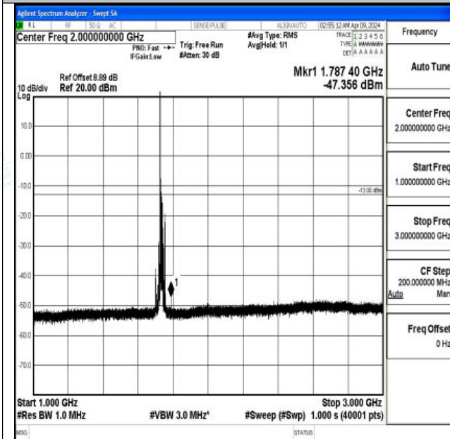
Band4_15MHz_16QAM_20175_1RB#0_1000~3000_1000~3000
