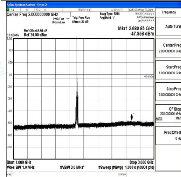
Band2_10MHz_16QAM_19150_1RB#0_1000~3000_1000~3000
