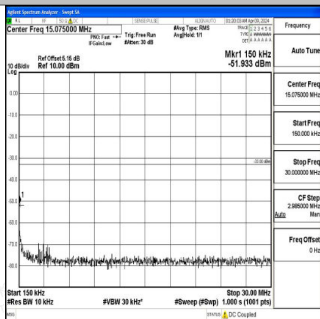
Band2_20MHz_QPSK_18700_1RB#0_0.15~30_0.15~30
