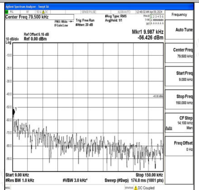
Band2_10MHz_16QAM_18650_1RB#0_0.009~0.15_0.009~0.15
