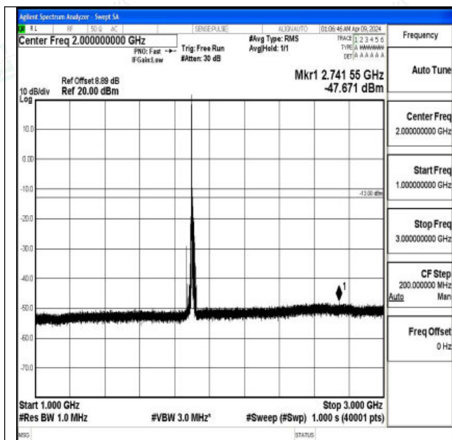
Band2_15MHz_16QAM_19125_1RB#0_1000~3000_1000 ~3000
