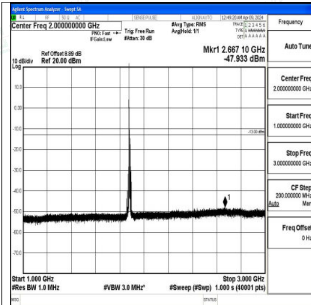
Band2_10MHz_16QAM_18900_1RB#0_1000~3000_1000 ~3000
