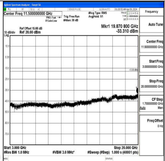
Band2_20MHz_16QAM_18700_1RB#0_3000~20000_3000~20000
