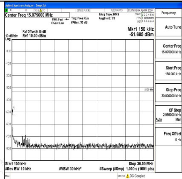
Band2_15MHz_QPSK_18900_1RB#0_0.15~30_0.15~30
