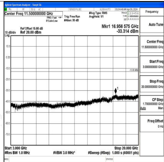
Band2_15MHz_16QAM_18675_1RB#0_3000~20000_3000 ~20000
