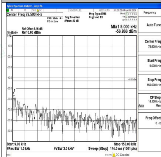
Band2_20MHz_QPSK_18700_1RB#0_0.009~0.15_0.009~ 0.15
