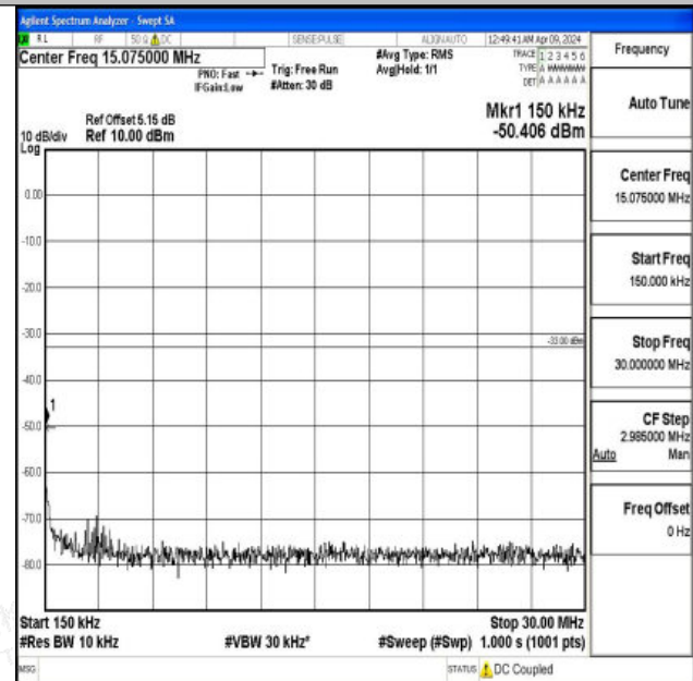
Band2_10MHz_QPSK_19150_1RB#0_0.15~30_0.15~30
