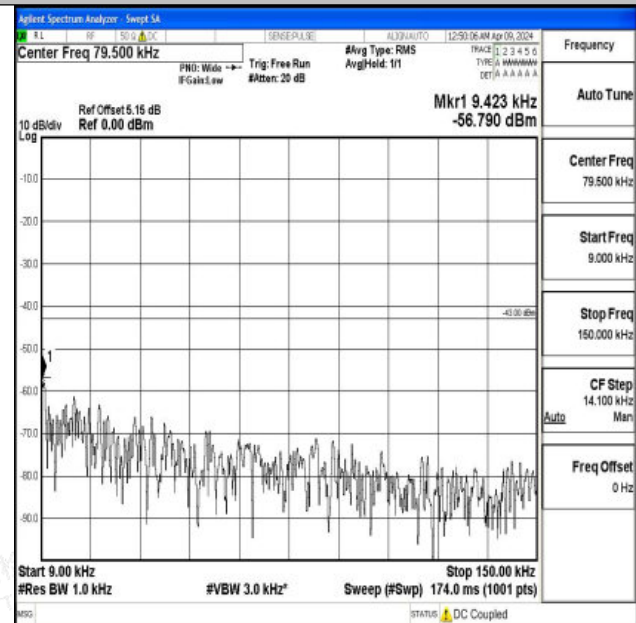
Band2_10MHz_16QAM_19150_1RB#0_0.009~0.15_0.009~0.15
