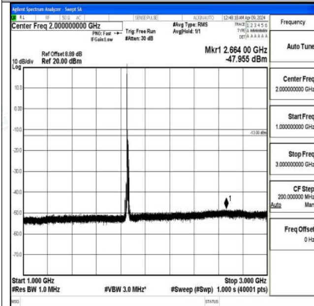
Band2_10MHz_16QAM_18650_1RB#0_1000~3000_1000 ~3000
