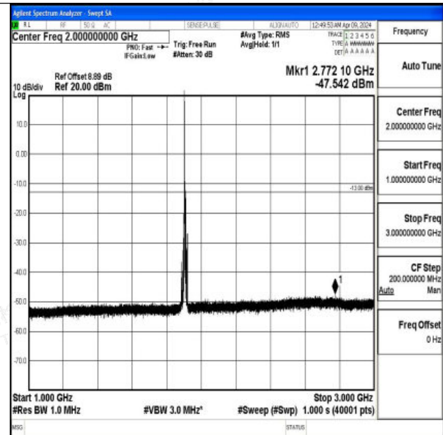
Band2_10MHz_QPSK_19150_1RB#0_1000~3000_1000~3000
