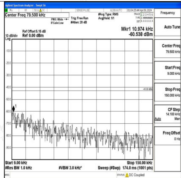
Band2_15MHz_16QAM_18675_1RB#0_0.009~0.15_0.009~0.15
