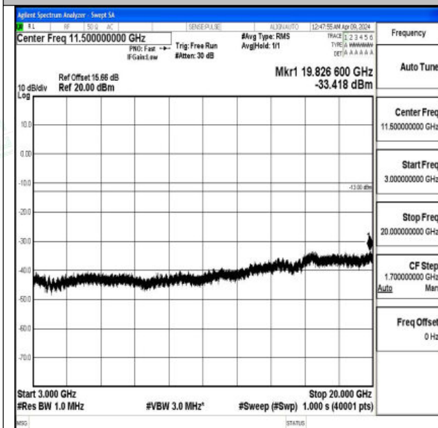
Band2_10MHz_QPSK_18650_1RB#0_3000~20000_3000~20000
