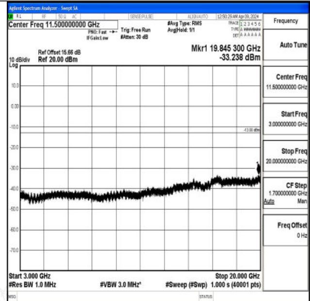
Band2_10MHz_16QAM_19150_1RB#0_3000~20000_3000~20000
