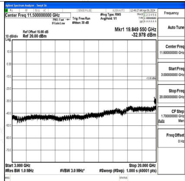
Band2_10MHz_16QAM_18900_1RB#0_3000~20000_3000 ~20000
