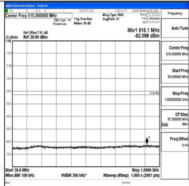
Band2_15MHz_16QAM_18675_1RB#0_30~1000_30~1000
