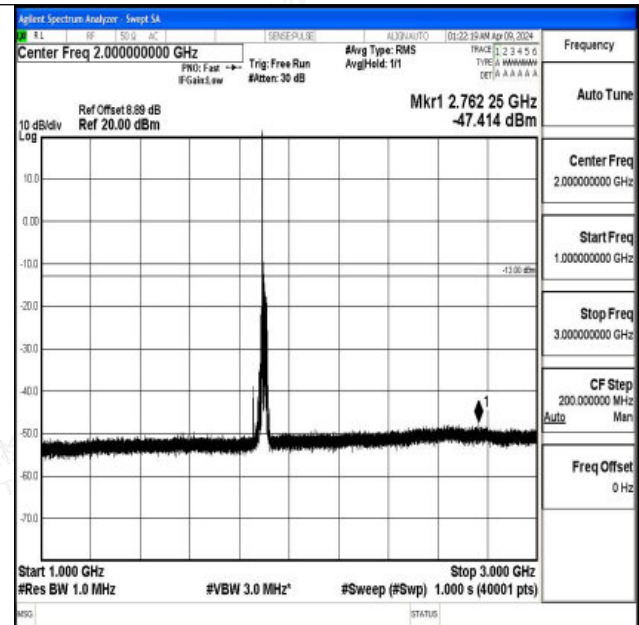
Band2_20MHz_QPSK_19100_1RB#0_1000~3000_1000~3000
