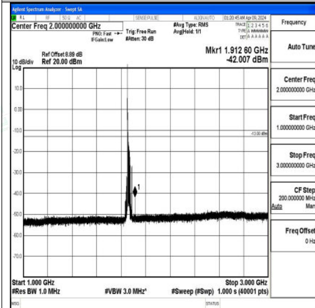
Band2_20MHz_16QAM_18700_1RB#0_1000~3000_1000~3000
