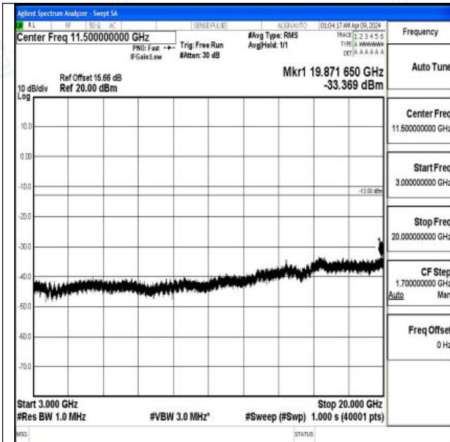
Band2_15MHz_QPSK_18675_1RB#0_3000~20000_3000~20000
