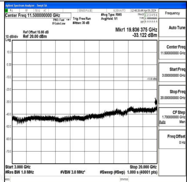
Band2_10MHz_16QAM_18650_1RB#0_3000~20000_3000 ~20000
