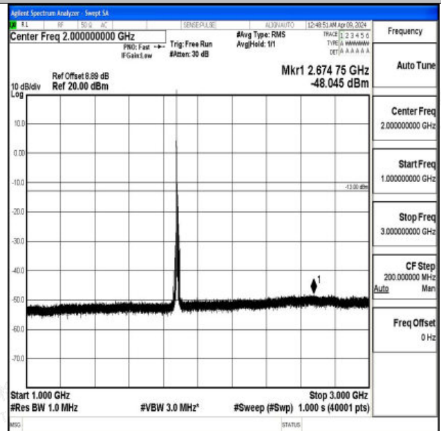
Band2_10MHz_QPSK_18900_1RB#0_1000~3000_1000~3000
