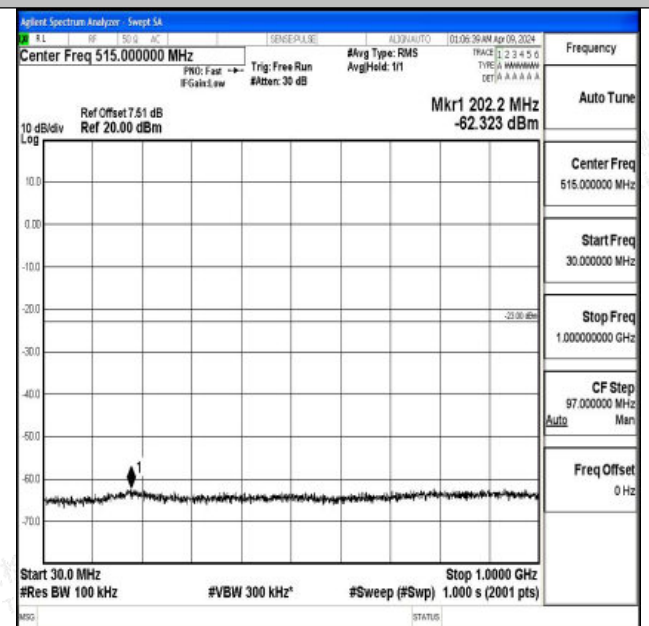
Band2_15MHz_16QAM_19125_1RB#0_30~1000_30~1000
