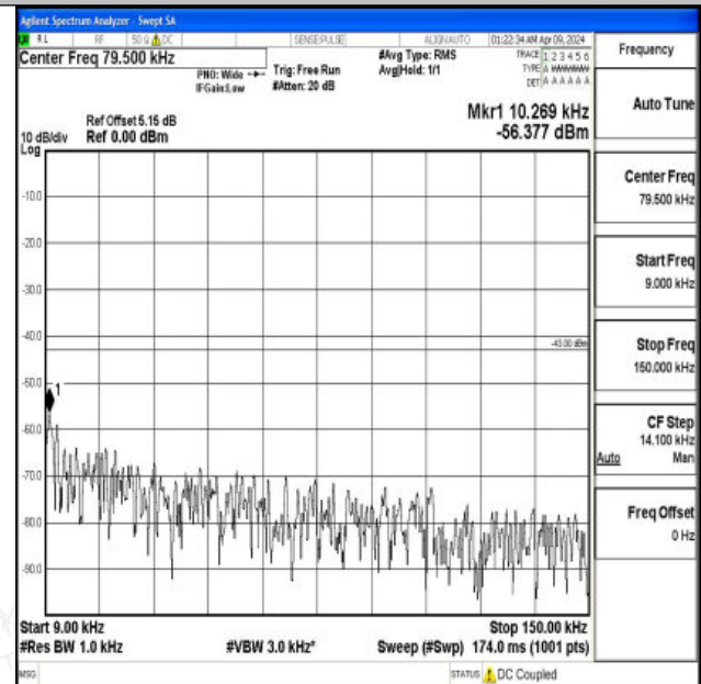
Band2_20MHz_16QAM_19100_1RB#0_0.009~0.15_0.009~0.15
