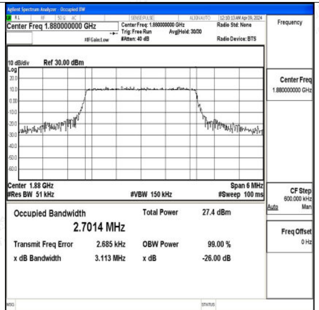
Band2-3MHz-16QAM-18900-15RB#0-PASS
