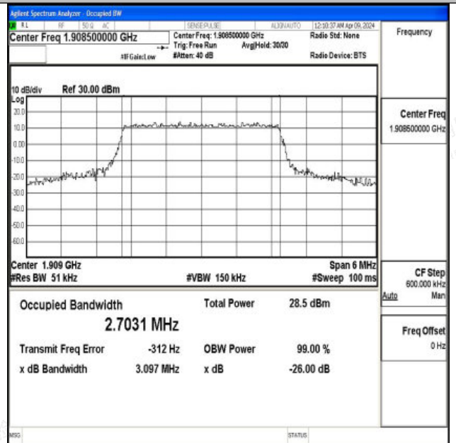
Band2-3MHz-16QAM-19185-15RB#0-PASS
