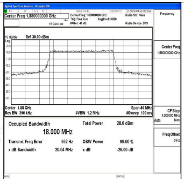
Band2-20MHz-16QAM-18900-100RB#0-PASS
