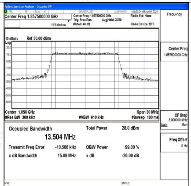
Band2-15MHz-16QAM-18675-75RB#0-PASS
