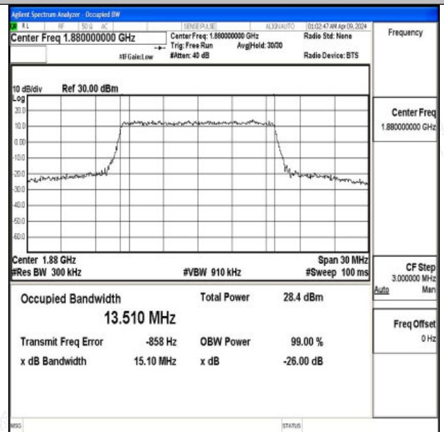
Band2-15MHz-16QAM-18900-75RB#0-PASS
