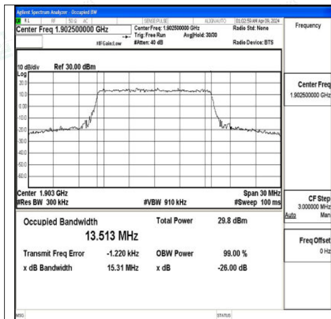
Band2-15MHz-QPSK-19125-75RB#0-PASS
