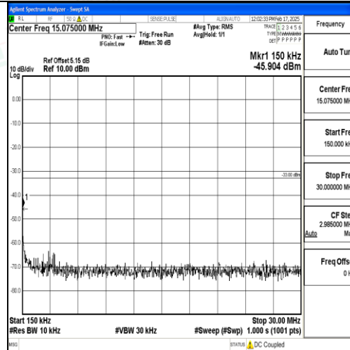
Band66_15MHz_16QAM_132047_1RB#0_0.15~30_0.15~30
