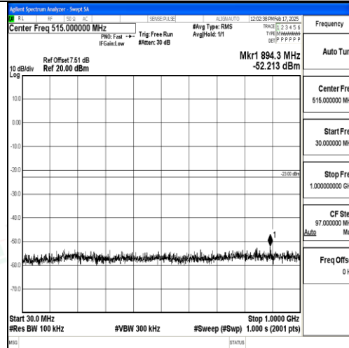
Band66_15MHz_16QAM_132047_1RB#0_30~1000_30~1000
