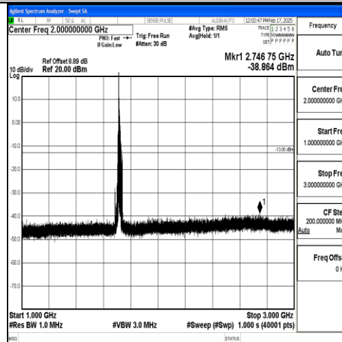
Band66_15MHz_16QAM_132047_1RB#0_1000~3000_1000~3000
