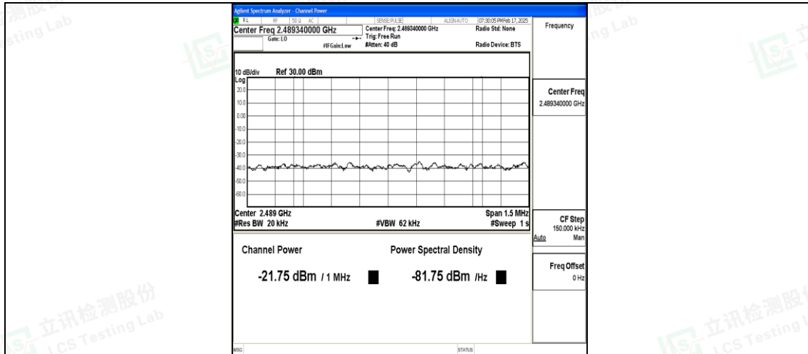
Band41_20MHz_16QAM_39750_100RB#0_Final1
