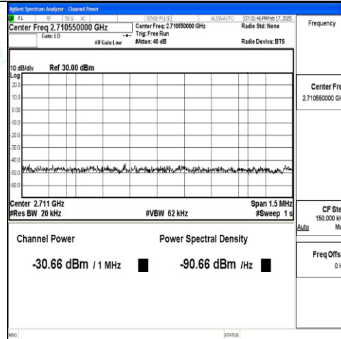
Band41_20MHz_16QAM_41490_100RB#0_Final1
