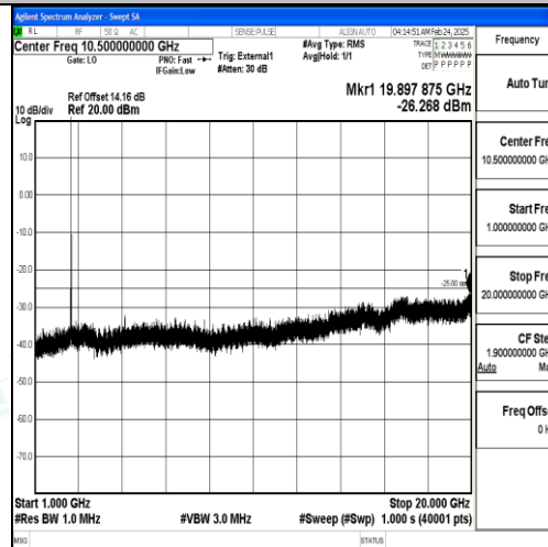
Band38_20MHz_16QAM_37850_1RB#0_1000~20000_1000~20000
