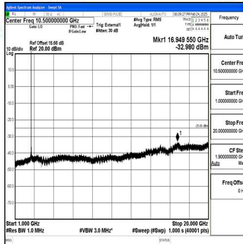
Band38_15MHz_QPSK_38000_1RB#0_1000~20000_1000~20000
