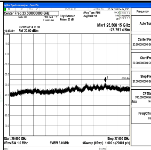
Band38_15MHz_QPSK_38000_1RB#0_20000~27000_20000~27000
