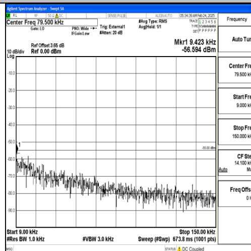
Band38_15MHz_16QAM_38000_1RB#0_0.009~0.15_0.009~0.15
