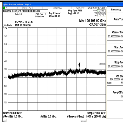
Band38_20MHz_16QAM_37850_1RB#0_20000~27000_20000~27000
