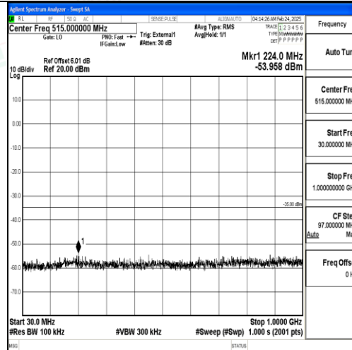
Band38_20MHz_16QAM_37850_1RB#0_30~1000_30~1000
