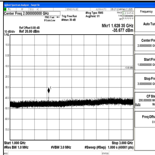
Band26_3MHz_16QAM_26705_1RB#0_1000~3000_1000~3000
