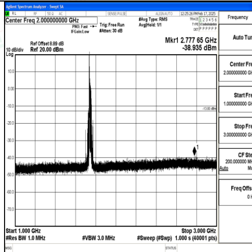
Band66_20MHz_16QAM_132322_1RB#0_1000~3000_1000~3000
