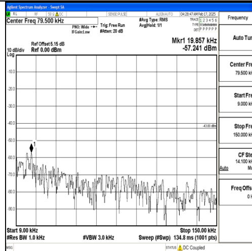
Band25_20MHz_16QAM_26140_1RB#0_0.009~0.15_0.009~0.15
