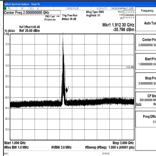
Band25_20MHz_QPSK_26140_1RB#0_1000~3000_1000~3000
