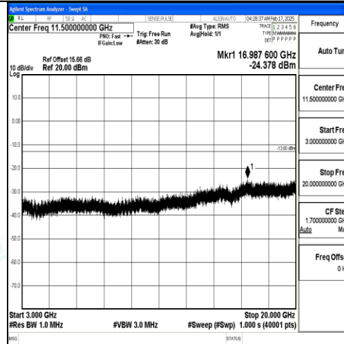
Band25_20MHz_QPSK_26140_1RB#0_3000~20000_3000~20000
